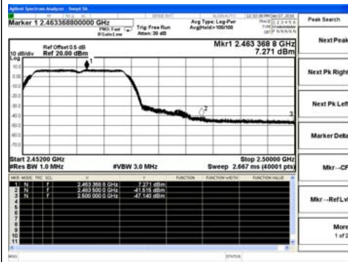
802.11g-High channel(Peak)
