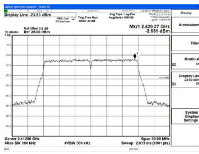
802.11n(HT20)-Low channel
