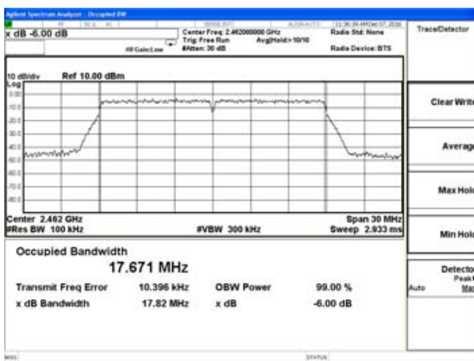
802.11n(HT20)-High channel
