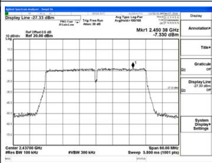
802.11n(HT40)-Middle channel
