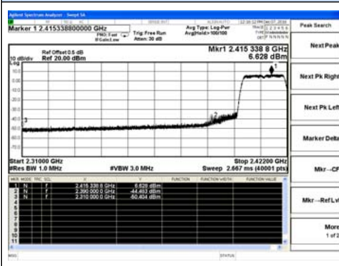
802.11n(HT20)-Low channel(Peak)
