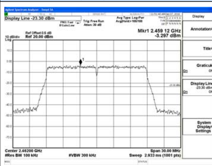
802.11n(HT20)-High channel
