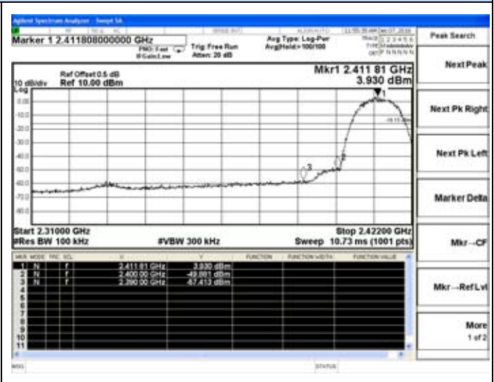
802.11b Low channel
