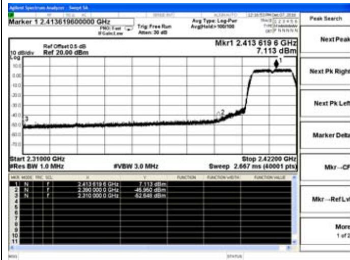
802.11g-Low channel(Peak)
