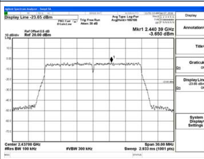
802.11n(HT20)-Middle channel
