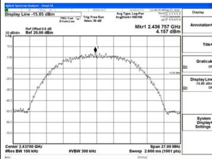
802.11b-Middle channel
