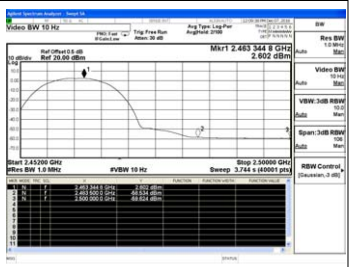
802.11b-High channel(Average)
