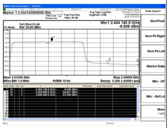
802.11n(HT40)-High channel(Average)
