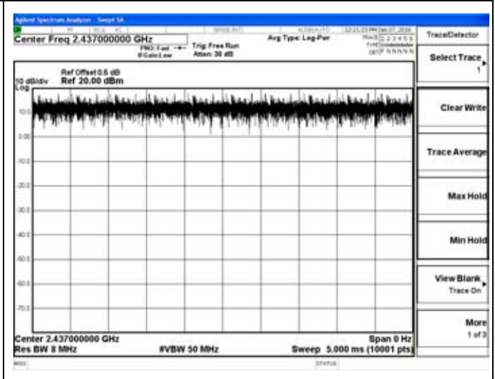
802.11g
