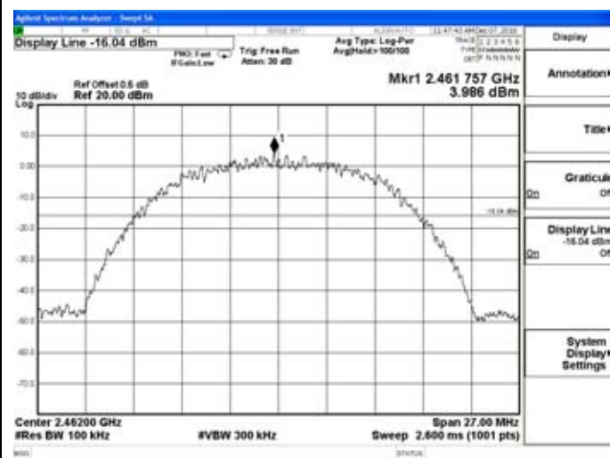
802.11b-High channel
