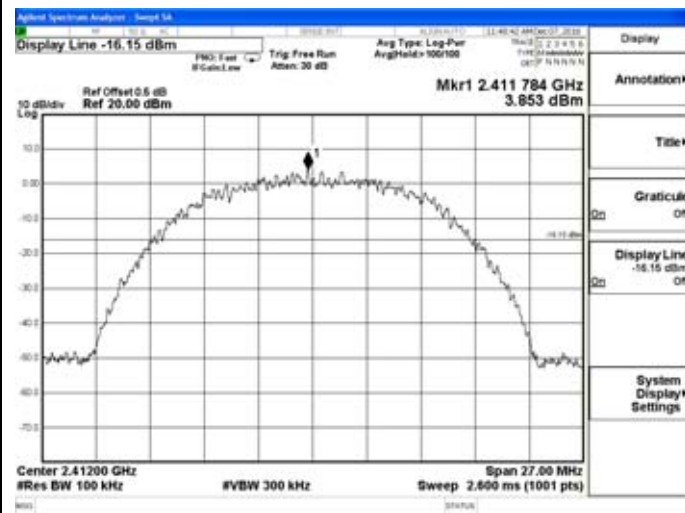
802.11b-Low channel
