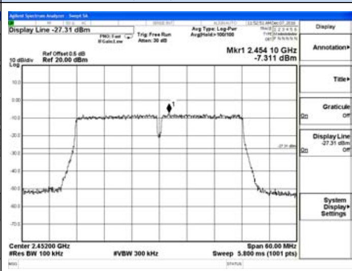
802.11n(HT40)-High channel
