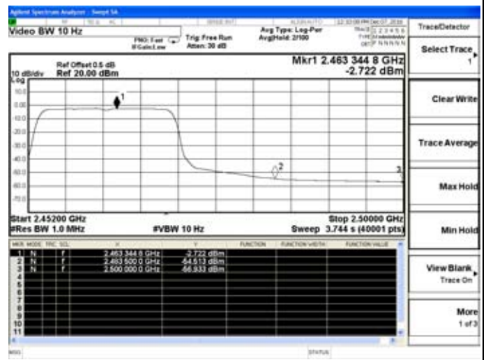
802.11g-High channel(Average)
