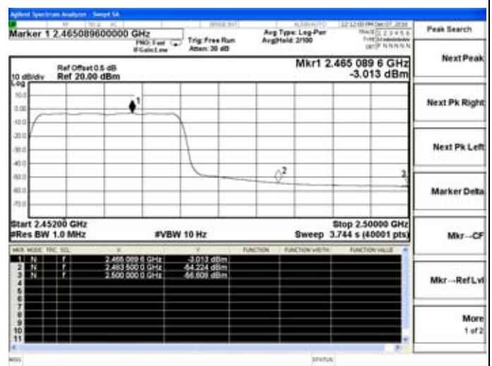
802.11n(HT20)-High channel(Average)
