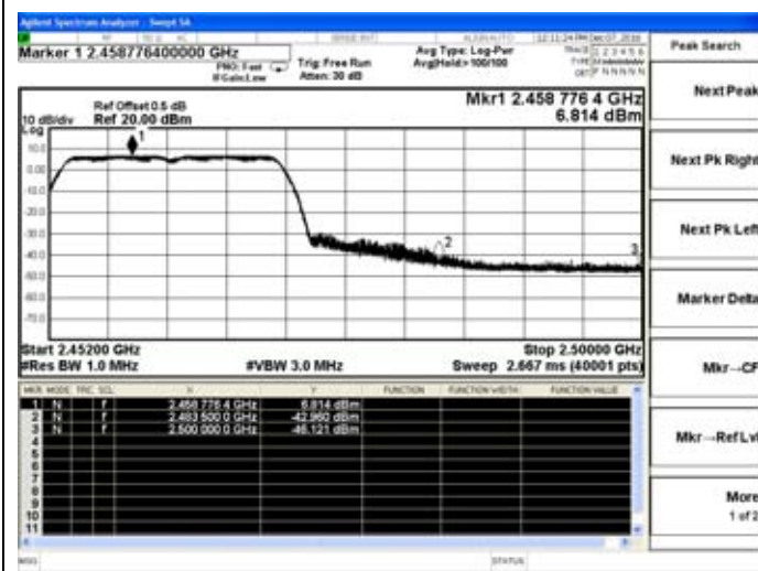
802.11n(HT20)-High channel(Peak)
