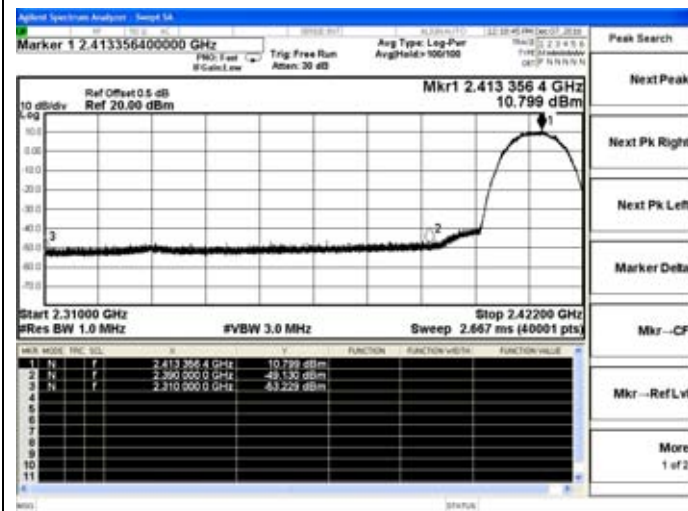
802.11b-Low channel(Peak)
