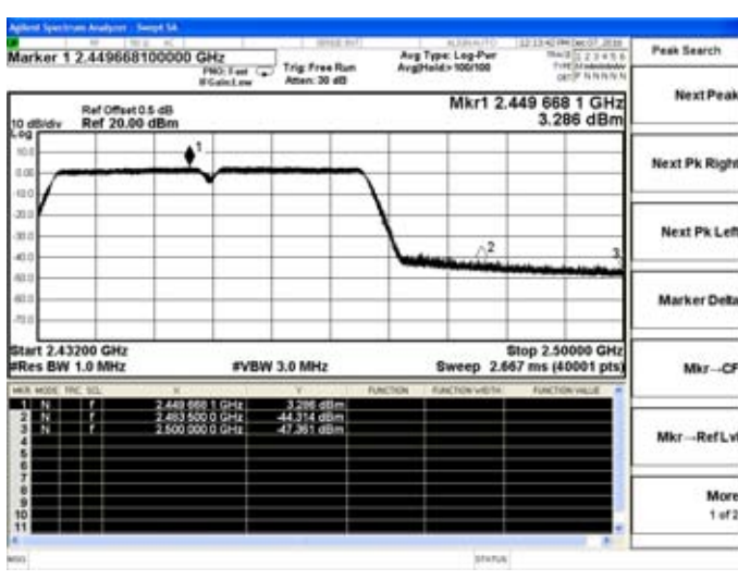
802.11n(HT40)-High channel(Peak)
