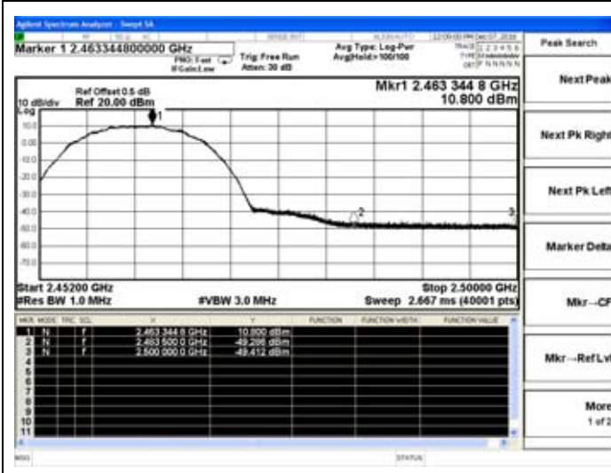
802.11b-High channel(Peak)
