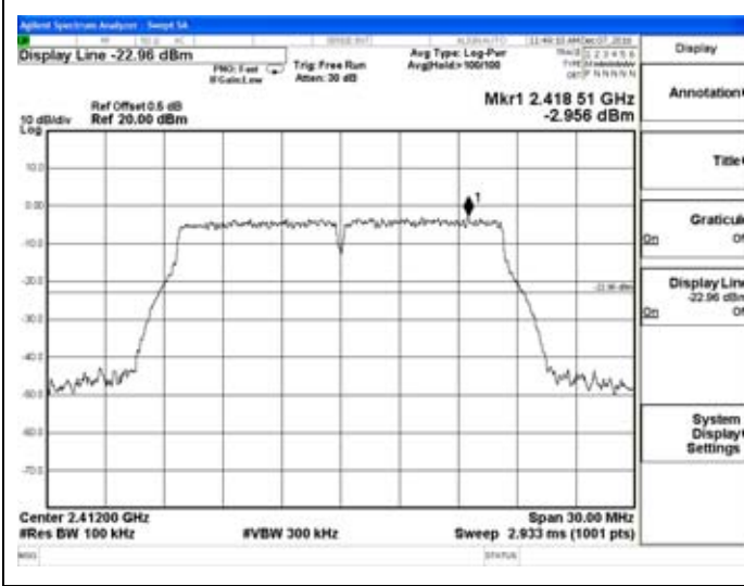
802.11g Low channel Reference
