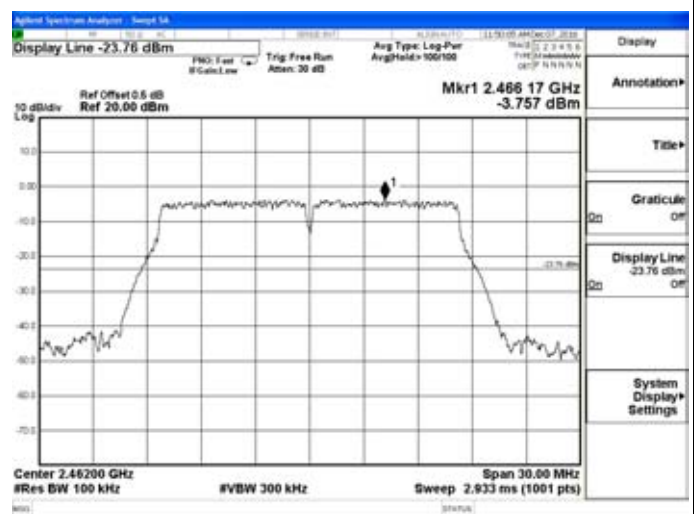
802.11g-High channel
