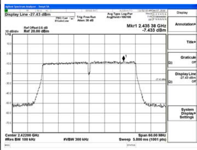
802.11n(HT40)-Low channel
