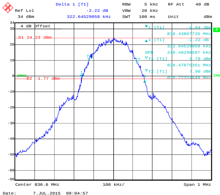
99% Occupied Bandwidth for GSM (GMSK) Mode
