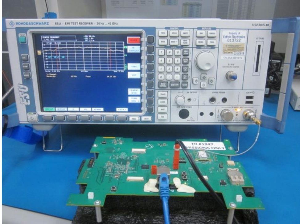
Figure B.1 - Conducted Measurement Test Setup
