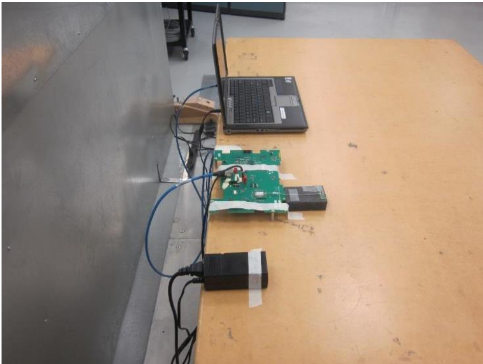
Figure B.5.2 - Conducted Emissions Test Setup - Side View
