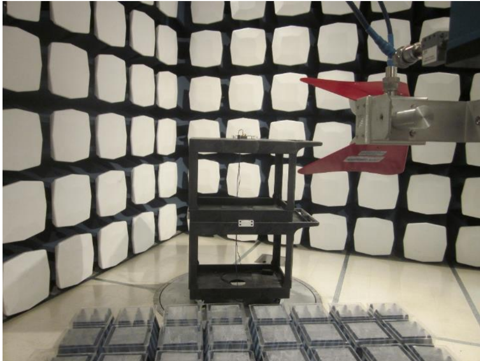
Figure B.3.1 - Radiated Emissions Test Setup - Front View (1 GHz-18 GHz)
