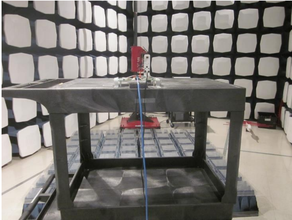
Figure B.4.1 - Radiated Emissions Test Setup - Front View (18 GHz-40 GHz)
