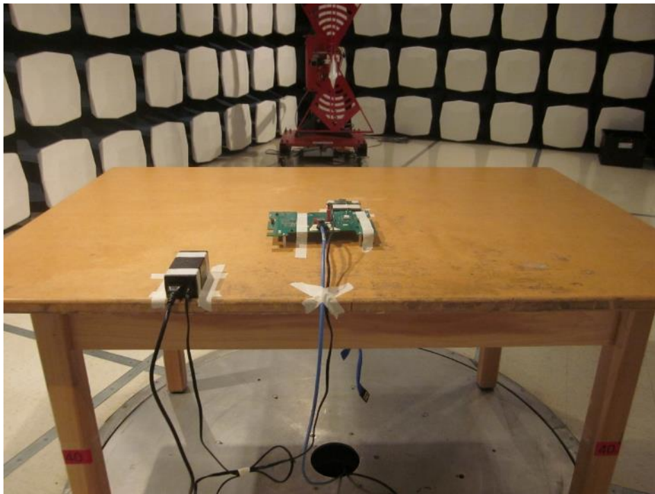
Figure B.2.2 - Radiated Emissions Test Setup - Rear View (30 MHz-1000 MHz)
