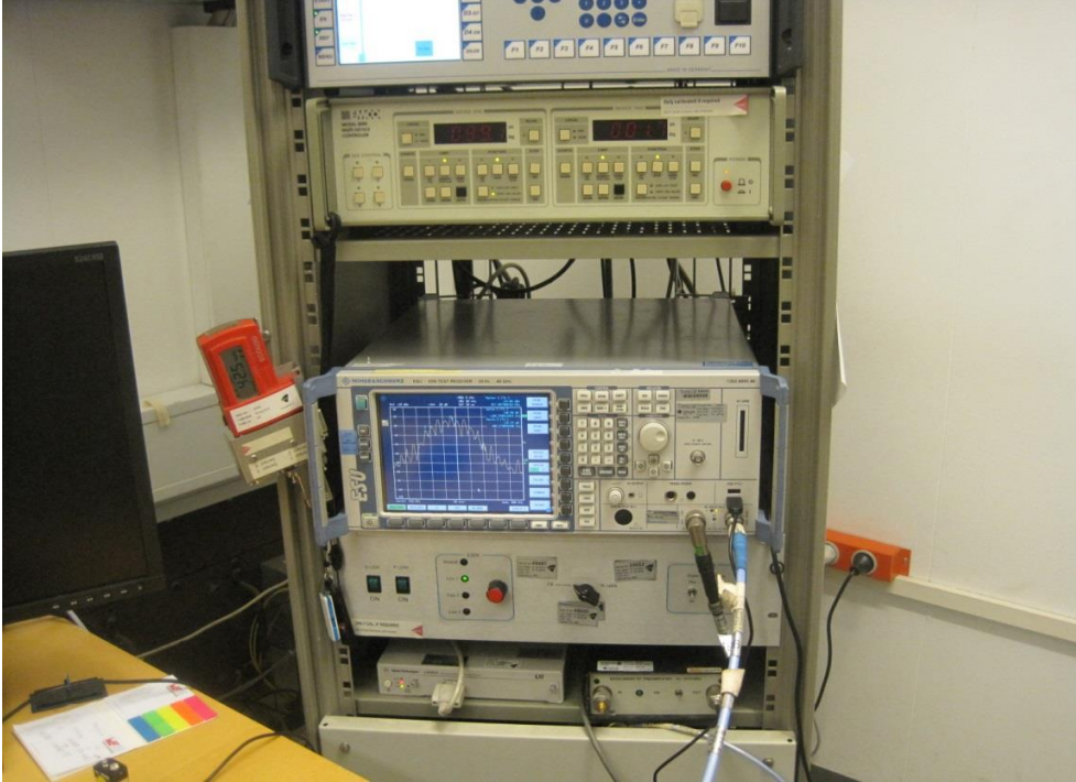
Photo 4.4.2 Test setup regarding measurement of 20 dB bandwidth.
