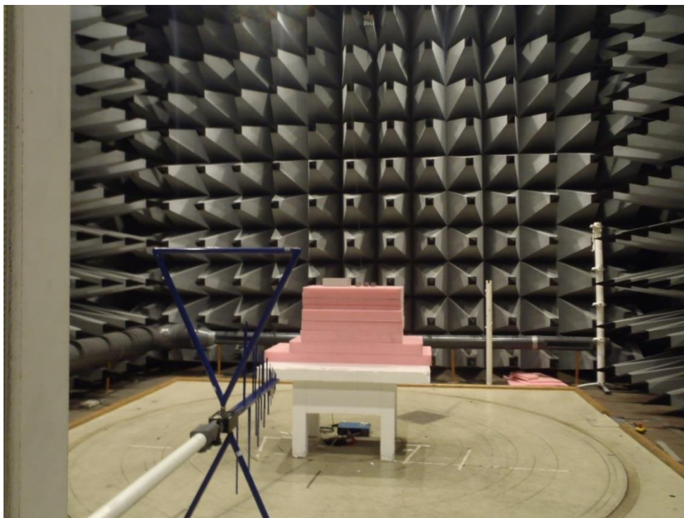
Photo 4.1.1 Test setup regarding measurement of radiated emission.
