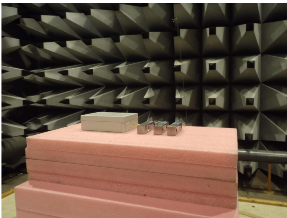
Photo 4.1.2 Test setup regarding measurement of radiated emission.
