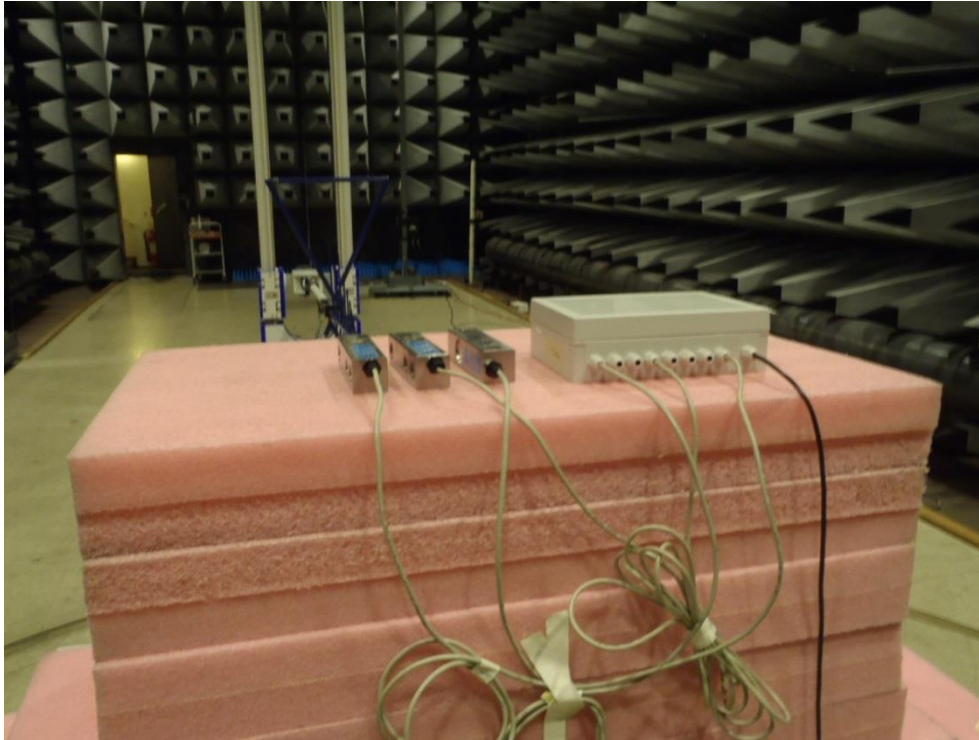
Photo 4.1.3 Test setup regarding measurement of radiated emission.
