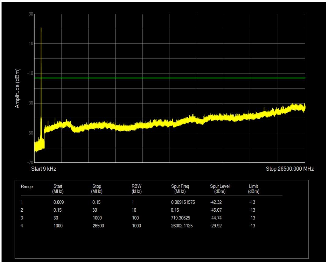
Band71 QPSK Channel=133297 nTones=1@47 Spacing=3.75kHz
