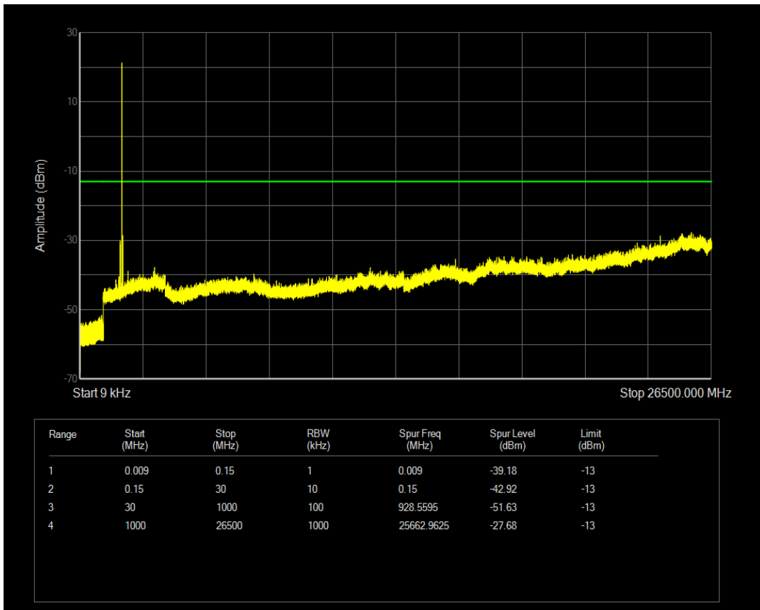
Band66 QPSK Channel=132670 nTones=1@47 Spacing=3.75kHz
