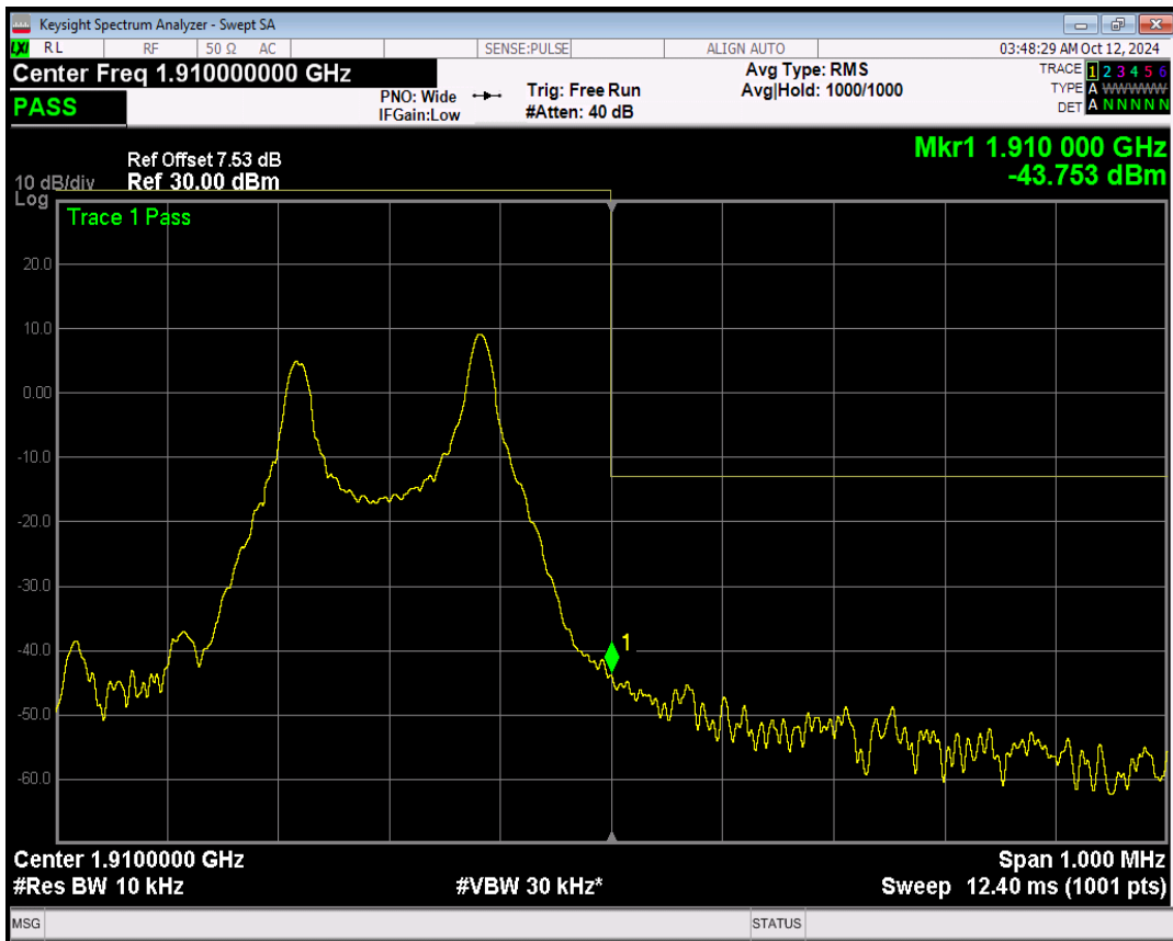
Band2 QPSK Channel=19198 nTones=12@0 Spacing=15kHz
