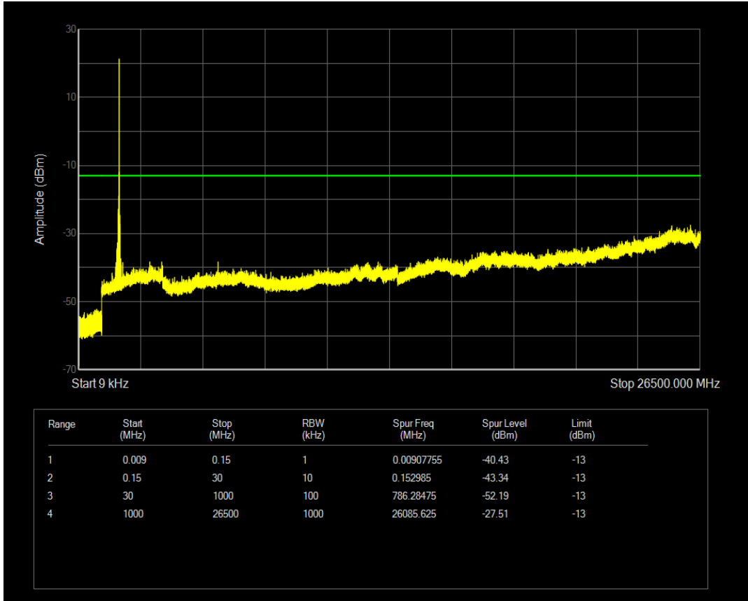
Band66 QPSK Channel=132322 nTones=1@47 Spacing=3.75kHz
