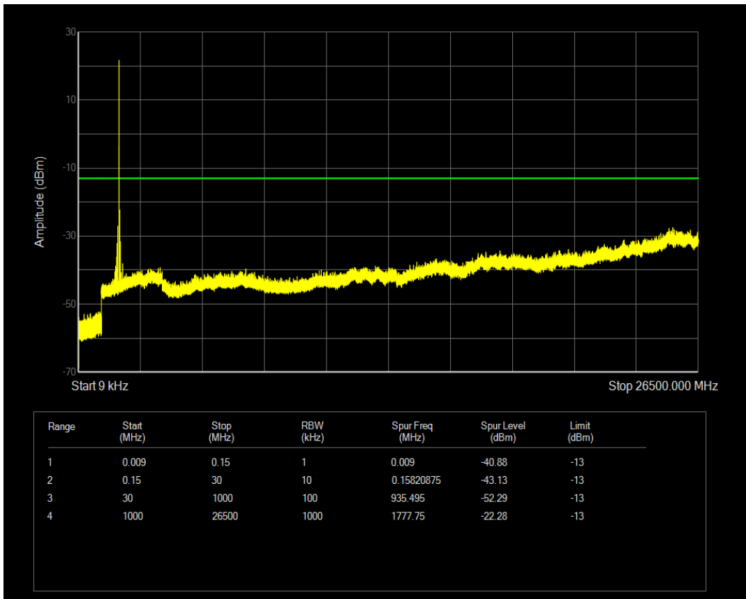
Band4 QPSK Channel=20398 nTones=1@47 Spacing=3.75kHz
