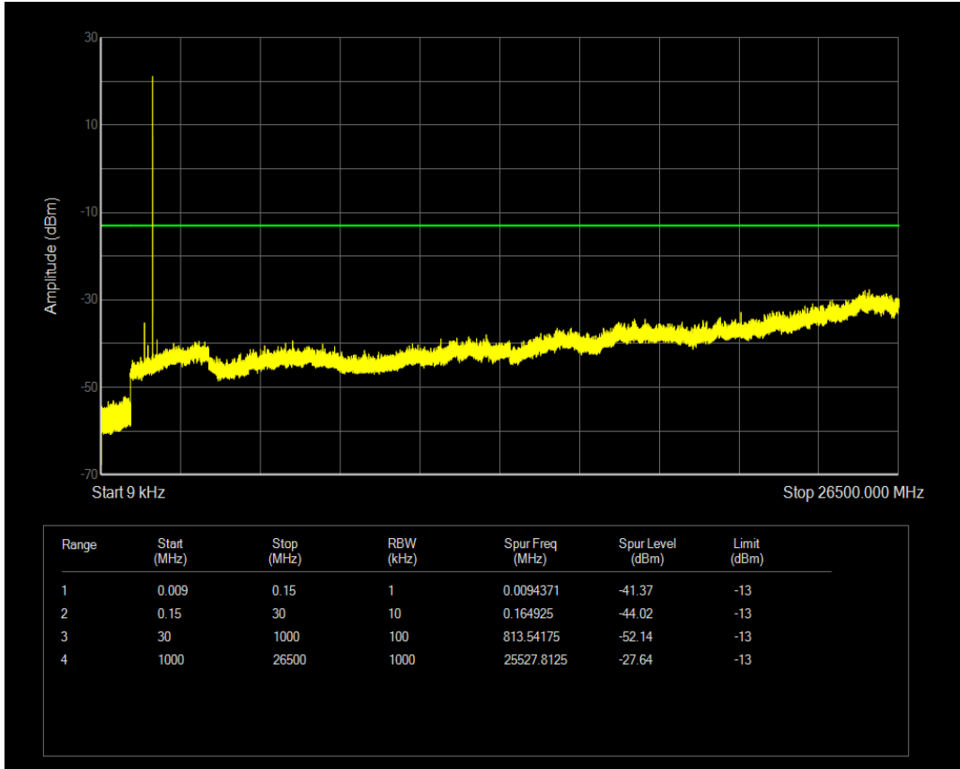
Band4 BPSK Channel=20398 nTones=1@0 Spacing=3.75kHz
