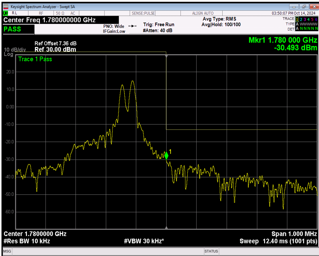
Band66 BPSK Channel=132670 nTones=1@11 Spacing=15kHz
