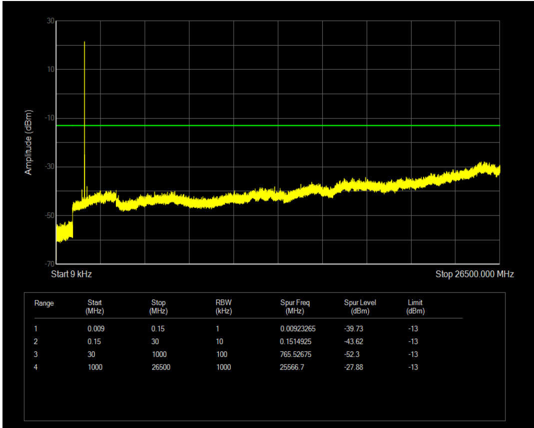
Band4 QPSK Channel=20175 nTones=1@47 Spacing=3.75kHz
