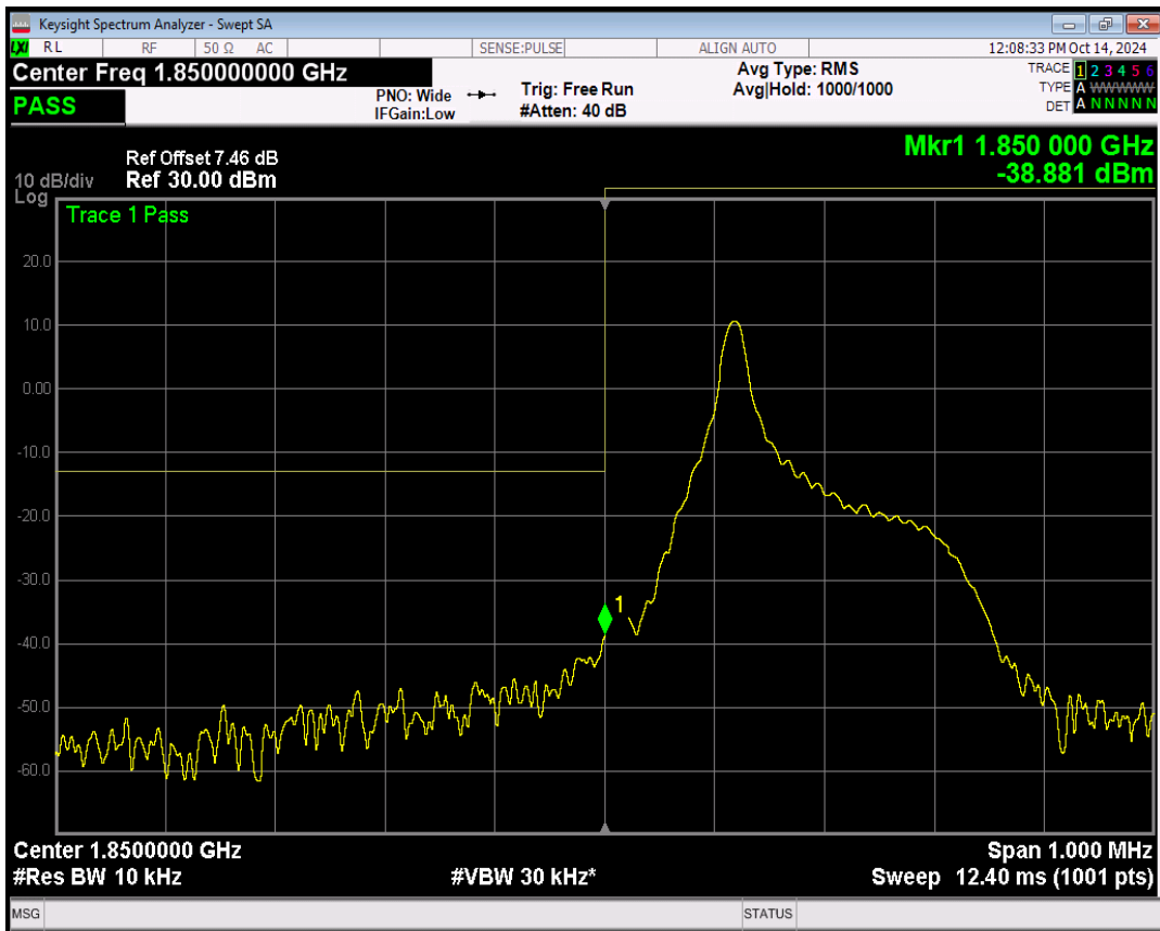
Band25 QPSK Channel=26042 nTones=1@0 Spacing=15kHz
