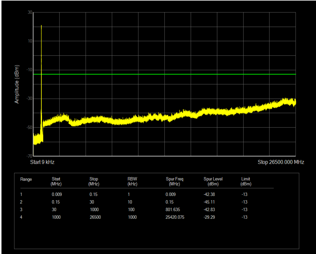
Band5 QPSK Channel=20402 nTones=1@0 Spacing=15kHz
