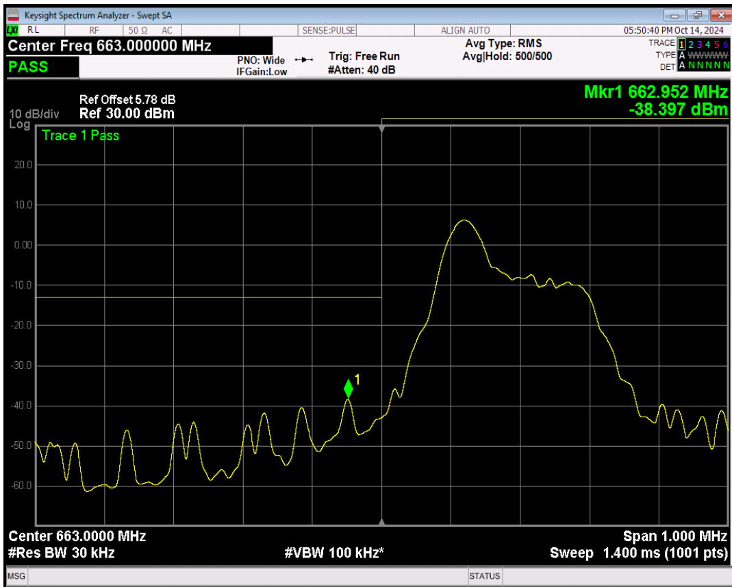
Band71 BPSK Channel=133470 nTones=1@47 Spacing=3.75kHz
