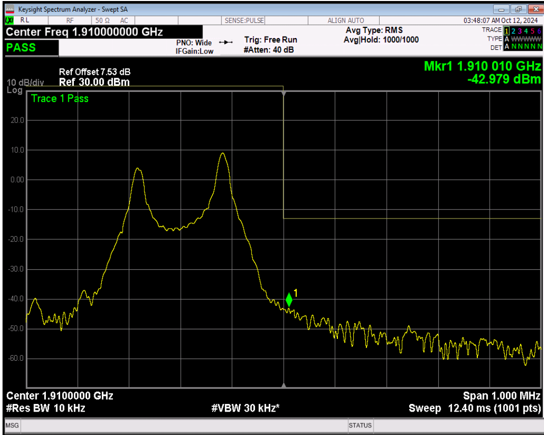
Band2 QPSK Channel=19198 nTones=1@11 Spacing=15kHz
