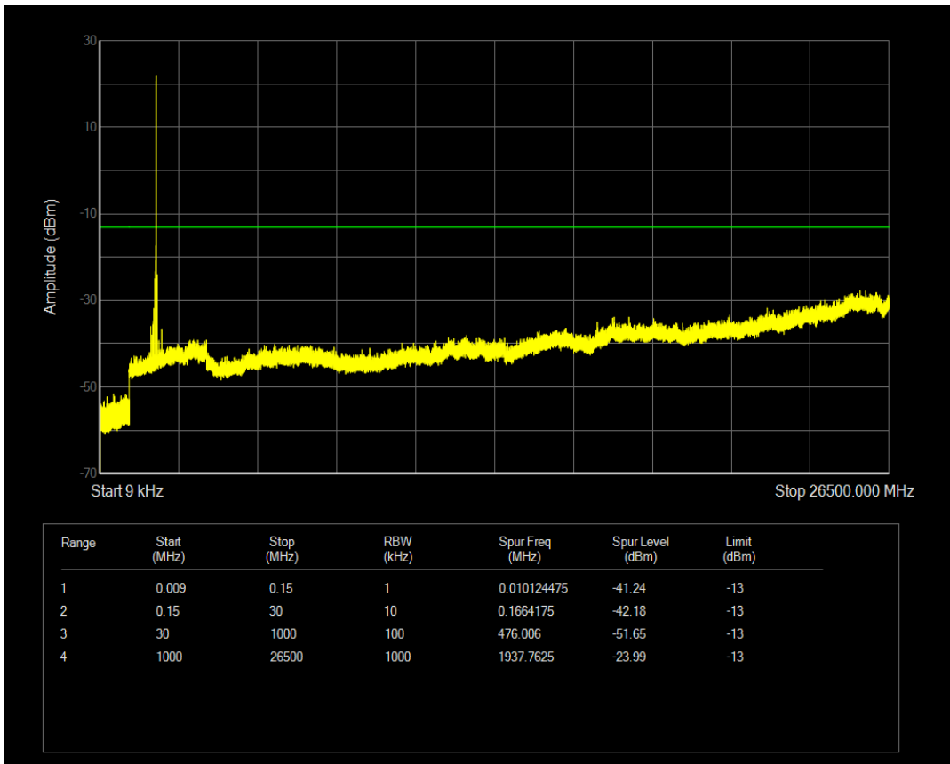
Band2 QPSK Channel=19198 nTones=1@47 Spacing=3.75kHz
