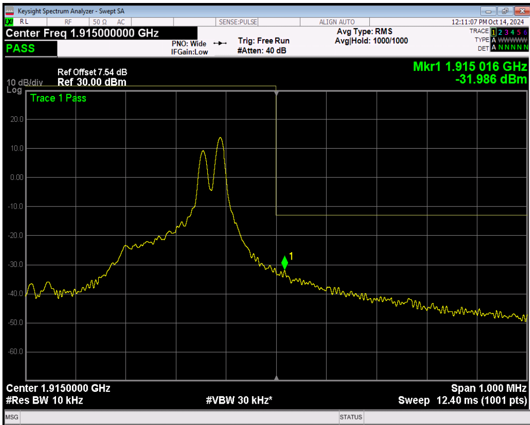
Band25 BPSK Channel=26688 nTones=1@11 Spacing=15kHz
