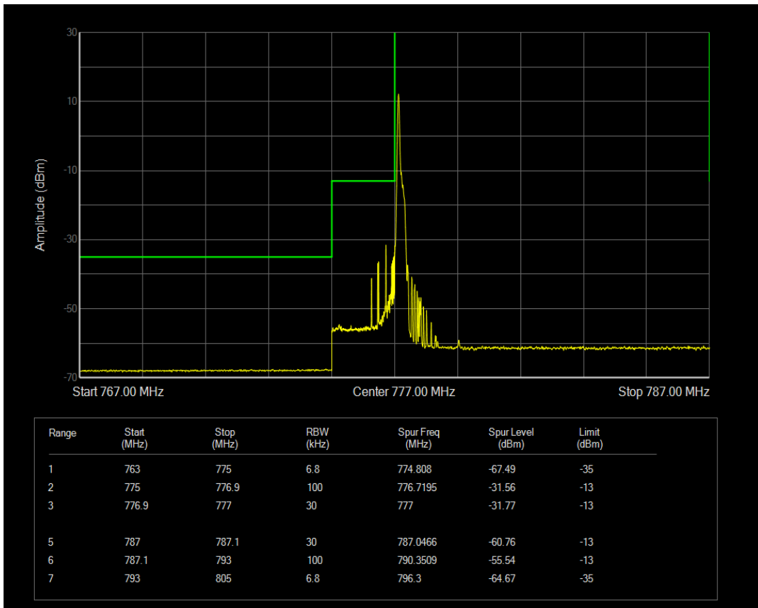
Band13 QPSK Channel=23182 nTones=1 @0 Spacing=15kHz
