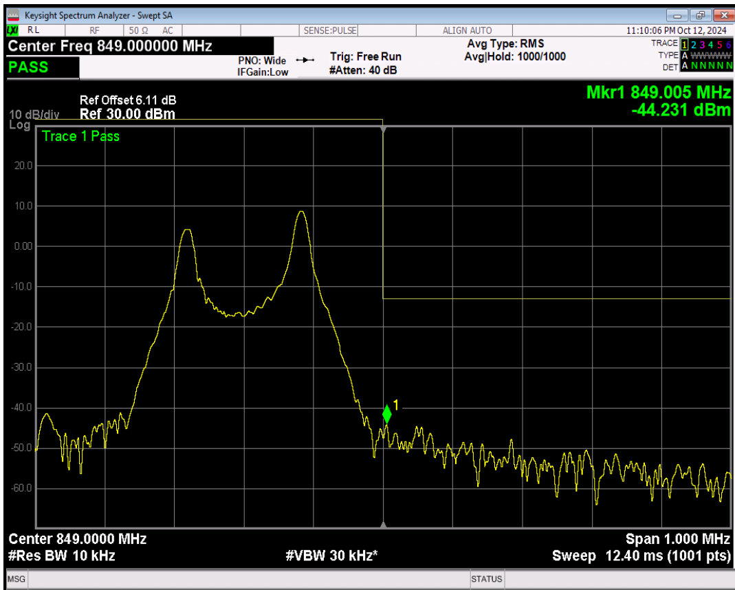
Band5 QPSK Channel=20648 nTones=12@0 Spacing=15kHz
