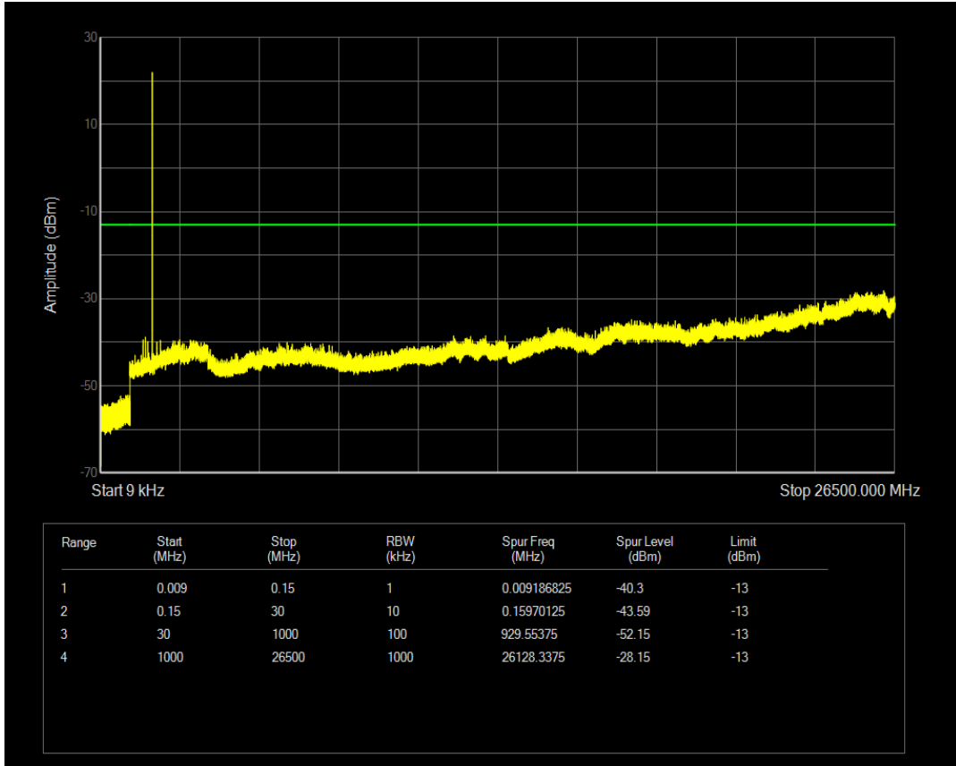
Band66 BPSK Channel=132670 nTones=1@0 Spacing=3.75kHz
