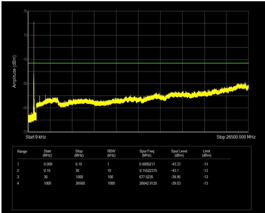
Band12 QPSK Channel=23012 nTones=1@47 Spacing=3.75kHz
