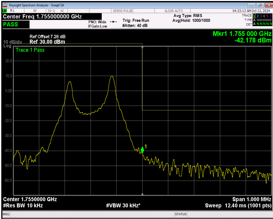
Band4 QPSK Channel=20398 nTones=1@11 Spacing=15kHz
