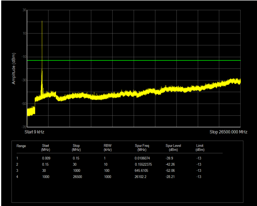
Band2 QPSK Channel=18900 nTones=1@47 Spacing=3.75kHz
