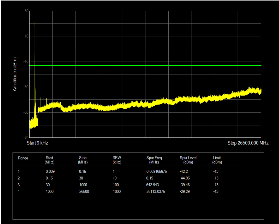
Band71 QPSK Channel=133124 nTones=1@47 Spacing=3.75kHz
