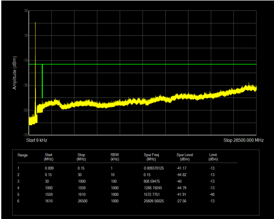
Band13 QPSK Channel=23278 nTones=1@47 Spacing=3.75kHz
