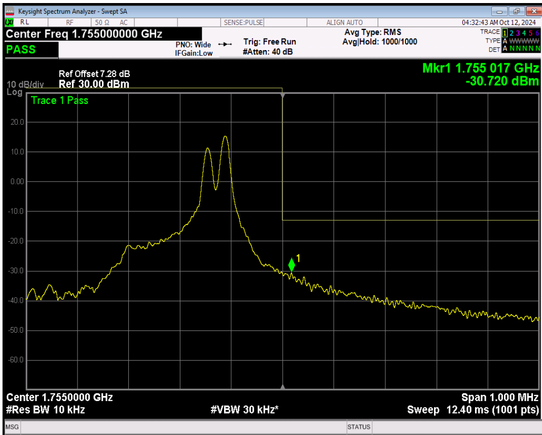
Band4 BPSK Channel=20398 nTones=1@11 Spacing=15kHz
