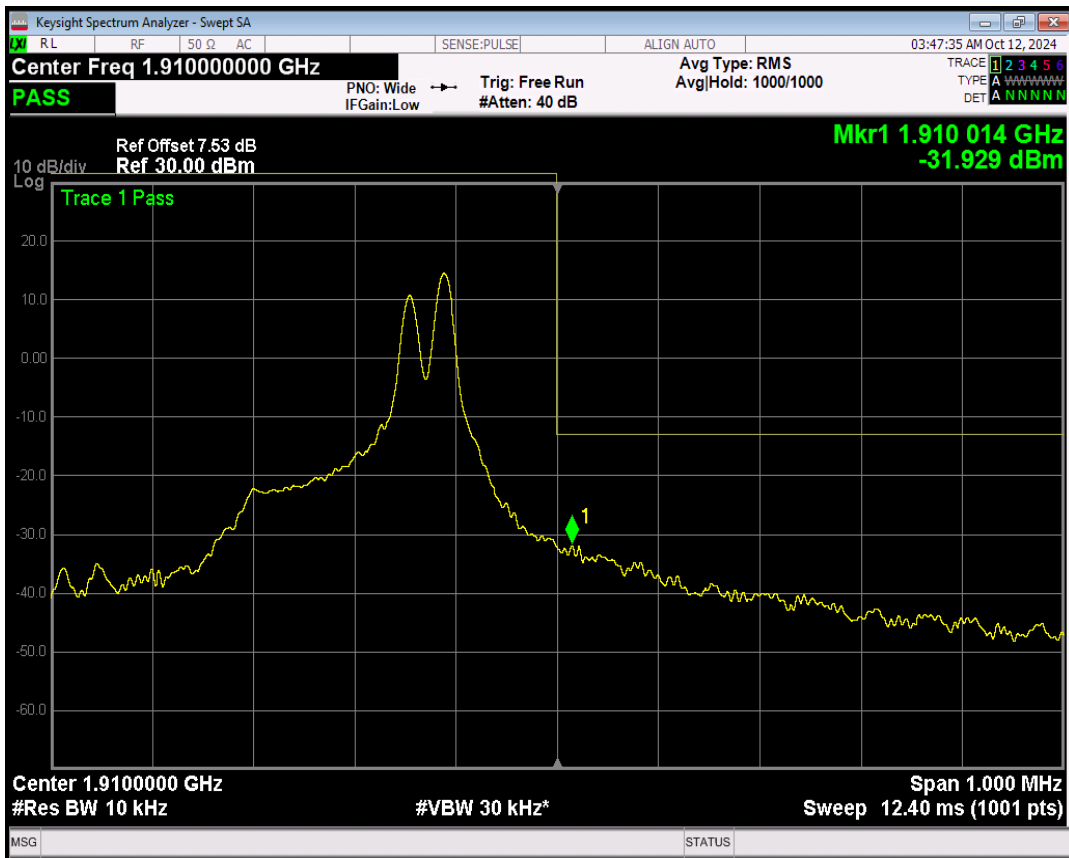
Band2 BPSK Channel=19198 nTones=1@11 Spacing=15kHz
