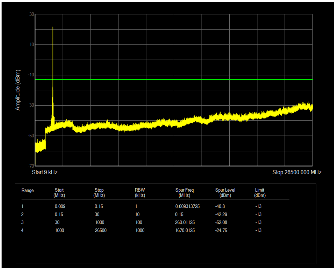
Band4 QPSK Channel=19952 nTones=1@47 Spacing=3.75kHz
