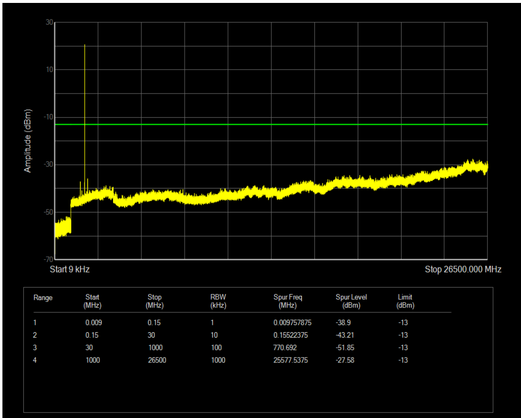
Band2 BPSK Channel=18900 nTones=1@0 Spacing=3.75kHz
