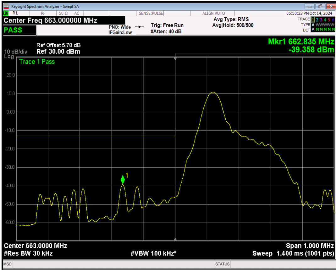
Band71 QPSK Channel=133124 nTones=12@0 Spacing=15kHz
