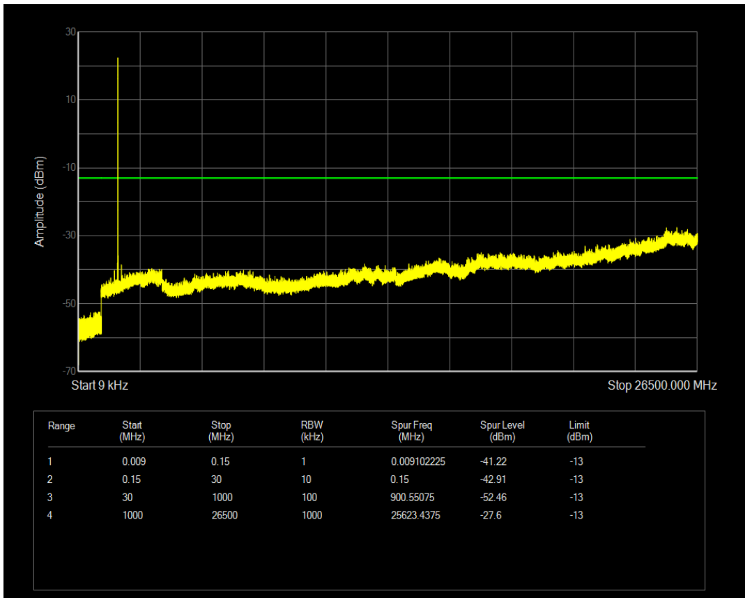
Band66 BPSK Channel=132322 nTones=1@0 Spacing=3.75kHz
