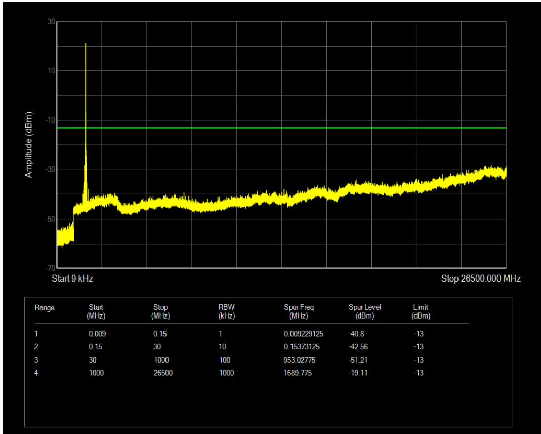
Band66 QPSK Channel=131974 nTones=1@47 Spacing=3.75kHz
