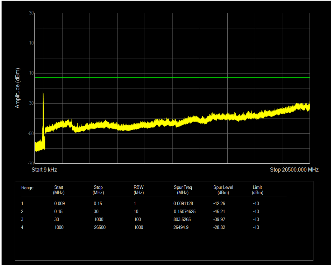
Band5 QPSK Channel=20402 nTones=1@47 Spacing=3.75kHz
