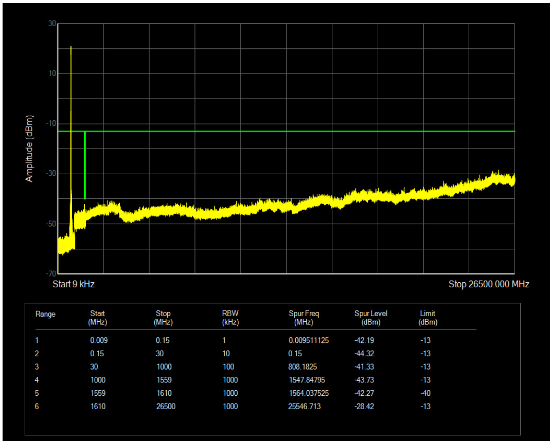
Band13 QPSK Channel=23230 nTones=1@47 Spacing=3.75kHz
