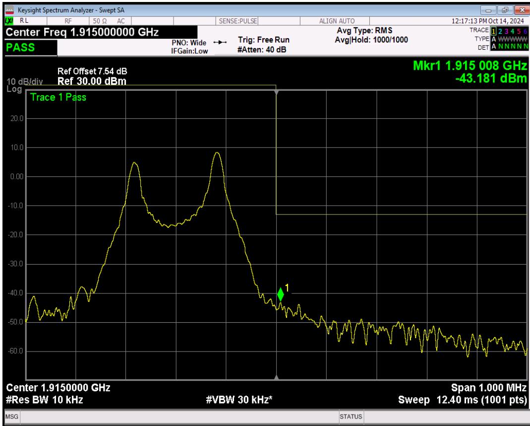
Band25 QPSK Channel=26688 nTones=1@11 Spacing=15kHz
