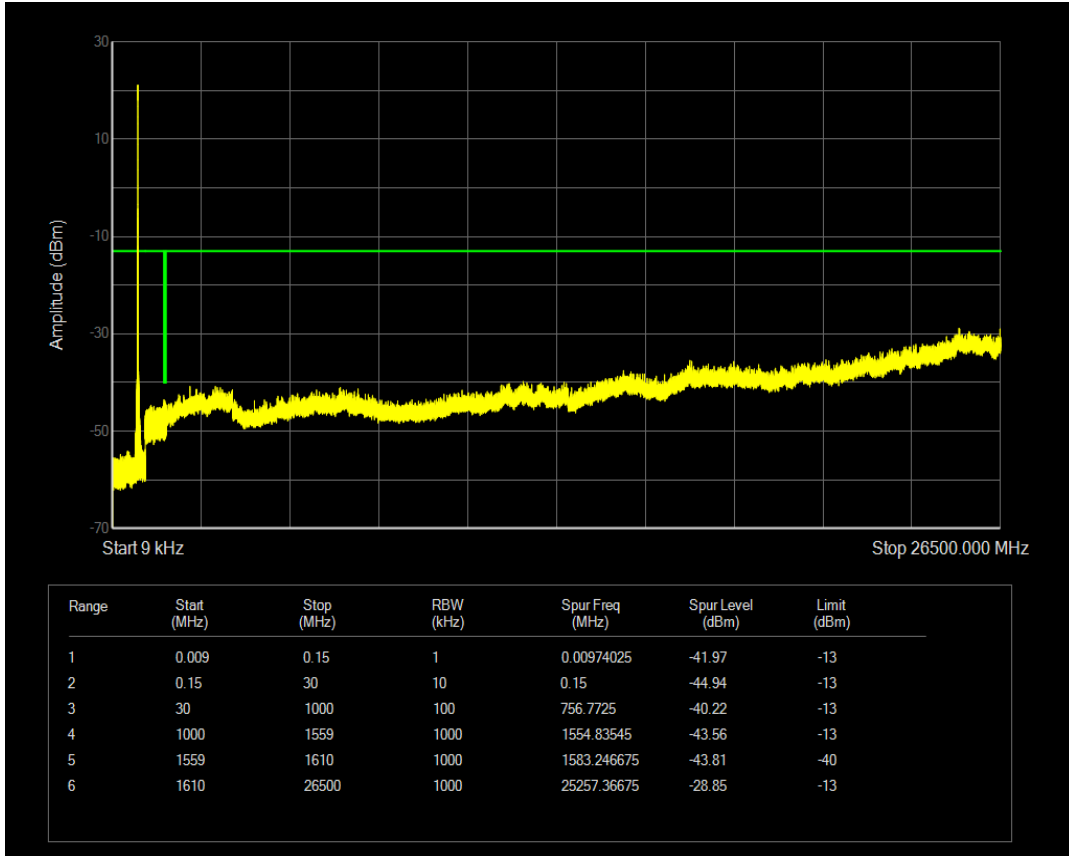
Band13 QPSK Channel=23182 nTones=1@47 Spacing=3.75kHz
