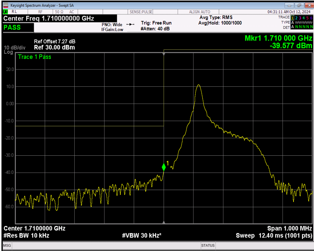
Band4 QPSK Channel=19952 nTones=12@0 Spacing=15kHz
