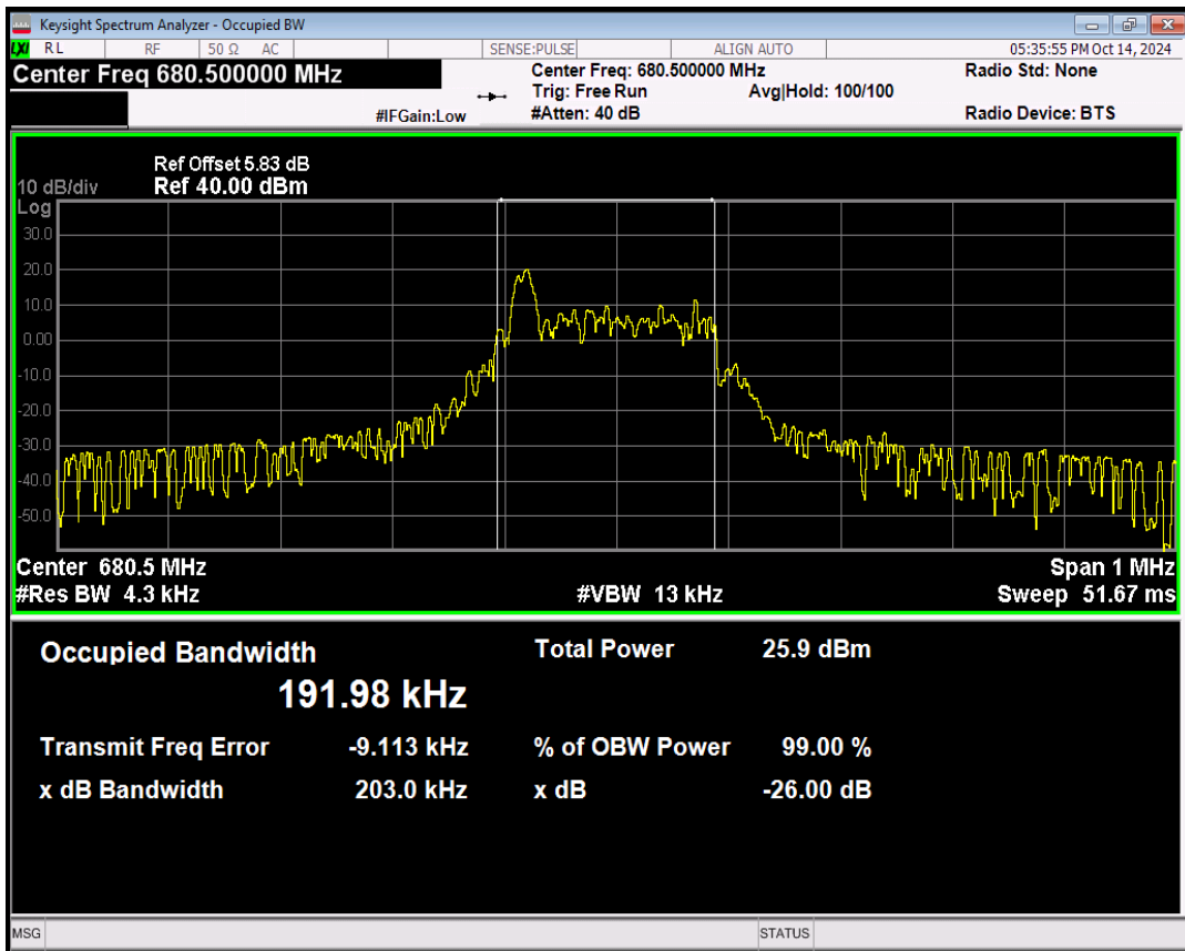
Band71 BPSK Channel=133470 nTones=1@0 Spacing=3.75kHz
