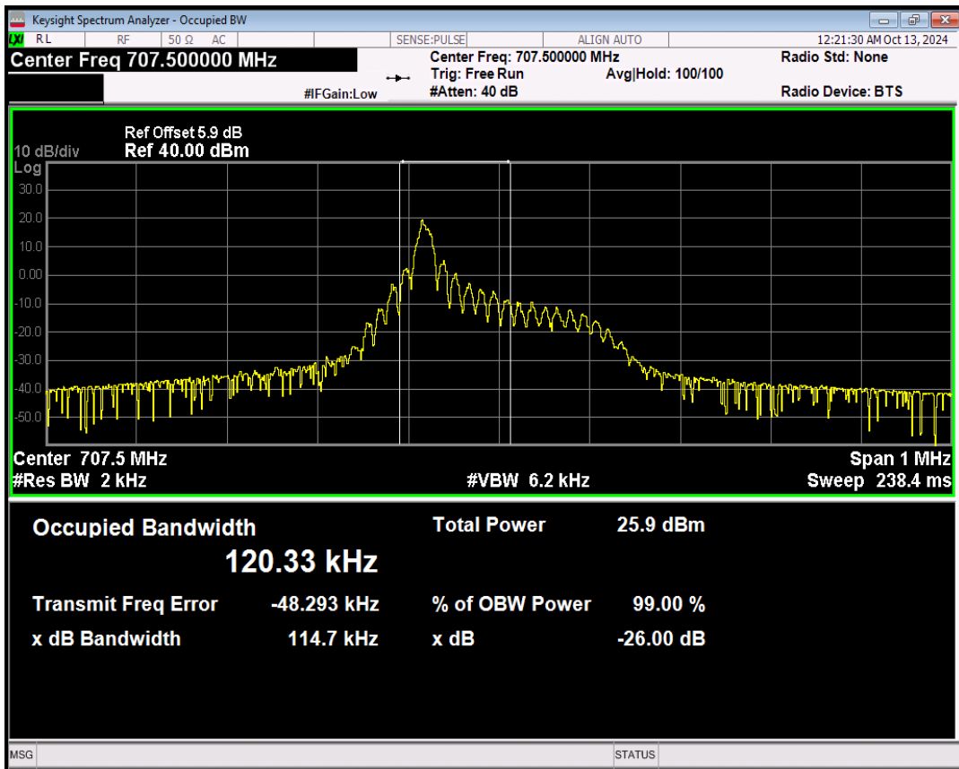
Band12 QPSK Channel=23095 nTones=12@0 Spacing=15kHz
