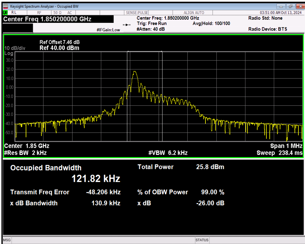
Band25 QPSK Channel=26042 nTones=12@0 Spacing=15kHz
