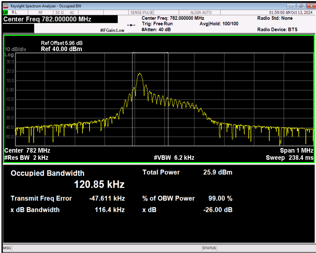
Band13 QPSK Channel=23230 nTones=12@0 Spacing=15kHz
