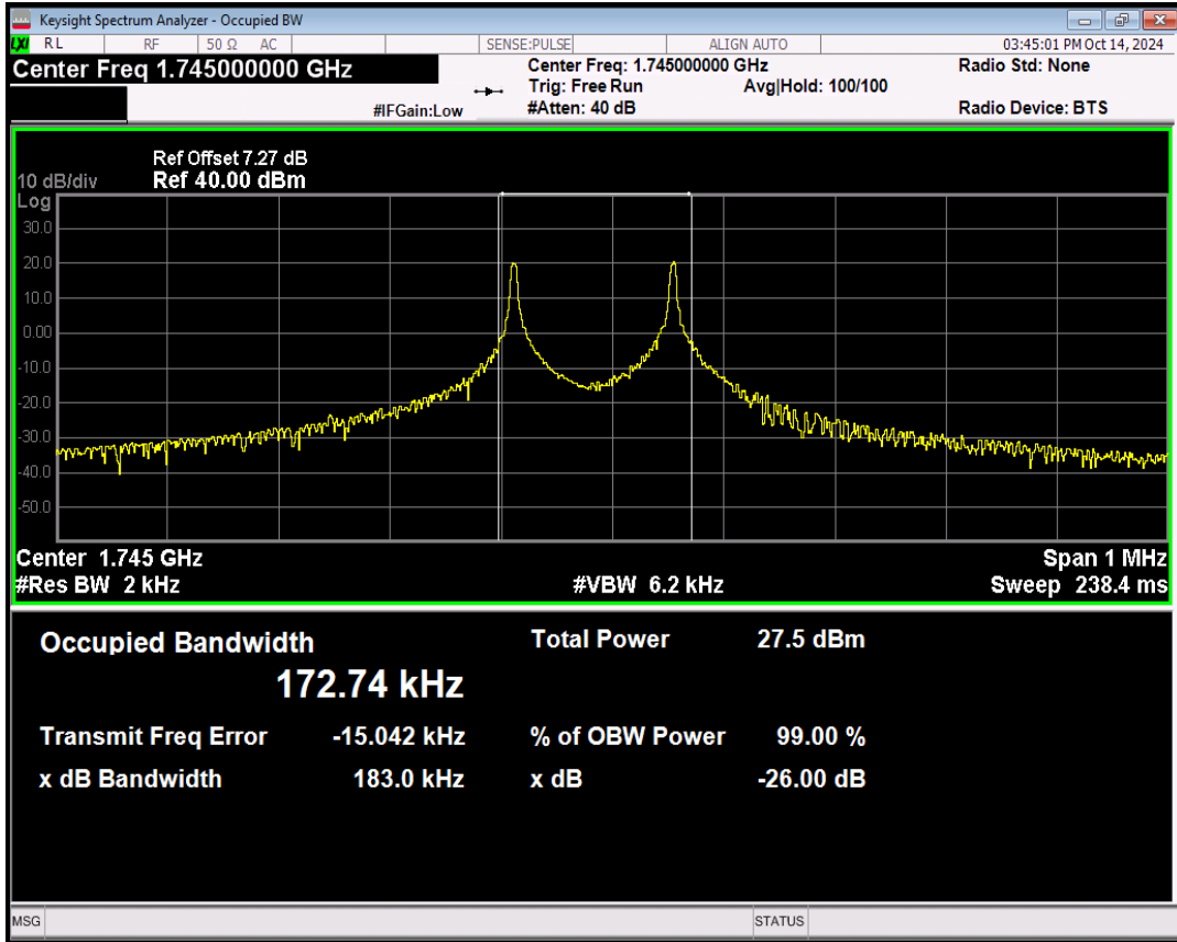
Band66 QPSK Channel=132322 nTones=1@0 Spacing=3.75kHz
