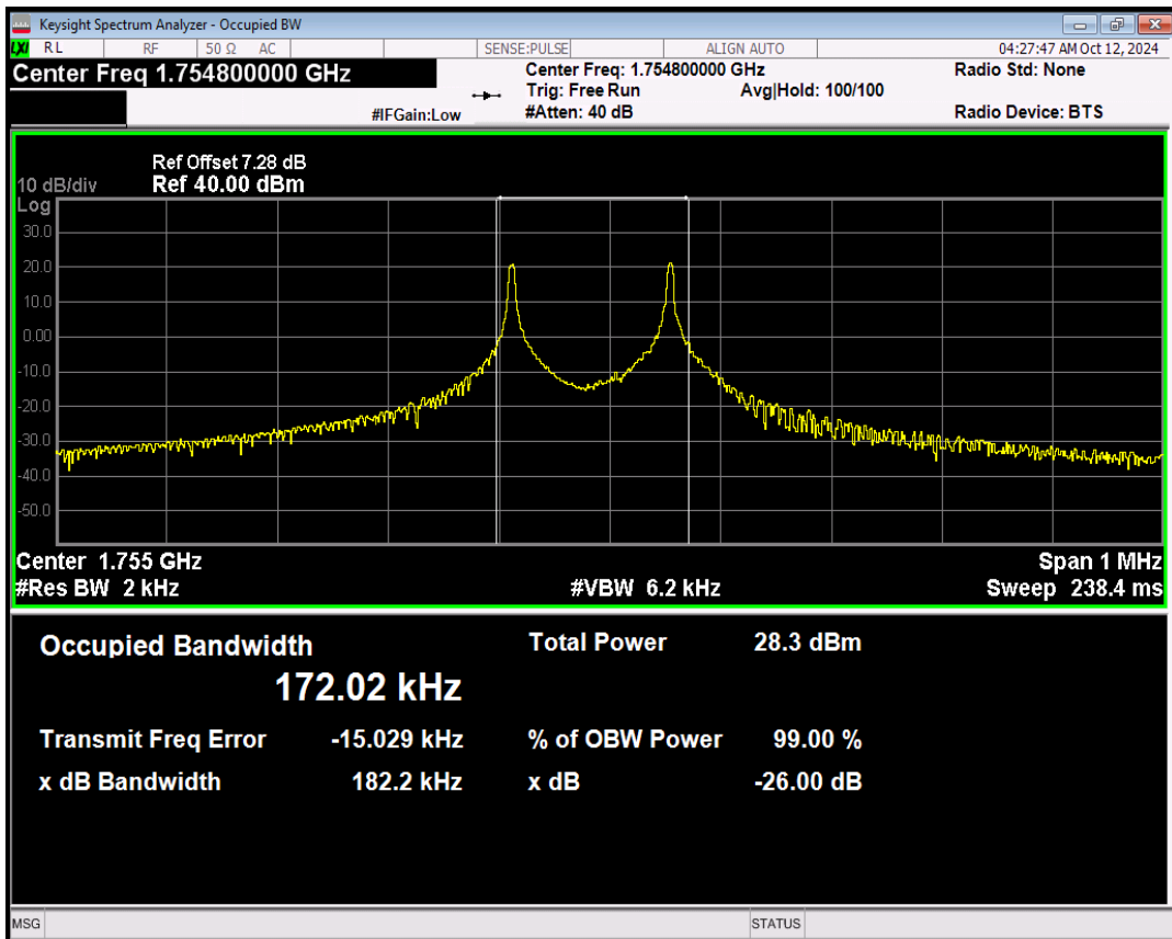
Band4 QPSK Channel=20398 nTones=1@0 Spacing=3.75kHz
