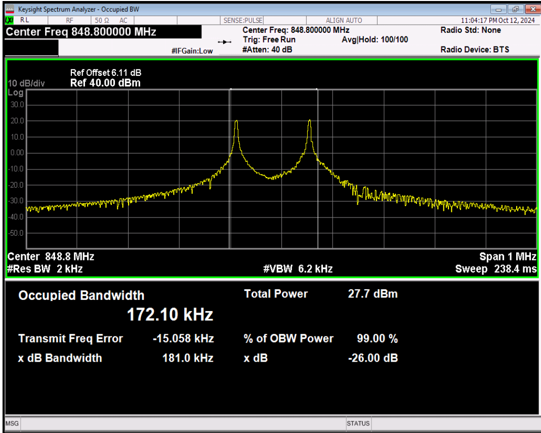
Band5 QPSK Channel=20648 nTones=1@0 Spacing=3.75kHz
