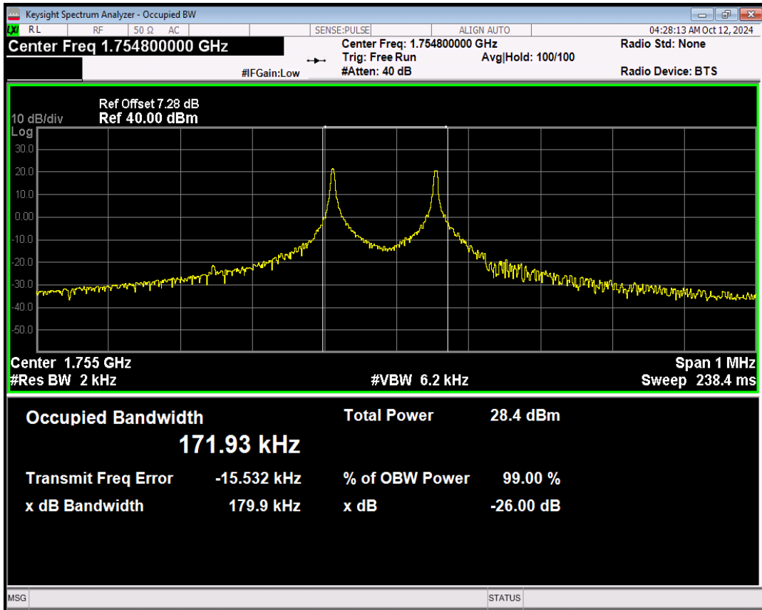
Band4 BPSK Channel=20398 nTones=1@0 Spacing=15kHz
