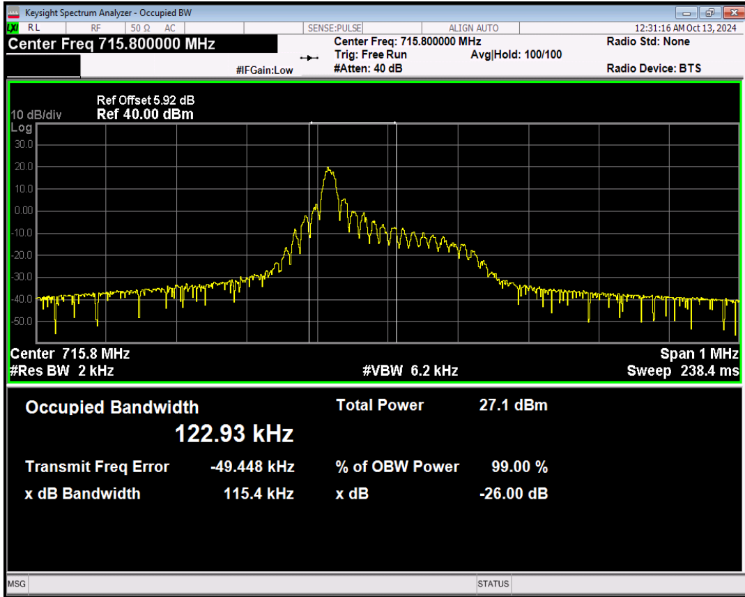
Band12 QPSK Channel=23178 nTones=12@0 Spacing=15kHz
