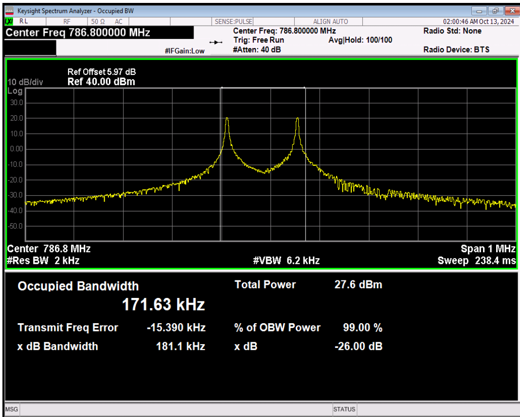
Band13 BPSK Channel=23278 nTones=1@0 Spacing=15kHz
