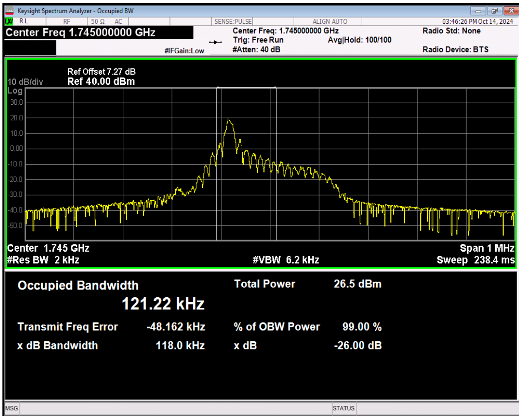
Band66 QPSK Channel=132322 nTones=12@0 Spacing=15kHz
