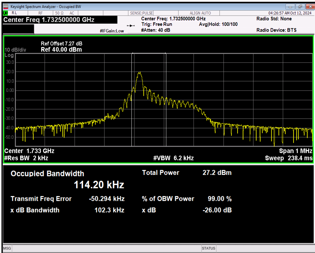
Band4 QPSK Channel=20175 nTones=12@0 Spacing=15kHz
