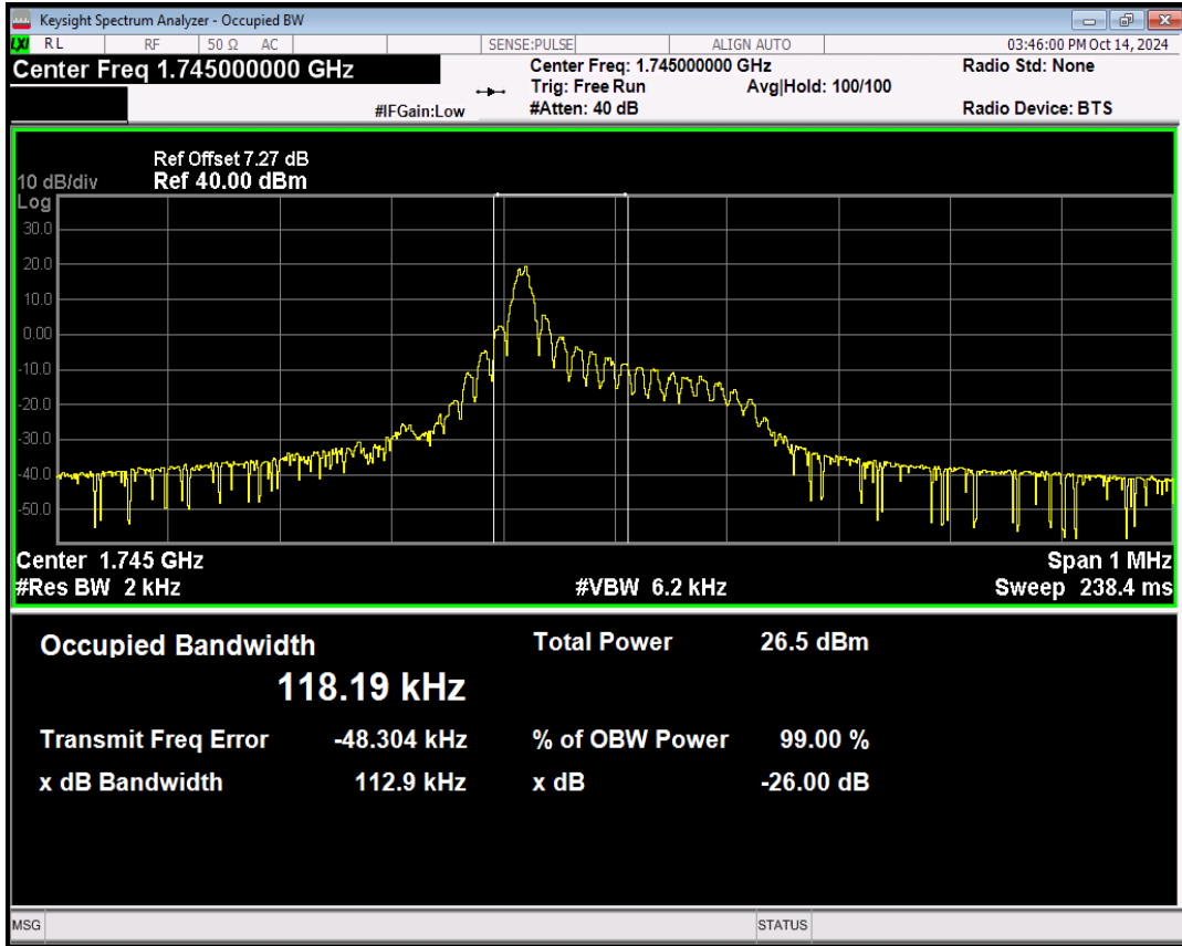
Band66 QPSK Channel=132322 nTones=1@0 Spacing=15kHz
