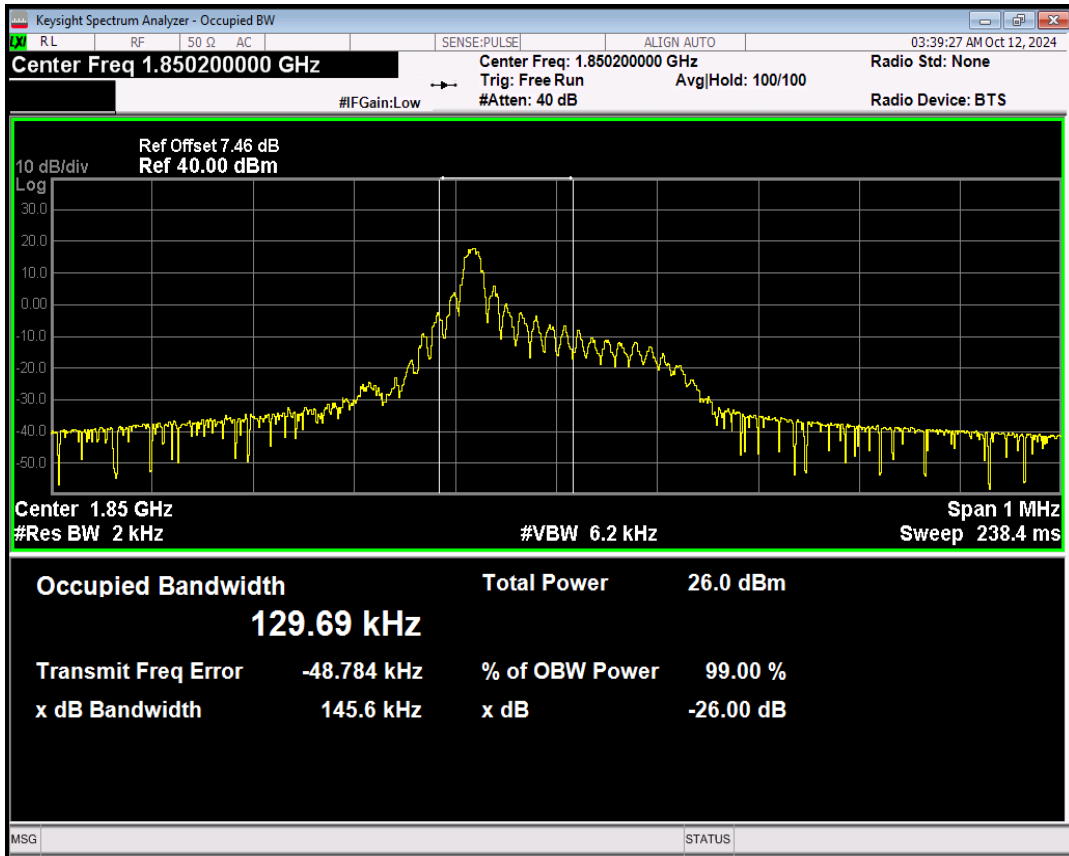
Band2 QPSK Channel=18602 nTones=12@0 Spacing=15kHz
