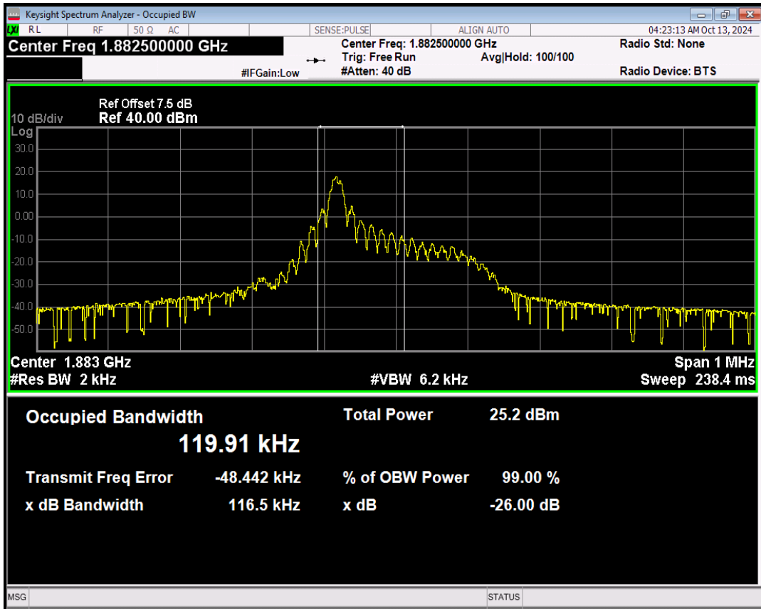
Band25 QPSK Channel=26365 nTones=12@0 Spacing=15kHz
