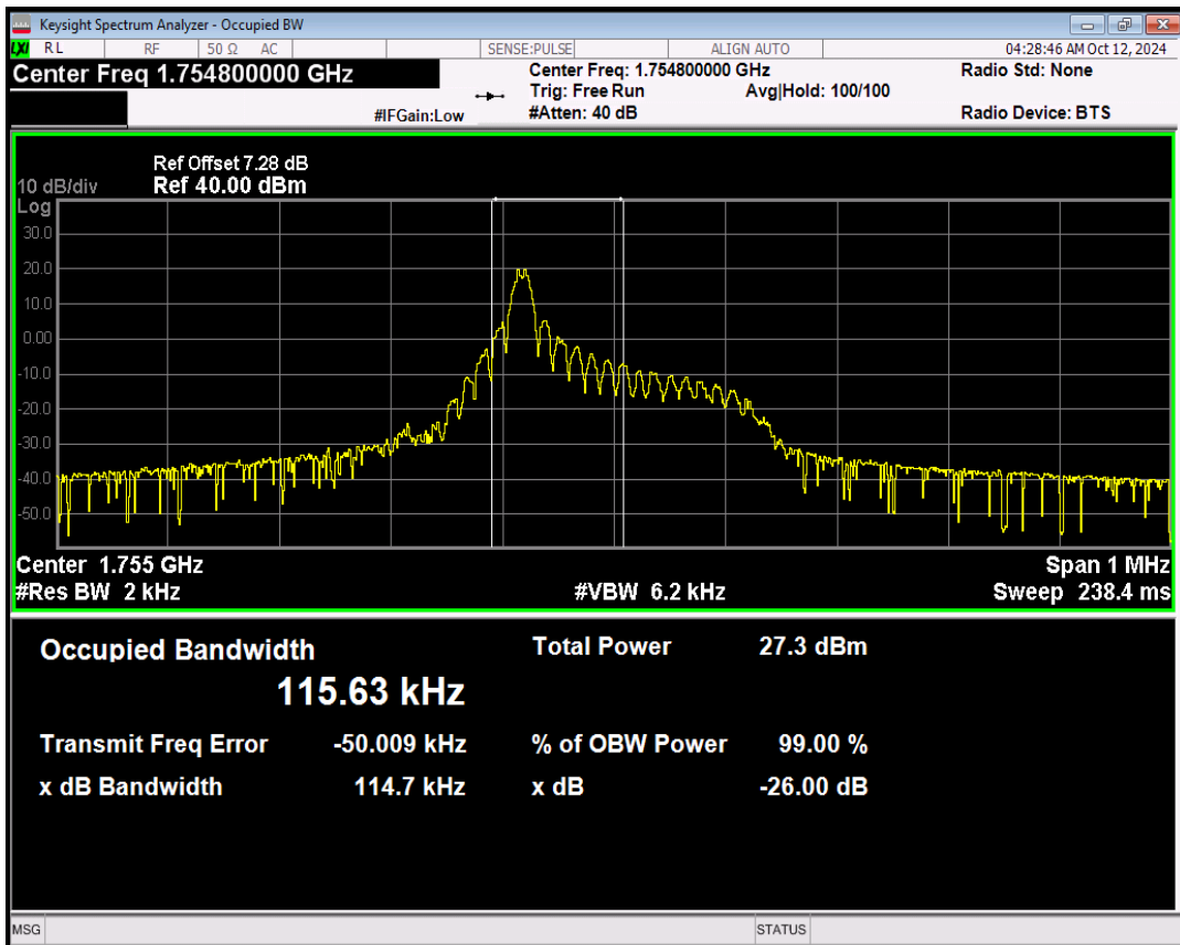
Band4 QPSK Channel=20398 nTones=1@0 Spacing=15kHz
