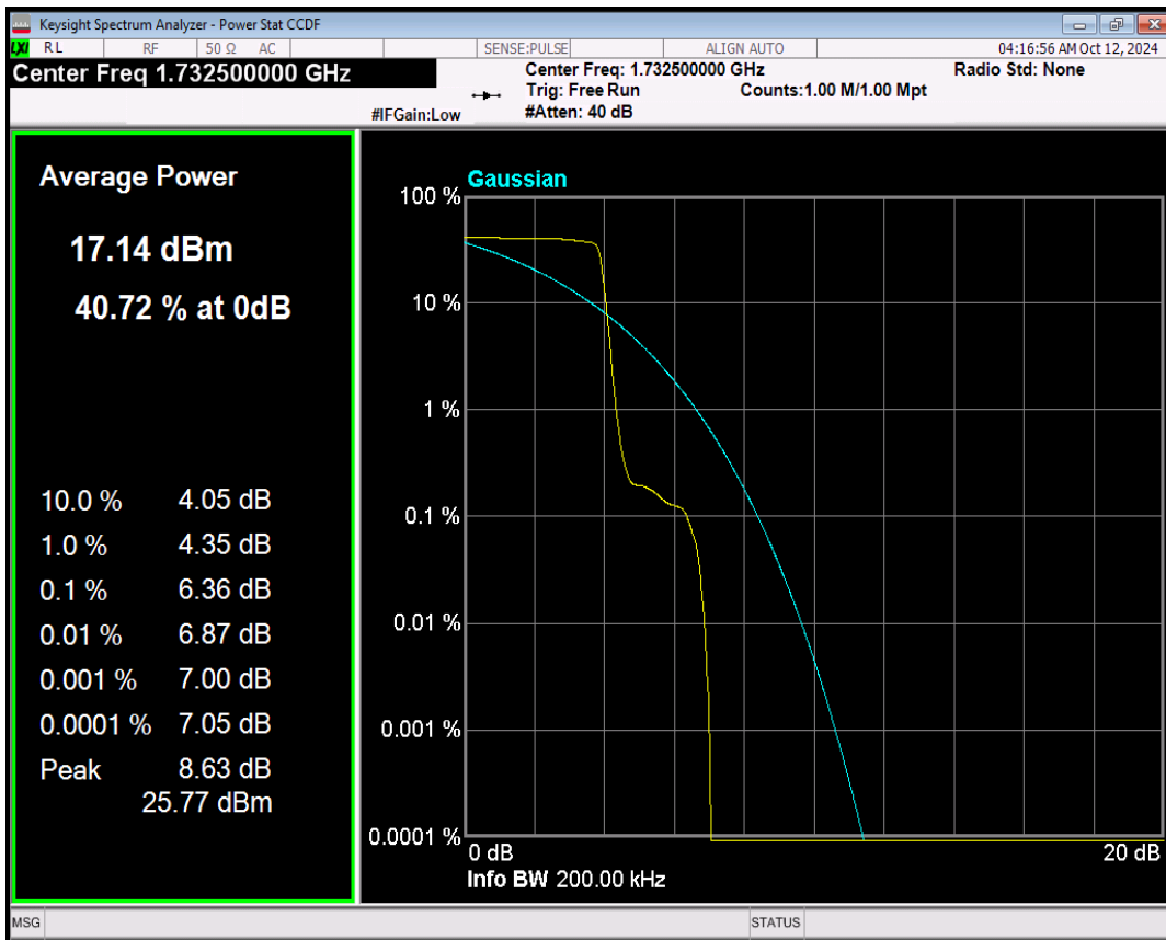
Band4 QPSK Channel=20175 nTones=1@0 Spacing=3.75kHz
