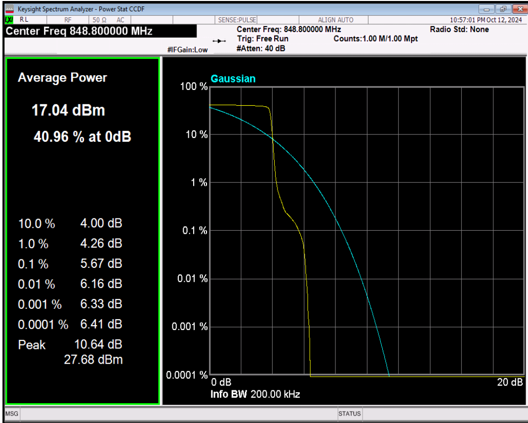
Band5 BPSK Channel=20648 nTones=1@0 Spacing=15kHz
