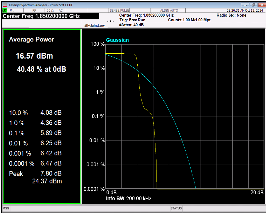
Band2 BPSK Channel=18602 nTones=1@0 Spacing=15kHz
