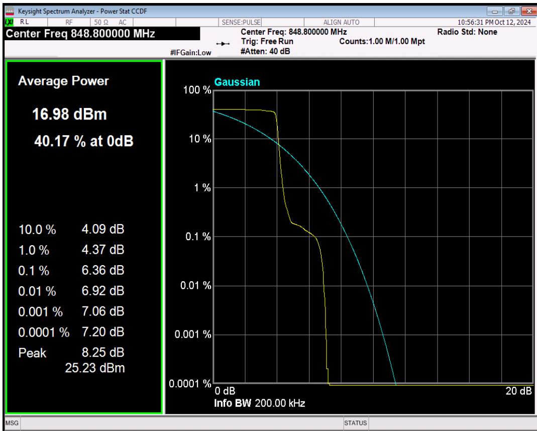
Band5 QPSK Channel=20648 nTones=1@0 Spacing=3.75kHz
