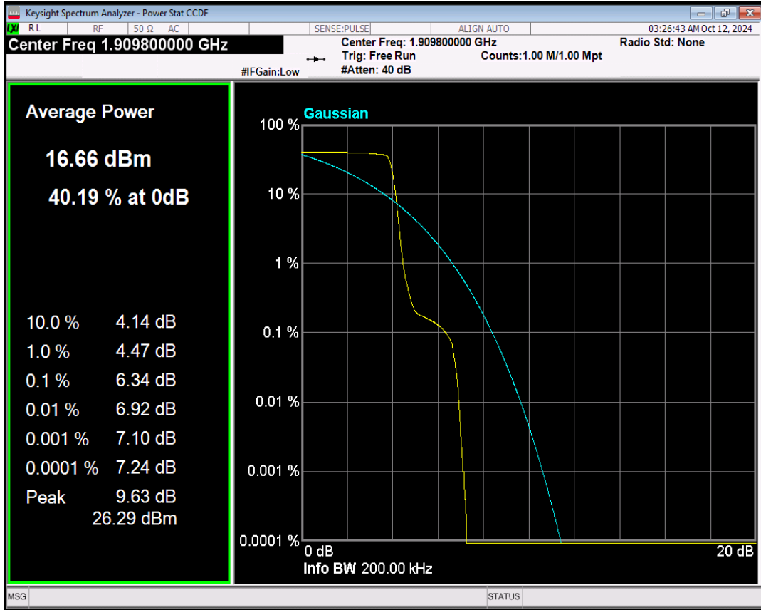
Band2 BPSK Channel=19198 nTones=1@0 Spacing=15kHz
