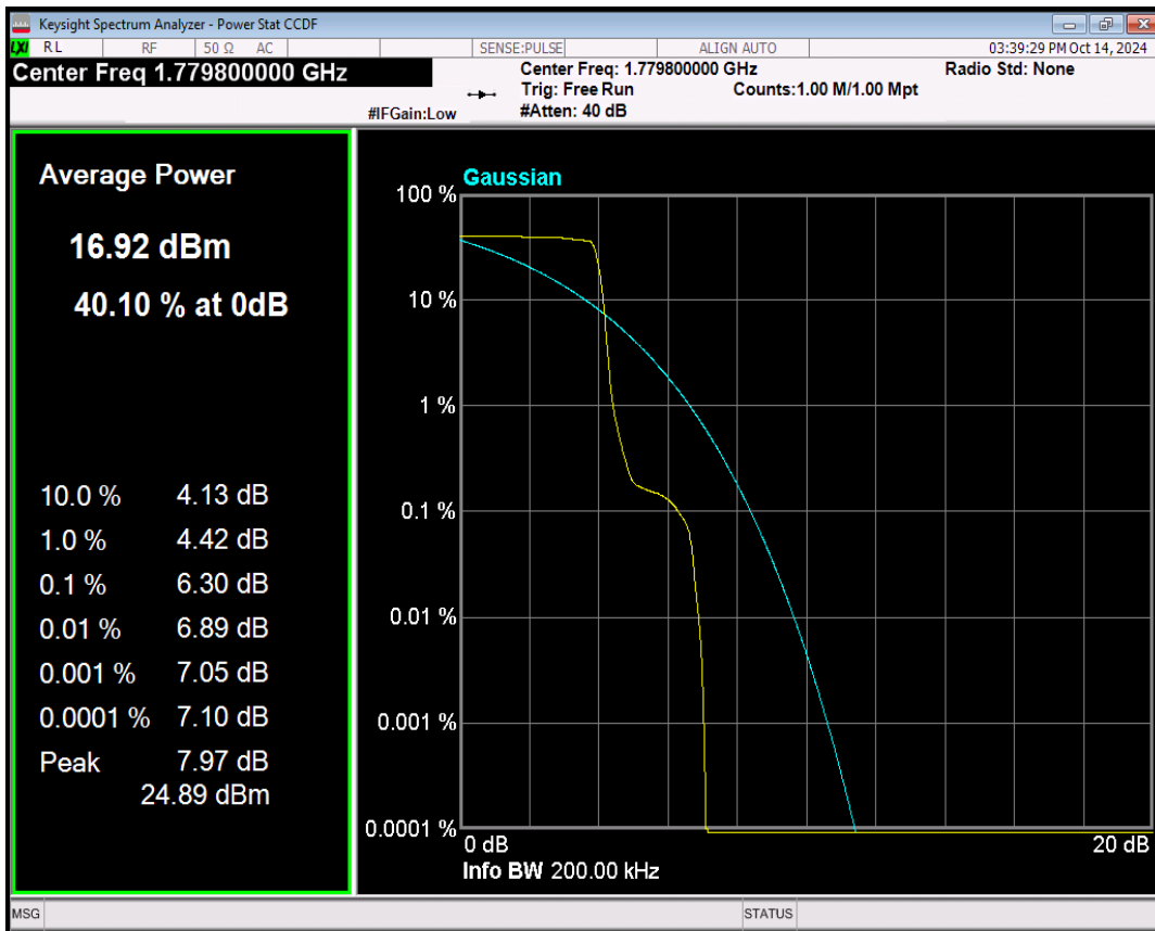
Band66 QPSK Channel=132670 nTones=1@0 Spacing=3.75kHz
