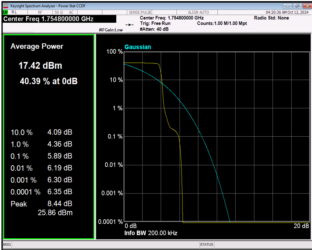
Band4 BPSK Channel=20398 nTones=1@0 Spacing=15kHz
