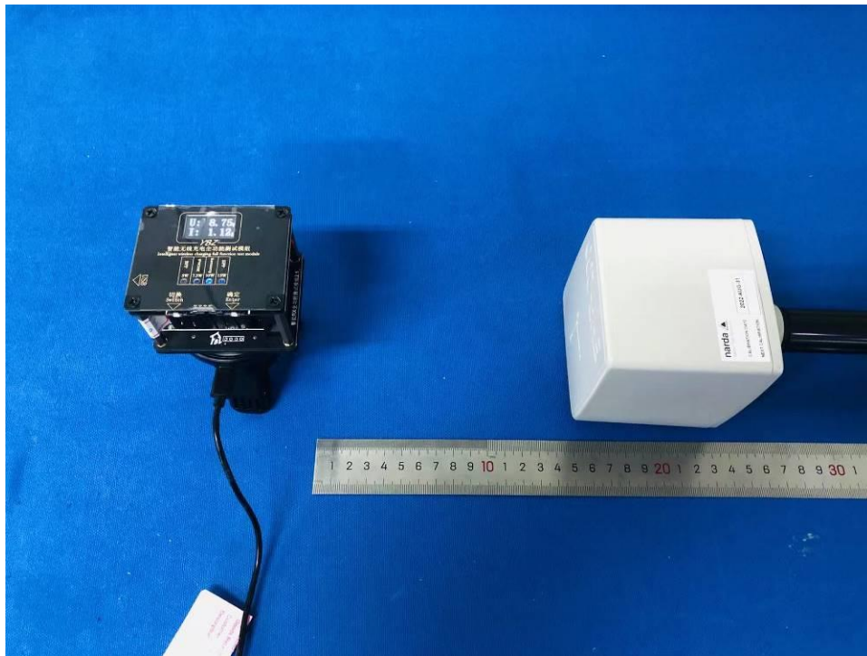
Photograph 1: Set-up photo for EMF (EPP)
