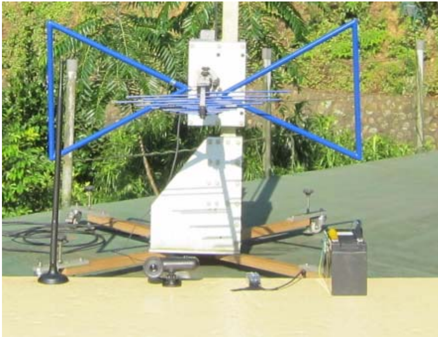
Closer View of the Test Setup below 1GHz
