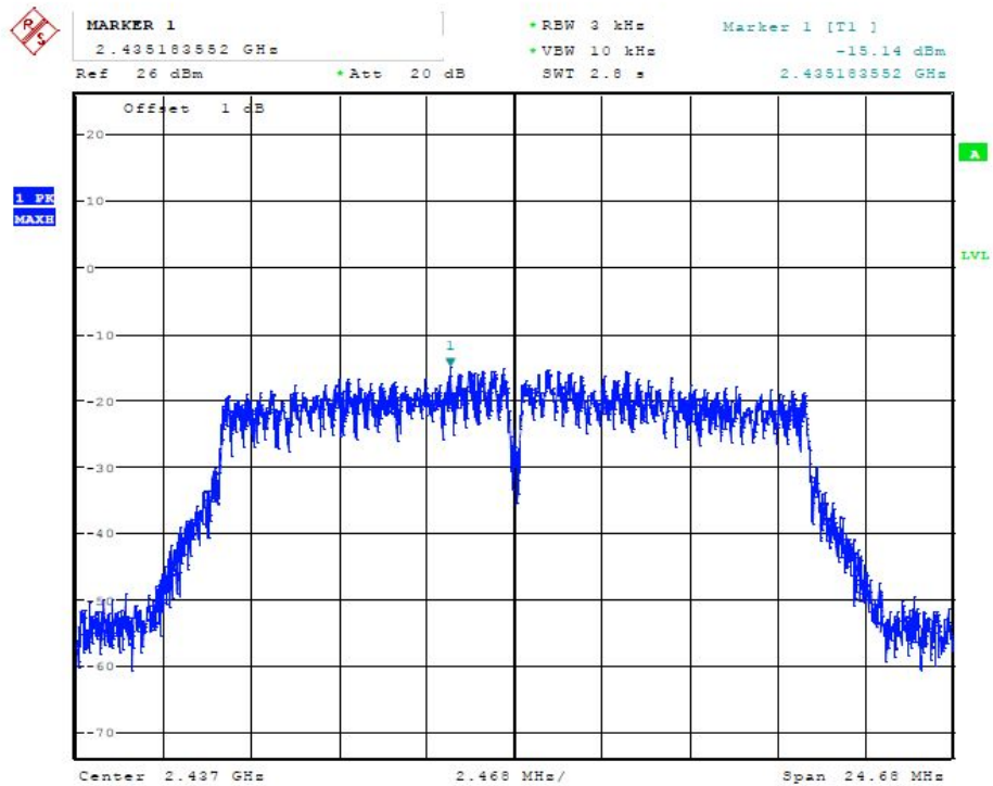
(Plot 4.4.2 B: Channel 6: 2437MHz @ 802.11g)
