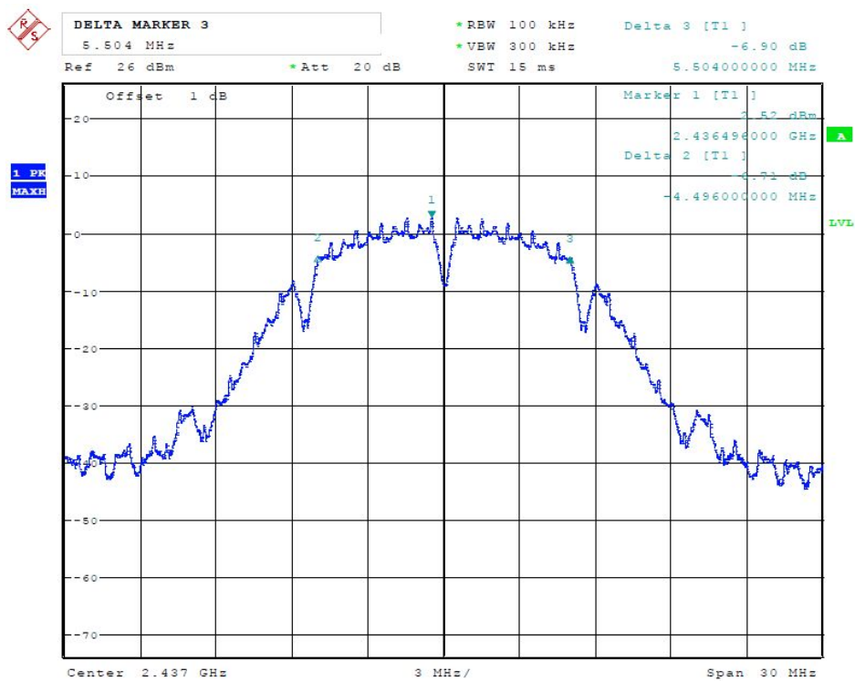
(Plot 4.7.1 B: Channel 6: 2437MHz @ 802.11b)
