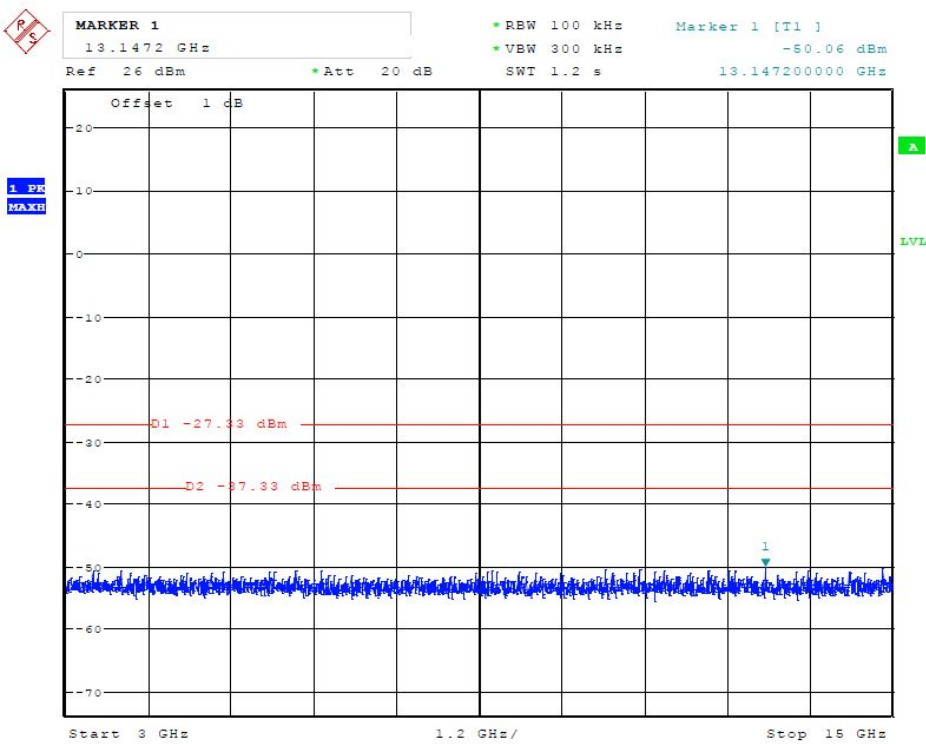
(Plot 4.6.4 A2: Channel 3: 2422MHz @ 802.11n HT40)
