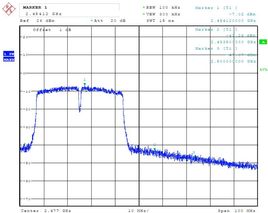
(Plot 4.5.2.4 B: Channel 9: 2452MHz @ 802.11n HT40)
