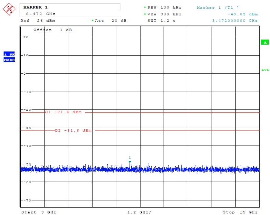
(Plot 4.6.2 C2: Channel 11: 2462MHz @ 802.11g)
