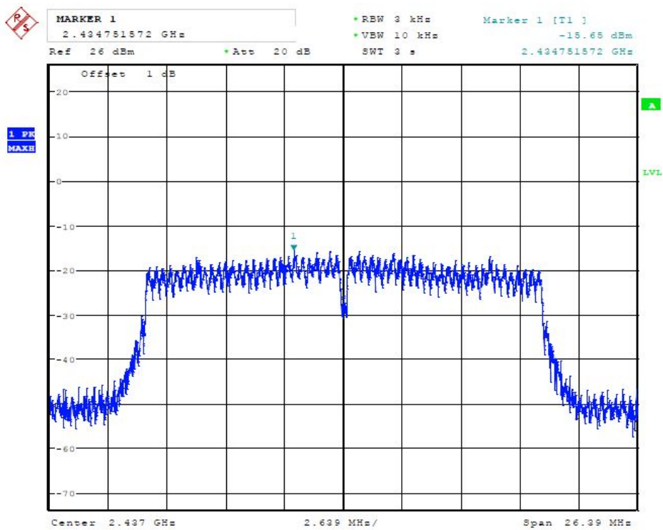
(Plot 4.4.3 B: Channel 6: 2437MHz @ 802.11n HT20)
