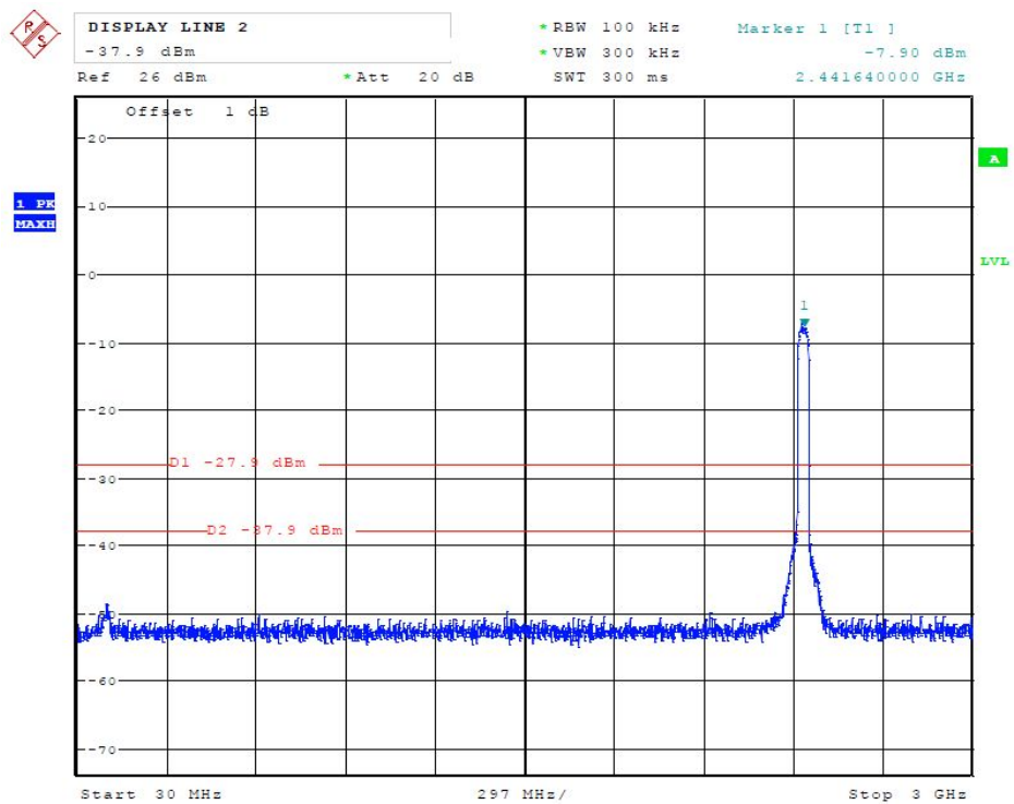
(Plot 4.6.4 B1: Channel 6: 2437MHz @ 802.11n HT40)
