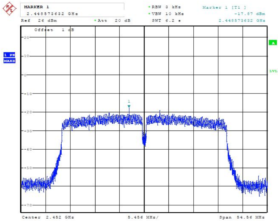
(Plot 4.4.4 C: Channel 6: 2452MHz @ 802.11n HT40)
