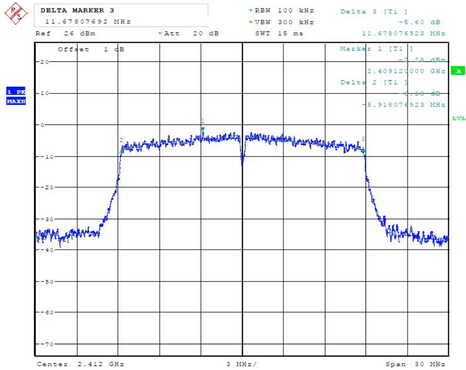
(Plot 4.7.3 A: Channel 1: 2412MHz @ 802.11n HT20)
