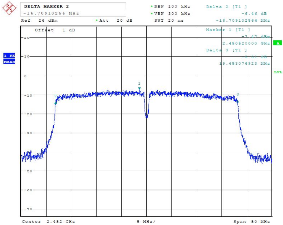
(Plot 4.7.4 C: Channel 9: 2452MHz @ 802.11n HT40)
