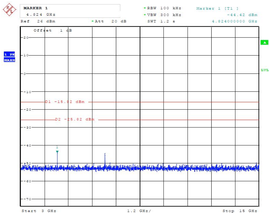
(Plot 4.6.1 A2: Channel 1: 2412MHz @ 802.11b)
