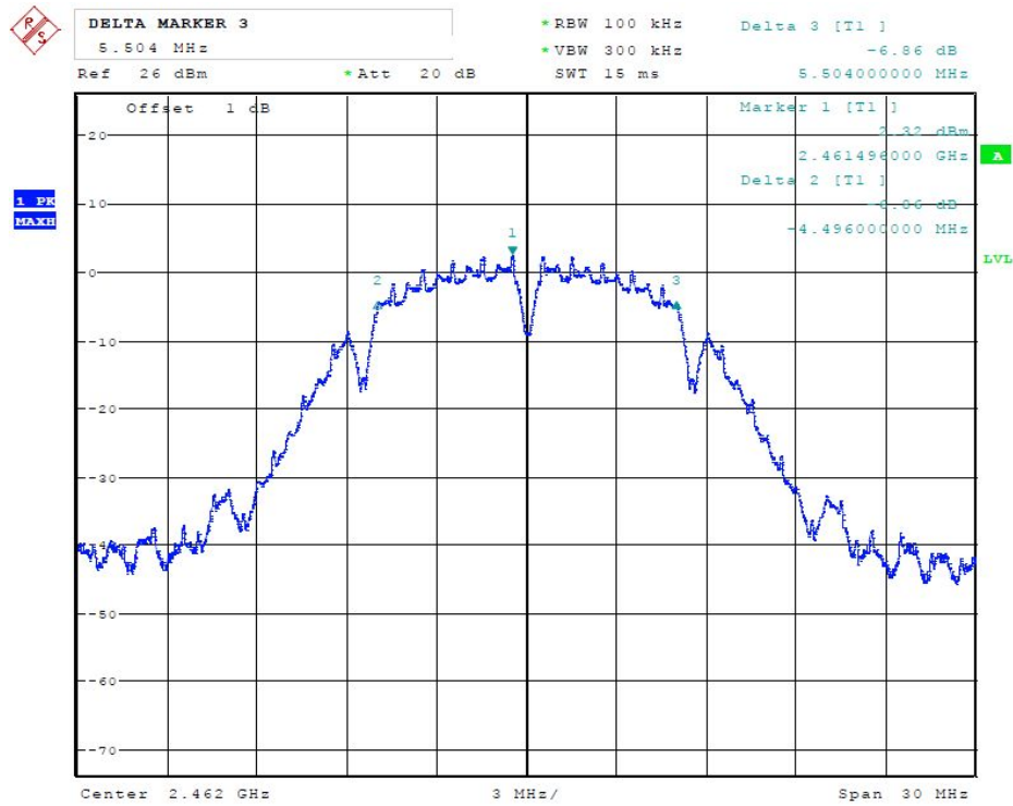
(Plot 4.7.1 C: Channel 11: 2462MHz @ 802.11b)
