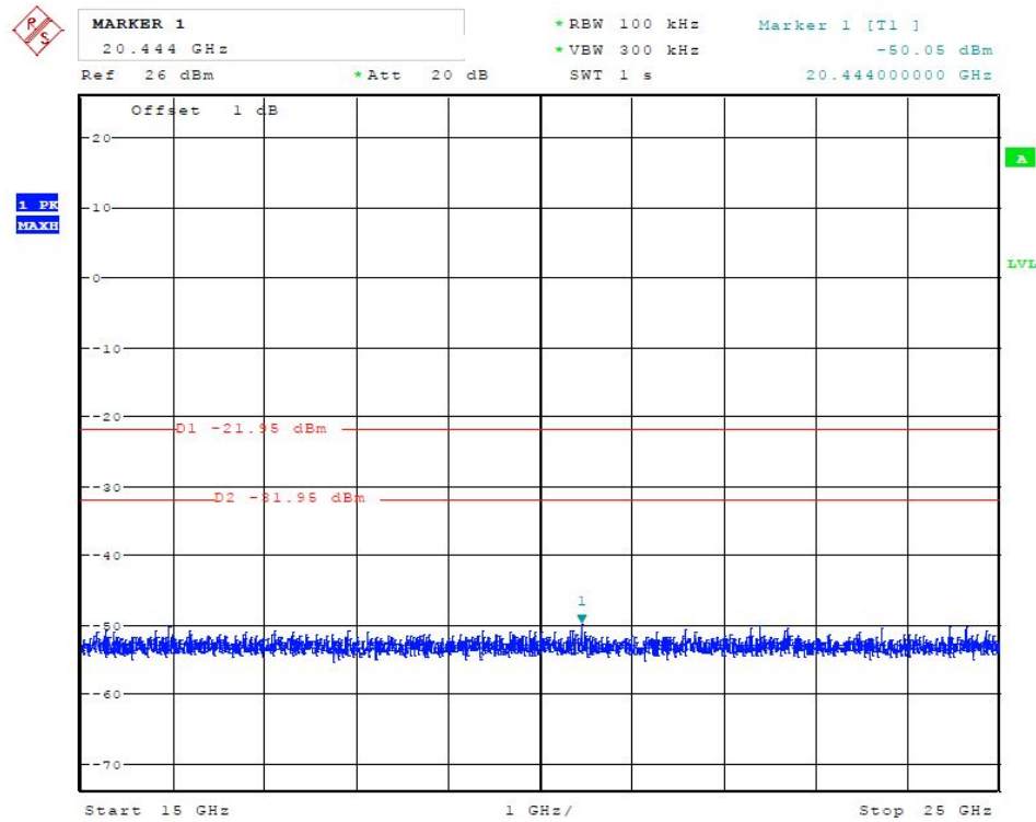
(Plot 4.6.3 A3: Channel 1: 2412MHz @ 802.11n HT20)
