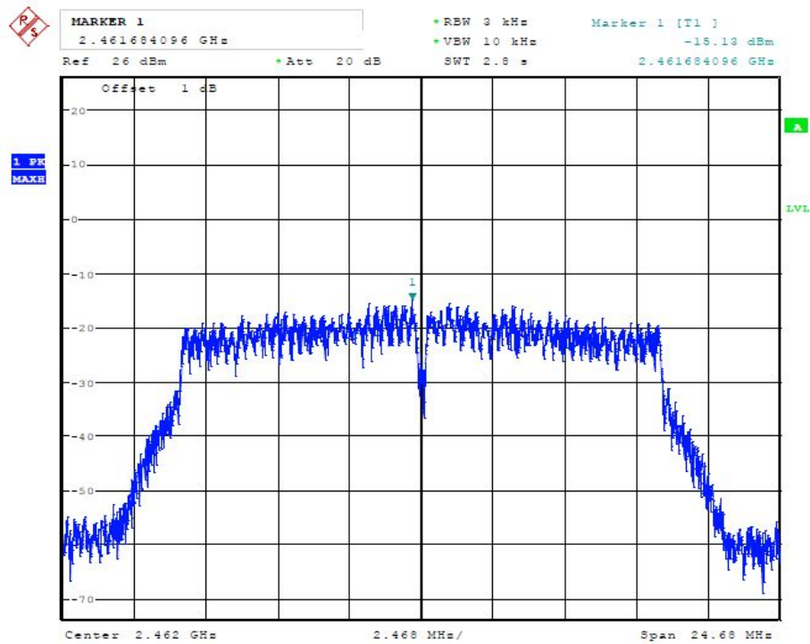
(Plot 4.4.2 C: Channel 11: 2462MHz @ 802.11g)
