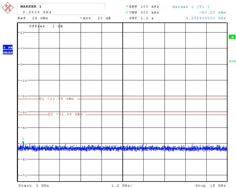
(Plot 4.6.3 A2: Channel 1: 2412MHz @ 802.11n HT20)
