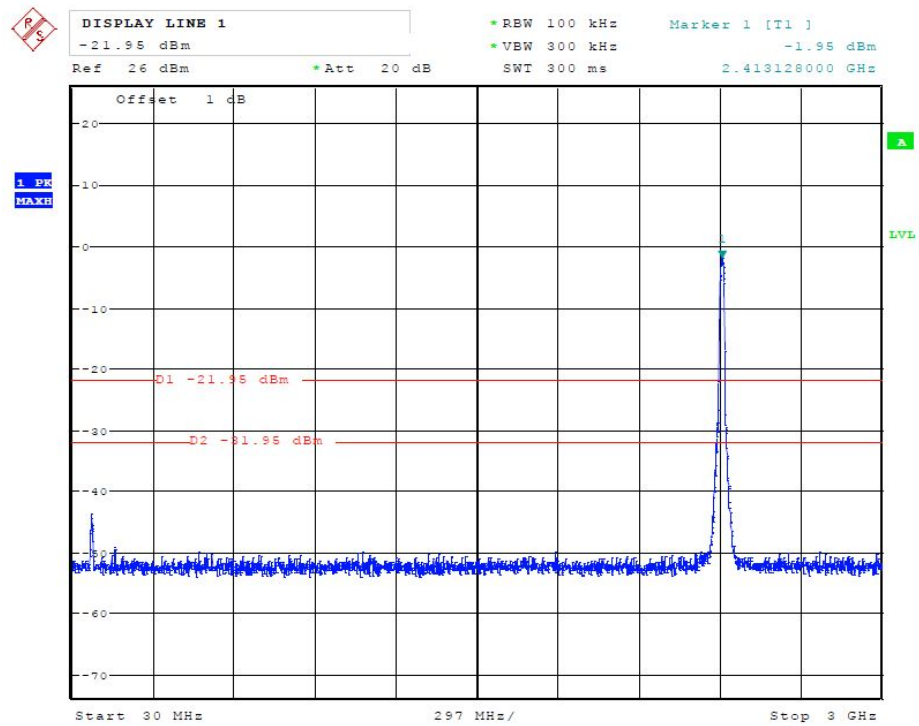
(Plot 4.6.3 A1: Channel 1: 2412MHz @ 802.11n HT20)
