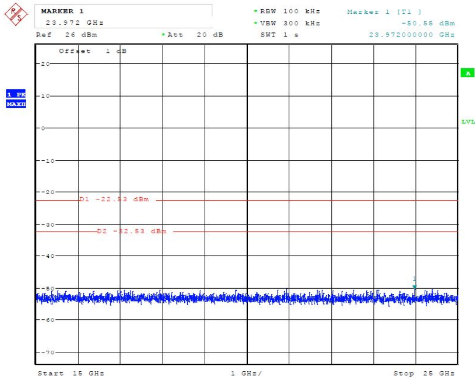
(Plot 4.6.3 C2: Channel 11: 2462MHz @ 802.11n HT20)
