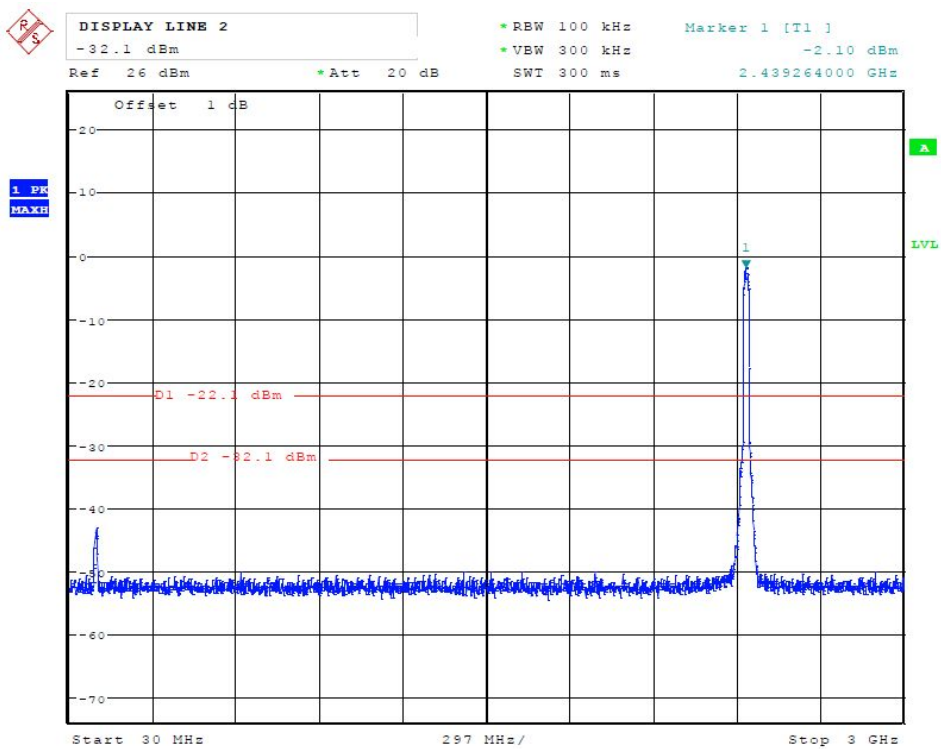
(Plot 4.6.3 B1: Channel 6: 2437MHz @ 802.11n HT20)
