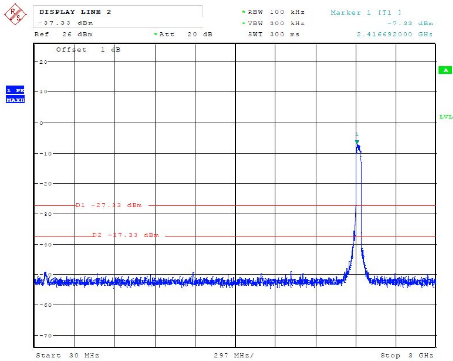
(Plot 4.6.4 A1: Channel 3: 2422MHz @ 802.11n HT40)
