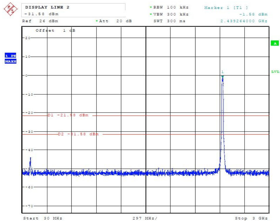
(Plot 4.6.2 B1: Channel 6: 2437MHz @ 802.11g)
