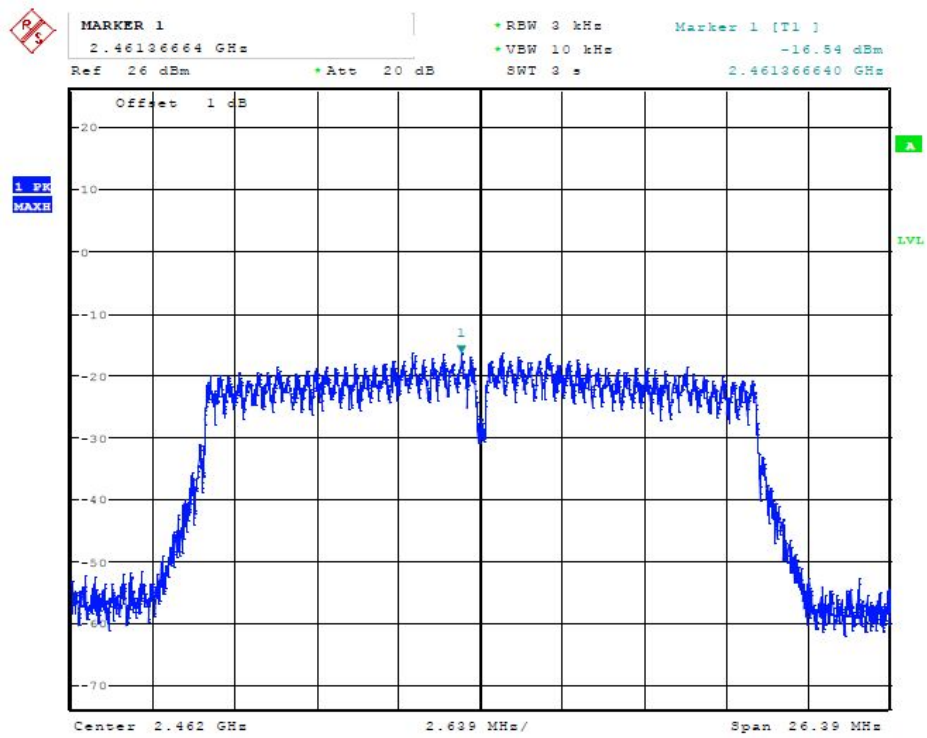
(Plot 4.4.3 C: Channel 11: 2462MHz @ 802.11n HT20)
