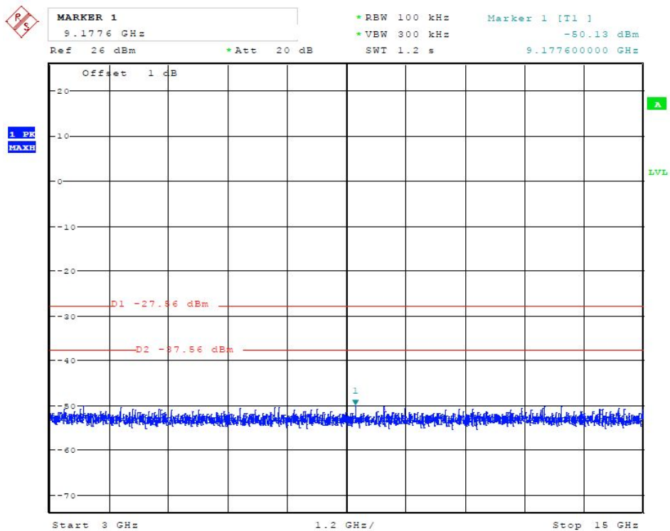
(Plot 4.6.4 C2: Channel 9: 2452MHz @ 802.11n HT40)
