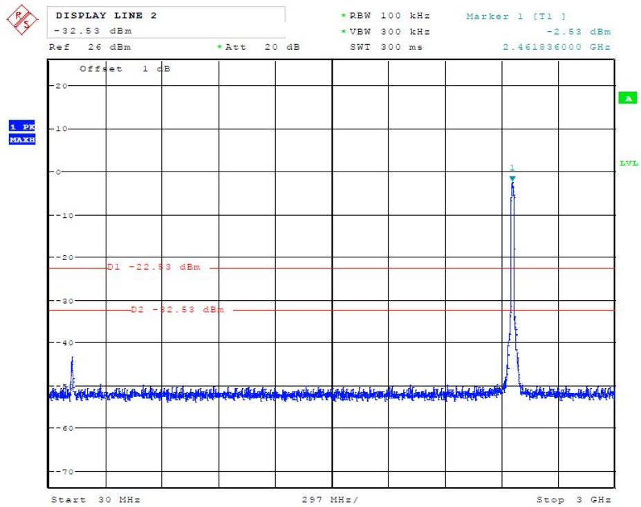
(Plot 4.6.3 C1: Channel 11: 2462MHz @ 802.11n HT20)
