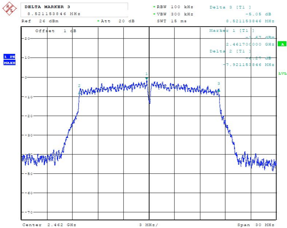
(Plot 4.7.2 C: Channel 11: 2462MHz @ 802.11g)
