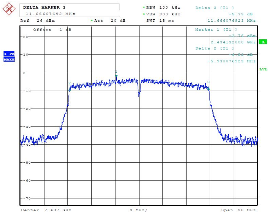
(Plot 4.7.3 B: Channel 6: 2437MHz @ 802.11n HT20)
