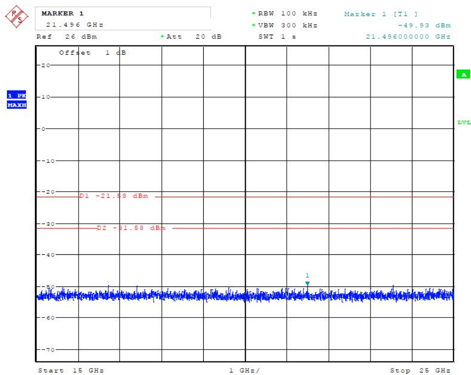
(Plot 4.6.2 B3: Channel 6: 2437MHz @ 802.11g)
