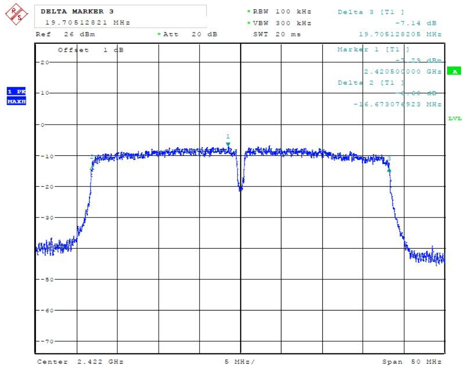
(Plot 4.7.4 A: Channel 3: 2422MHz @ 802.11n HT40)
