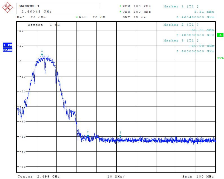
(Plot 4.5.2.1 B: Channel 11: 2462MHz @ 802.11 b )
