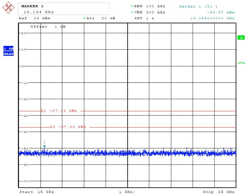
(Plot 4.6.4 A3: Channel 3: 2422MHz @ 802.11n HT40)
