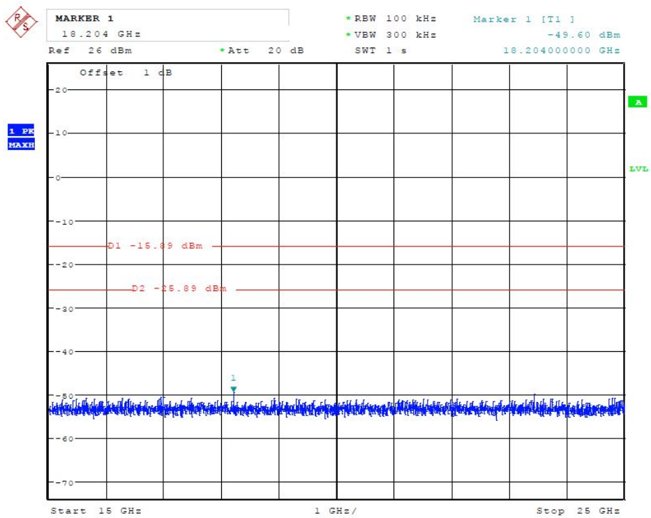
(Plot 4.6.1 B3: Channel 6: 2437MHz @ 802.11b)
