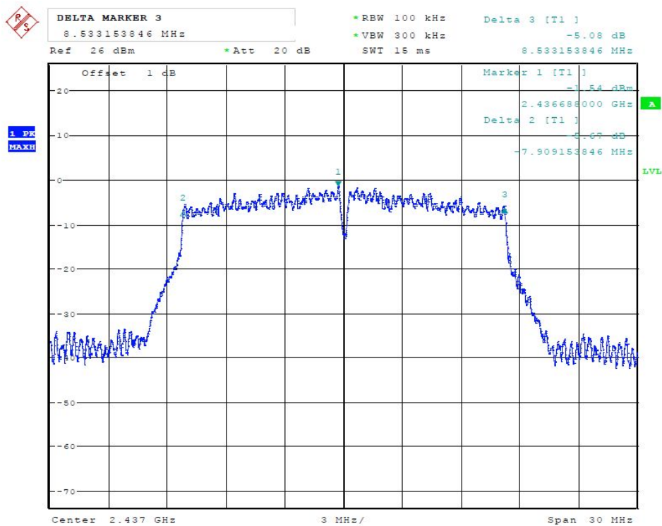
(Plot 4.7.2 B: Channel 6: 2437MHz @ 802.11g)
