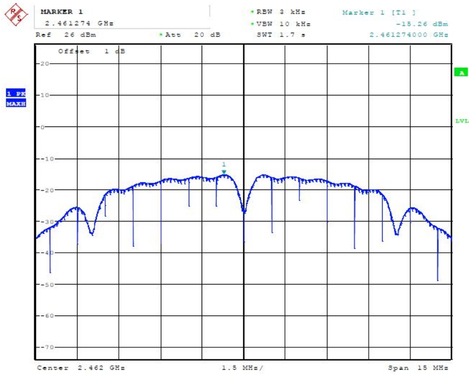
(Plot 4.4.1 C: Channel 11: 2462MHz @ 802.11b)
