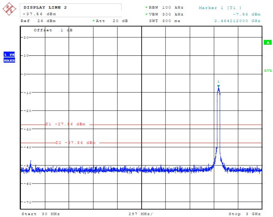
(Plot 4.6.4 C1: Channel 9 : 2452MHz @ 802.11n HT40)
