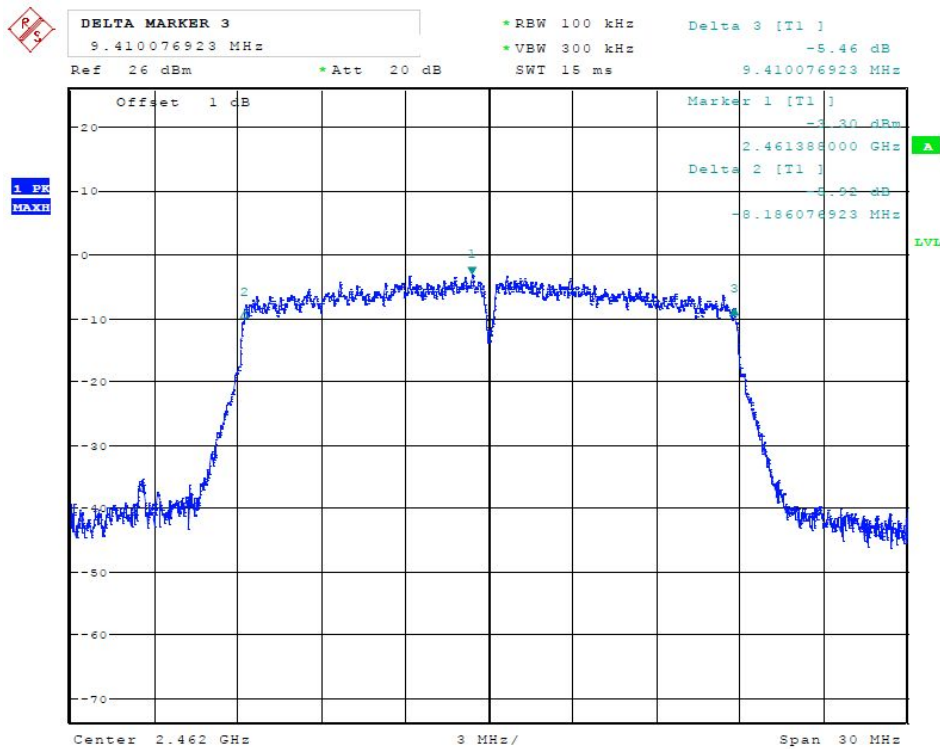
(Plot 4.7.3 C: Channel 11: 2462MHz @ 802.11n HT20)
