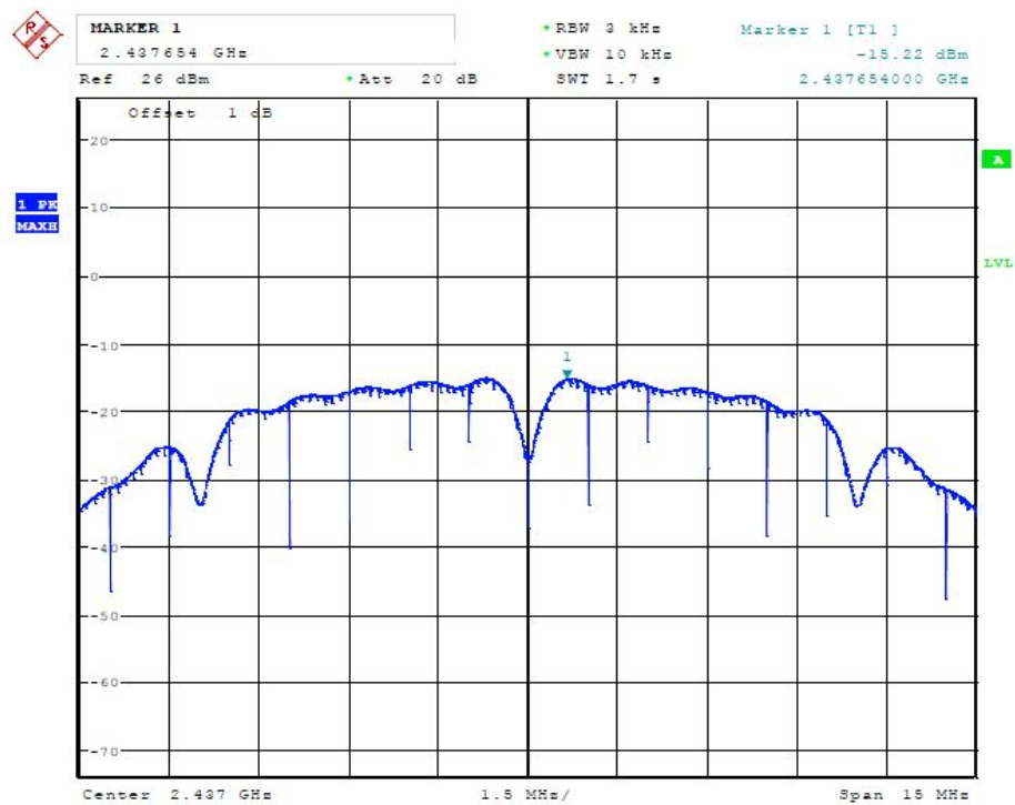
(Plot 4.4.1 B: Channel 6: 2437MHz @ 802.11b)
