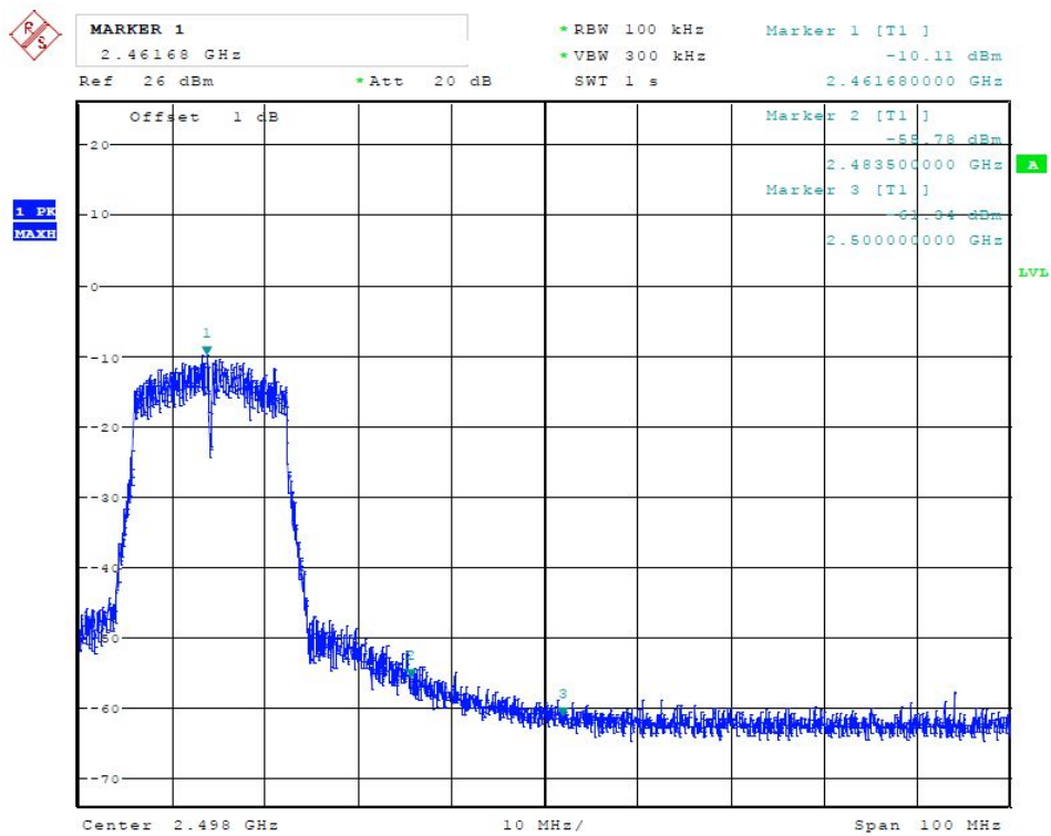
(Plot 4.5.2.2 B: Channel 11: 2462MHz @ 802.11 g)
