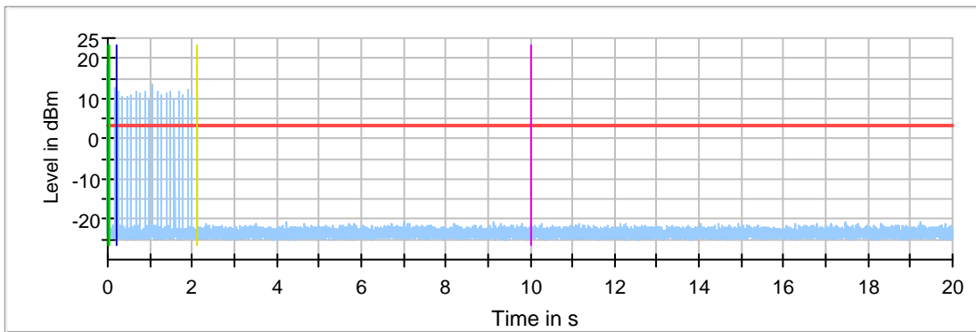
— In-Service Monitoring Channel Move Time — Threshold — Start of Radar — Trigger at end of Radar — First 200ms of Channel Closing Tx Time — 10sec Channel Move Time Limit — Last measured edge of Channel Closing Tx Time
