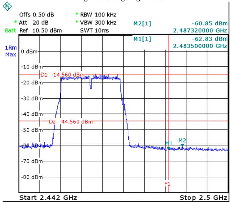
11g: Band edge-right side
