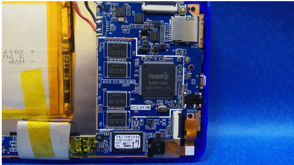
MAIN BOARD TOP VIEW
