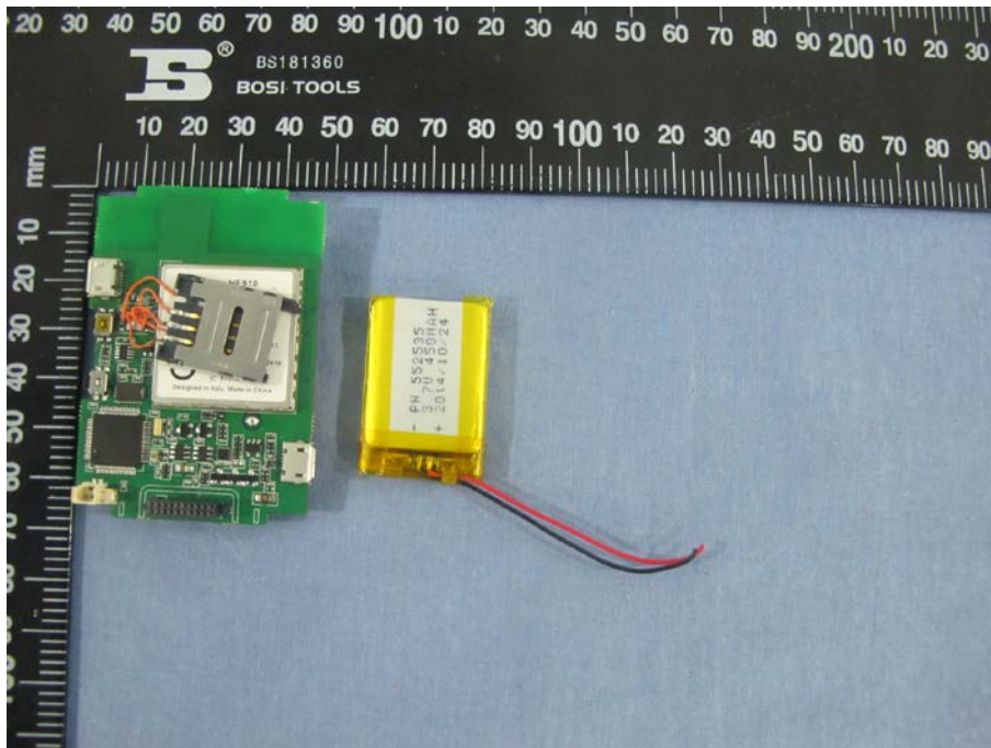
Pic.2 Internal Photo
