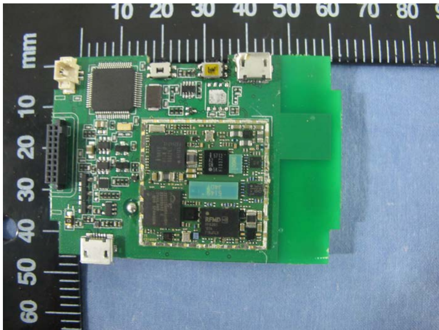
Pic.4 PCB front side
