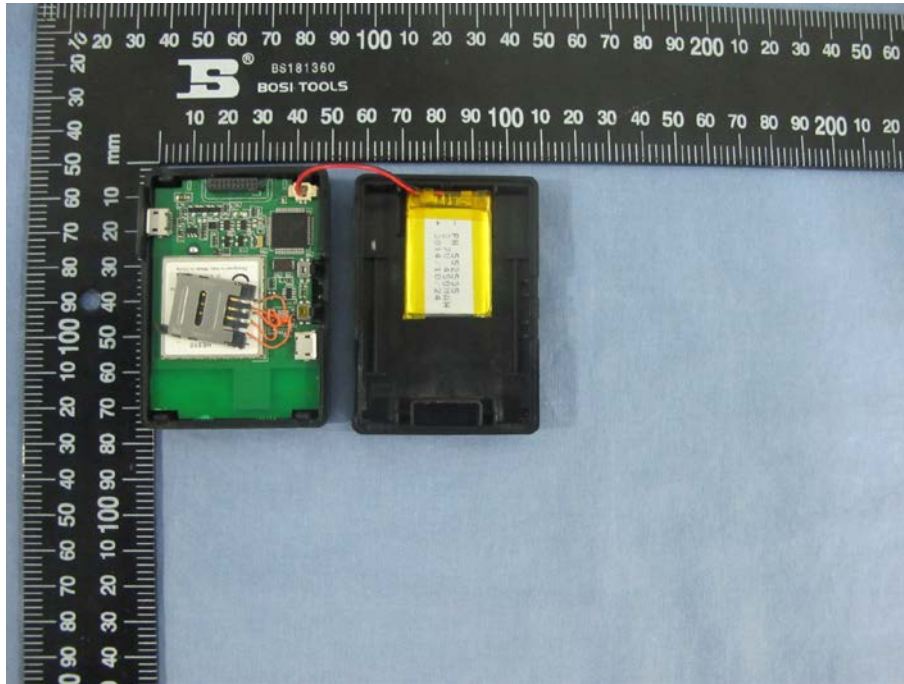
Pic.1 Internal Photo
