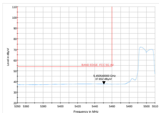
802.11a-Channel 100: Average
