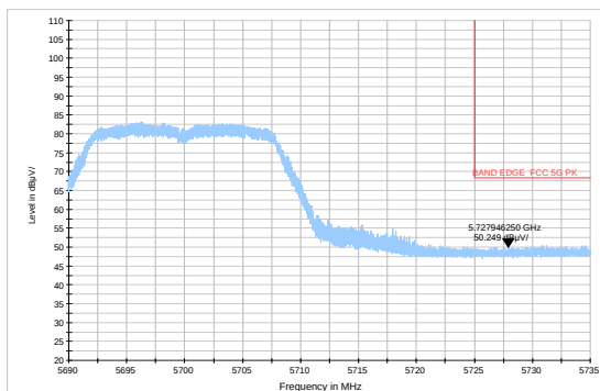
802.11a-Channel 140: Peak
