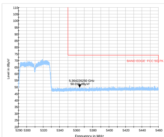
802.11ac HT40-Channel 62: Peak
