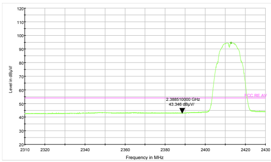
802.11b-Channel 1: Average
