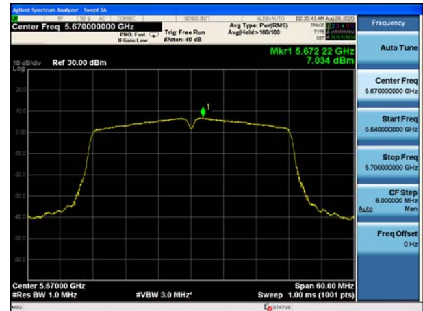
U-NII-2C, 802.11n HT40, Channel No.: 134
