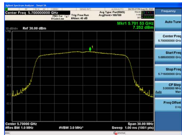
U-NII-2C, 802.11ax HE20, Channel No.: 140
