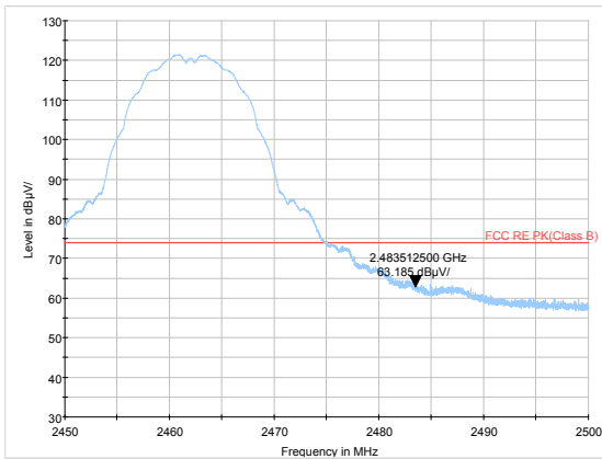
802.11b-Channel 11 Peak
