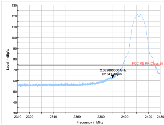
802.11b-Channel 1 Peak
