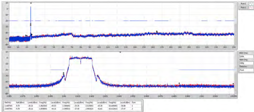
802.11g_Nss1,(6Mbps)_2TX 2412MHz
