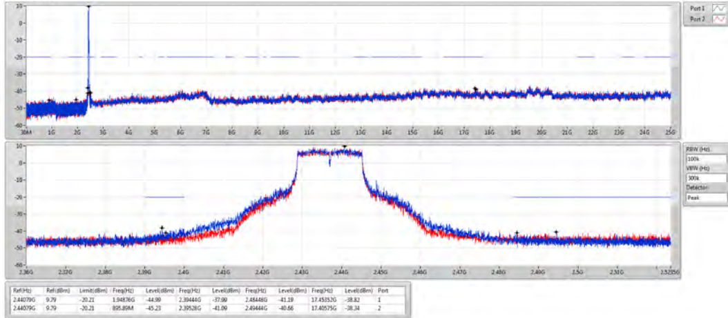
802.11g_Nss1,(6Mbps)_2TX 2437MHz
