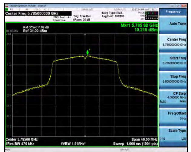
U-NII-3, 802.11ac VHT20, Channel No.: 157
