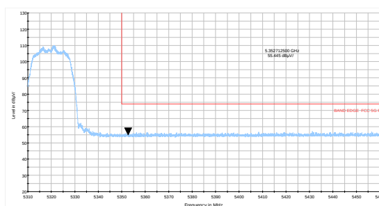
802.11a-Channel 64: Average
