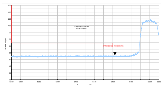
802.11a-Channel 100: Average
