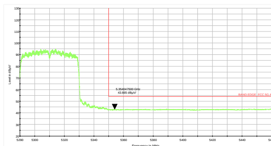
802.11ac VHT80- Channel 58: Average
