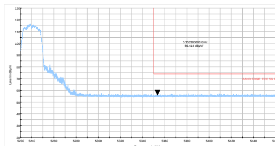
802.11a-Channel 48: Average
