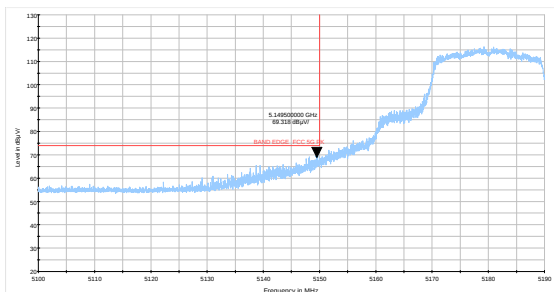
802.11ax HE20-Channel 36: Average
