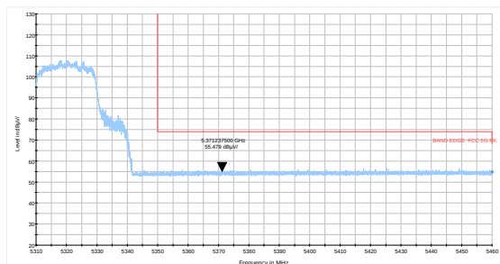
802.11ax HE20 -Channel 64: Average
