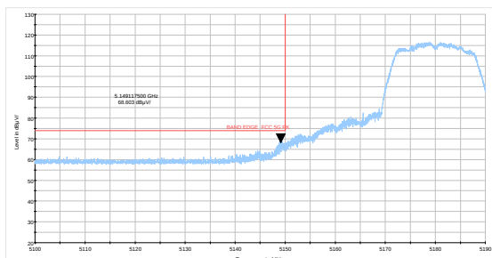
802.11a-Channel 36: Average
