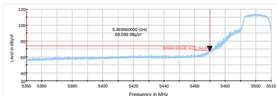
802.11a-Channel 100: Average
