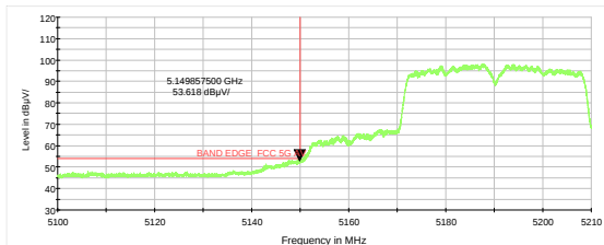
802.11ac VHT20 -Channel 36: Peak
