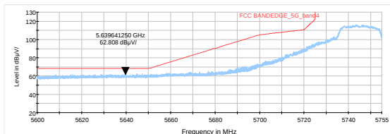
802.11ac VHT40-Channel 151: Peak
