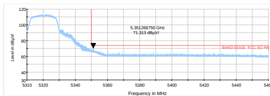
802.11a-Channel 64: Peak
