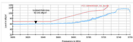
802.11a-Channel 149: Peak
