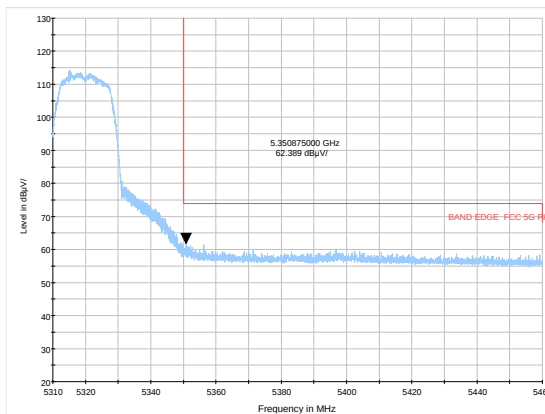
802.11a-Channel 64: Average
