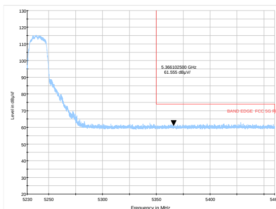
802.11a-Channel 48: Average
