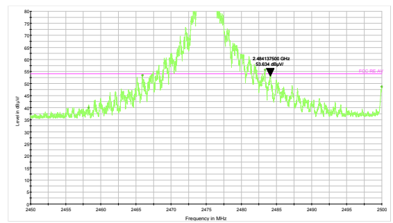
Zigbee-Channel 25: Average
