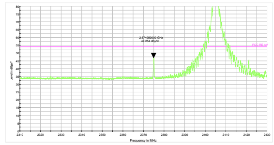
Zigbee-Channel 11: Average
