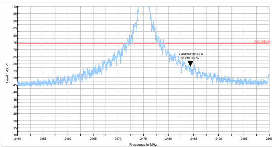
Zigbee-Channel 25: Peak
