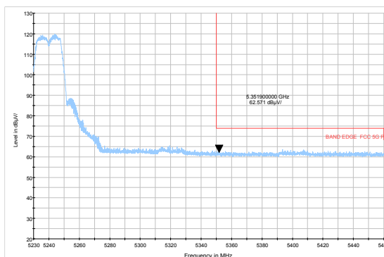
802.11a-Channel 48: Average
