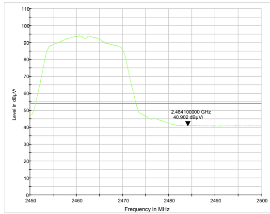
802.11g-Channel 11: Average
