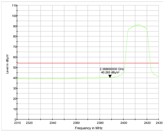
802.11g-Channel 1: Average
