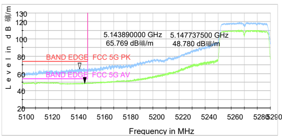
802.11n HT40-Channel 54: Peak + Average
