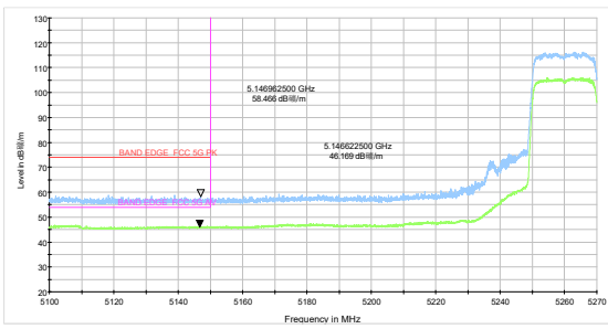
802.11ax HE40-Channel 54: Peak + Average
