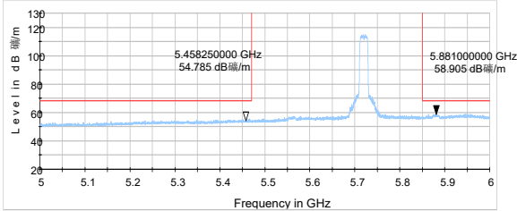
802.11a-Channel 144: Peak
