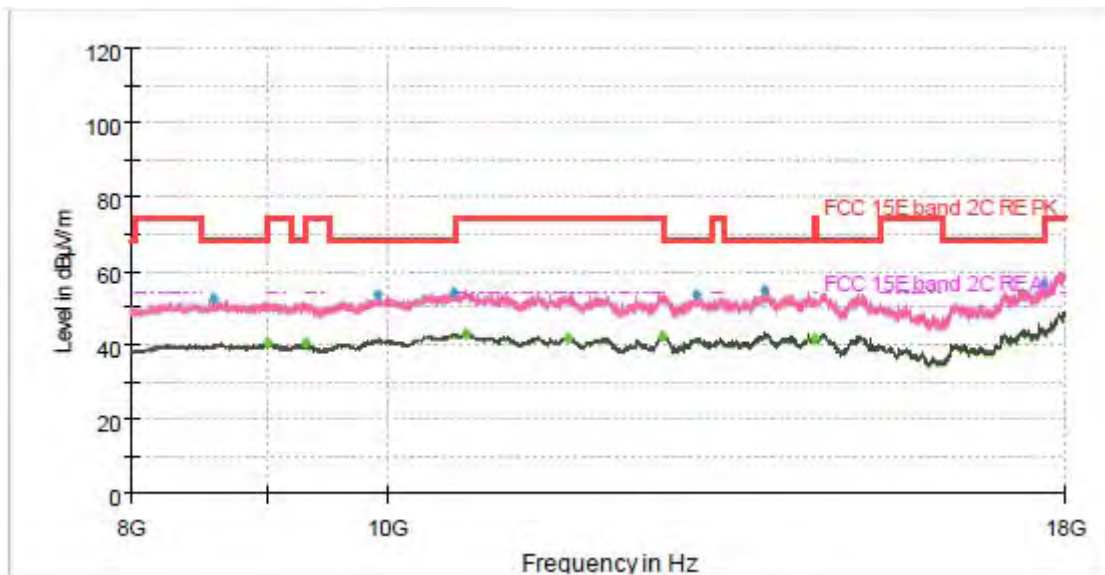
Radiates Emission from 8GHz to 18GHz
