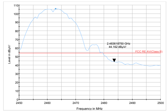
802.11g-Channel 11: Peak
