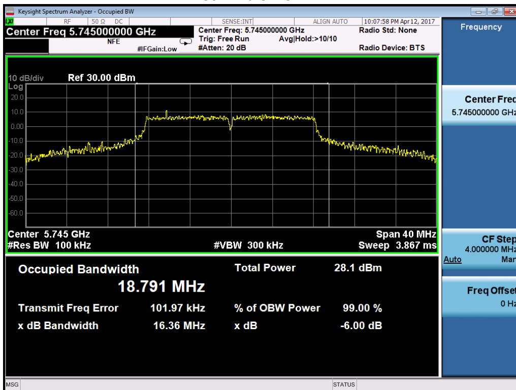
802.11a-5745MHz
