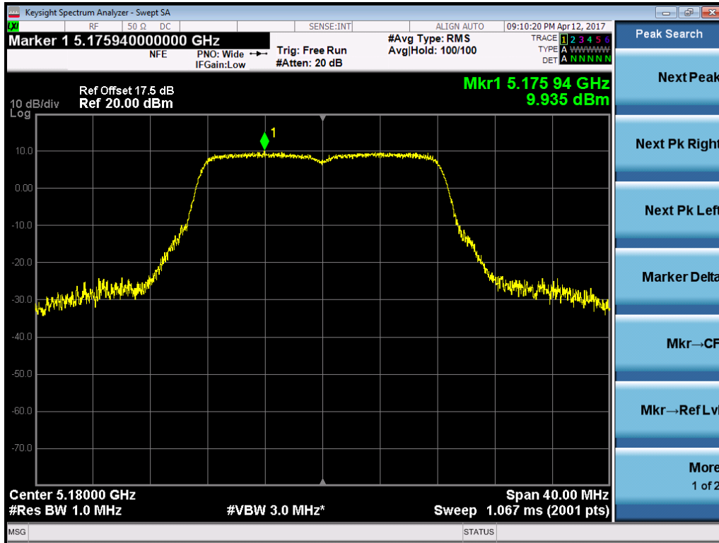
802.11a-5180MHz
