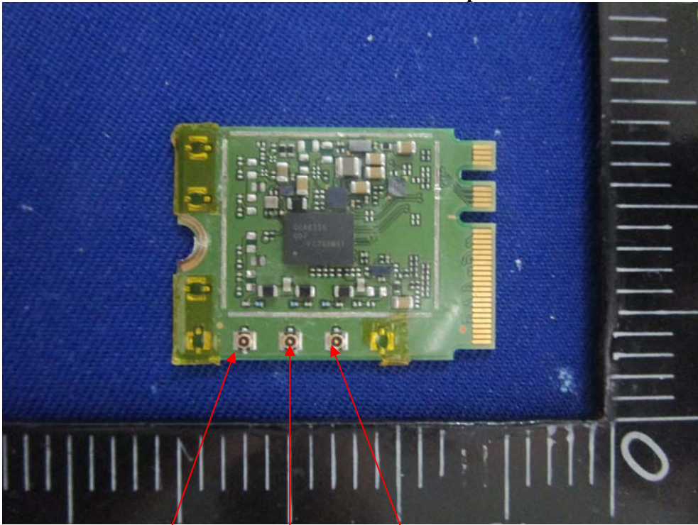
RF Port 0 RF Port 1 RF Port 2
