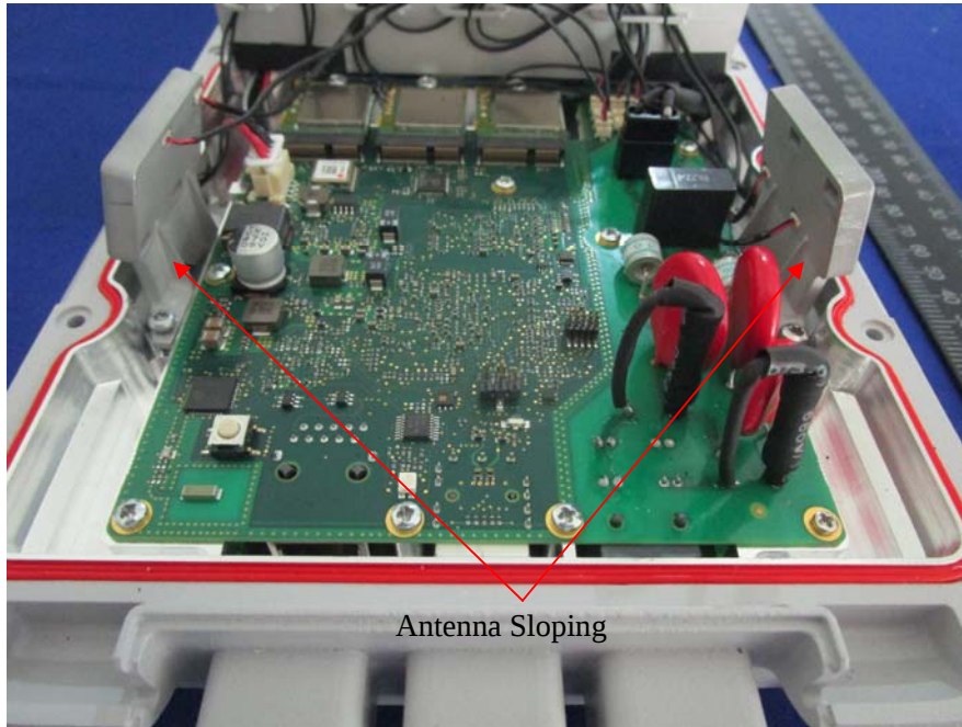
EUT –802.11ad Side Ant View
