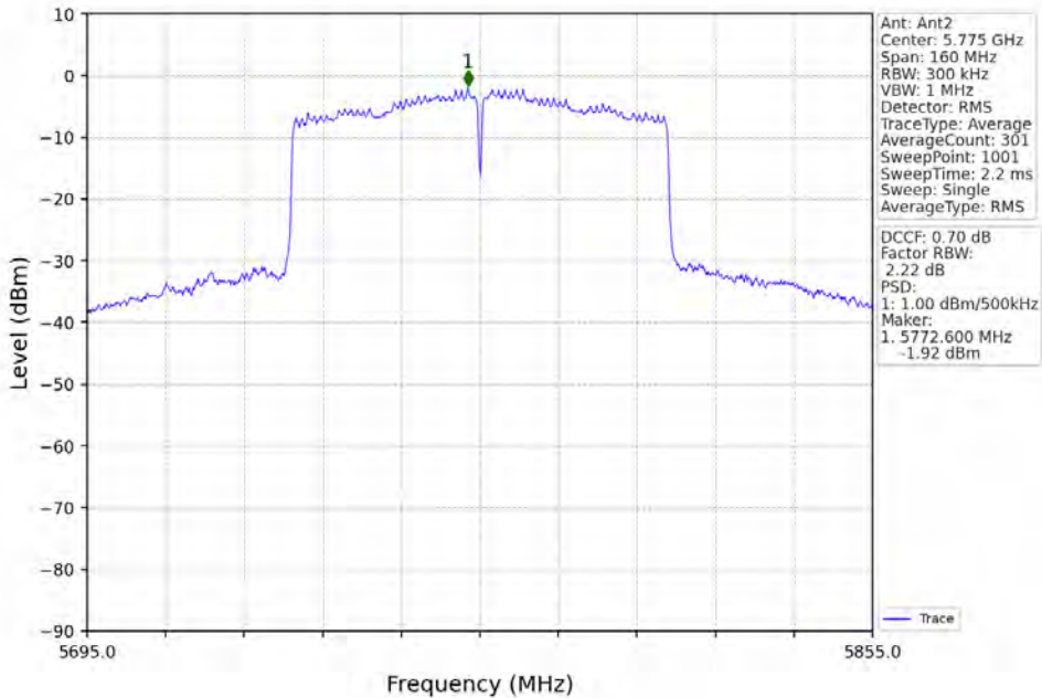
802.11ac(VHT80)_MCH_5775MHz_MIMO_NTNV
