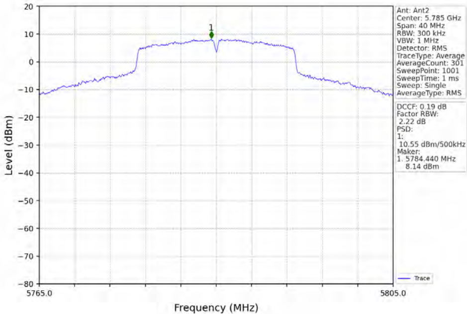
802.11ac(VHT20)_MCH_5785MHz_MIMO_NTNV
