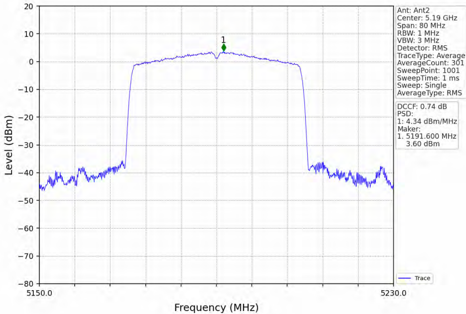
802.11ax(HEW40)_LCH_5190MHz_RU484_Left_MIMO_NTNV
