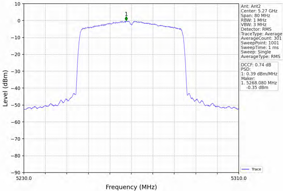
802.11ax(HEW40)_LCH_5270MHz_RU484_Left_MIMO_NTNV
