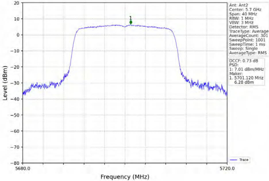
802.11ax(HEW20)_HCH_5700MHz_RU242_Left_MIMO_NTNV
