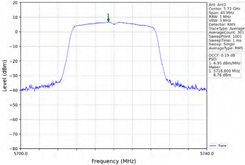
802.11ac(VHT20)_HCH_5720MHz_MIMO_NTNV
