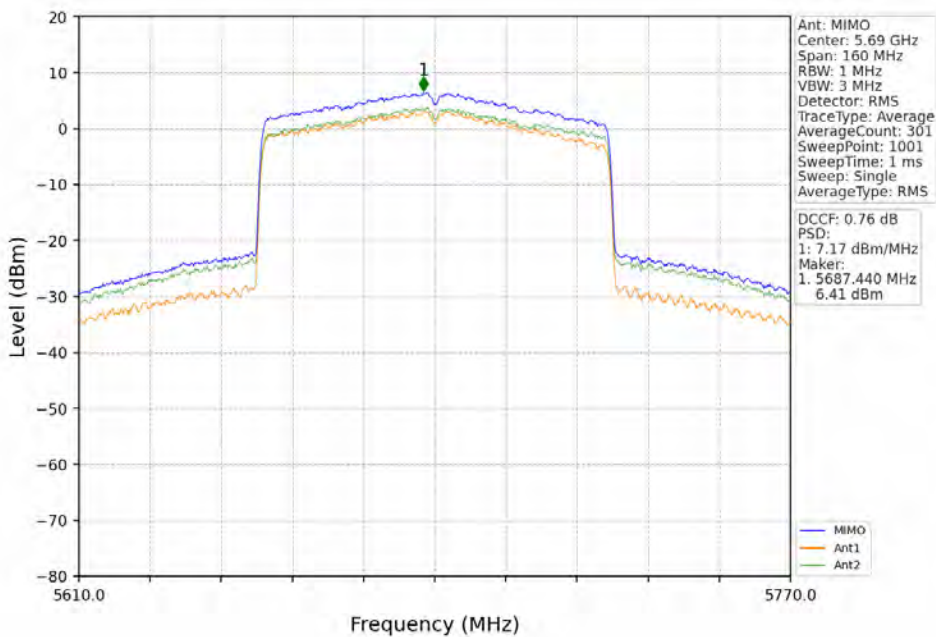
802.11ax(HEW80)_HCH_5690MHz_RU996_Left_MIMO_NTNV
