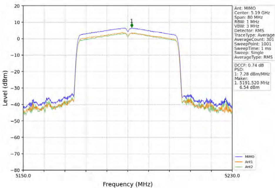
802.11ax(HEW40)_LCH_5190MHz_RU484_Left_MIMO_NTNV
