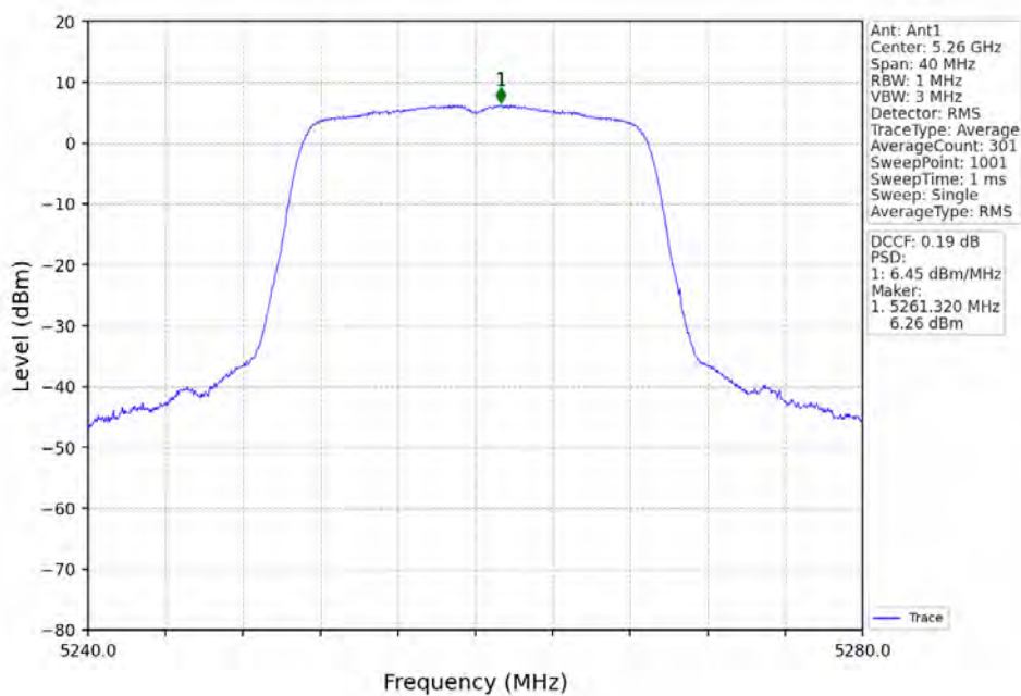
802.11ac(VHT20)_LCH_5260MHz_Ant1_NTNV
