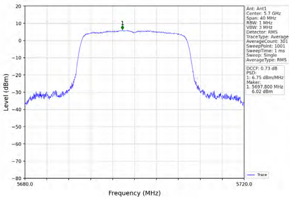
802.11ax(HEW20)_HCH_5700MHz_RU242_Left_Ant1_NTNV
