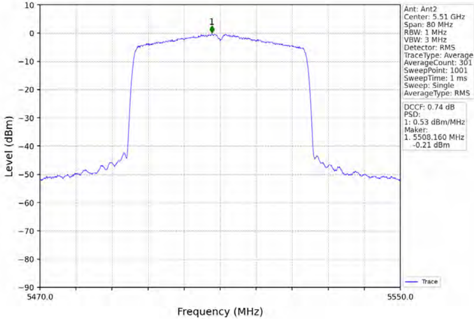
802.11ax(HEW40)_LCH_5510MHz_RU484_Left_MIMO_NTNV
