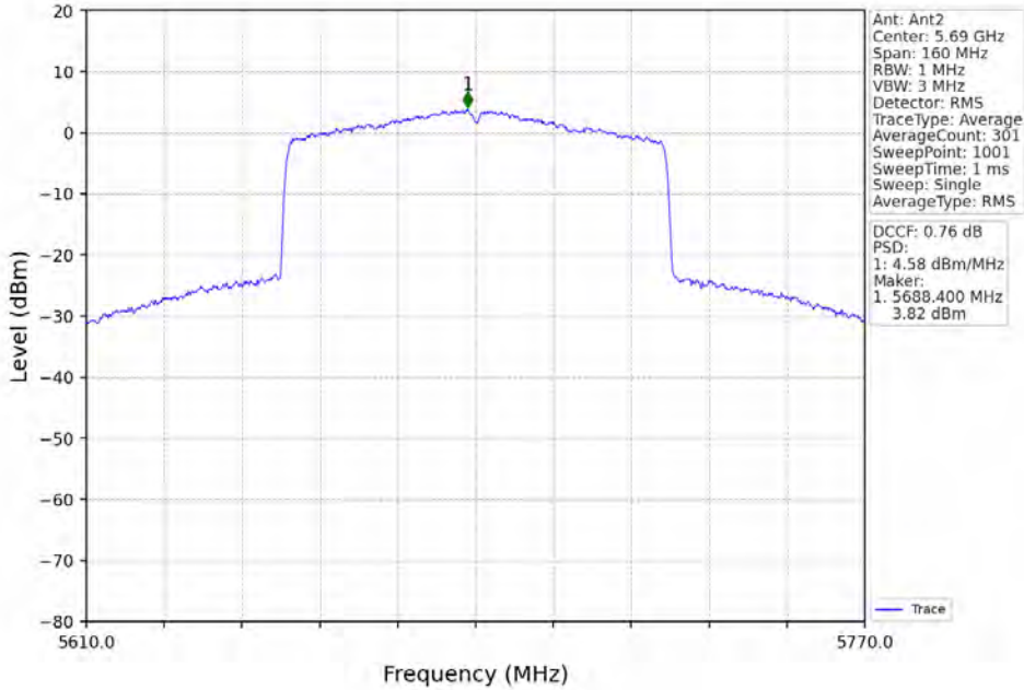
802.11ax(HEW80)_HCH_5690MHz_RU996_Left_MIMO_NTNV
