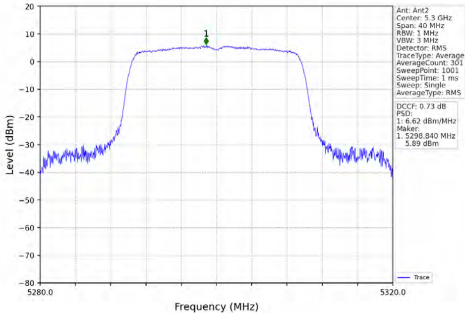
802.11ax(HEW20)_MCH_5300MHz_RU242_Left_MIMO_NTNV
