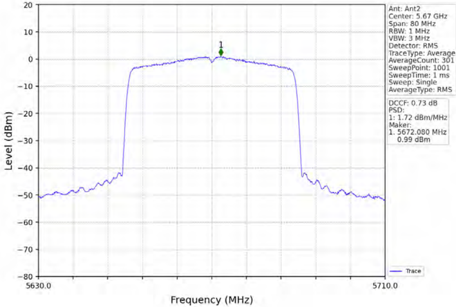
802.11ax(HEW40)_HCH_5670MHz_RU484_Left_MIMO_NTNV
