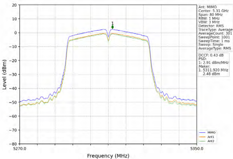
802.11n(HT40)_HCH_5310MHz_MIMO_NTNV
