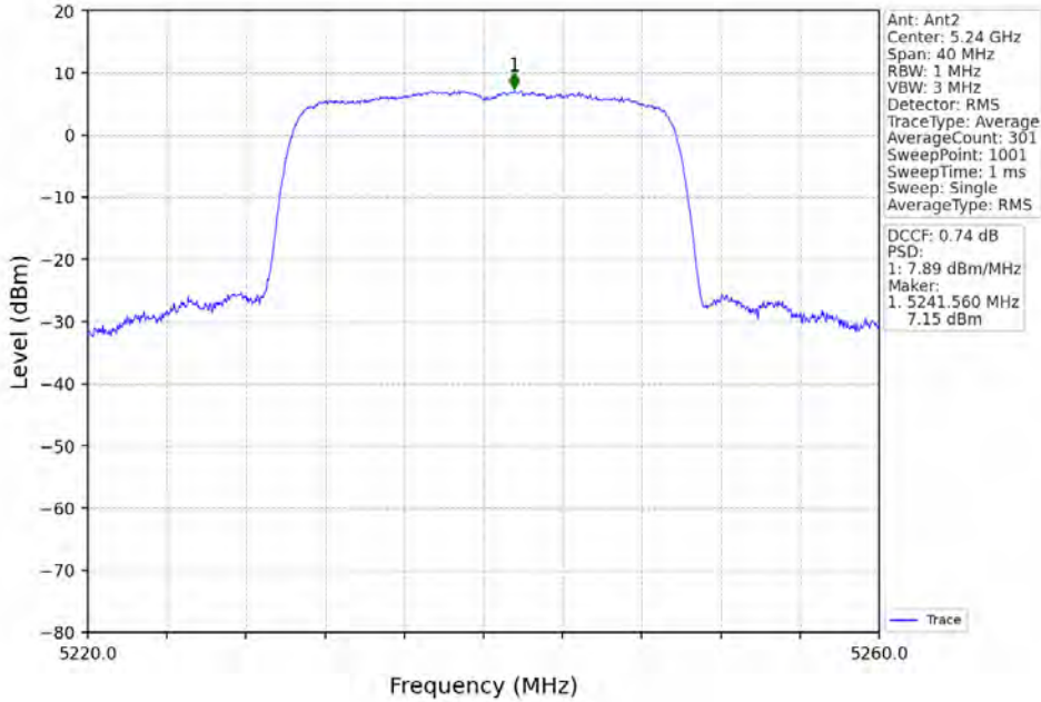
802.11ax(HEW20)_HCH_5240MHz_RU242_Left_MIMO_NTNV
