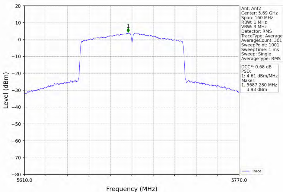
802.11ac(VHT80)_HCH_5690MHz_Ant2_NTNV
