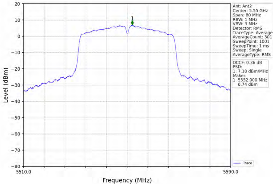
802.11ac(VHT40)_MCH_5550MHz_MIMO_NTNV
