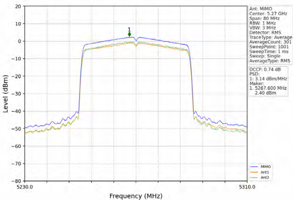
802.11ax(HEW40)_LCH_5270MHz_RU484_Left_MIMO_NTNV
