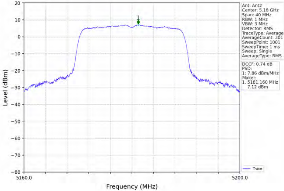
802.11ax(HEW20)_LCH_5180MHz_RU242_Left_MIMO_NTNV
