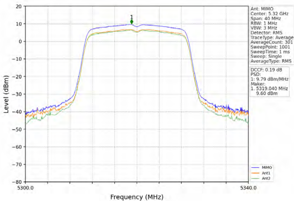
802.11ac(VHT20)_HCH_5320MHz_MIMO_NTNV
