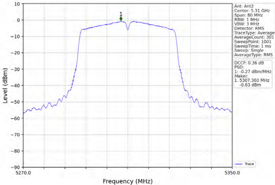
802.11ac(VHT40)_HCH_5310MHz_MIMO_NTNV
