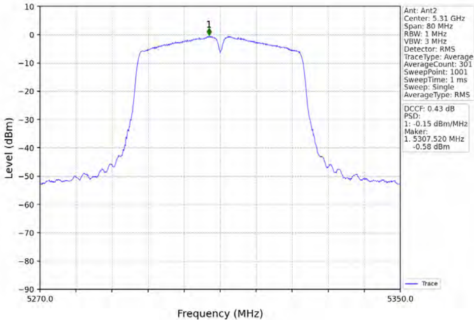
802.11n(HT40)_HCH_5310MHz_MIMO_NTNV
