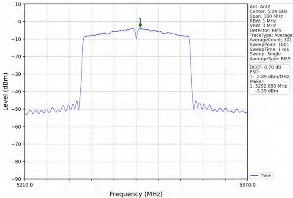
802.11ac(VHT80)_MCH_5290MHz_MIMO_NTNV
