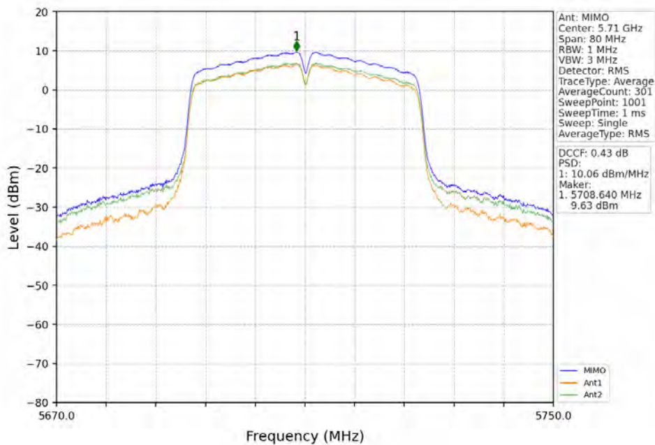
802.11n(HT40)_HCH_5710MHz_MIMO_NTNV
