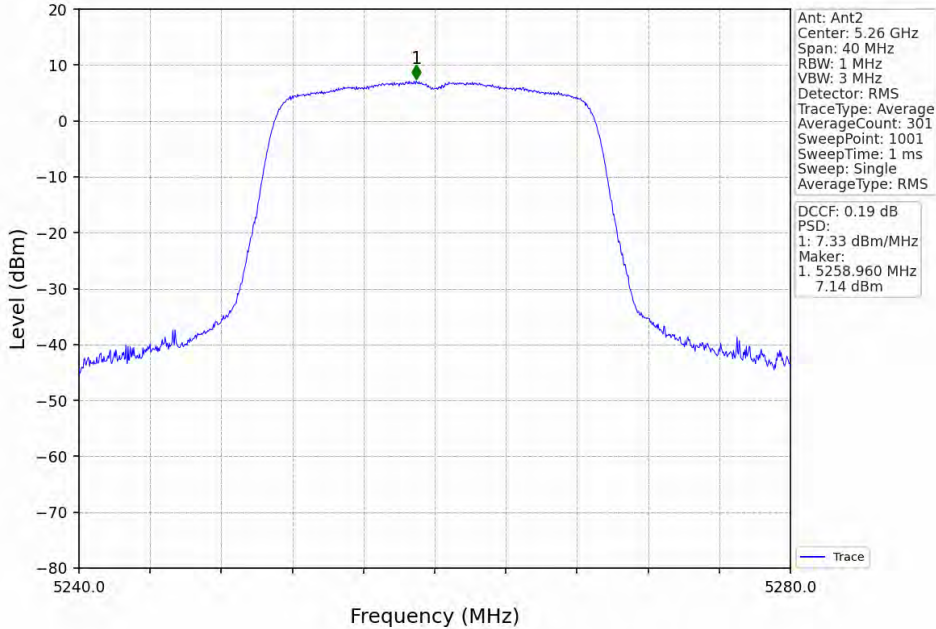
802.11n(HT20)_LCH_5260MHz_MIMO_NTNV
