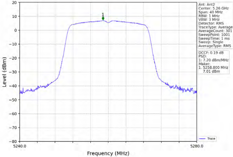
802.11ac(VHT20)_LCH_5260MHz_MIMO_NTNV
