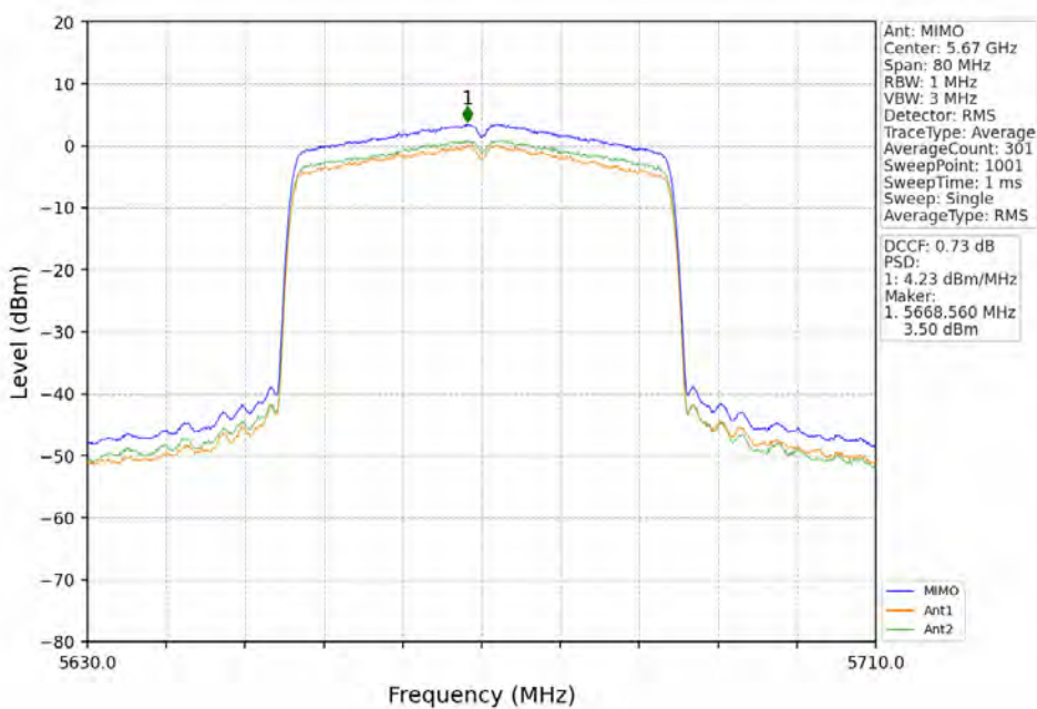
802.11ax(HEW40)_HCH_5670MHz_RU484_Left_MIMO_NTNV
