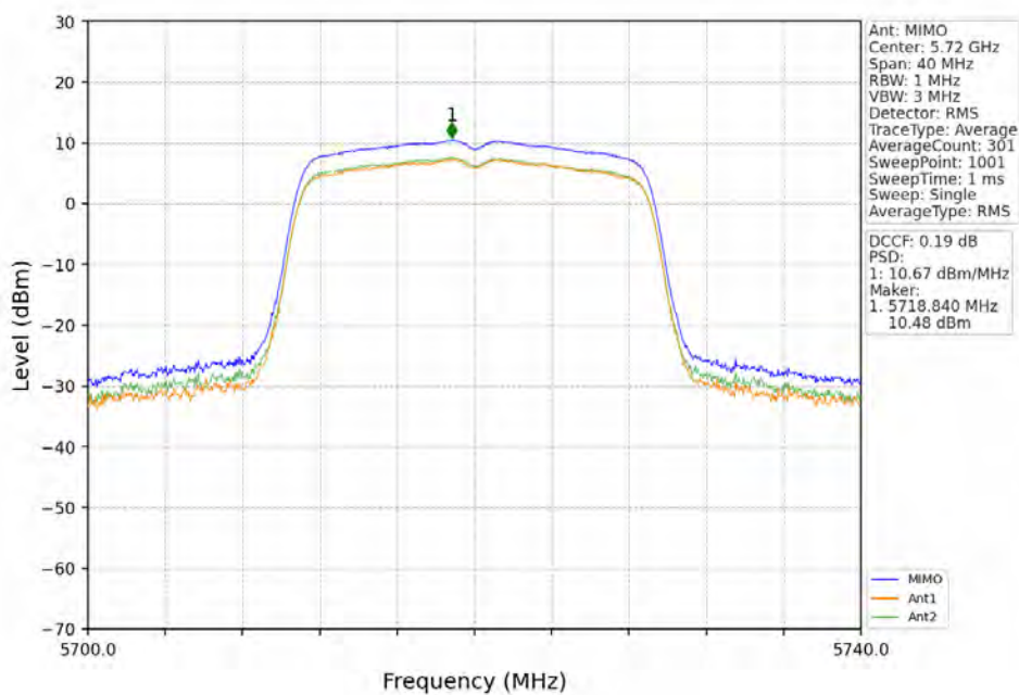
802.11ac(VHT20)_HCH_5720MHz_MIMO_NTNV
