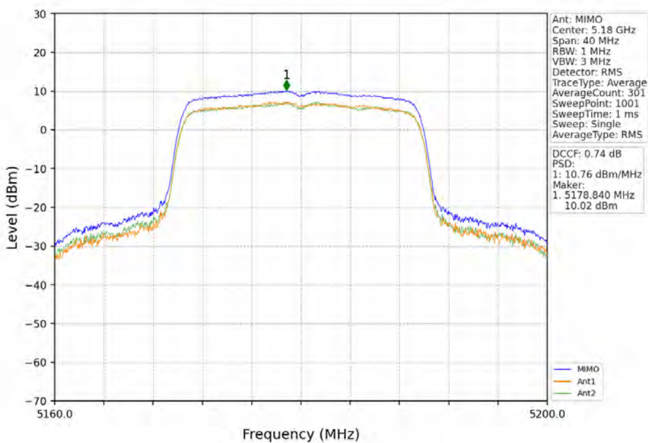
802.11ax(HEW20)_LCH_5180MHz_RU242_Left_MIMO_NTNV
