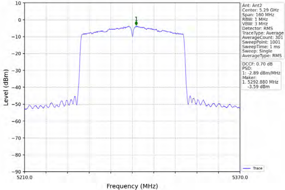
802.11ac(VHT80)_MCH_5290MHz_MIMO_NTNV
