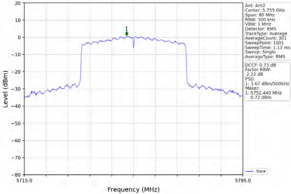
802.11ax(HEW40)_LCH_5755MHz_RU484_Left_MIMO_NTNV
