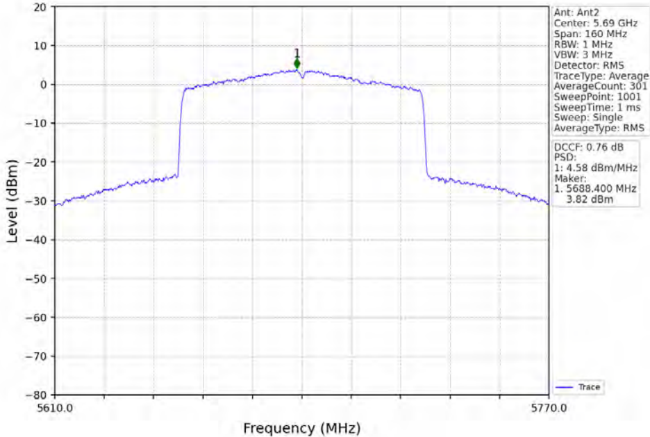
802.11ax(HEW80)_HCH_5690MHz_RU996_Left_MIMO_NTNV
