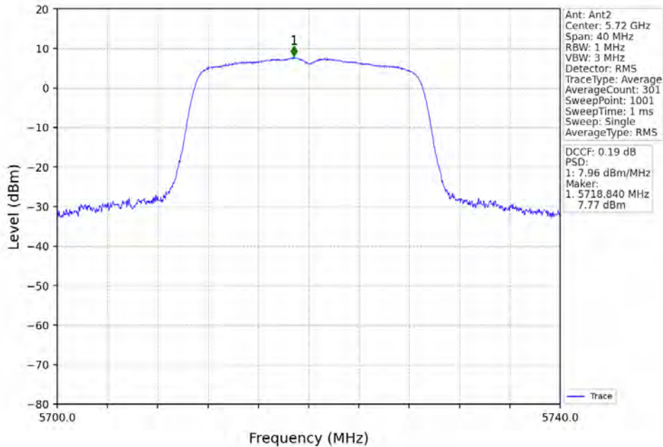
802.11ac(VHT20)_HCH_5720MHz_MIMO_NTNV
