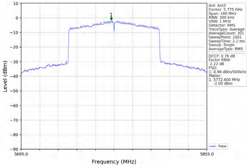
802.11ax(HEW80)_MCH_5775MHz_RU996_Left_MIMO_NTNV
