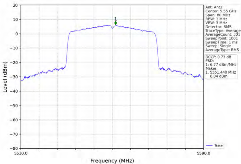
802.11ax(HEW40)_MCH_5550MHz_RU484_Left_Ant2_NTNV
