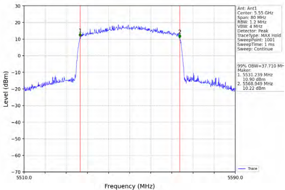
802.11ax(HEW40)_MCH_5550MHz_RU484_Left_Ant1_NTNV
