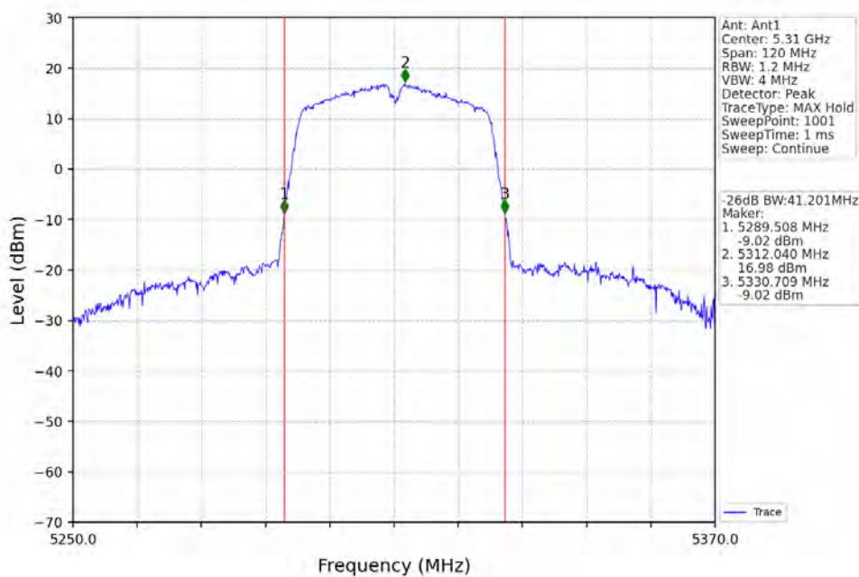
802.11ac(VHT40)_HCH_5310MHz_Ant1_NTNV
