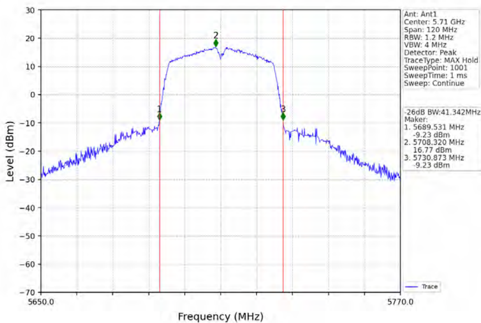
802.11ac(VHT40)_HCH_5710MHz_Ant1_NTNV
