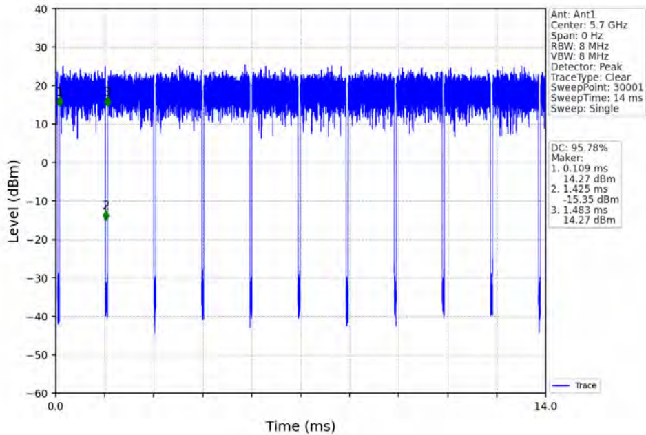
802.11ac(VHT20)_LCH_5745MHz_Ant1_NTNV
