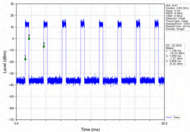
n78d_30kHz_SISO_NTNV_100MHz_CP-OFDM 256 QAM_3649.98MHz_Inner_Full
