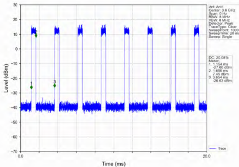
n78d_30kHz_SISO_NTNV_100MHz_CP-OFDM 256 QAM_3600MHz_Inner_Full
