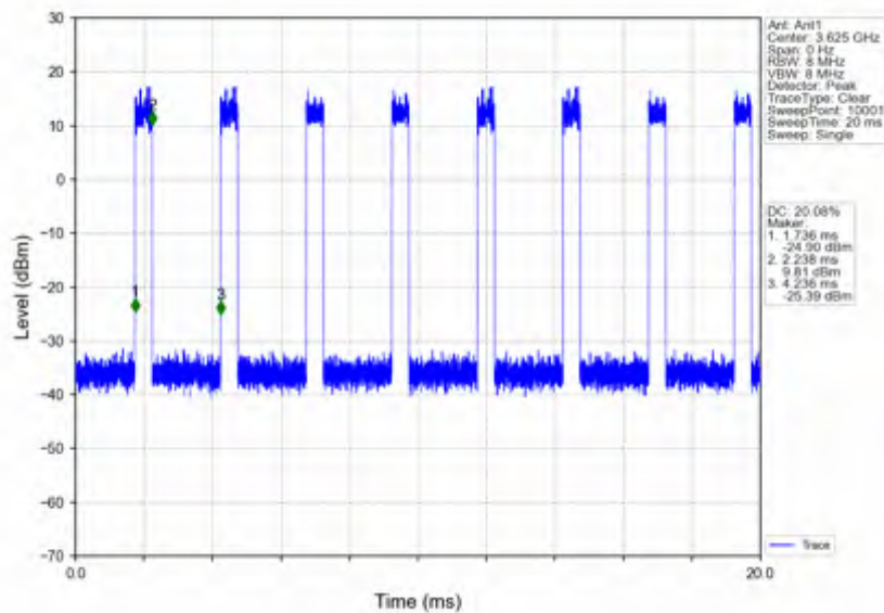
n78d_30kHz_SISO_NTNV_100MHz_CP-OFDM 256 QAM_3624.99MHz_Inner_Full
