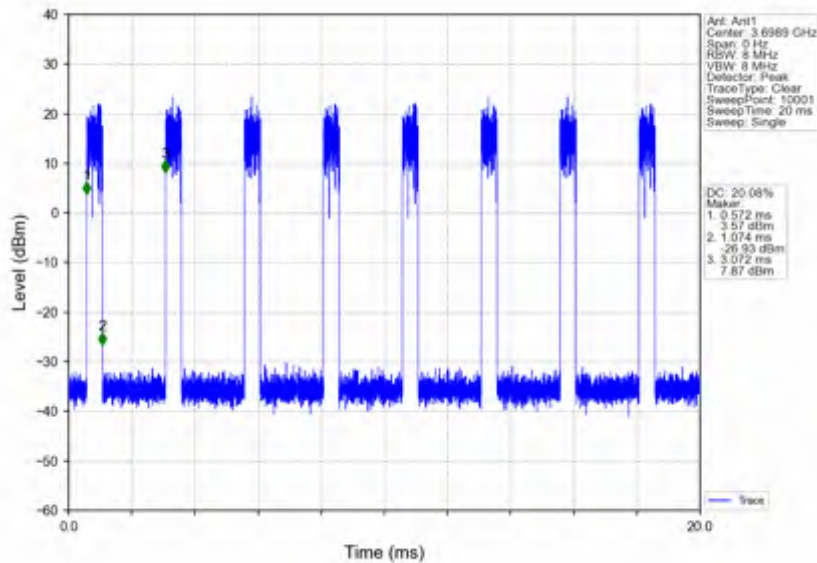
n78d_30kHz_SISO_NTNV_80MHz_CP-OFDM_16 QAM_3660MHz_Edge_1RB_Right
