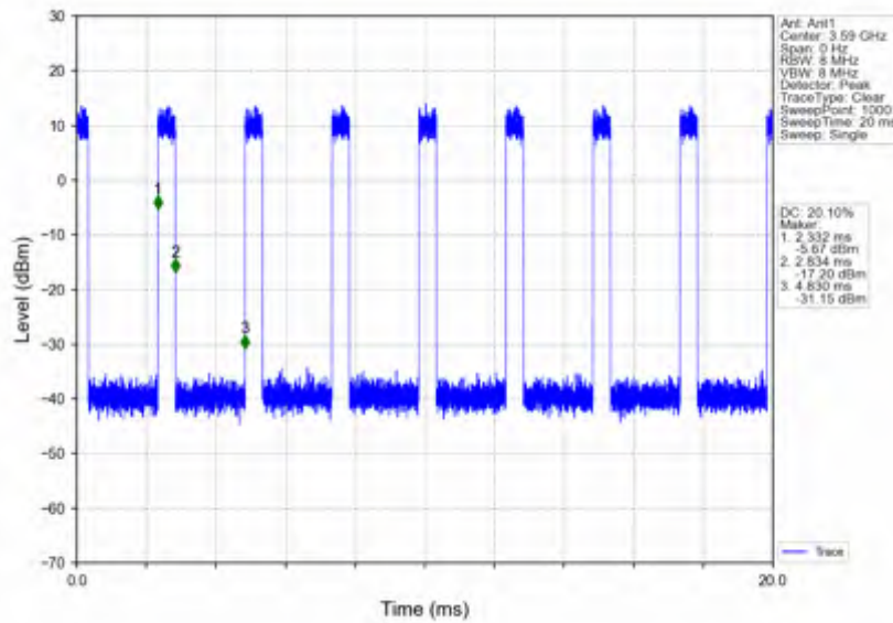
n78d_30kHz_SISO_NTV_80MHz_CP-OFDM 64 QAM_3590.01MHz_Inner_Full
