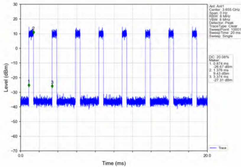
n78d_30kHz_SISO_NTNV_90MHz_CP-OFDM 64 QAM_3654.99MHz_Inner_Full
