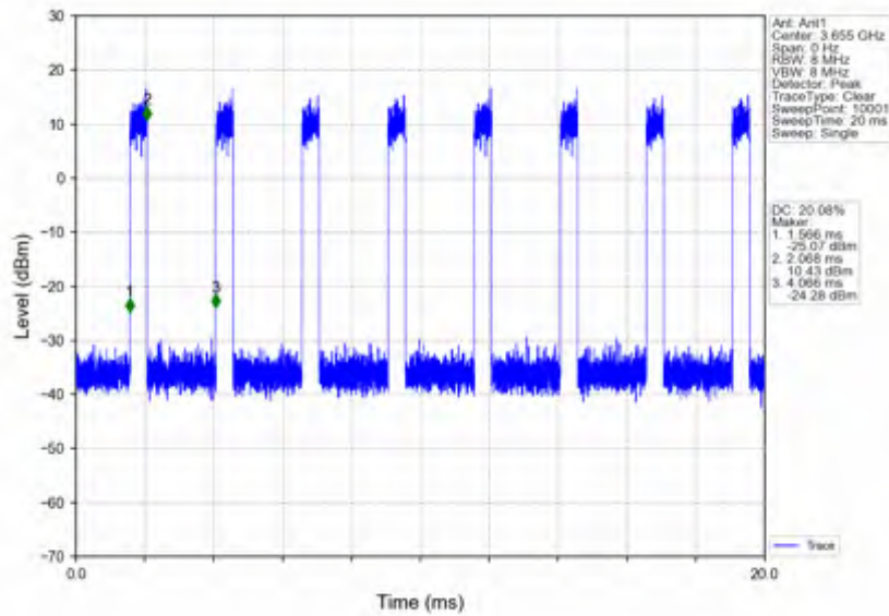
n78d_30kHz_SISO_NTNV_90MHz_CP-OFDM QPSK_3654.99MHz_Inner_Full
