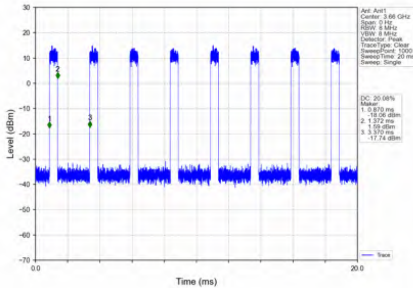
n78d_30kHz_SISO_NTNV_80MHz_CP-OFDM_256_QAM_3660MHz_Inner_Full
