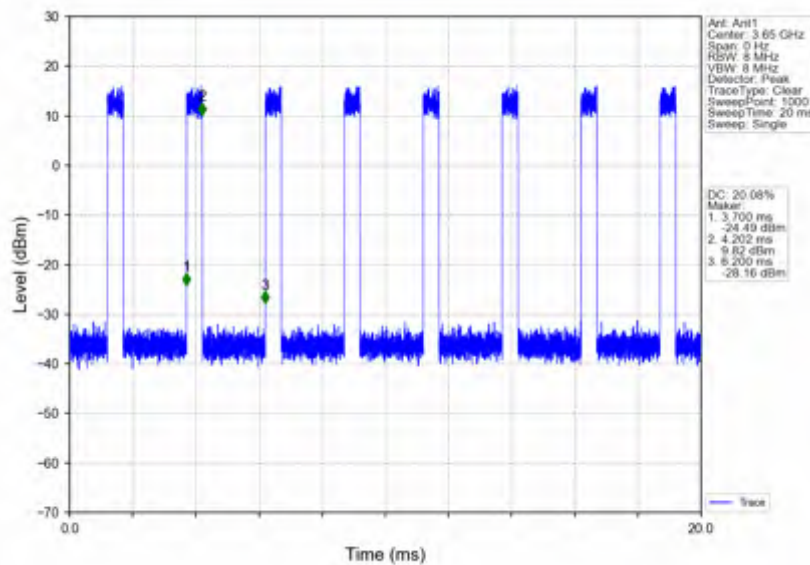
n78d_30kHz_SISO_NTNV_100MHz_CP-OFDM QPSK_3649.98MHz_Inner_Full
