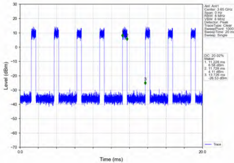
n78d_30kHz_SISO_NTNV_100MHz_CP-OFDM 64 QAM_3649.98MHz_Inner_Full
