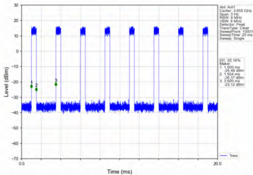
n78d_30kHz_SISO_NTNV_90MHz_CP-OFDM 256 QAM_3654.99MHz_Inner_Full
