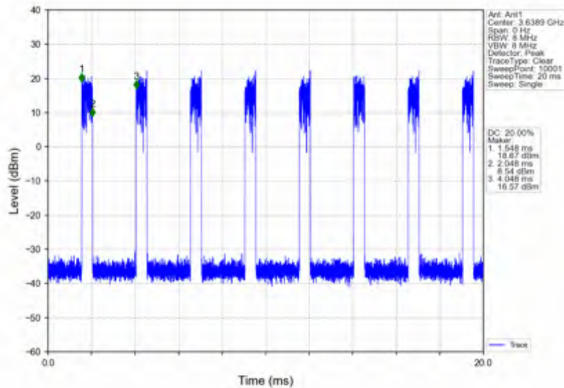
n78d_30kHz_SISO_NTNV_90MHz_CP-OFDM 256 QAM_3595.02MHz_Edge_1RB_Right
