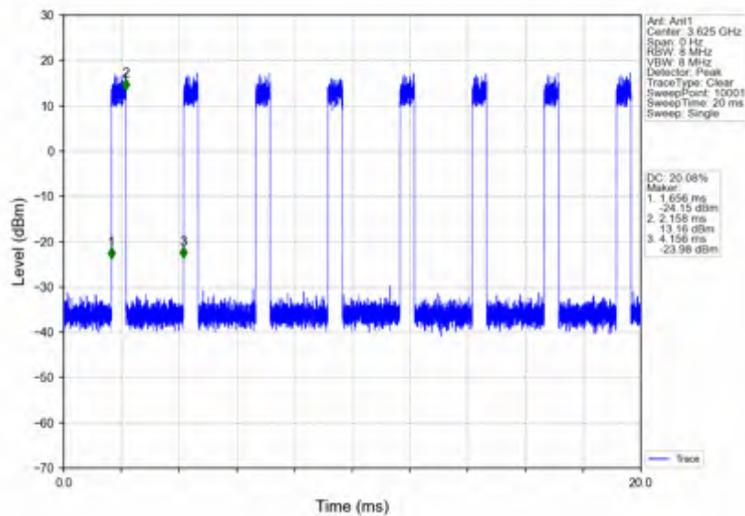
n78d_30kHz_SISO_NTNV_90MHz_CP-OFDM QPSK_3624.99MHz_Inner_Full
