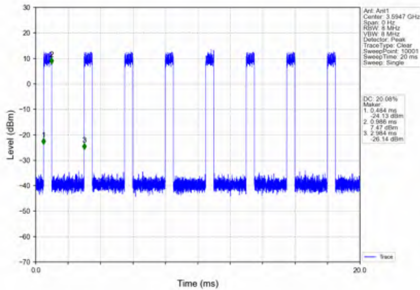
n78d_30kHz_SISO_NTNV_90MHz_DFT-s-OFDM 64 QAM_3595.02MHz_Inner_Full
