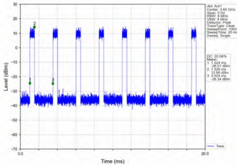
n78d_30kHz_SISO_NTNV_100MHz_CP-OFDM 16 QAM_3649.98MHz_Inner_Full
