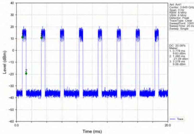
n78d_30kHz_SISO_NTNV_100MHz_DFT-s-OFDM_16_QAM_3600MHz_Edge_1RB_Right
