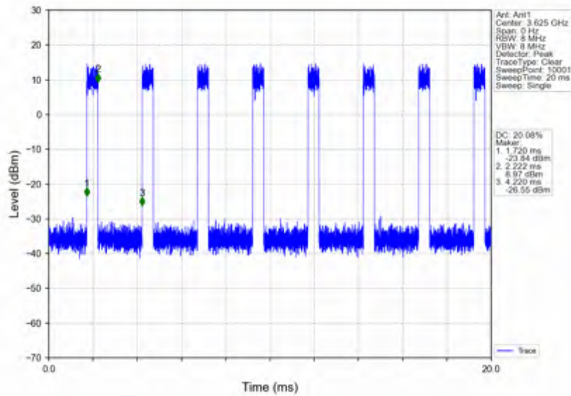
n78d_30kHz_SISO_NTV_90MHz_CP-OFDM 16 QAM_3624.99MHz_Inner_Full
