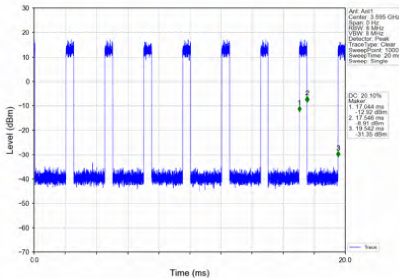
n78d_30kHz_SISO_NTNV_90MHz_CP-OFDM QPSK_3595.02MHz_Inner_Full
