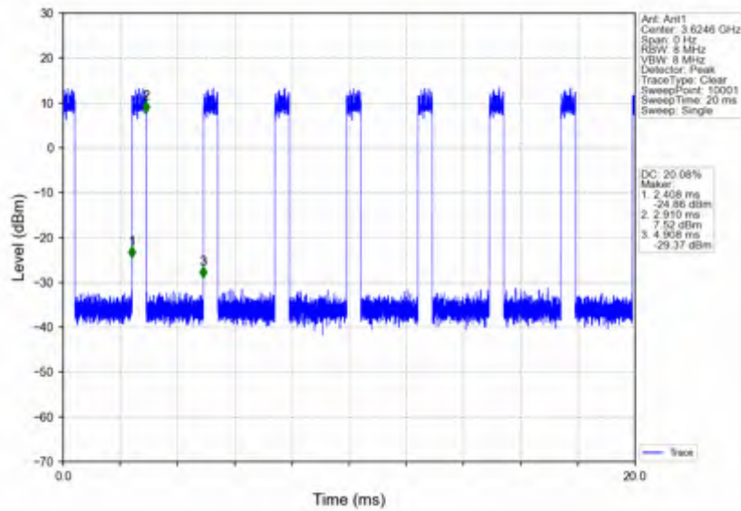
n78d_30kHz_SISO_NTNV_90MHz_DFT-s-OFDM 64 QAM_3624.99MHz_Inner_Full
