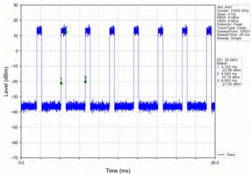
n78d_30kHz_SISO_NTV_90MHz_CP-OFDM 16 QAM_3654.99MHz_Inner_Full
