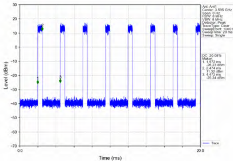
n78d_30kHz_SISO_NTNV_90MHz_CP-OFDM 64 QAM_3595.02MHz_Inner_Full
