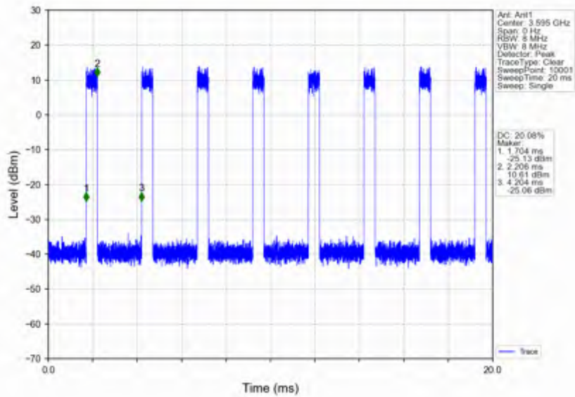
n78d_30kHz_SISO_NTNV_90MHz_CP-OFDM 256 QAM_3595.02MHz_Inner_Full
