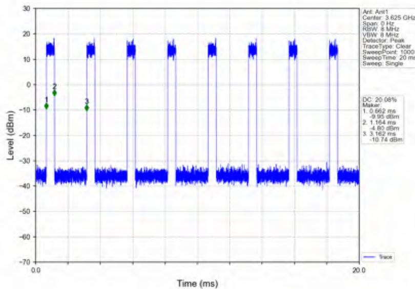
n78d_30kHz_SISO_NTV_80MHz_CP-OFDM 64 QAM_3624.99MHz_Inner_Full
