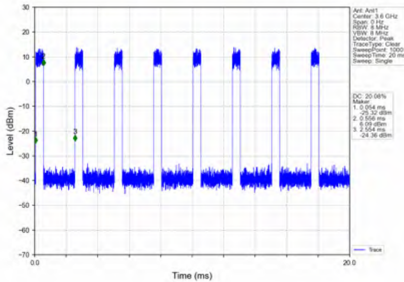
n78d_30kHz_SISO_NTNV_100MHz_CP-OFDM 64 QAM_3600MHz_Inner_Full
