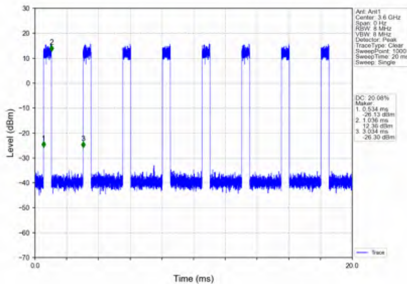
n78d_30kHz_SISO_NTNV_100MHz_CP-OFDM QPSK_3600MHz_Inner_Full
