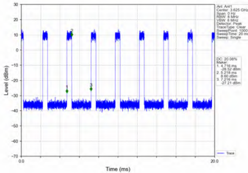
n78d_30kHz_SISO_NTNV_100MHz_CP-OFDM QPSK_3624.99MHz_Inner_Full
