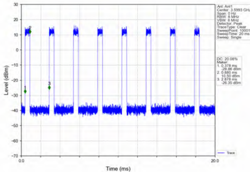
n78d_30kHz_SISO_NTNV_100MHz_DFT-s-OFDM_64_QAM_3600MHz_Inner_Full
