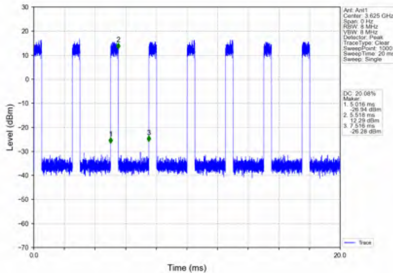
n78d_30kHz_SISO_NTNV_100MHz_CP-OFDM 16 QAM_3624.99MHz_Inner_Full
