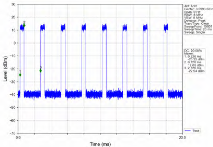
n78d_30kHz_SISO_NTNV_100MHz_DFT-s-OFDM_16_QAM_3600MHz_Inner_Full
