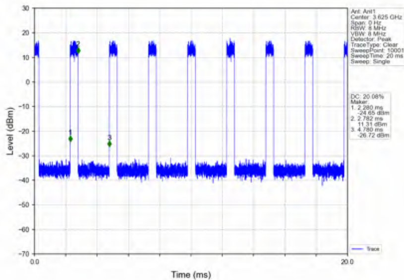
n78d_30kHz_SISO_NTV_90MHz_CP-OFDM 64 QAM_3624.99MHz_Inner_Full
