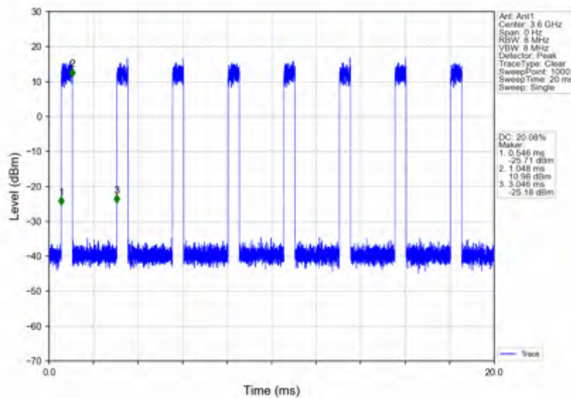
n78d_30kHz_SISO_NTNV_100MHz_CP-OFDM 16 QAM_3600MHz_Inner_Full
