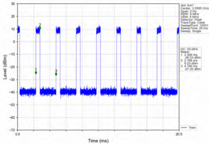
n78d_30kHz_SISO_NTNV_100MHz_DFT-s-OFDM 256 QAM_3600MHz_Inner_Full
