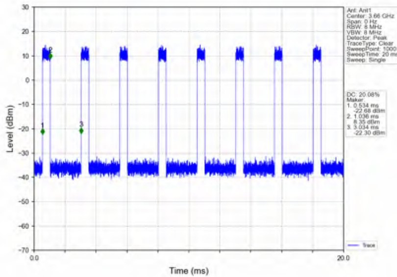
n78d_30kHz_SISO_NTNV_80MHz_CP-OFDM 64 QAM_3660MHz_Inner_Full
