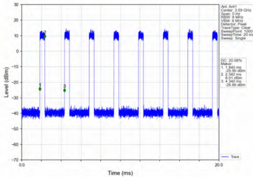
n78d_30kHz_SISO_NTNV_80MHz_CP-OFDM 256 QAM_3590.01MHz_Inner_Full
