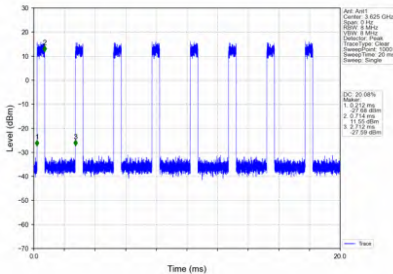
n78d_30kHz_SISO_NTNV_100MHz_CP-OFDM 64 QAM_3624.99MHz_Inner_Full
