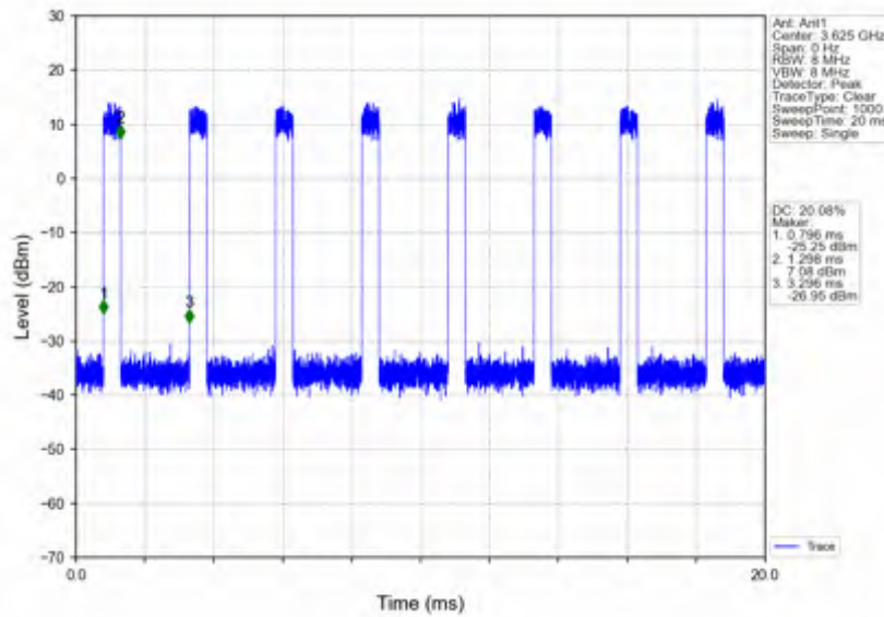
n78d_30kHz_SISO_NTNV_80MHz_CP-OFDM 256 QAM_3624.99MHz_Inner_Full
