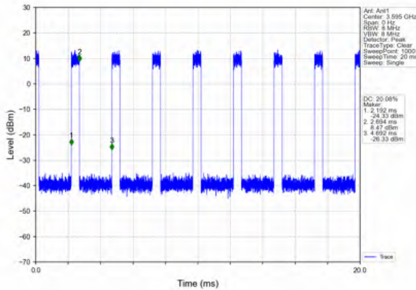
n78d_30kHz_SISO_NTNV_90MHz_CP-OFDM 16 QAM_3595.02MHz_Inner_Full
