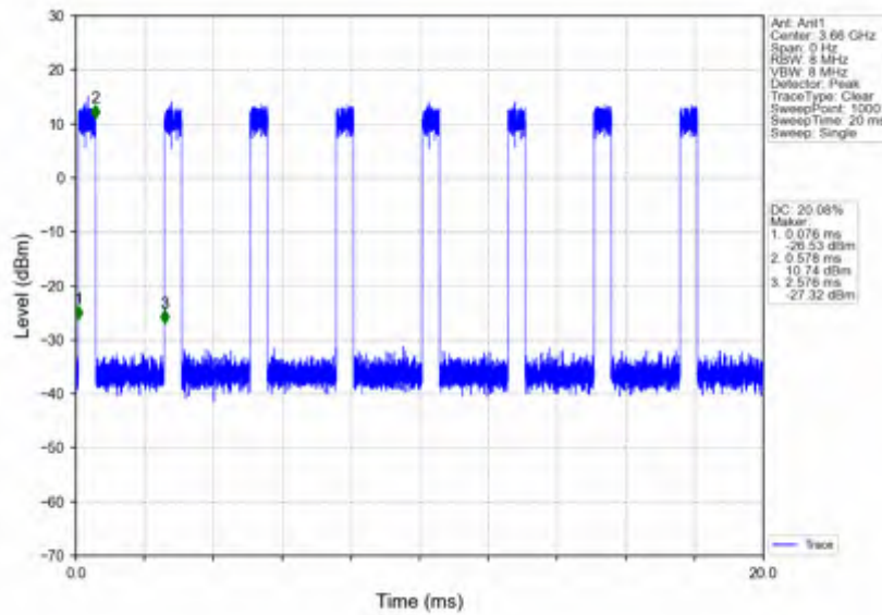
n78d_30kHz_SISO_NTNV_80MHz_CP-OFDM_16 QAM_3660MHz_Inner_Full
