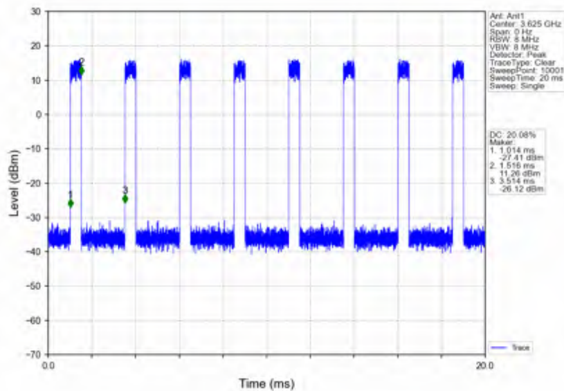
n78d_30kHz_SISO_NTNV_90MHz_CP-OFDM 256 QAM_3624.99MHz_Inner_Full
