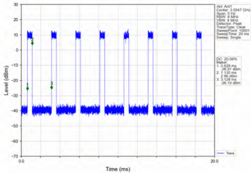
n78d_30kHz_SISO_NTNV_90MHz_DFT-s-OFDM_256_QAM_3595.02MHz_Inner_Full
