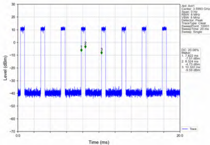
n78d_30kHz_SISO_NTNV_100MHz_DFT-s-OFDM PI/2 BPSK_3600MHz_Inner_Full
