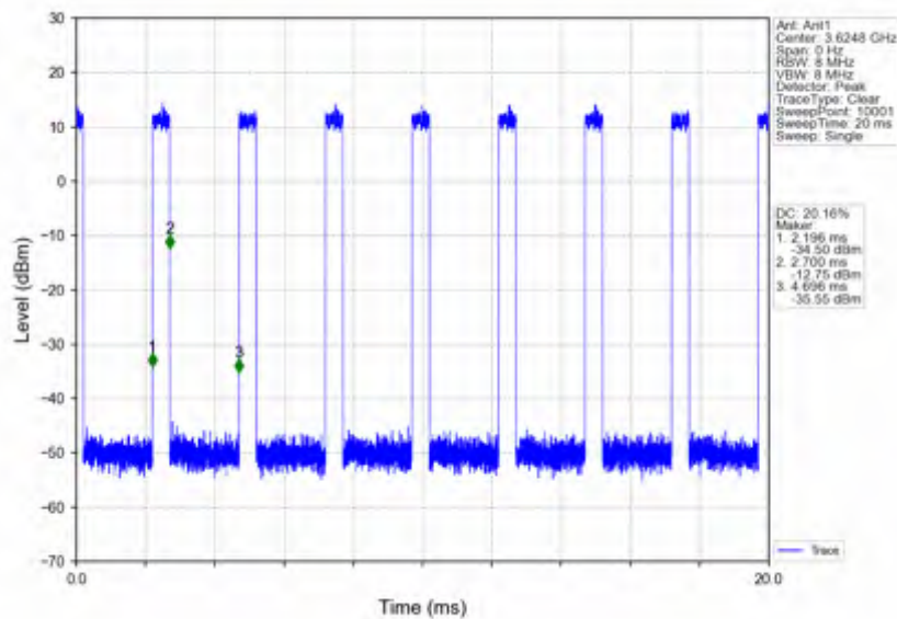
n78d_30kHz_SISO_NTNV_80MHz_DFT-s-OFDM PI/2 BPSK_3624.99MHz_Inner_Full
