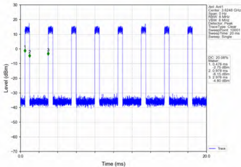
n78d_30kHz_SISO_NTNV_80MHz_DFT-s-OFDM_16 QAM_3624.99MHz_Inner_Full
