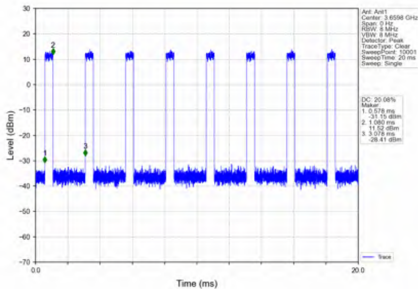
n78d_30kHz_SISO_NTNV_80MHz_DFT-s-OFDM PI/2 BPSK_3660MHz_Inner_Full
