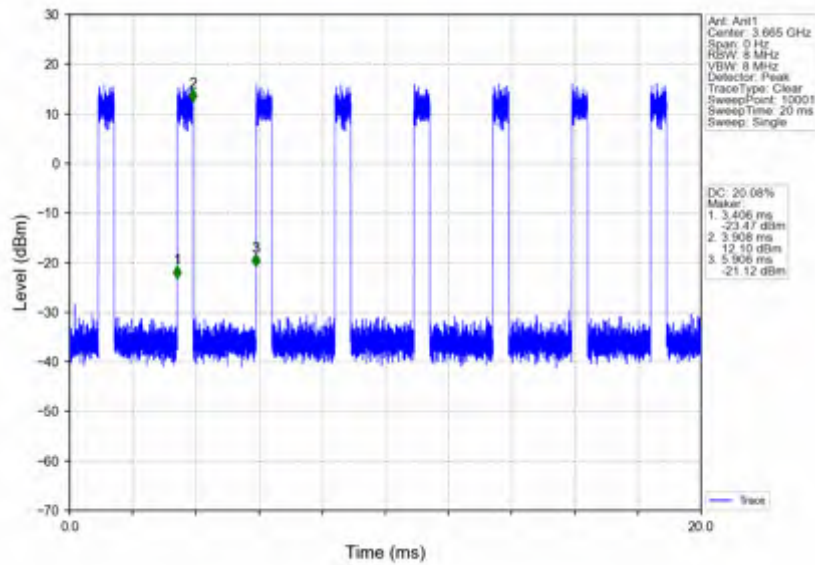
n78d_30kHz_SISO_NTNV_70MHz_CP-OFDM_256_QAM_3664.98MHz_Inner_Full
