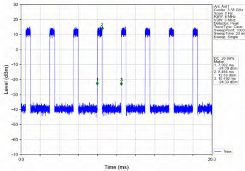
n78d_30kHz_SISO_NTNV_60MHz_CP-OFDM 256 QAM_3580.02MHz_Inner_Full
