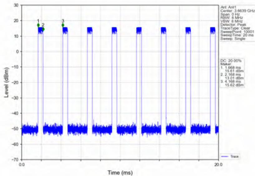
n78d_30kHz_SISO_NTNV_80MHz_DFT-s-OFDM PI/2 BPSK_3624.99MHz_Edge_1RB_Right
