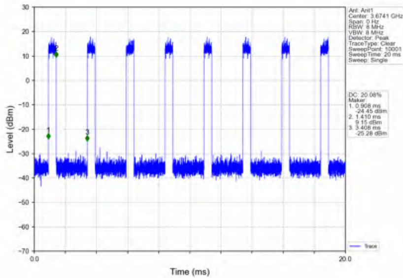
n78d_30kHz_SISO_NTNV_50MHz_DFT-s-OFDM_16_QAM_3675MHz_Inner_Full
