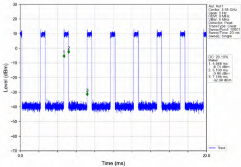
n78d_30kHz_SISO_NTNV_60MHz_DFT-s-OFDM PI/2 BPSK_3580.02MHz_Inner_Full
