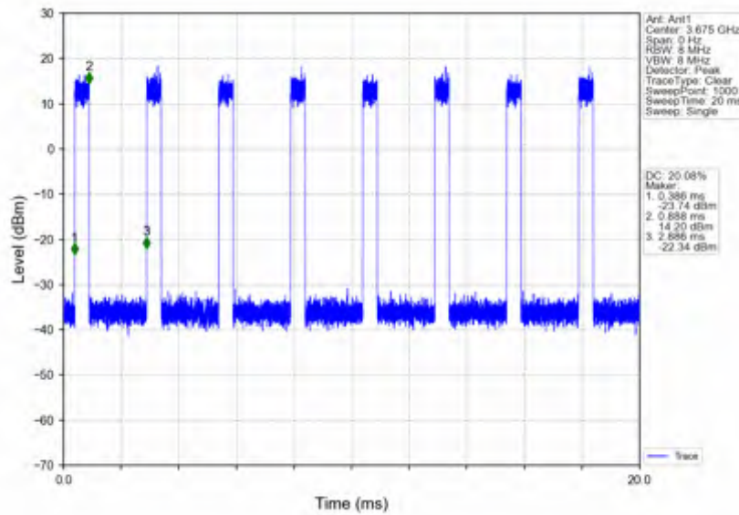
n78d_30kHz_SISO_NTNV_50MHz_CP-OFDM QPSK_3675MHz_Inner_Full
