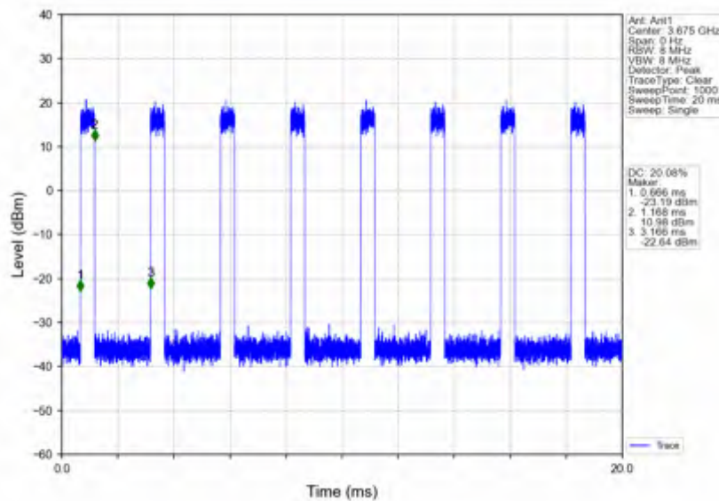
n78d_30kHz_SISO_NTNV_50MHz_CP-OFDM 64 QAM_3675MHz_Inner_Full
