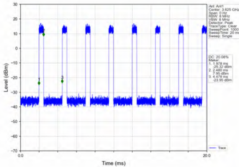
n78d_30kHz_SISO_NTNV_50MHz_CP-OFDM 64 QAM_3624.99MHz_Inner_Full
