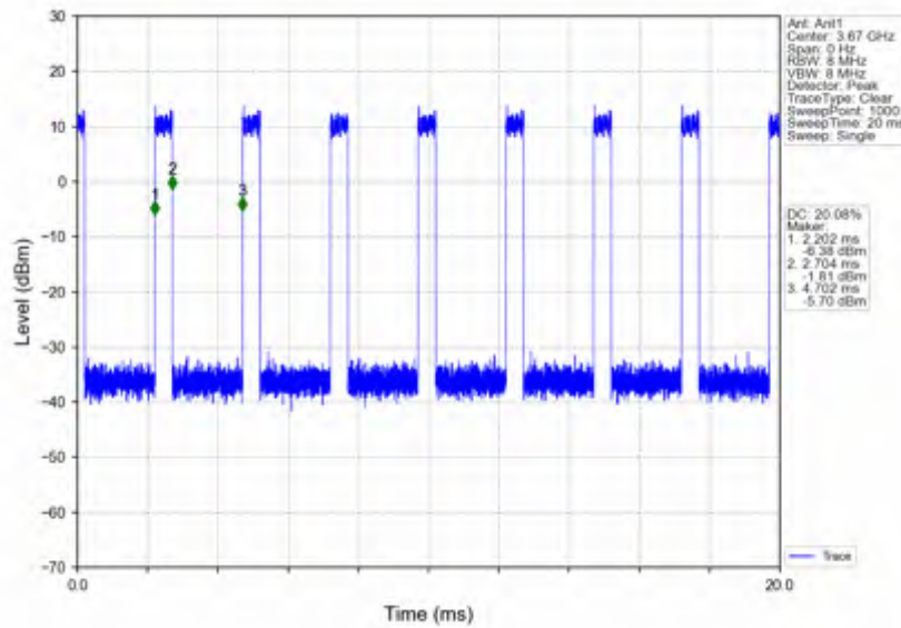
n78d_30kHz_SISO_NTNV_60MHz_DFT-s-OFDM PI/2 BPSK_3669.99MHz_Inner_Full
