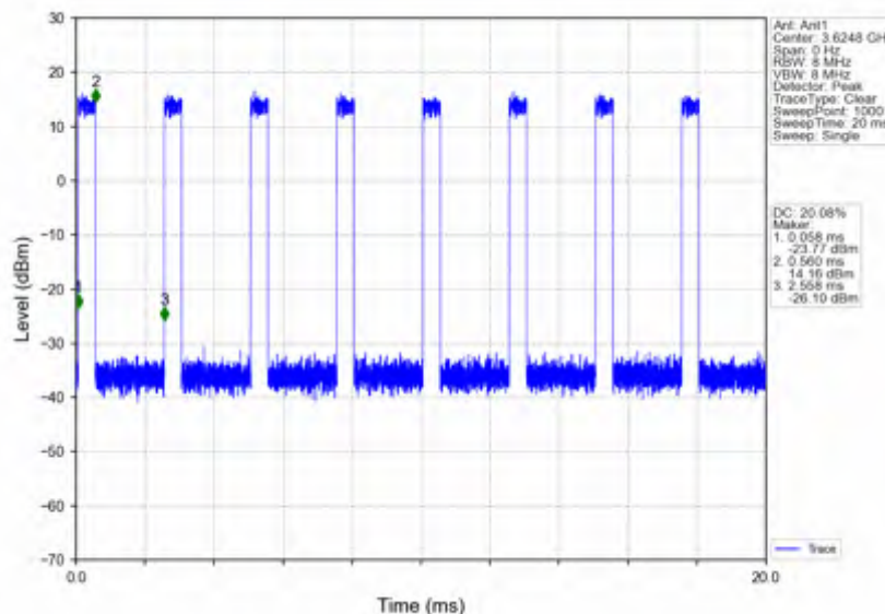
n78d_30kHz_SISO_NTNV_60MHz_DFT-s-OFDM QPSK_3624.99MHz_Inner_Full
