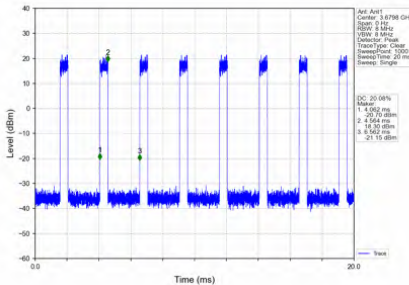
n78d_30kHz_SISO_NTV_40MHz_CP-OFDM 16 QAM_3679.98MHz_Inner_Full
