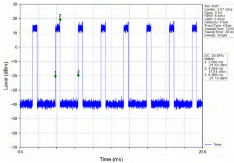
n78d_30kHz_SISO_NTNV_40MHz_CP-OFDM_16 QAM_3570MHz_Inner_Full
