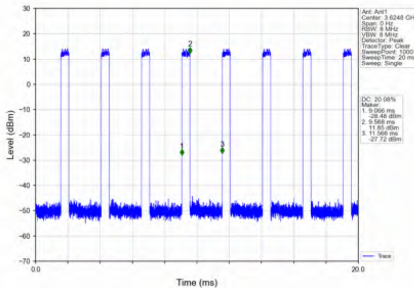
n78d_30kHz_SISO_NTNV_60MHz_DFT-s-OFDM PI/2 BPSK_3624.99MHz_Inner_Full
