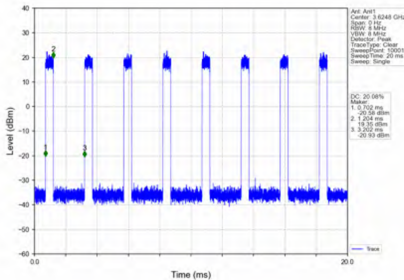
n78d_30kHz_SISO_NTV_30MHz_CP-OFDM 64 QAM_3624.99MHz_Inner_Full
