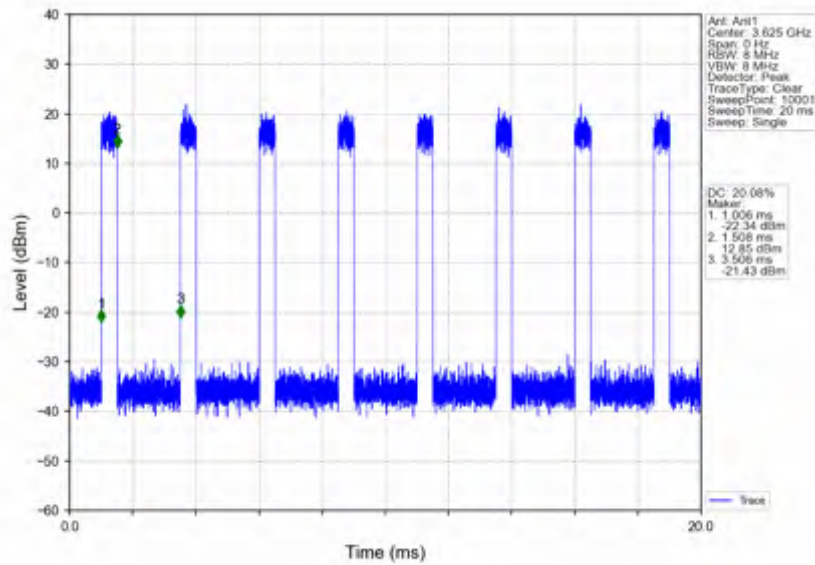
n78d_30kHz_SISO_NTNV_25MHz_CP-OFDM 256 QAM_3624.99MHz_Inner_Full
