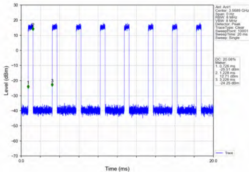
n78d_30kHz_SISO_NTV_40MHz_DFT-s-OFDM 16 QAM_3570MHz_Inner_Full
