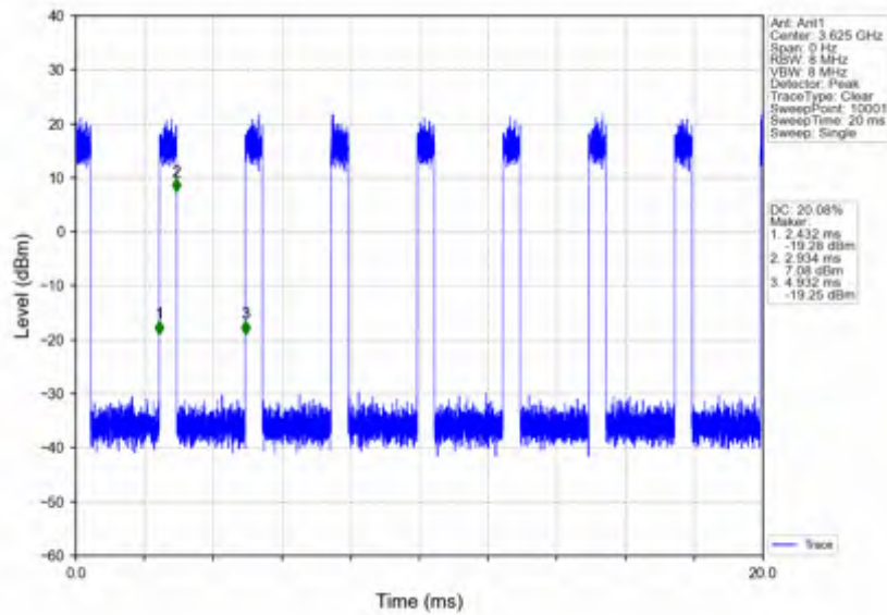
n78d_30kHz_SISO_NTNV_25MHz_CP-OFDM QPSK_3624.99MHz_Inner_Full
