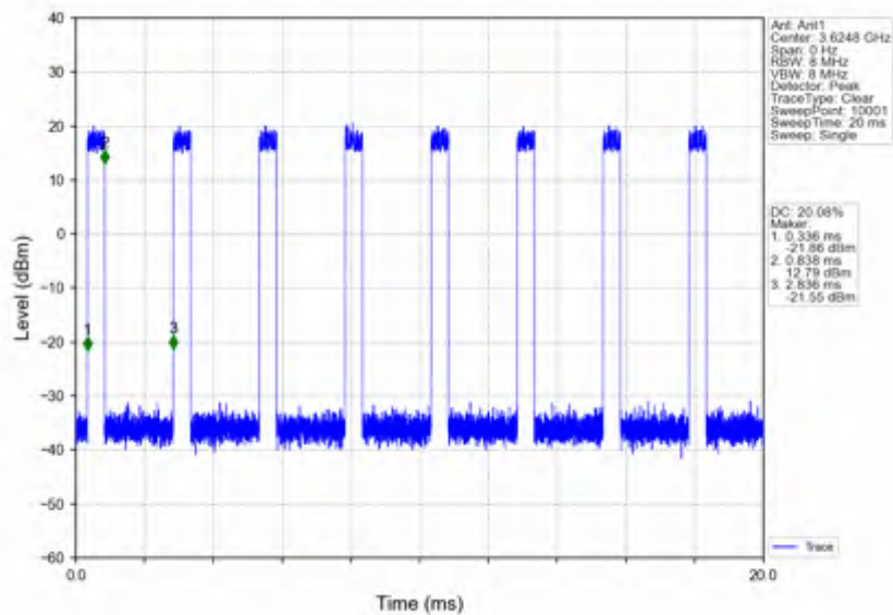
n78d_30kHz_SISO_NTNV_25MHz_DFT-s-OFDM_256_QAM_3624.99MHz_Inner_Full
