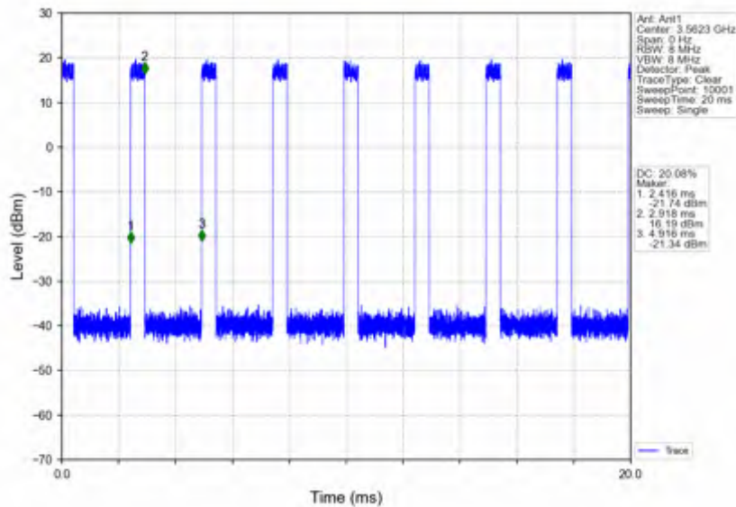
n78d_30kHz_SISO_NTNV_25MHz_DFT-s-OFDM_256_QAM_3562.5MHz_Inner_Full
