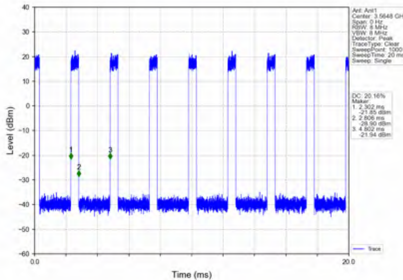
n78d_30kHz_SISO_NTNV_30MHz_CP-OFDM QPSK_3565.02MHz_Inner_Full
