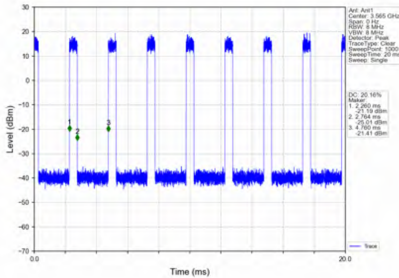
n78d_30kHz_SISO_NTNV_30MHz_CP-OFDM 256 QAM_3565.02MHz_Inner_Full
