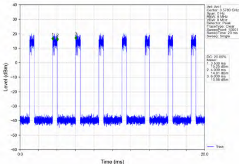
n78d_30kHz_SISO_NTNV_30MHz_DFT-s-OFDM 64 QAM_3565.02MHz_Edge_1RB_Right
