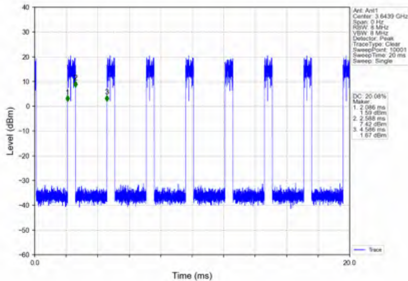
n78d_30kHz_SISO_NTNV_40MHz_DFT-s-OFDM 64 QAM_3624.99MHz_Edge_1RB_Right
