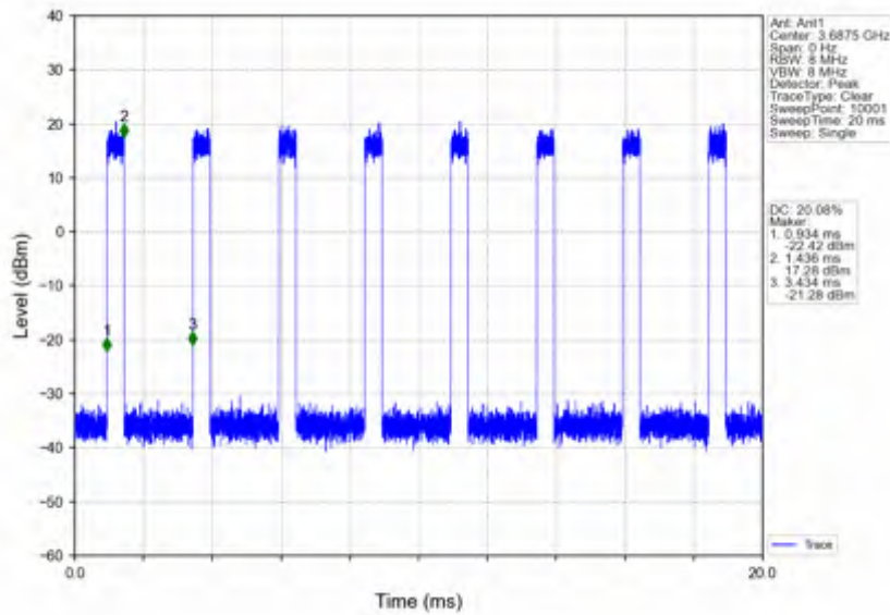
n78d_30kHz_SISO_NTV_25MHz_CP-OFDM 64 QAM_3687.48MHz_Inner_Full
