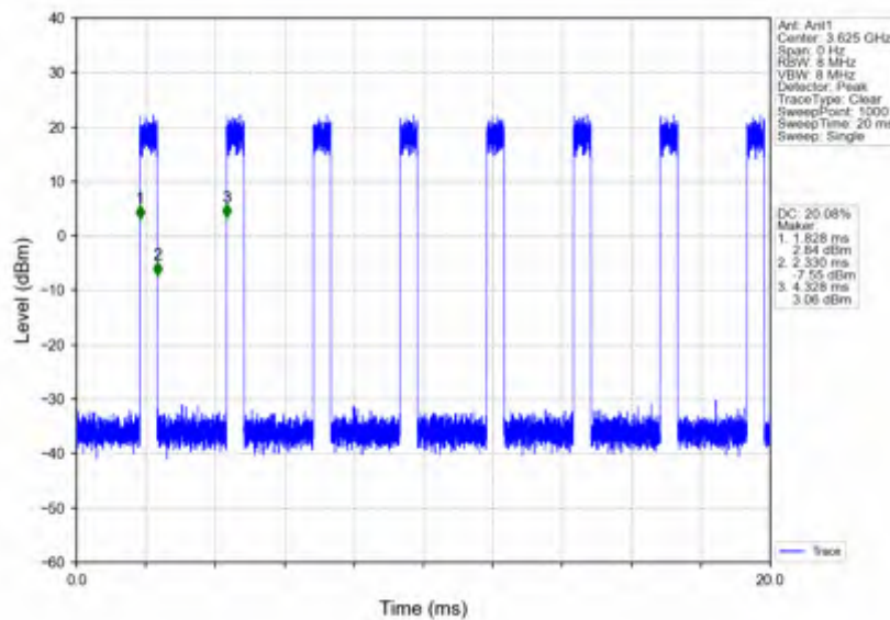
n78d_30kHz_SISO_NTV_25MHz_CP-OFDM 64 QAM_3624.99MHz_Inner_Full
