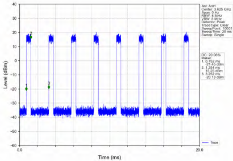
n78d_30kHz_SISO_NTNV_25MHz_CP-OFDM 16 QAM_3624.99MHz_Inner_Full
