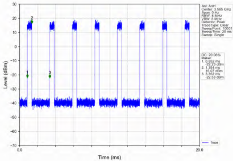
n78d_30kHz_SISO_NTV_30MHz_CP-OFDM 16 QAM_3565.02MHz_Inner_Full
