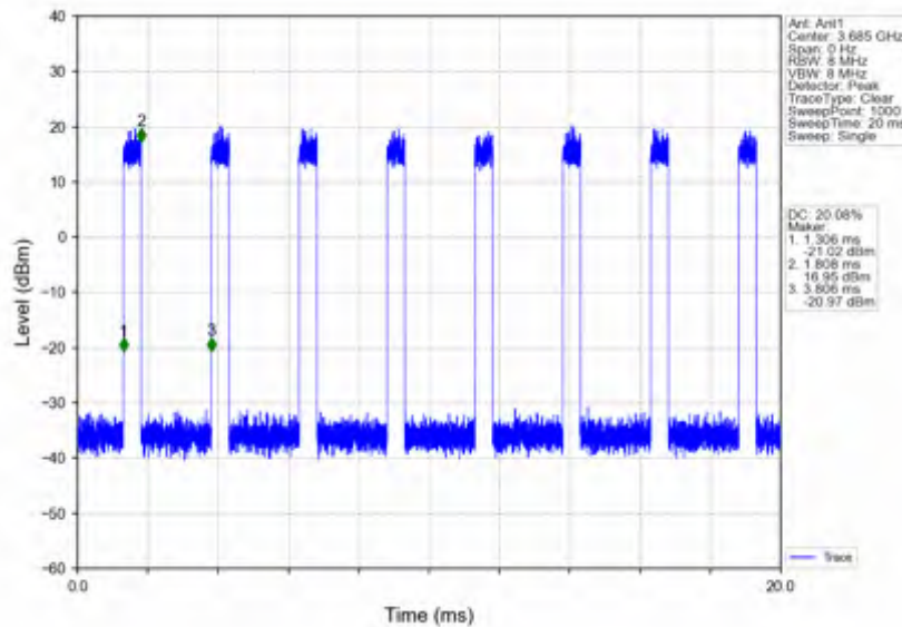
n78d_30kHz_SISO_NTV_30MHz_CP-OFDM 16 QAM_3684.99MHz_Inner_Full
