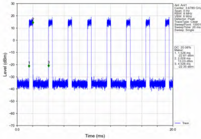
n78d_30kHz_SISO_NTNV_40MHz_DFT-s-OFDM 64 QAM_3679.98MHz_Inner_Full
