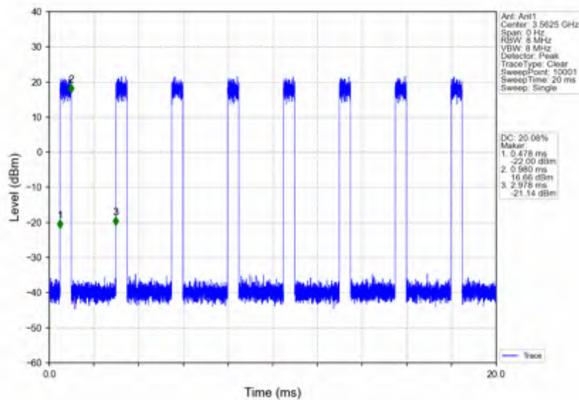
n78d_30kHz_SISO_NTV_25MHz_CP-OFDM 256 QAM_3562.5MHz_Inner_Full
