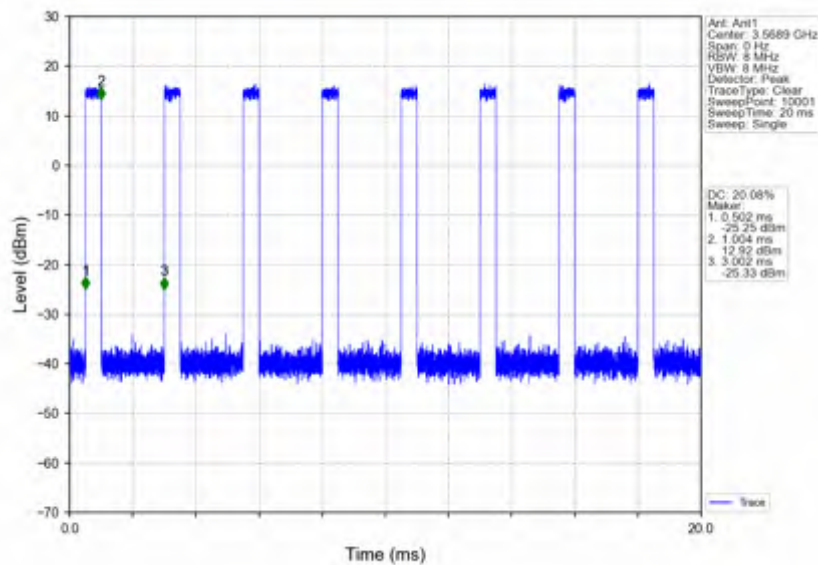
n78d_30kHz_SISO_NTNV_40MHz_DFT-s-OFDM QPSK_3570MHz_Inner_Full
