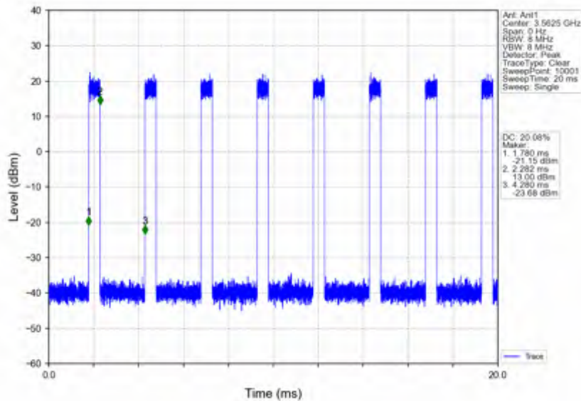
n78d_30kHz_SISO_NTNV_25MHz_CP-OFDM 64 QAM_3562.5MHz_Inner_Full
