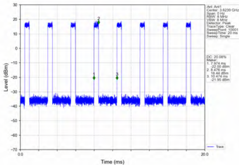
n78d_30kHz_SISO_NTNV_40MHz_DFT-s-OFDM_256_QAM_3624.99MHz_Inner_Full
