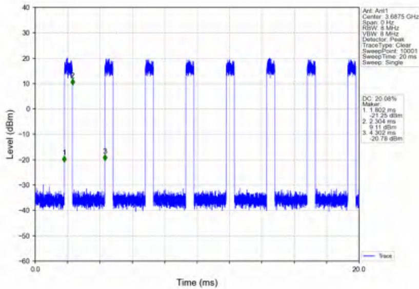
n78d_30kHz_SISO_NTNV_25MHz_CP-OFDM 256 QAM_3687.48MHz_Inner_Full
