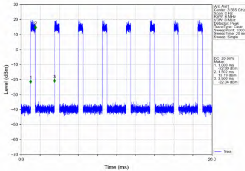
n78d_30kHz_SISO_NTV_30MHz_CP-OFDM 64 QAM_3565.02MHz_Inner_Full
