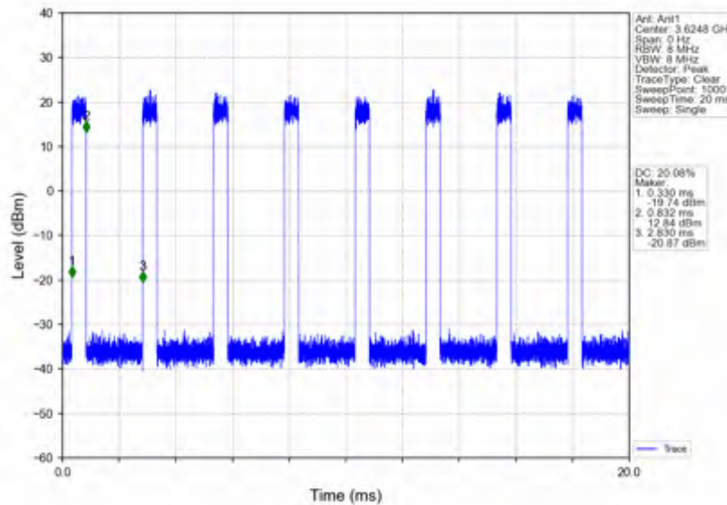
n78d_30kHz_SISO_NTNV_30MHz_CP-OFDM 256 QAM_3624.99MHz_Inner_Full
