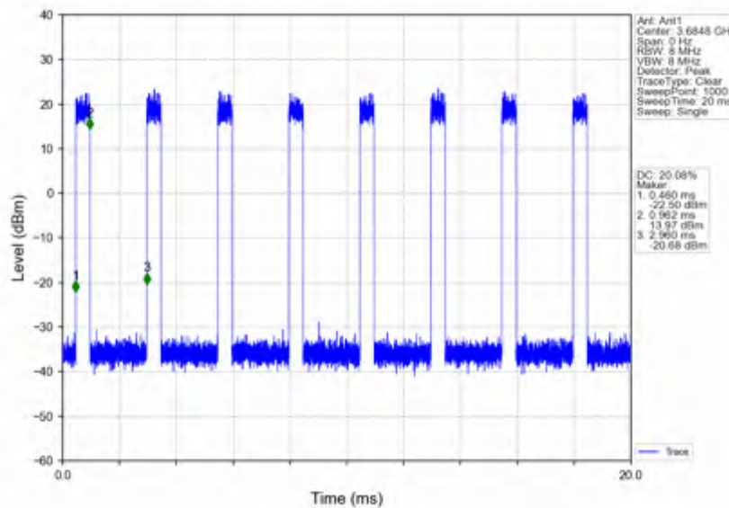
n78d_30kHz_SISO_NTNV_30MHz_CP-OFDM 256 QAM_3684.99MHz_Inner_Full
