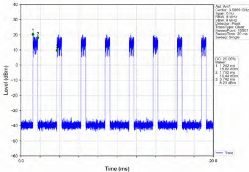
n78d_30kHz_SISO_NTNV_40MHz_DFT-s-OFDM 256 QAM_3570MHz_Edge_1RB_Right
