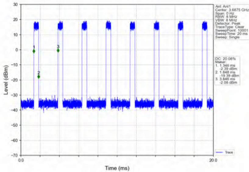
n78d_30kHz_SISO_NTV_25MHz_CP-OFDM 16 QAM_3687.48MHz_Inner_Full
