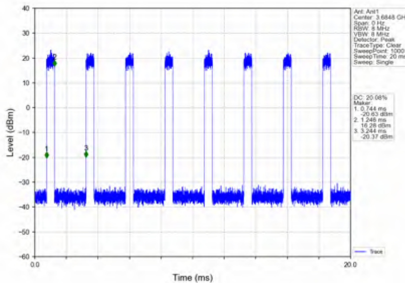
n78d_30kHz_SISO_NTV_30MHz_CP-OFDM 64 QAM_3684.99MHz_Inner_Full
