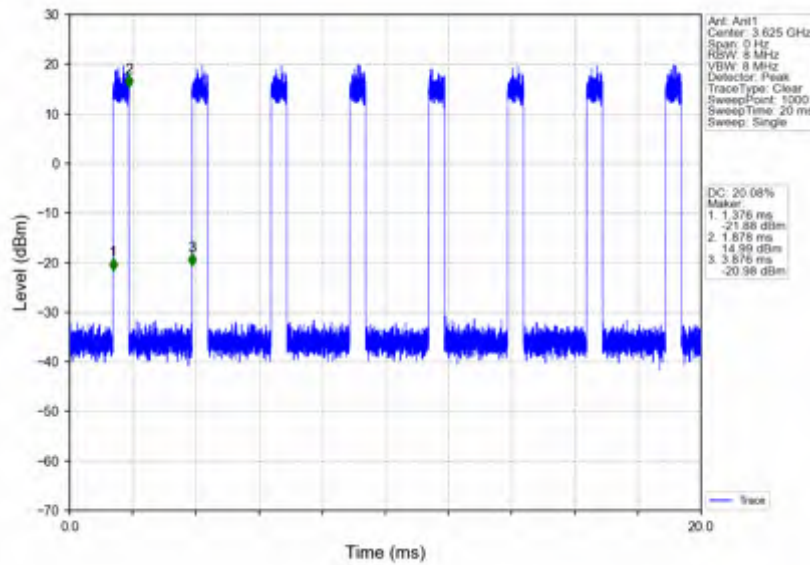
n78d_30kHz_SISO_NTV_30MHz_CP-OFDM 16 QAM_3624.99MHz_Inner_Full
