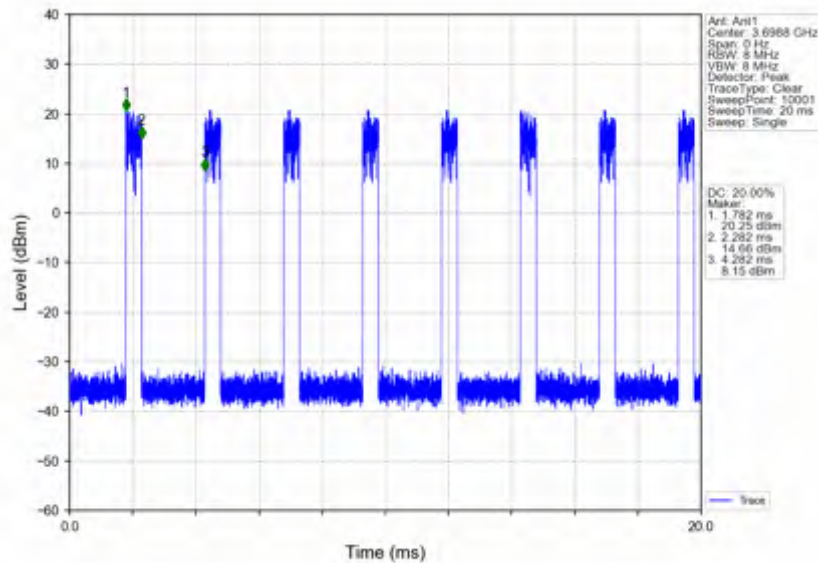
n78d_30kHz_SISO_NTNV_30MHz_DFT-s-OFDM 256 QAM_3684.99MHz_Edge_1RB_Right
