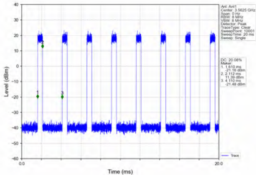
n78d_30kHz_SISO_NTNV_25MHz_CP-OFDM 16 QAM_3562.5MHz_Inner_Full
