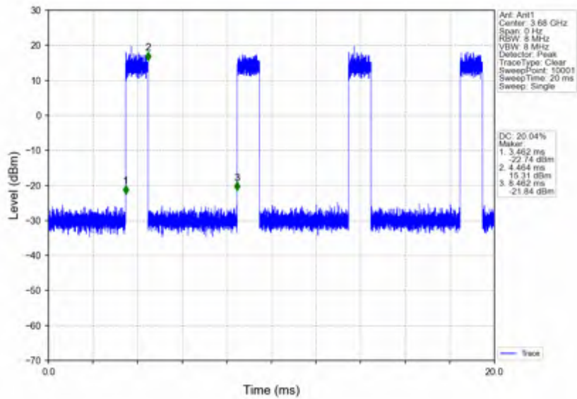
n78d_15kHz_SISO_NTNV_40MHz_CP-OFDM 256 QAM_3679.995MHz_Inner_Full
