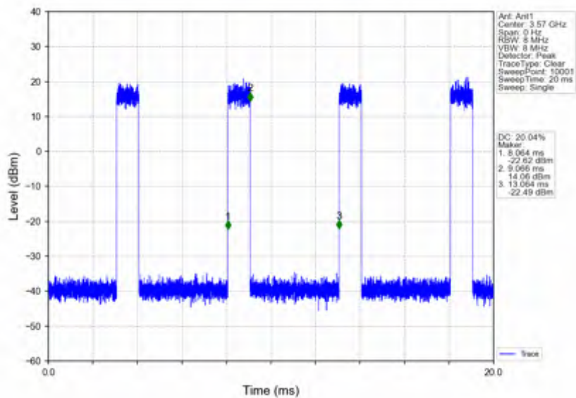
n78d_15kHz_SISO_NTNV_40MHz_CP-OFDM QPSK_3570MHz_Inner_Full
