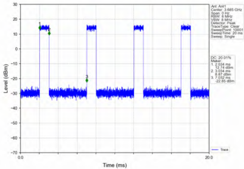
n78d_15kHz_SISO_NTNV_30MHz_DFT-s-OFDM QPSK_3684.99MHz_Inner_Full
