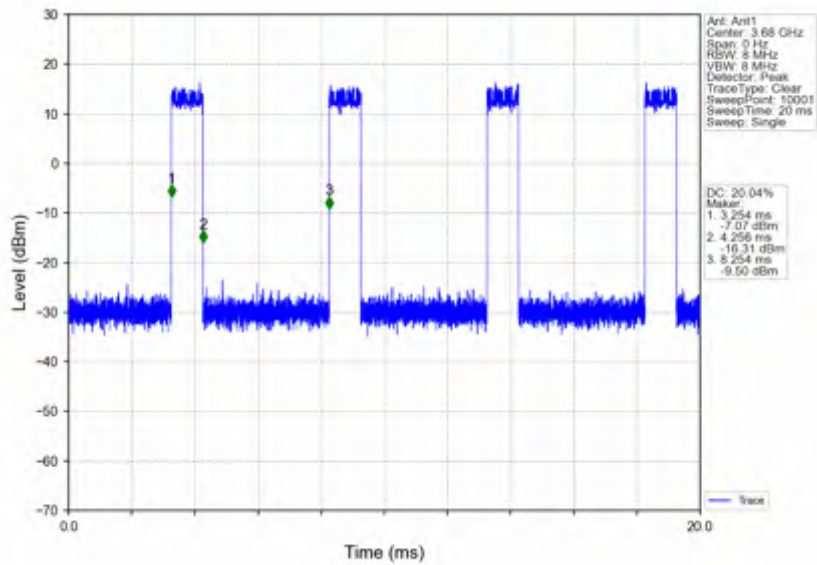
n78d_15kHz_SISO_NTNV_40MHz_DFT-s-OFDM QPSK_3679.995MHz_Inner_Full
