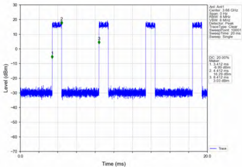
n78d_15kHz_SISO_NTNV_40MHz_DFT-s-OFDM_16 QAM_3679.995MHz_Inner_Full
