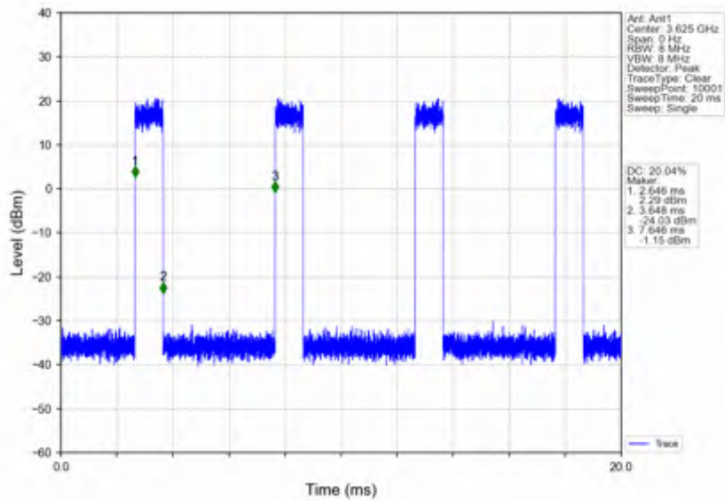
n78d_15kHz_SISO_NTNV_40MHz_CP-OFDM 16 QAM_3625.005MHz_Inner_Full
