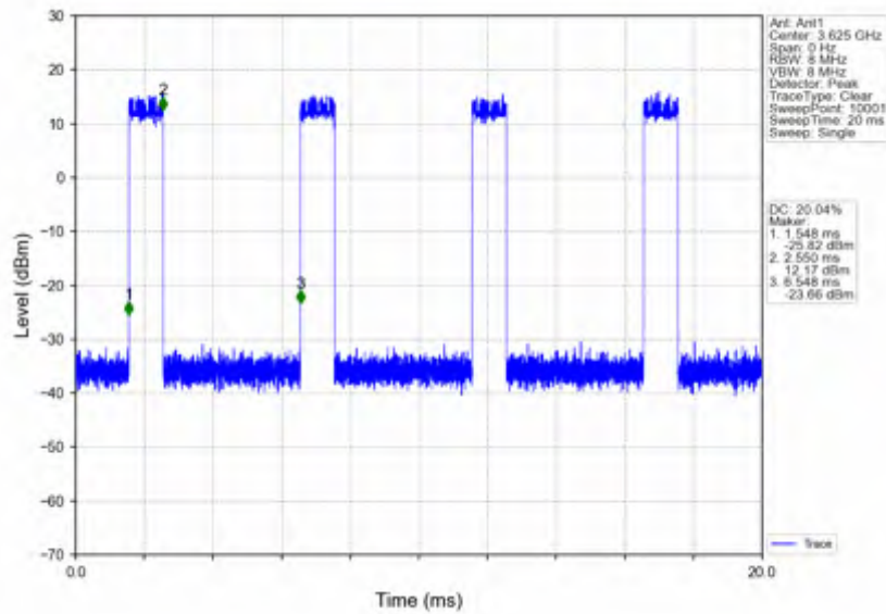
n78d_15kHz_SISO_NTNV_40MHz_DFT-s-OFDM QPSK_3625.005MHz_Inner_Full
