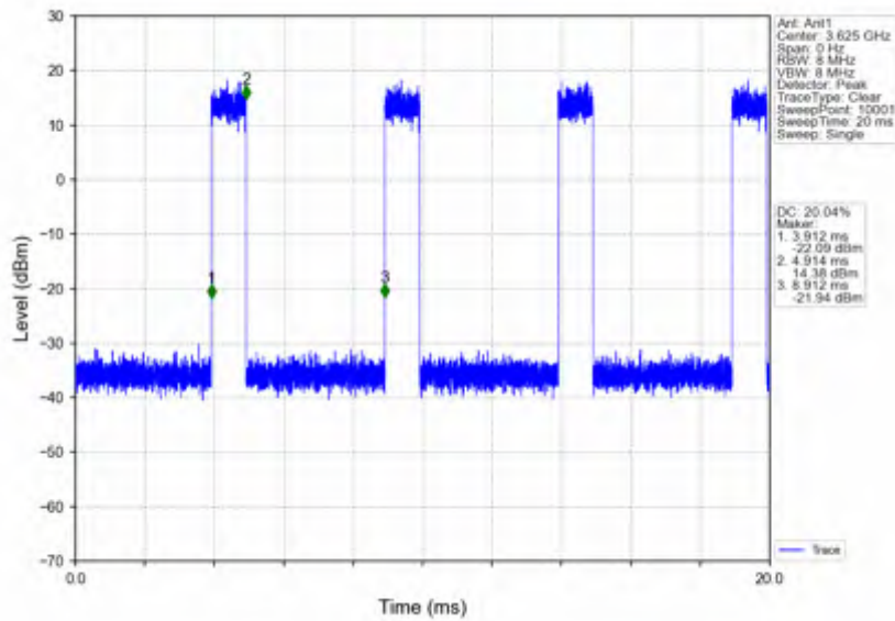
n78d_15kHz_SISO_NTNV_40MHz_CP-OFDM 64 QAM_3625.005MHz_Inner_Full
