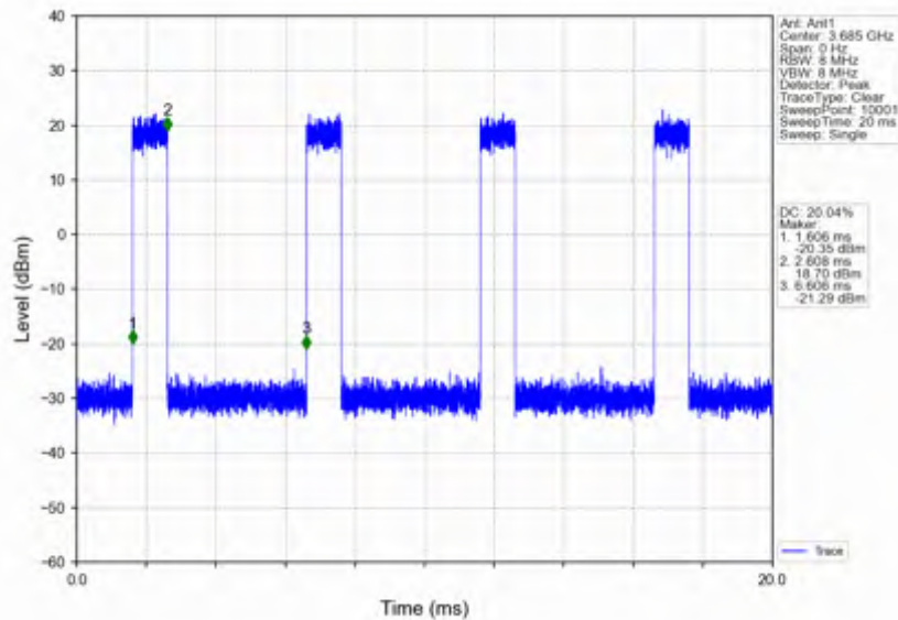
n78d_15kHz_SISO_NTNV_30MHz_CP-OFDM_QPSK_3684.99MHz_Inner_Full
