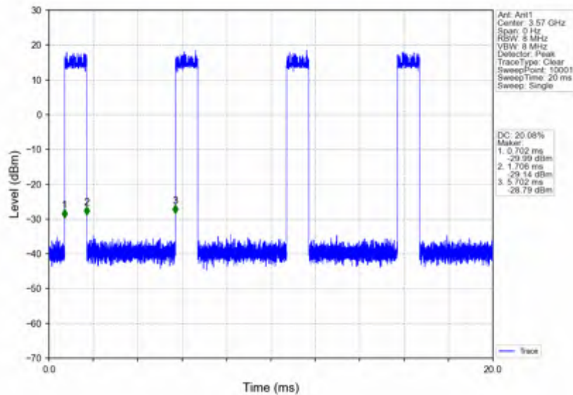
n78d_15kHz_SISO_NTNV_40MHz_DFT-s-OFDM_256_QAM_3570MHz_Inner_Full
