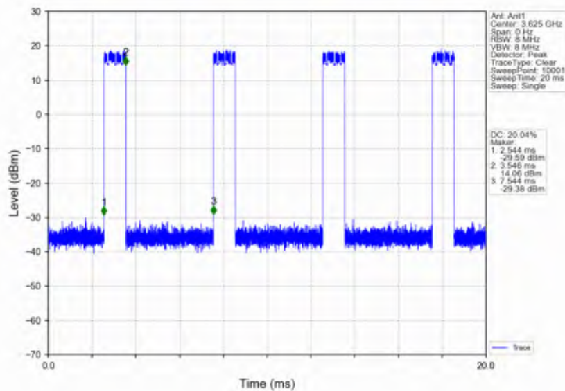
n78d_15kHz_SISO_NTNV_30MHz_DFT-s-OFDM_16_QAM_3625.005MHz_Inner_Full
