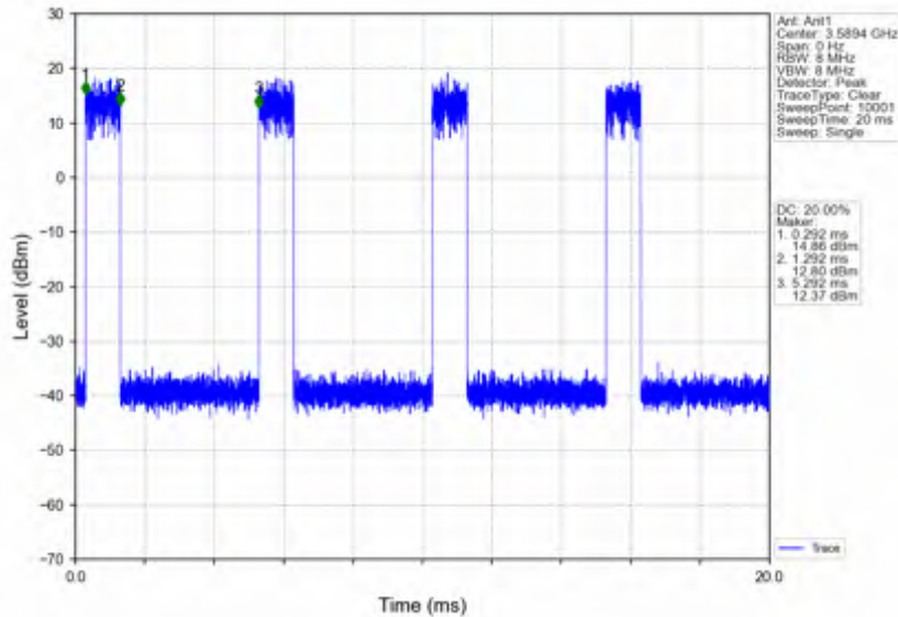
n78d_15kHz_SISO_NTVV_40MHz_DFT-s-OFDM QPSK_3570MHz_Edge_1RB_Right
