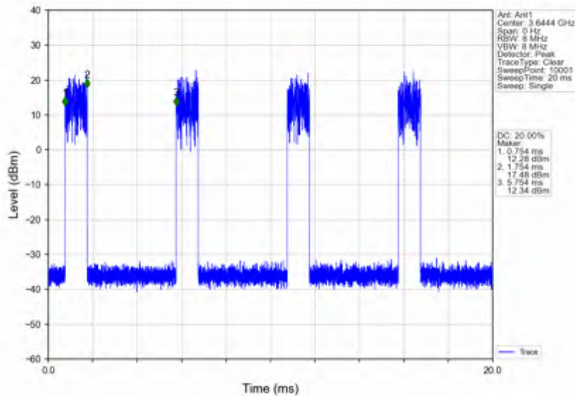
n78d_15kHz_SISO_NTNV_40MHz_CP-OFDM 64 QAM_3625.005MHz_Edge_1RB_Right
