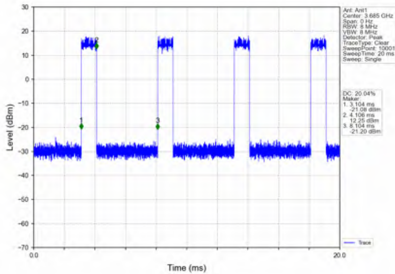
n78d_15kHz_SISO_NTNV_30MHz_DFT-s-OFDM_16 QAM_3684.99MHz_Inner_Full
