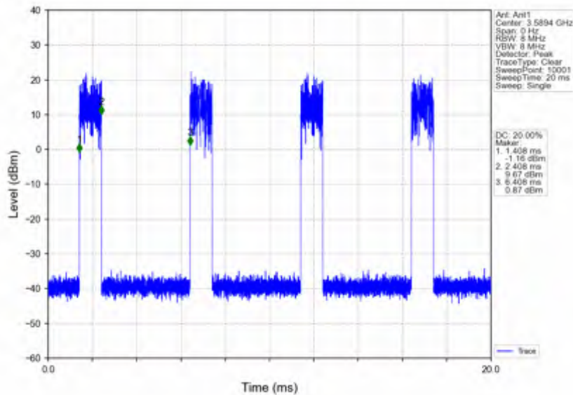
n78d_15kHz_SISO_NTNV_40MHz_CP-OFDM 256 QAM_3570MHz_Edge_1RB_Right
