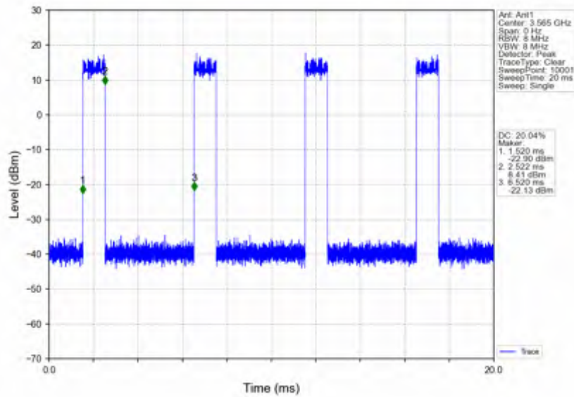
n78d_15kHz_SISO_NTNV_30MHz_DFT-s-OFDM 64 QAM_3565.005MHz_Inner_Full
