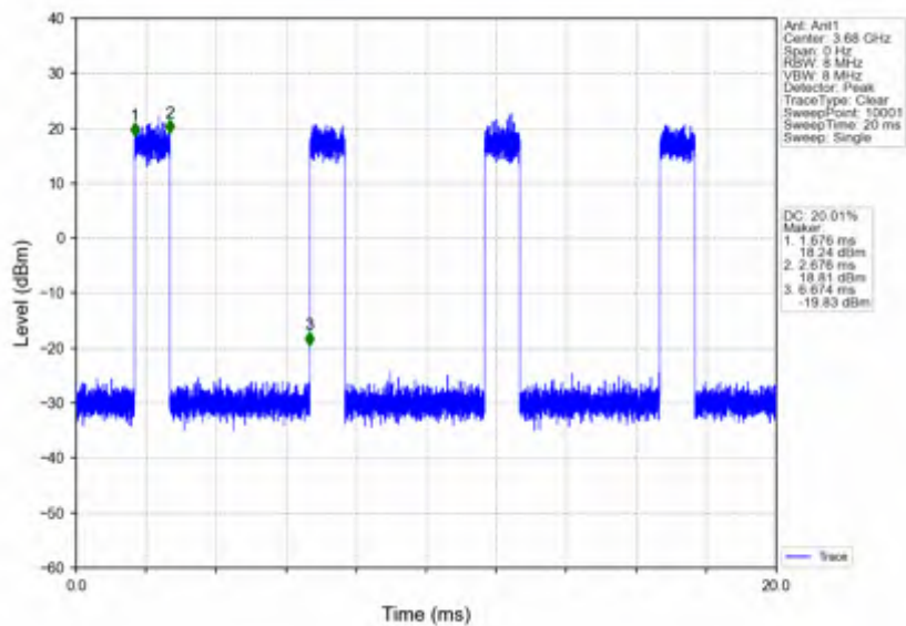
n78d_15kHz_SISO_NTNV_40MHz_CP-OFDM QPSK_3679.995MHz_Inner_Full
