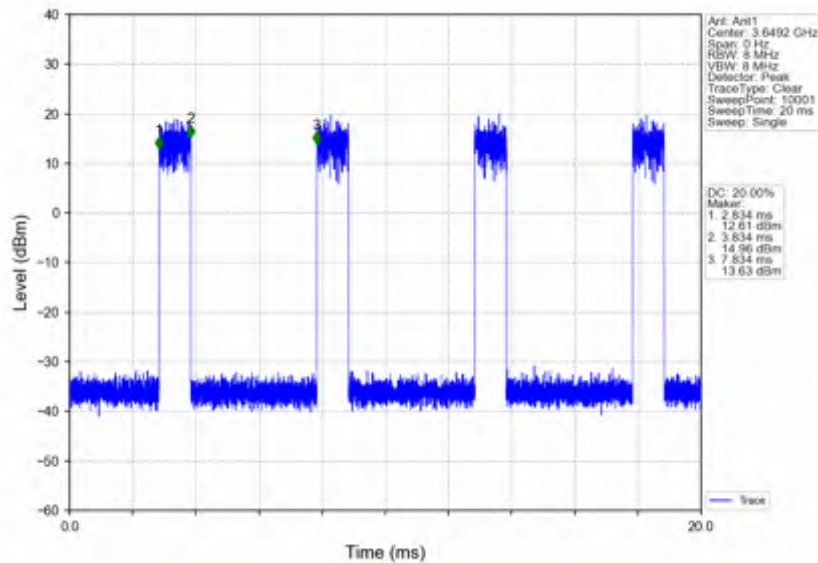
n78d_15kHz_SISO_NTNV_50MHz_DFT-s-OFDM QPSK_3625.005MHz_Edge_1RB_Right
