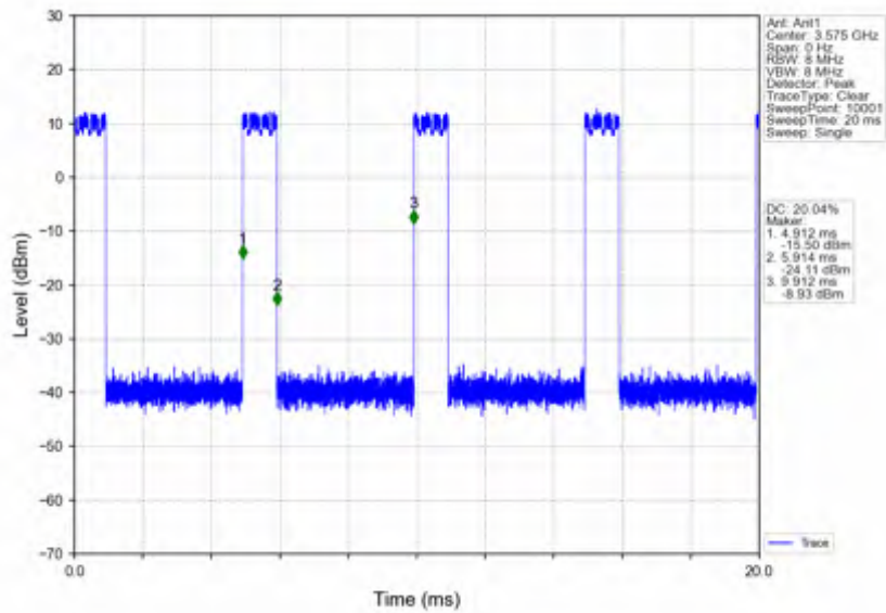
n78d_15kHz_SISO_NTNV_50MHz_DFT-s-OFDM PI/2 BPSK_3575.01MHz_Inner_Full
