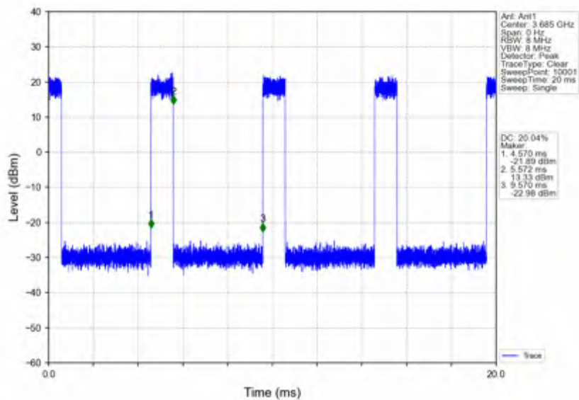
n78d_15kHz_SISO_NTV_30MHz_CP-OFDM 64 QAM_3684.99MHz_Inner_Full
