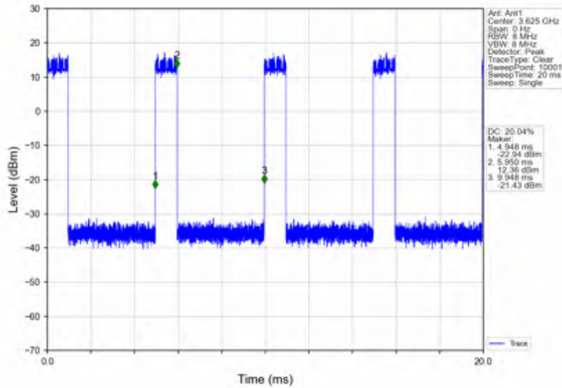
n78d_15kHz_SISO_NTNV_40MHz_DFT-s-OFDM 256 QAM_3625.005MHz_Inner_Full
