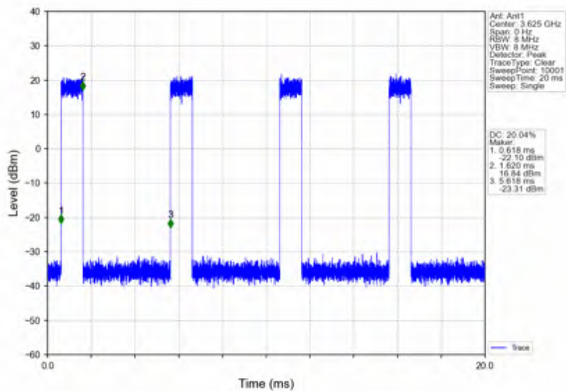
n78d_15kHz_SISO_NTNV_30MHz_CP-OFDM 16 QAM_3625.005MHz_Inner_Full
