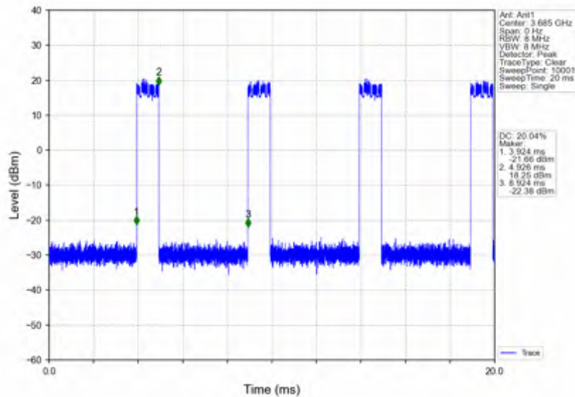
n78d_15kHz_SISO_NTNV_30MHz_DFT-s-OFDM_256_QAM_3684.99MHz_Inner_Full
