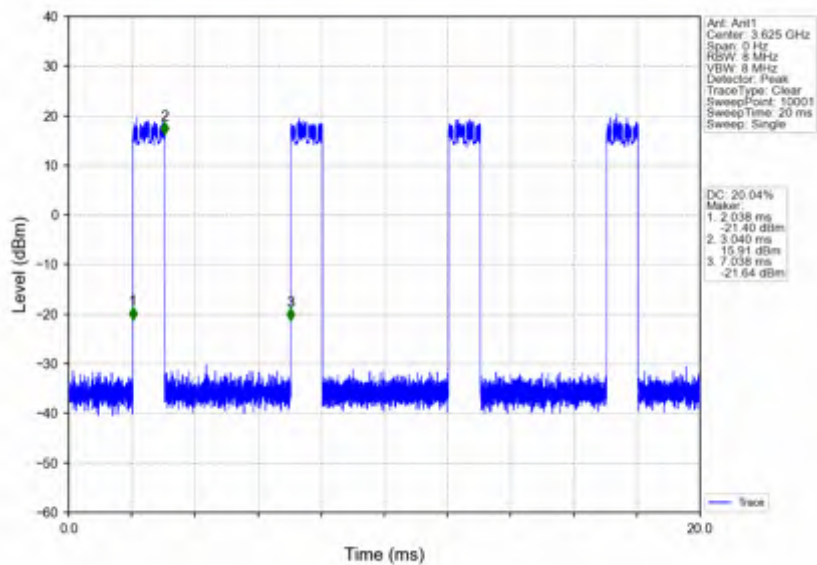
n78d_15kHz_SISO_NTNV_30MHz_DFT-s-OFDM_256_QAM_3625.005MHz_Inner_Full
