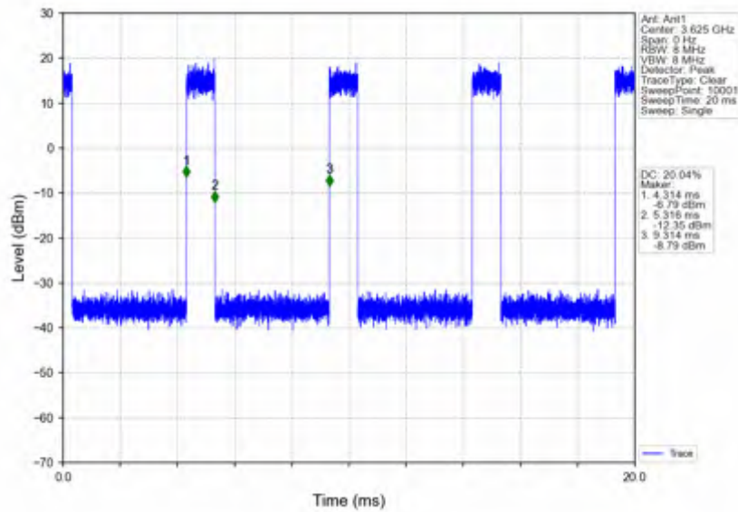
n78d_15kHz_SISO_NTNV_30MHz_CP-OFDM 64 QAM_3625.005MHz_Inner_Full
