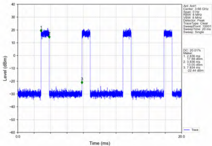
n78d_15kHz_SISO_NTNV_40MHz_CP-OFDM 64 QAM_3679.995MHz_Inner_Full
