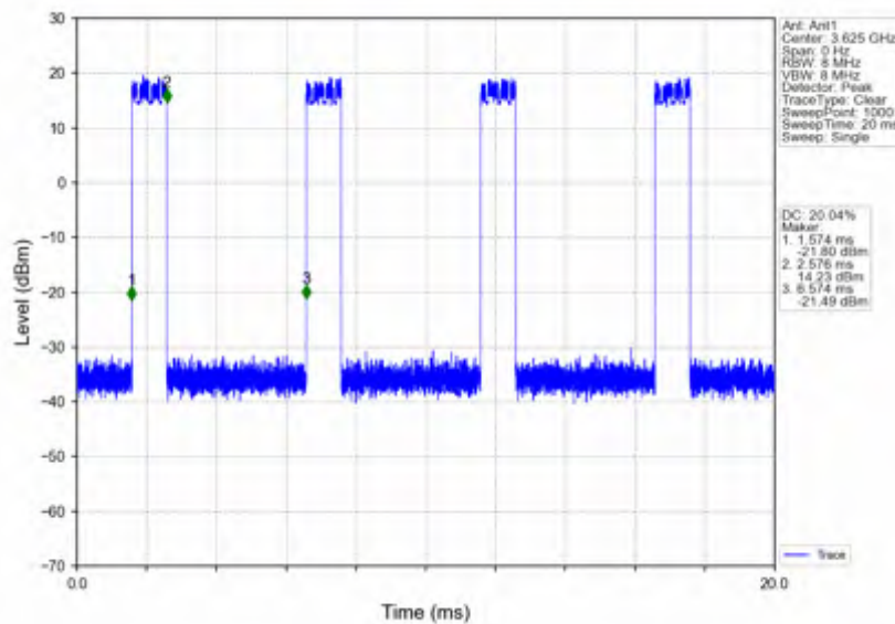
n78d_15kHz_SISO_NTNV_30MHz_DFT-s-OFDM 64 QAM_3625.005MHz_Inner_Full
