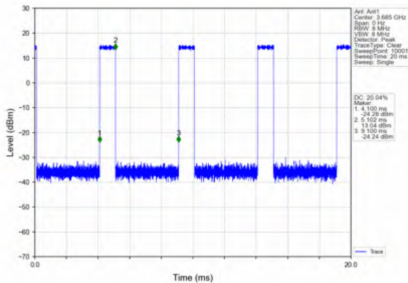
n78d_15kHz_SISO_NTNV_30MHz_DFT-s-OFDM PI/2 BPSK_3684.99MHz_Inner_Full
