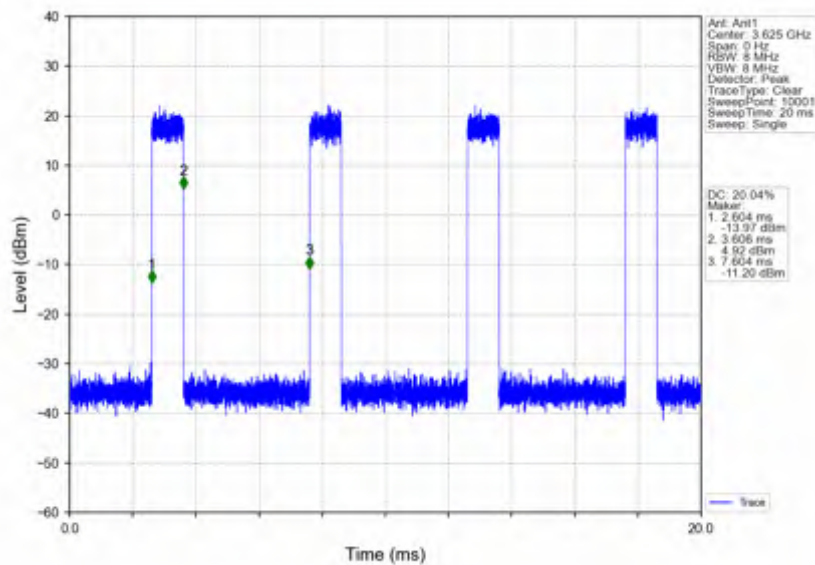
n78d_15kHz_SISO_NTNV_30MHz_CP-OFDM QPSK_3625.005MHz_Inner_Full
