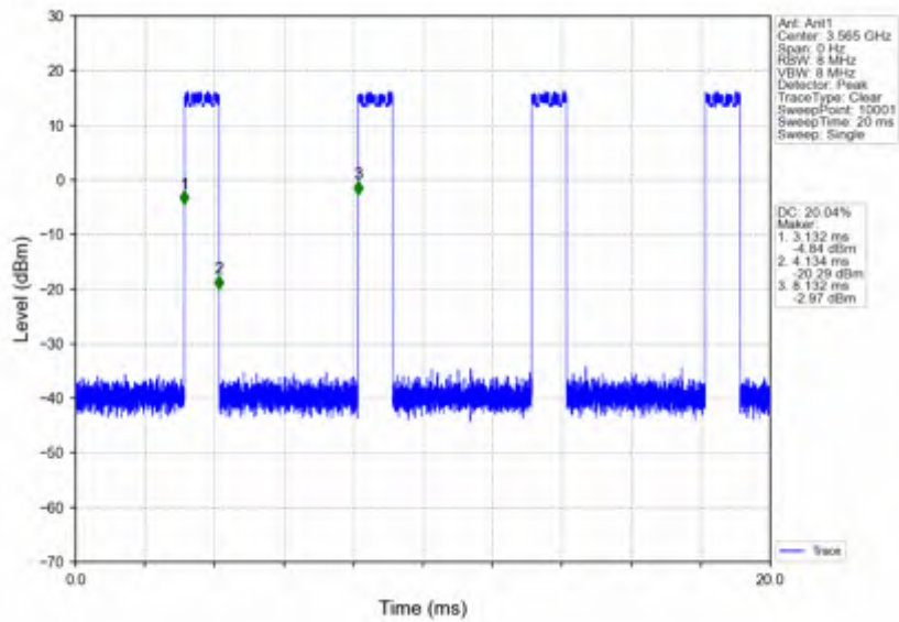
n78d_15kHz_SISO_NTNV_30MHz_DFT-s-OFDM QPSK_3565.005MHz_Inner_Full
