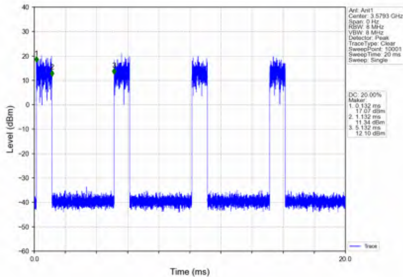
n78d_15kHz_SISO_NTNV_30MHz_DFT-s-OFDM 64 QAM_3565.005MHz_Edge_1RB_Right
