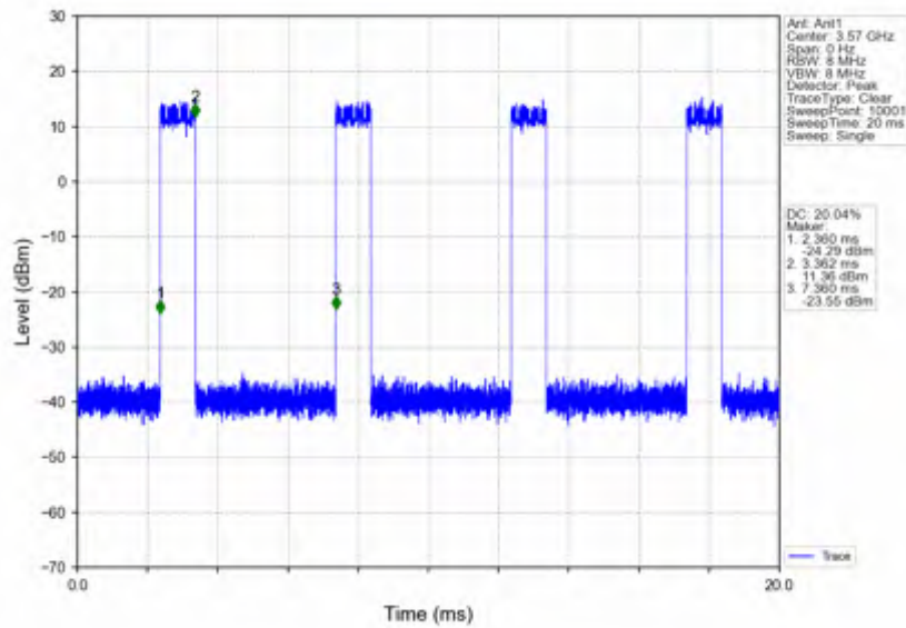
n78d_15kHz_SISO_NTNV_40MHz_DFT-s-OFDM_QPSK_3570MHz_Inner_Full
