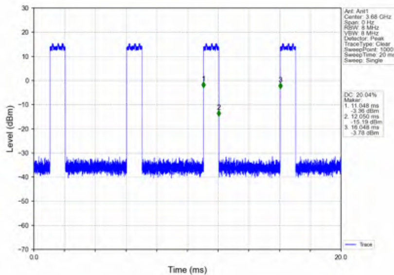
n78d_15kHz_SISO_NTNV_40MHz_DFT-s-OFDM PI/2 BPSK_3679.995MHz_Inner_Full
