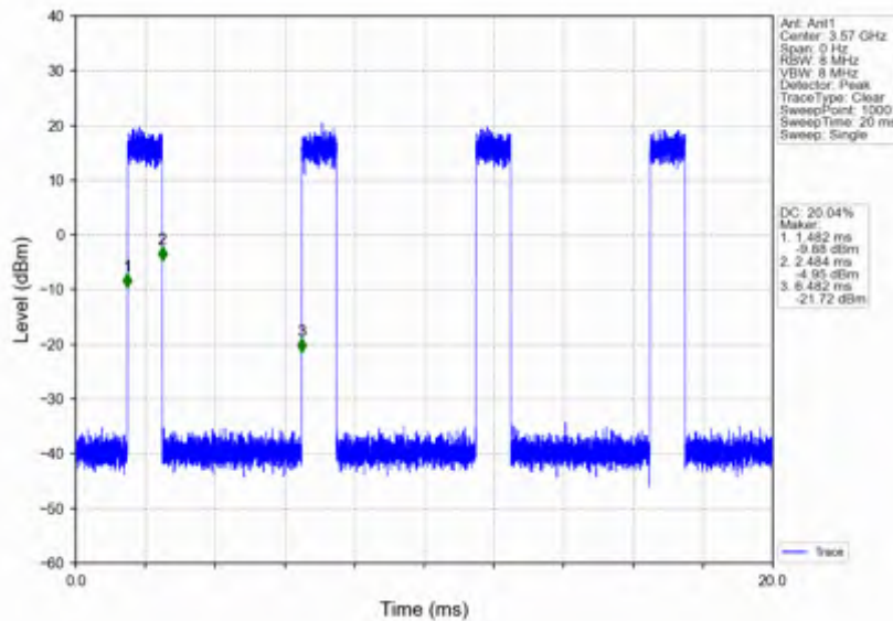
n78d_15kHz_SISO_NTNV_40MHz_CP-OFDM 256 QAM_3570MHz_Inner_Full
