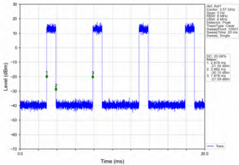
n78d_15kHz_SISO_NTNV_40MHz_CP-OFDM 64 QAM_3570MHz_Inner_Full
