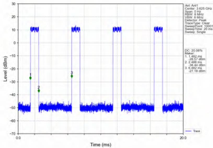
n78d_15kHz_SISO_NTNV_50MHz_DFT-s-OFDM PI/2 BPSK_3625.005MHz_Inner_Full
