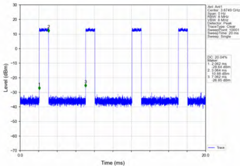
n78d_15kHz_SISO_NTNV_50MHz_DFT-s-OFDM PI/2 BPSK_3675MHz_Inner_Full
