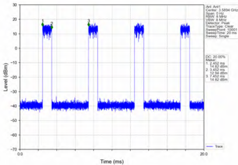
n78d_15kHz_SISO_NTNV_40MHz_DFT-s-OFDM_PI/2_BPSK_3570MHz_Edge_1RB_Right
