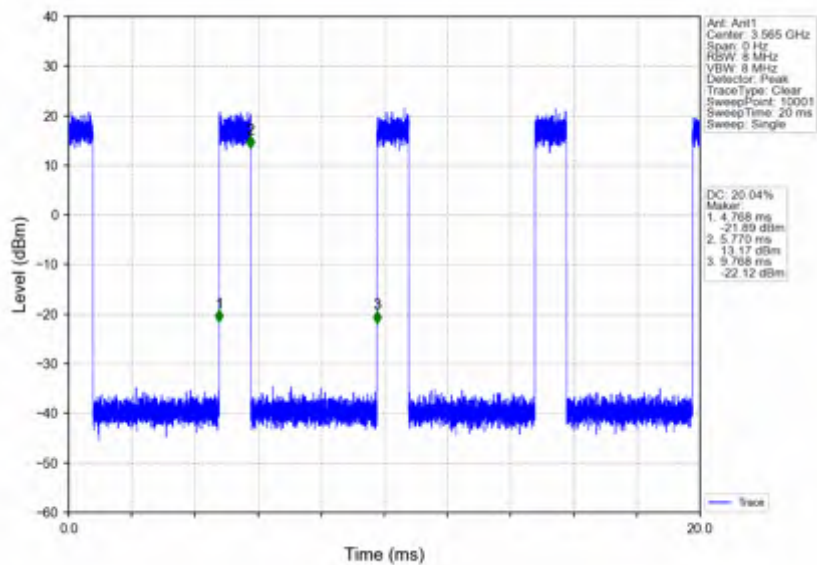
n78d_15kHz_SISO_NTNV_30MHz_CP-OFDM 16 QAM_3565.005MHz_Inner_Full
