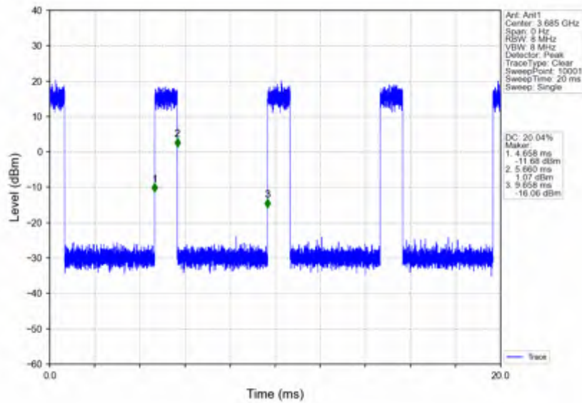
n78d_15kHz_SISO_NTV_30MHz_CP-OFDM 16 QAM_3684.99MHz_Inner_Full
