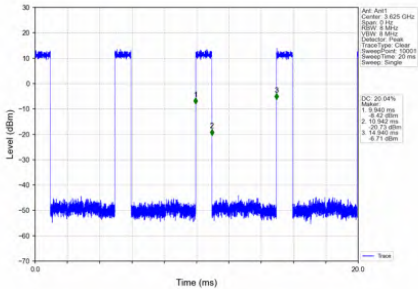
n78d_15kHz_SISO_NTNV_40MHz_DFT-s-OFDM PI/2 BPSK_3625.005MHz_Inner_Full
