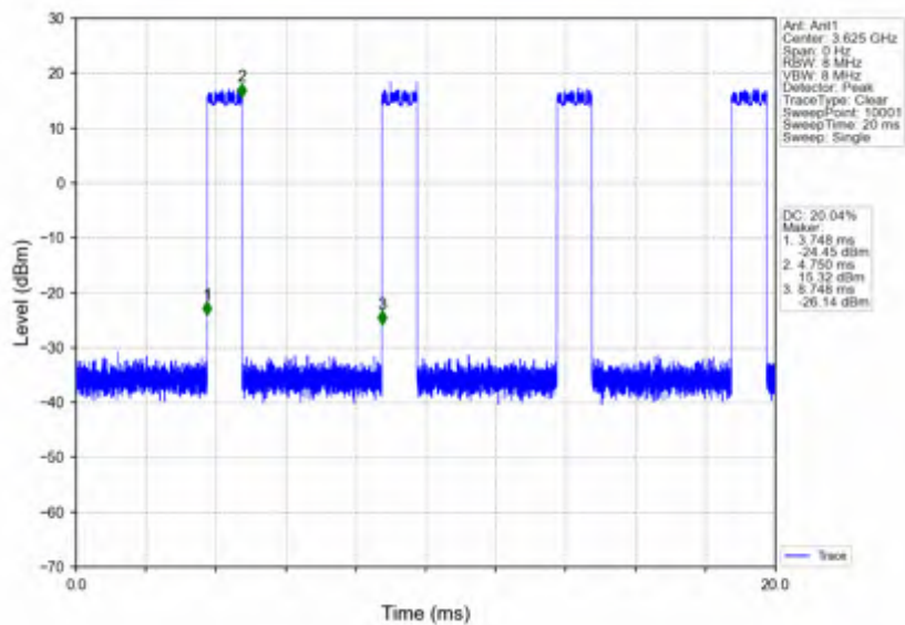
n78d_15kHz_SISO_NTNV_30MHz_DFT-s-OFDM QPSK_3625.005MHz_Inner_Full
