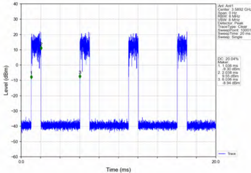
n78d_15kHz_SISO_NTNV_40MHz_CP-OFDM QPSK_3570MHz_Inner_1RB_Right
