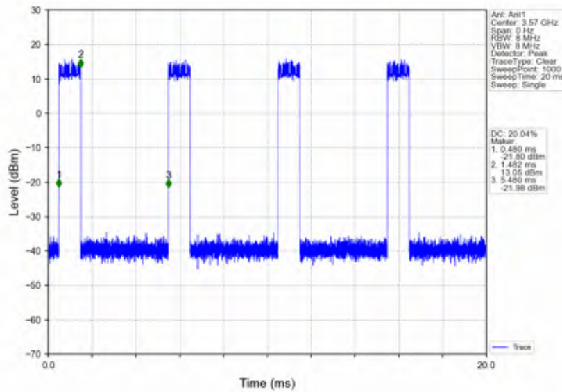
n78d_15kHz_SISO_NTNV_40MHz_DFT-s-OFDM 16 QAM_3570MHz_Inner_Full
