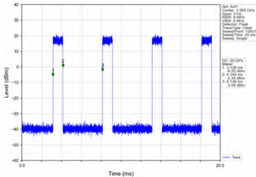
n78d_15kHz_SISO_NTNV_30MHz_CP-OFDM 64 QAM_3565.005MHz_Inner_Full
