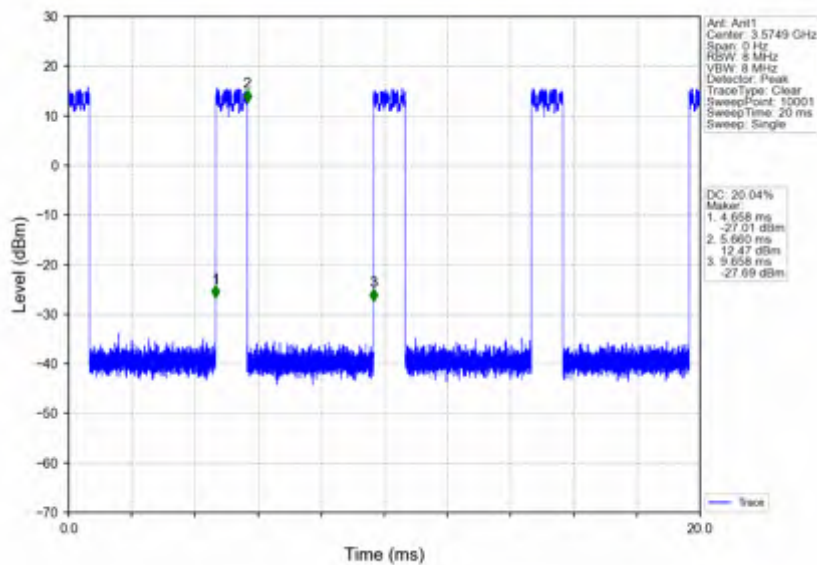
n78d_15kHz_SISO_NTNV_50MHz_DFT-s-OFDM_QPSK_3575.01MHz_Inner_Full
