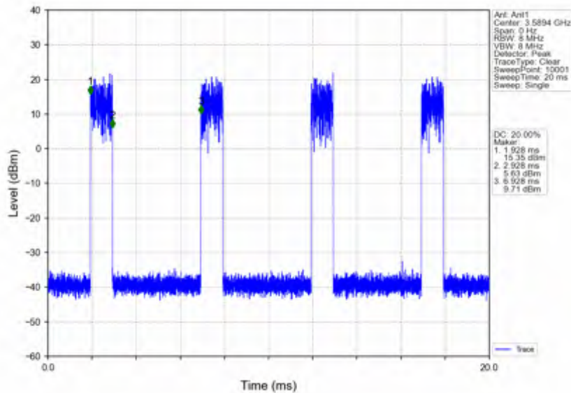
n78d_15kHz_SISO_NTNV_40MHz_CP-OFDM QPSK_3570MHz_Edge_1RB_Right
