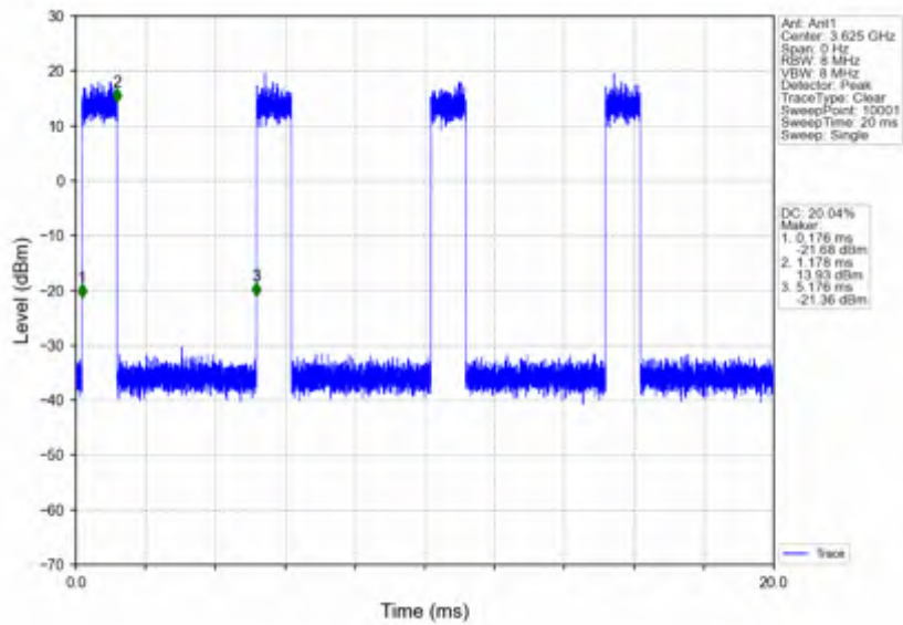
n78d_15kHz_SISO_NTNV_40MHz_CP-OFDM 256 QAM_3625.005MHz_Inner_Full
