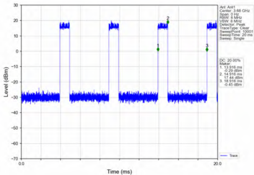
n78d_15kHz_SISO_NTNV_40MHz_DFT-s-OFDM 256 QAM_3679.995MHz_Inner_Full
