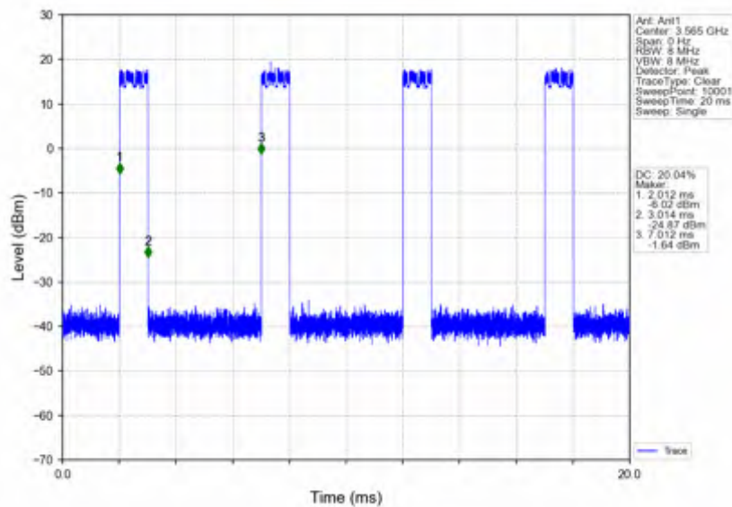
n78d_15kHz_SISO_NTNV_30MHz_DFT-s-OFDM_16_QAM_3565.005MHz_Inner_Full
