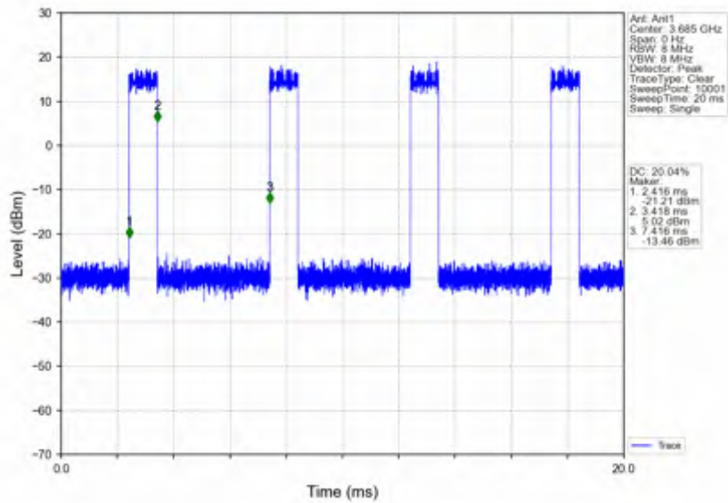
n78d_15kHz_SISO_NTNV_30MHz_DFT-s-OFDM 64 QAM_3684.99MHz_Inner_Full
