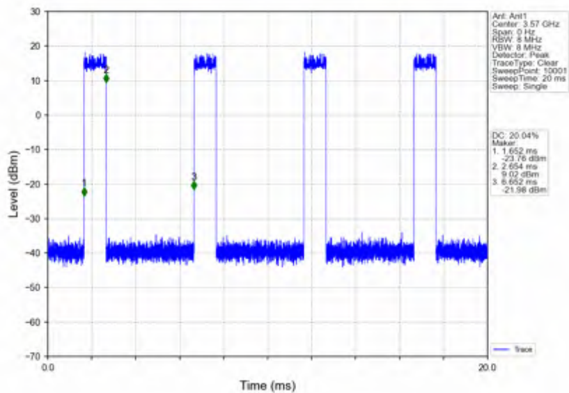
n78d_15kHz_SISO_NTV_40MHz_DFT-s-OFDM 64 QAM_3570MHz_Inner_Full
