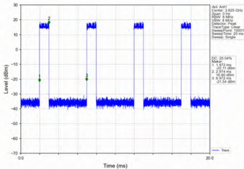
n78d_15kHz_SISO_NTNV_40MHz_DFT-s-OFDM 64 QAM_3625.005MHz_Inner_Full
