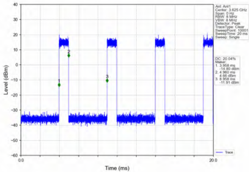
n78d_15kHz_SISO_NTNV_30MHz_CP-OFDM 256 QAM_3625.005MHz_Inner_Full
