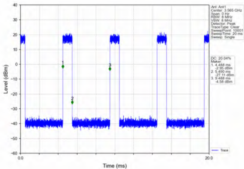
n78d_15kHz_SISO_NTNV_30MHz_CP-OFDM 256 QAM_3565.005MHz_Inner_Full
