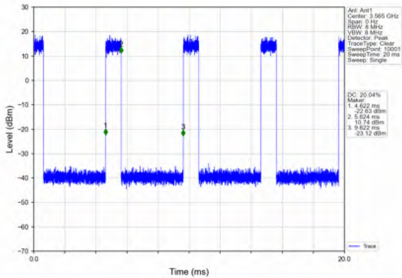
n78d_15kHz_SISO_NTNV_30MHz_CP-OFDM QPSK_3565.005MHz_Inner_Full
