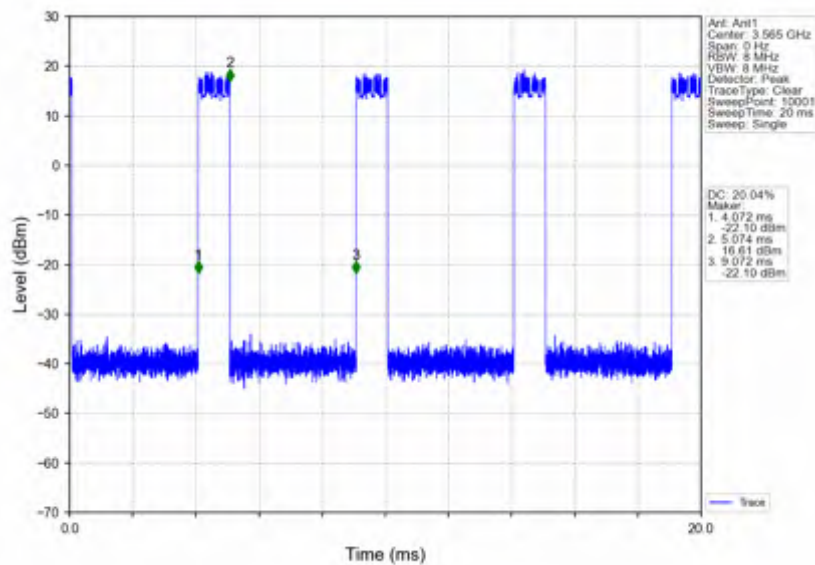
n78d_15kHz_SISO_NTNV_30MHz_DFT-s-OFDM 256 QAM_3565.005MHz_Inner_Full
