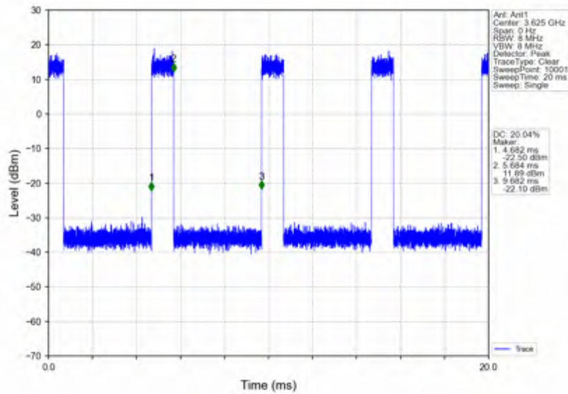
n78d_15kHz_SISO_NTNV_40MHz_CP-OFDM QPSK_3625.005MHz_Inner_Full
