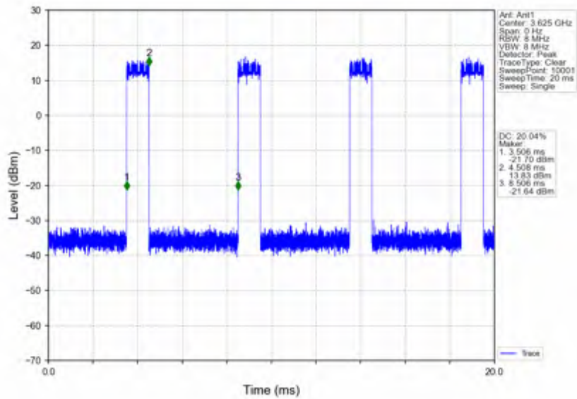
n78d_15kHz_SISO_NTNV_40MHz_DFT-s-OFDM_16_QAM_3625.005MHz_Inner_Full
