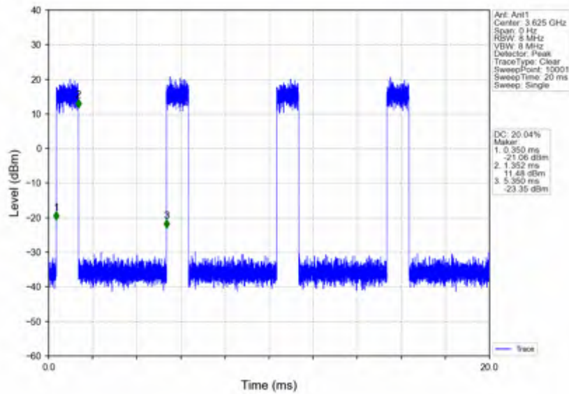
n78d_15kHz_SISO_NTNV_25MHz_CP-OFDM 64 QAM_3625.005MHz_Inner_Full
