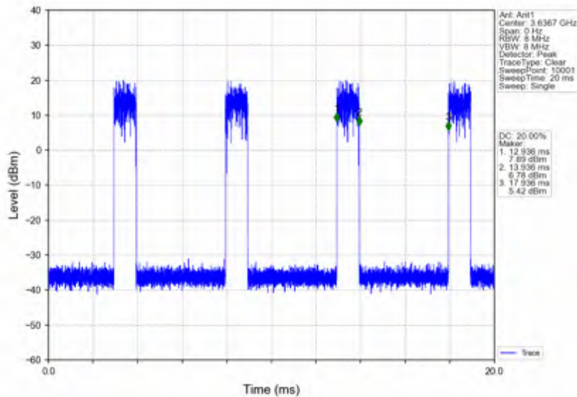
n78d_15kHz_SISO_NTNV_25MHz_DFT-s-OFDM_256_QAM_3625.005MHz_Inner_1RB_Right
