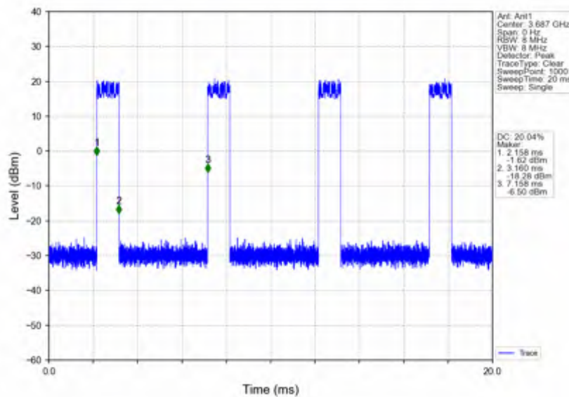
n78d_15kHz_SISO_NTNV_25MHz_DFT-s-OFDM 64 QAM_3687.495MHz_Inner_Full
