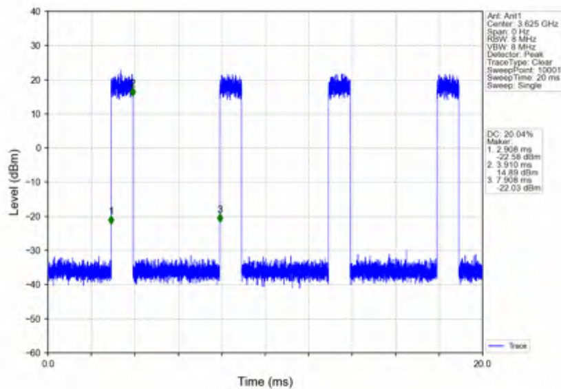
n78d_15kHz_SISO_NTNV_25MHz_CP-OFDM_16 QAM_3625.005MHz_Inner_Full
