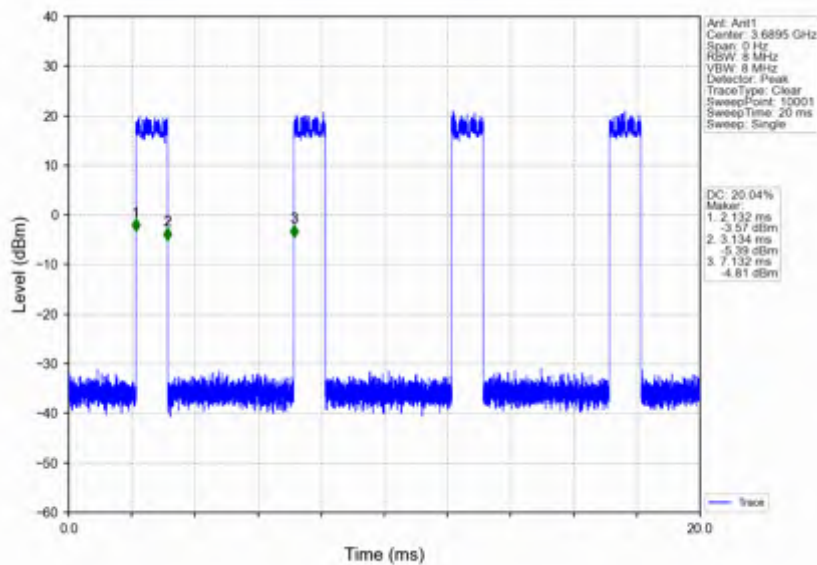
n78d_15kHz_SISO_NTNV_20MHz_DFT-s-OFDM 16 QAM_3690MHz_Inner_Full
