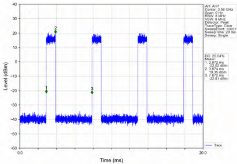
n78d_15kHz_SISO_NTV_20MHz_CP-OFDM 16 QAM_3560.01MHz_Inner_Full
