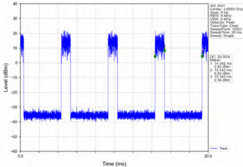
n78d_15kHz_SISO_NTNV_20MHz_CP-OFDM_16 QAM_3690MHz_Inner_1RB_Right
