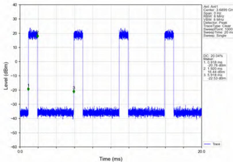
n78d_15kHz_SISO_NTNV_20MHz_CP-OFDM_256 QAM_3690MHz_Inner_Full
