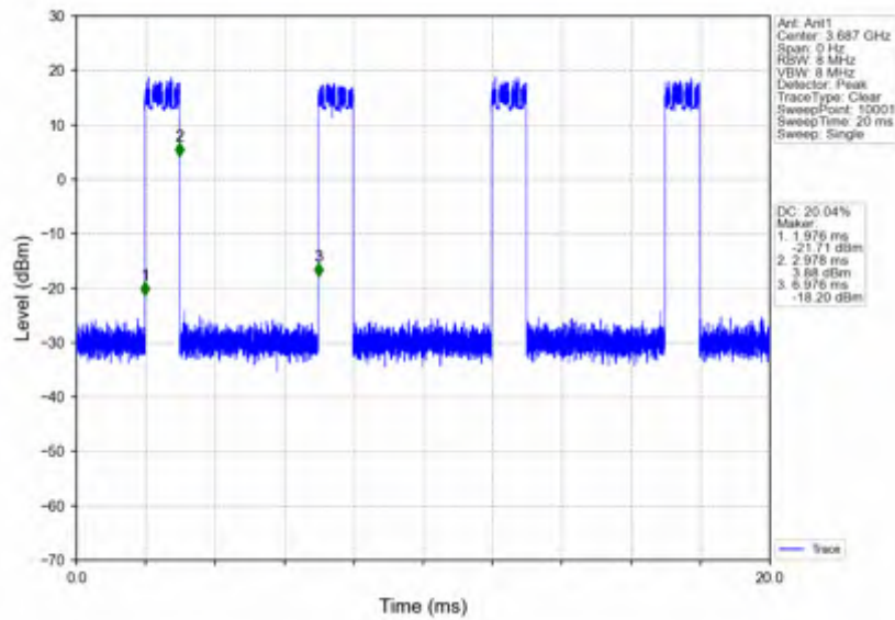
n78d_15kHz_SISO_NTNV_25MHz_DFT-s-OFDM_256 QAM_3687.495MHz_Inner_Full
