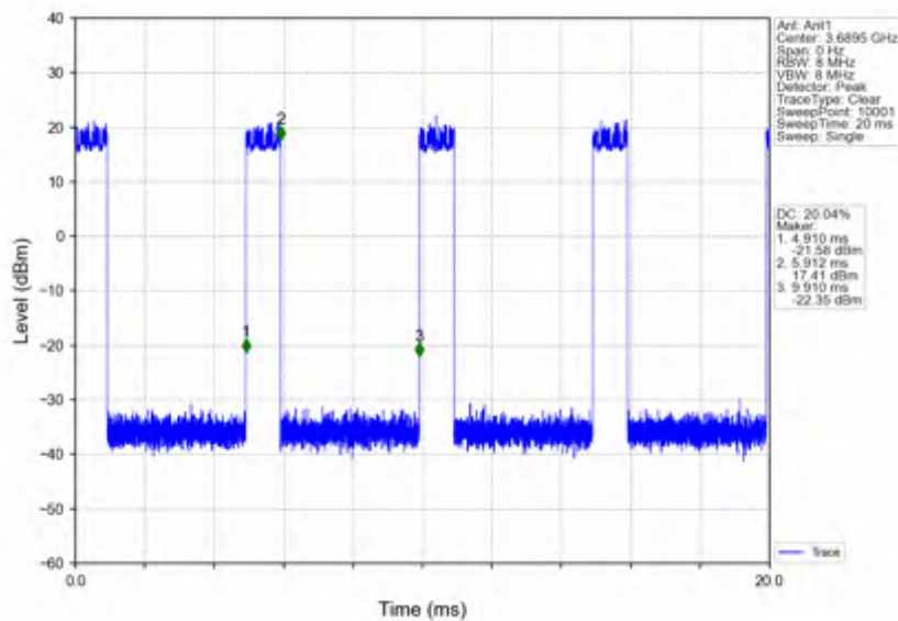
n78d_15kHz_SISO_NTNV_20MHz_DFT-s-OFDM 64 QAM_3690MHz_Inner_Full
