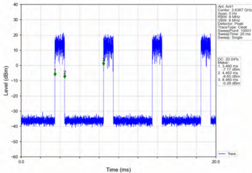
n78d_15kHz_SISO_NTV_25MHz_CP-OFDM QPSK_3625.005MHz_Inner_1RB_Right
