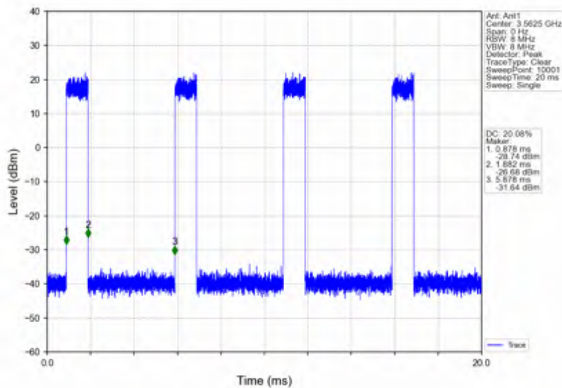
n78d_15kHz_SISO_NTV_25MHz_CP-OFDM 256 QAM_3562.5MHz_Inner_Full
