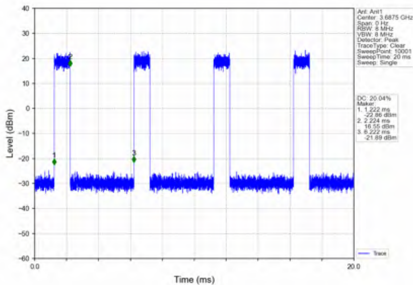
n78d_15kHz_SISO_NTNV_25MHz_CP-OFDM 64 QAM_3687.495MHz_Inner_Full
