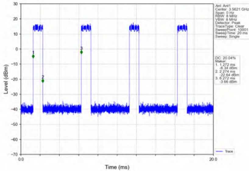
n78d_15kHz_SISO_NTNV_25MHz_DFT-s-OFDM 16 QAM_3562.5MHz_Inner_Full
