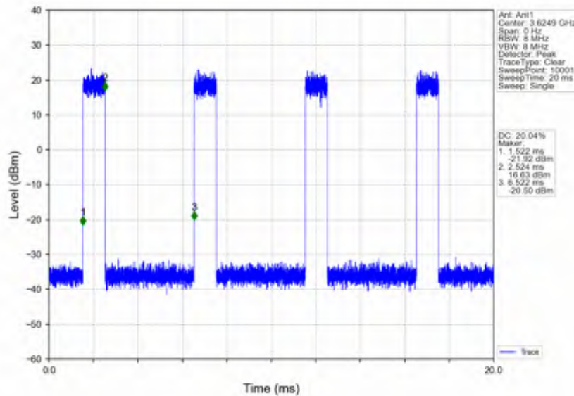
n78d_15kHz_SISO_NTNV_20MHz_CP-OFDM 16 QAM_3625.005MHz_Inner_Full
