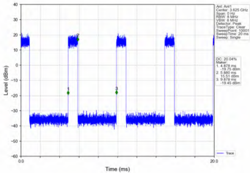
n78d_15kHz_SISO_NTNV_25MHz_CP-OFDM 256 QAM_3625.005MHz_Inner_Full
