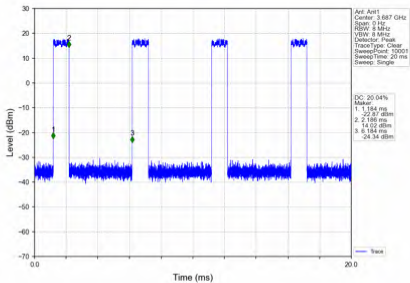
n78d_15kHz_SISO_NTNV_25MHz_DFT-s-OFDM QPSK_3687.495MHz_Inner_Full
