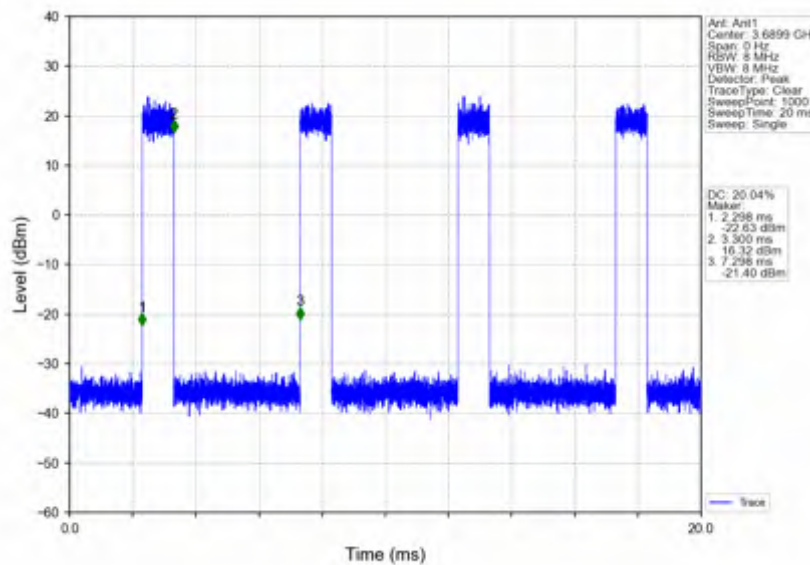
n78d_15kHz_SISO_NTNV_20MHz_CP-OFDM_16 QAM_3690MHz_Inner_Full
