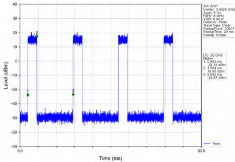
n78d_15kHz_SISO_NTNV_25MHz_CP-OFDM_16 QAM_3562.5MHz_Inner_Full
