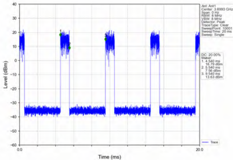
n78d_15kHz_SISO_NTNV_20MHz_CP-OFDM QPSK_3690MHz_Inner_1RB_Right
