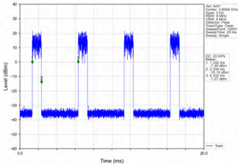
n78d_15kHz_SISO_NTNV_20MHz_CP-OFDM_16 QAM_3690MHz_Edge_1RB_Right
