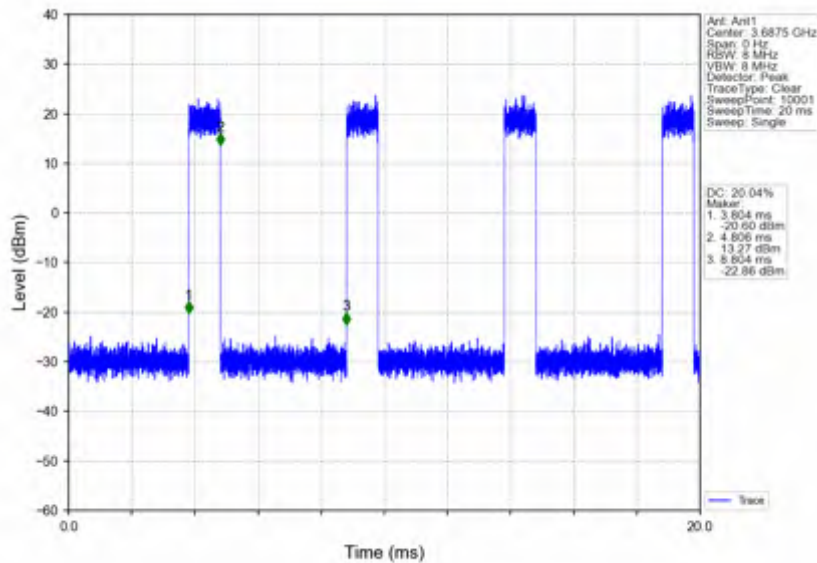
n78d_15kHz_SISO_NTNV_25MHz_CP-OFDM 256 QAM_3687.495MHz_Inner_Full
