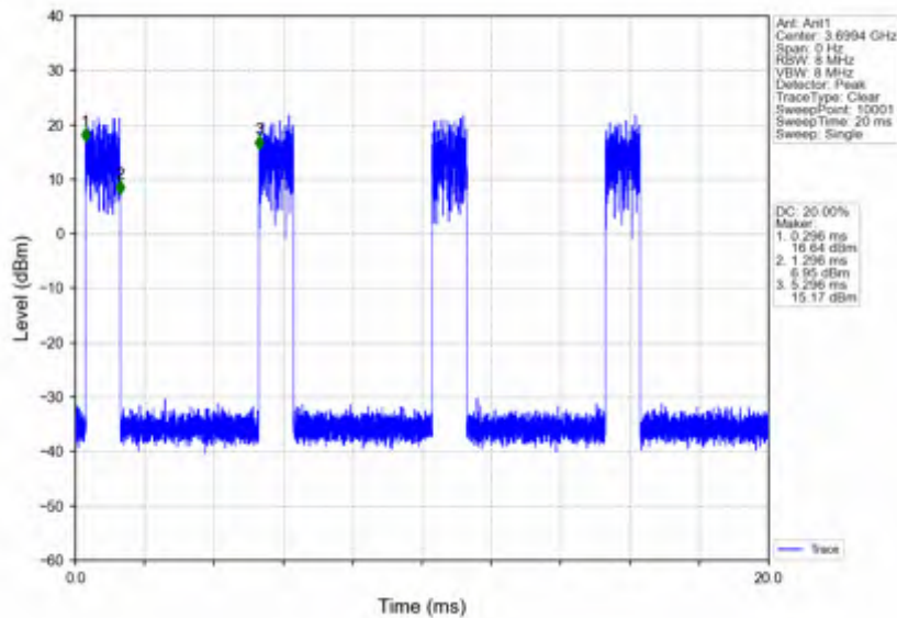
n78d_15kHz_SISO_NTNV_20MHz_CP-OFDM_QPSK_3690MHz_Edge_1RB_Right
