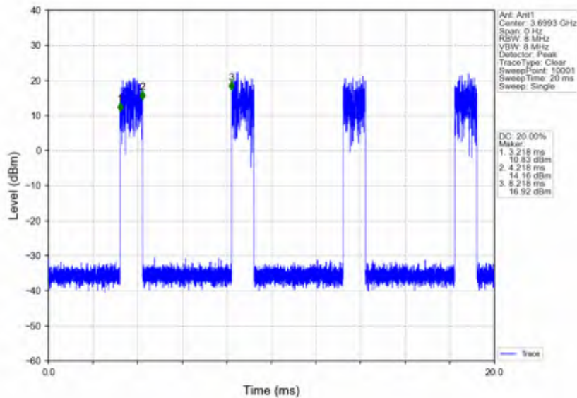
n78d_15kHz_SISO_NTV_20MHz_CP-OFDM 256 QAM_3690MHz_Inner_1RB_Right
