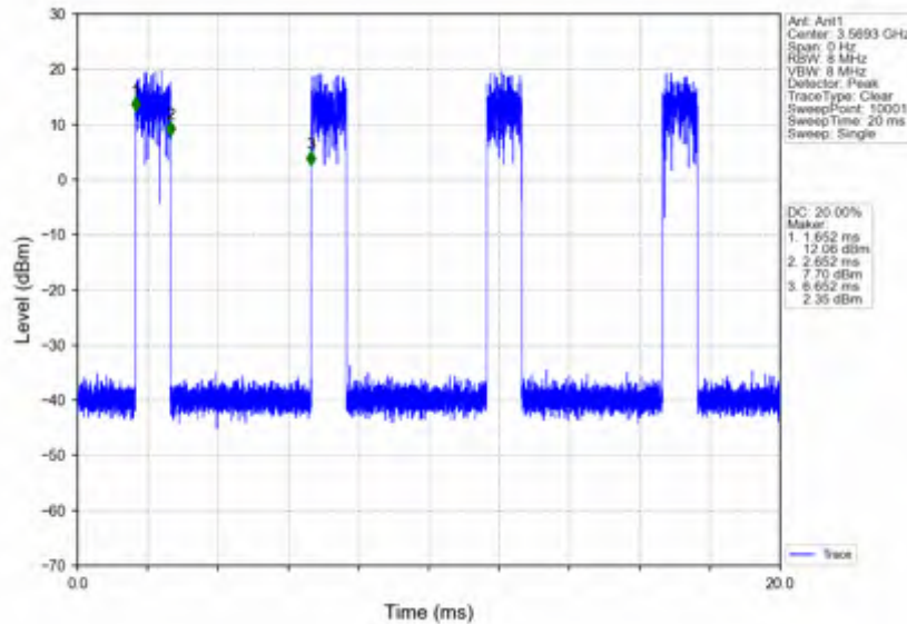
n78d_15kHz_SISO_NTNV_20MHz_DFT-s-OFDM 256 QAM_3560.01MHz_Inner_1RB_Right
