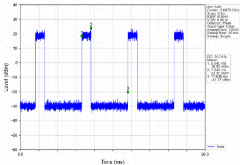
n78d_15kHz_SISO_NTNV_25MHz_CP-OFDM QPSK_3687.495MHz_Inner_Full
