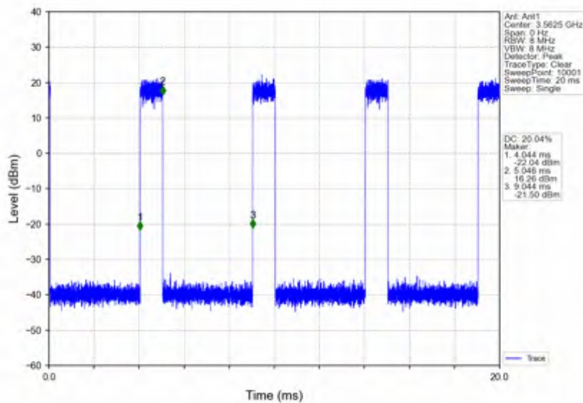
n78d_15kHz_SISO_NTNV_25MHz_CP-OFDM 64 QAM_3562.5MHz_Inner_Full
