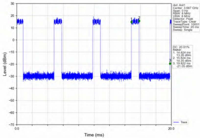
n78d_15kHz_SISO_NTNV_25MHz_DFT-s-OFDM_16_QAM_3687.495MHz_Inner_Full
