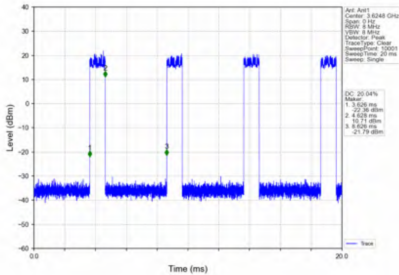
n78d_15kHz_SISO_NTNV_10MHz_DFT-s-OFDM 64 QAM_3625.005MHz_Inner_Full
