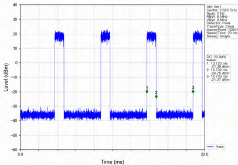
n78d_15kHz_SISO_NTNV_10MHz_CP-OFDM 16 QAM_3625.005MHz_Inner_Full
