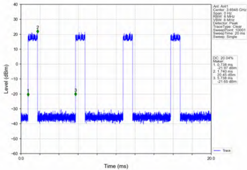
n78d_15kHz_SISO_NTNV_10MHz_DFT-s-OFDM 64 QAM_3694.995MHz_Inner_Full
