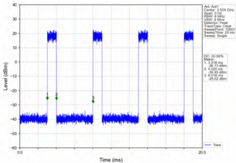
n78d_15kHz_SISO_NTNV_10MHz_CP-OFDM QPSK_3555MHz_Inner_Full
