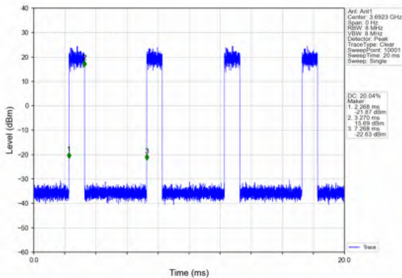
n78d_15kHz_SISO_NTV_15MHz_CP-OFDM 64 QAM_3692.49MHz_Inner_Full
