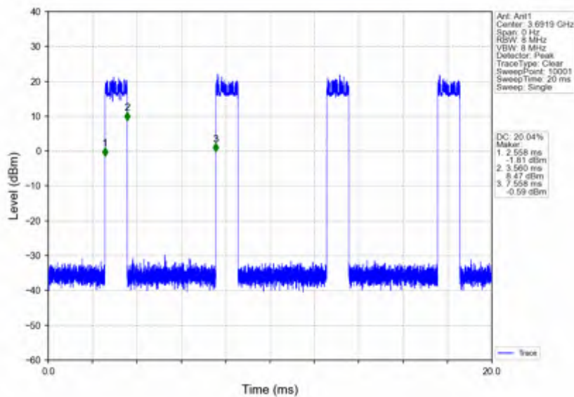
n78d_15kHz_SISO_NTNV_15MHz_DFT-s-OFDM 16 QAM_3692.49MHz_Inner_Full
