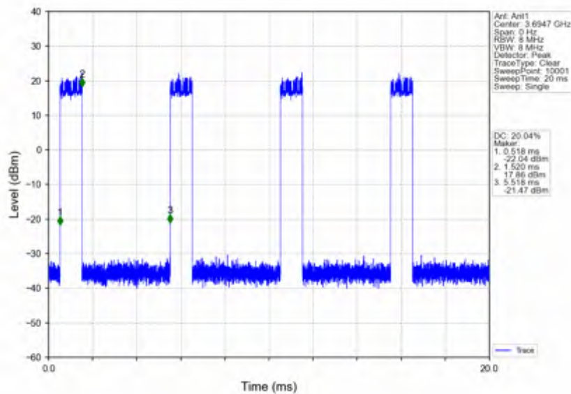
n78d_15kHz_SISO_NTNV_10MHz_DFT-s-OFDM 256 QAM_3694.995MHz_Inner_Full
