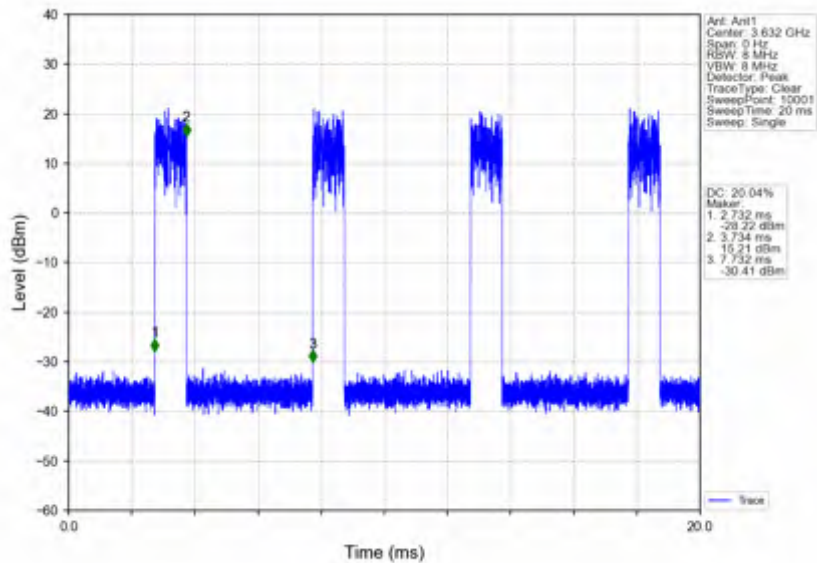
n78d_15kHz_SISO_NTNV_15MHz_CP-OFDM 16 QAM_3625.005MHz_Edge_1RB_Right
