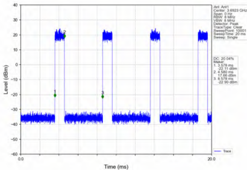
n78d_15kHz_SISO_NTV_15MHz_CP-OFDM 16 QAM_3692.49MHz_Inner_Full
