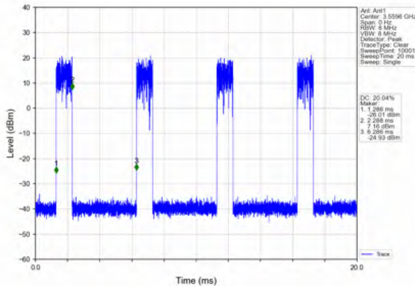
n78d_15kHz_SISO_NTNV_10MHz_CP-OFDM QPSK_3555MHz_Edge_1RB_Right
