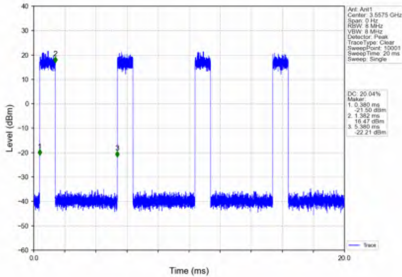
n78d_15kHz_SISO_NTNV_15MHz_CP-OFDM 64 QAM_3557.505MHz_Inner_Full
