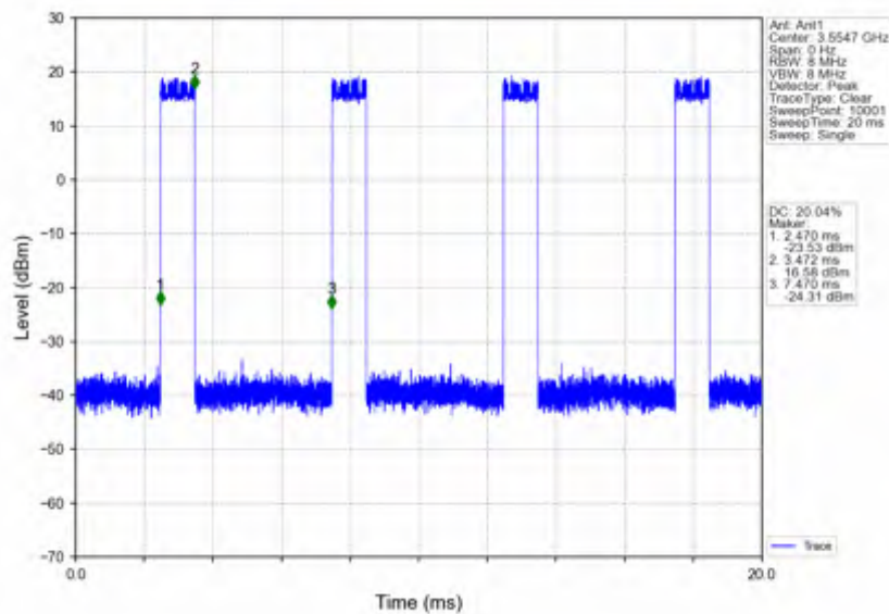
n78d_15kHz_SISO_NTNV_10MHz_DFT-s-OFDM QPSK_3555MHz_Inner_Full
