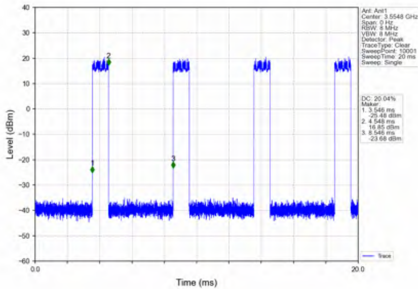
n78d_15kHz_SISO_NTNV_10MHz_DFT-s-OFDM 64 QAM_3555MHz_Inner_Full
