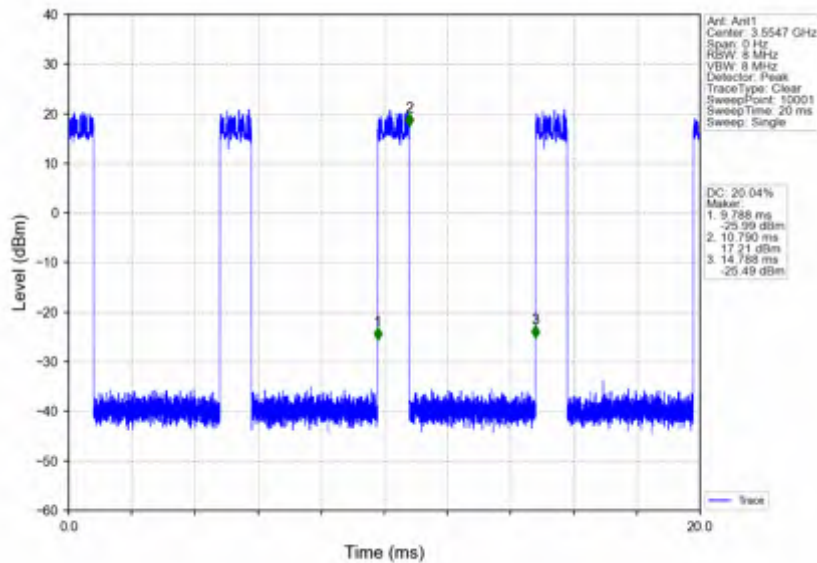
n78d_15kHz_SISO_NTNV_10MHz_DFT-s-OFDM_256_QAM_3555MHz_Inner_Full
