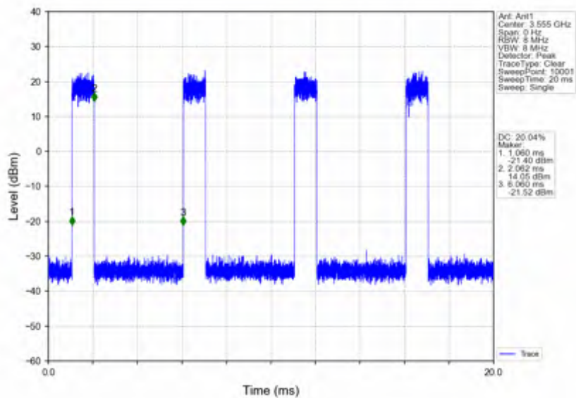
n78d_15kHz_SISO_NTNV_10MHz_CP-OFDM_16 QAM_3555MHz_Inner_Full
