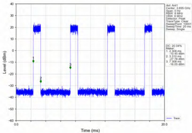
n78d_15kHz_SISO_NTNV_10MHz_CP-OFDM 256 QAM_3694.995MHz_Inner_Full
