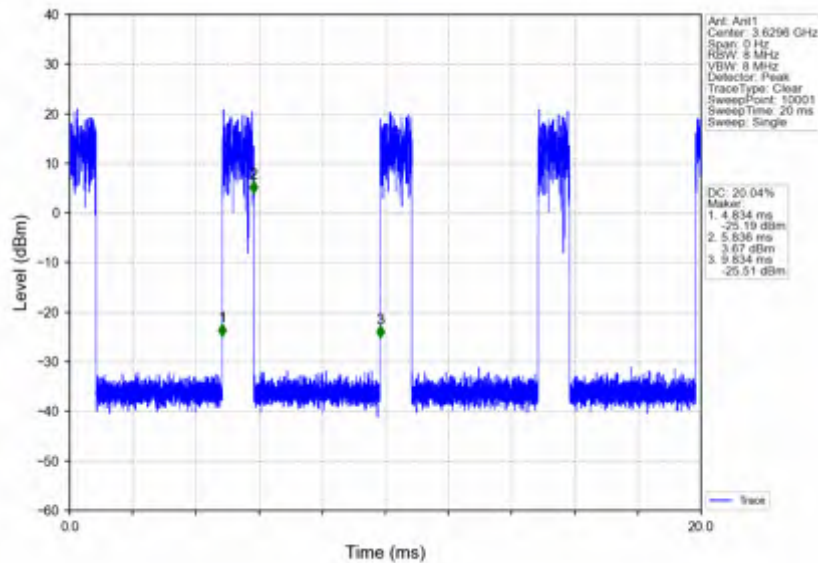
n78d_15kHz_SISO_NTNV_10MHz_CP-OFDM 16 QAM_3625.005MHz_Edge_1RB_Right
