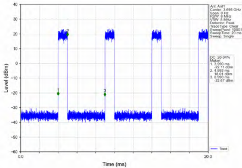
n78d_15kHz_SISO_NTNV_10MHz_CP-OFDM 16 QAM_3694.995MHz_Inner_Full
