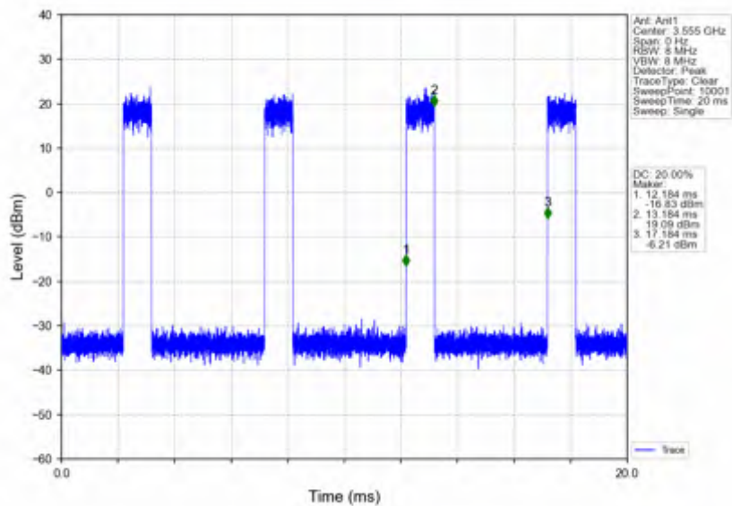
n78d_15kHz_SISO_NTNV_10MHz_CP-OFDM 64 QAM_3555MHz_Inner_Full
