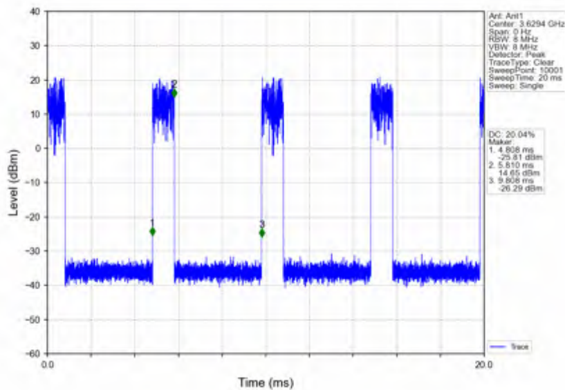
n78d_15kHz_SISO_NTNV_10MHz_CP-OFDM 16 QAM_3625.005MHz_Inner_1RB_Right
