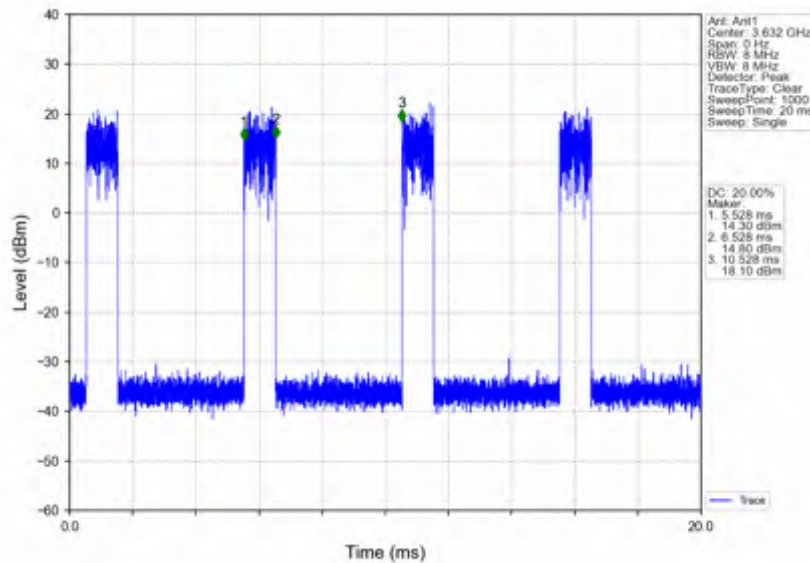
n78d_15kHz_SISO_NTNV_15MHz_CP-OFDM QPSK_3625.005MHz_Edge_1RB_Right
