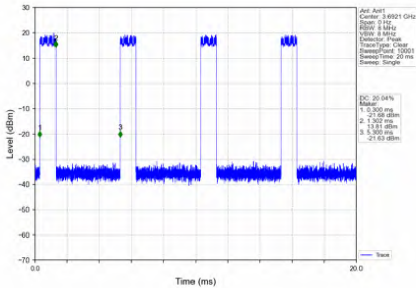
n78d_15kHz_SISO_NTNV_15MHz_DFT-s-OFDM 64 QAM_3692.49MHz_Inner_Full
