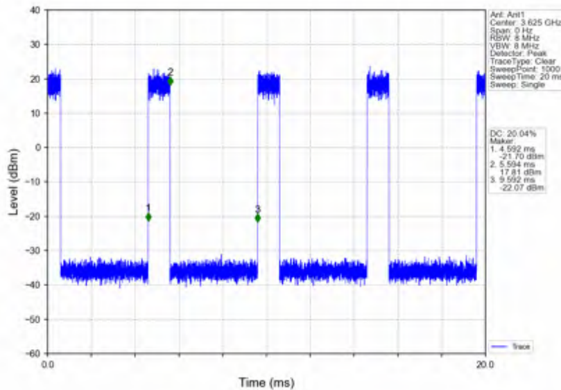
n78d_15kHz_SISO_NTNV_10MHz_CP-OFDM 256 QAM_3625.005MHz_Inner_Full
