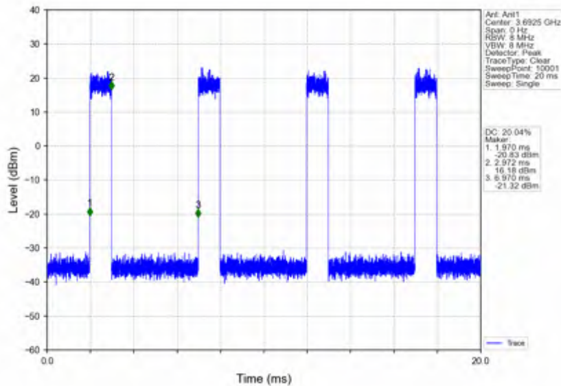
n78d_15kHz_SISO_NTNV_15MHz_CP-OFDM 256 QAM_3692.49MHz_Inner_Full
