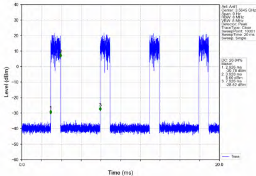
n78d_15kHz_SISO_NTNV_15MHz_CP-OFDM 64 QAM_3557.505MHz_Edge_1RB_Right
