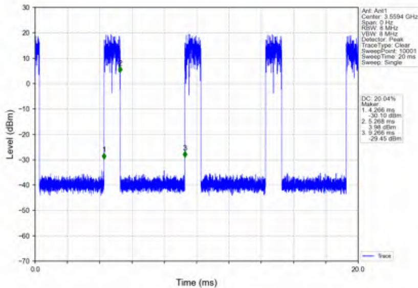
n78d_15kHz_SISO_NTNV_10MHz_DFT-s-OFDM 256 QAM_3555MHz_Inner_1RB_Right
