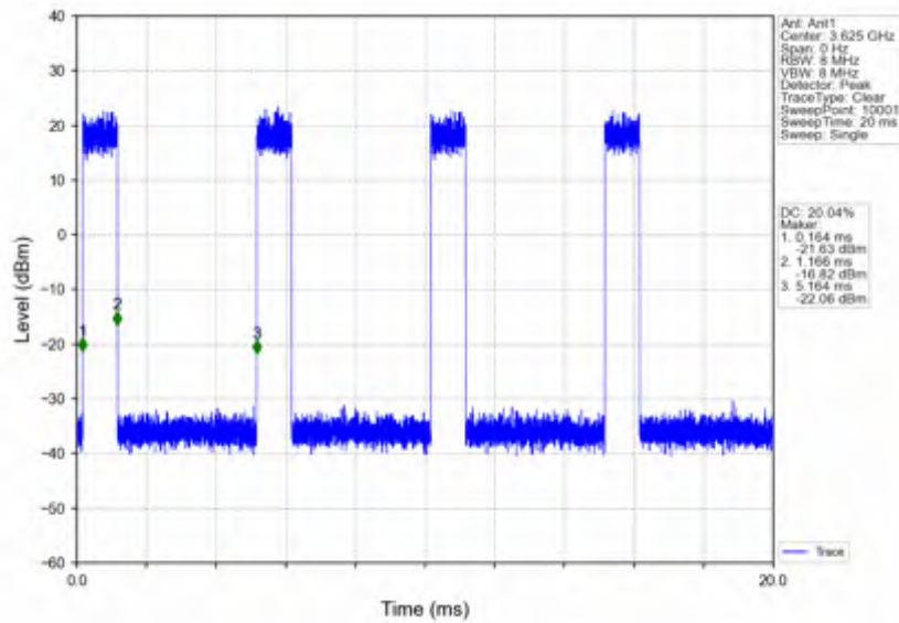
n78d_15kHz_SISO_NTNV_10MHz_CP-OFDM QPSK_3625.005MHz_Inner_Full
