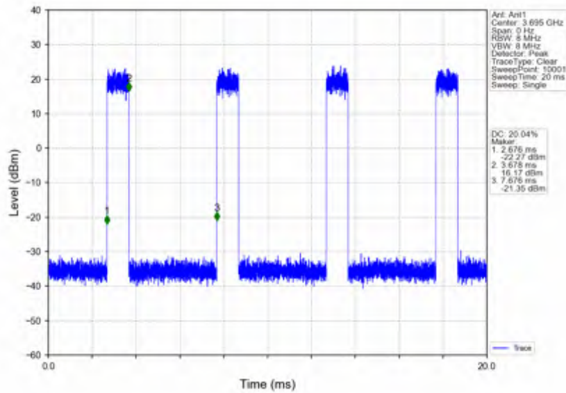
n78d_15kHz_SISO_NTNV_10MHz_CP-OFDM QPSK_3694.995MHz_Inner_Full
