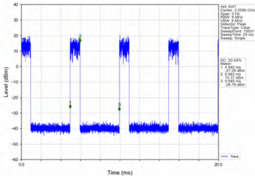
n78d_15kHz_SISO_NTNV_10MHz_DFT-s-OFDM 16 QAM_3555MHz_Edge_1RB_Right
