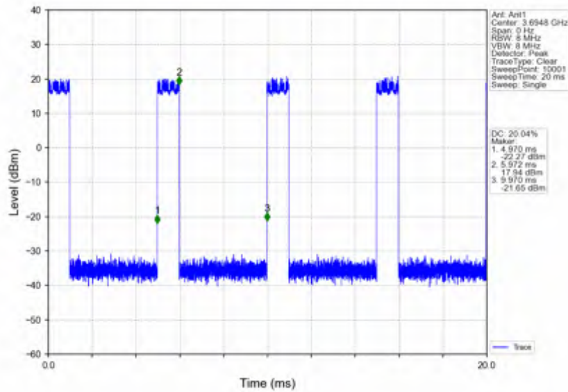
n78d_15kHz_SISO_NTNV_10MHz_DFT-s-OFDM_16_QAM_3694.995MHz_Inner_Full
