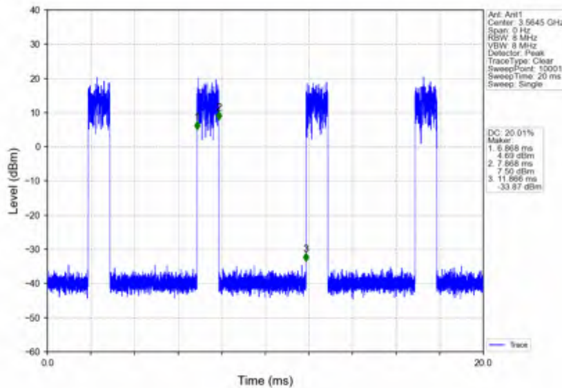
n78d_15kHz_SISO_NTNV_15MHz_DFT-s-OFDM_16_QAM_3557.505MHz_Edge_1RB_Right
