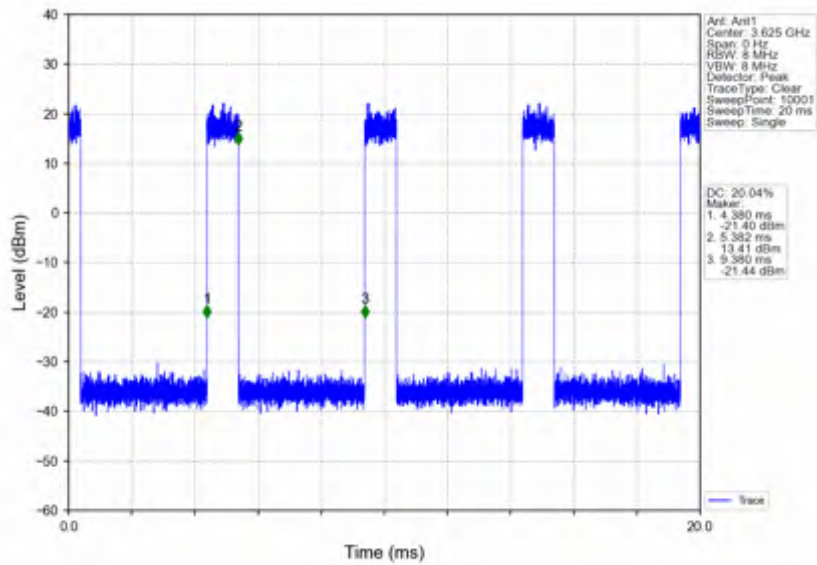
n78d_15kHz_SISO_NTNV_15MHz_CP-OFDM_16 QAM_3625.005MHz_Inner_Full
