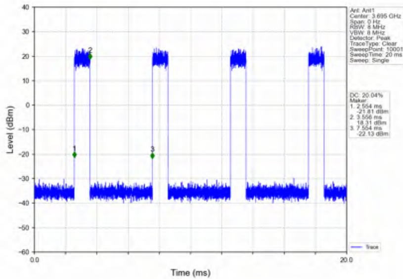
n78d_15kHz_SISO_NTNV_10MHz_CP-OFDM 64 QAM_3694.995MHz_Inner_Full
