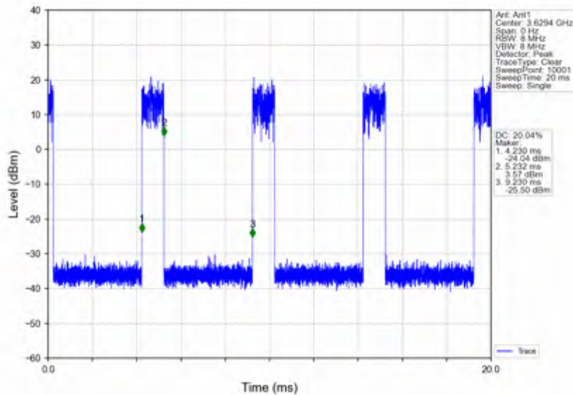
n78d_15kHz_SISO_NTNV_10MHz_DFT-s-OFDM 16 QAM_3625.005MHz_Inner_1RB_Right
