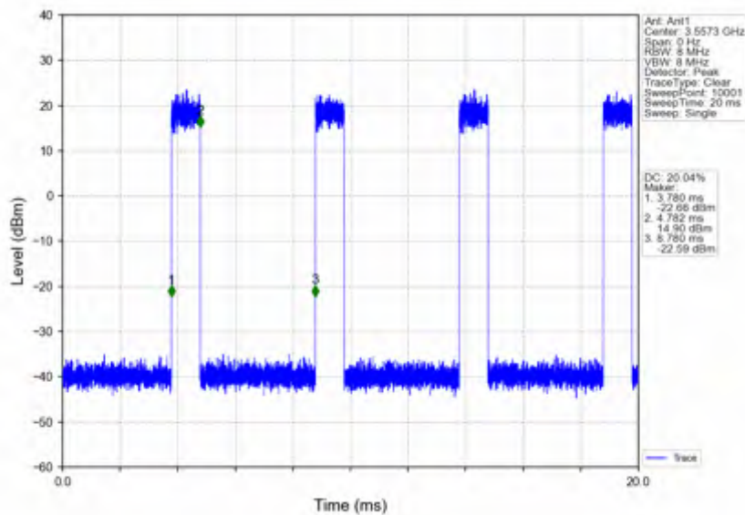
n78d_15kHz_SISO_NTNV_15MHz_CP-OFDM 256 QAM_3557.505MHz_Inner_Full
