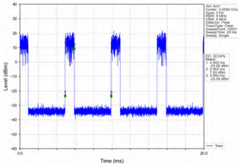
n78d_15kHz_SISO_NTNV_10MHz_CP-OFDM_16 QAM_3555MHz_Inner_1RB_Right
