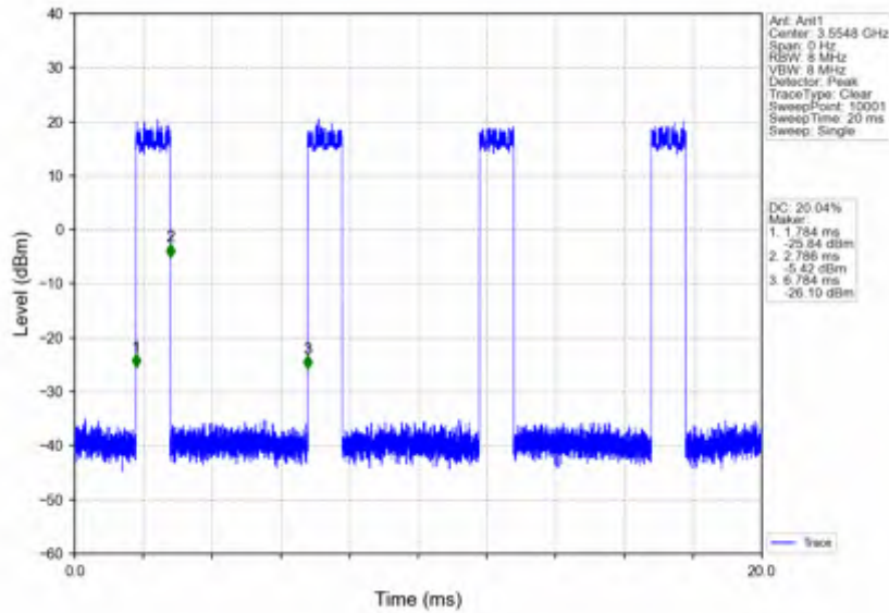
n78d_15kHz_SISO_NTNV_10MHz_DFT-s-OFDM 16 QAM_3555MHz_Inner_Full
