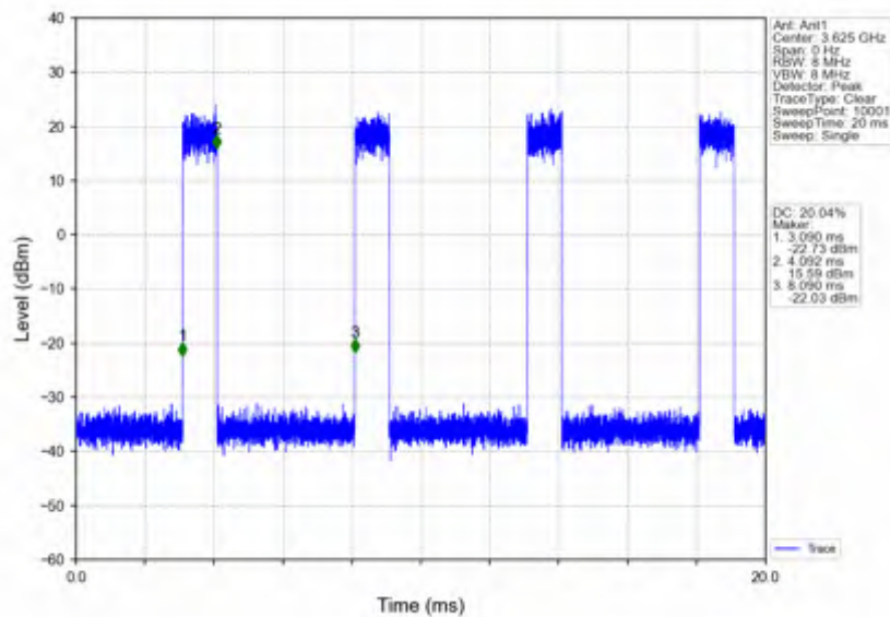
n78d_15kHz_SISO_NTNV_10MHz_CP-OFDM 64 QAM_3625.005MHz_Inner_Full
