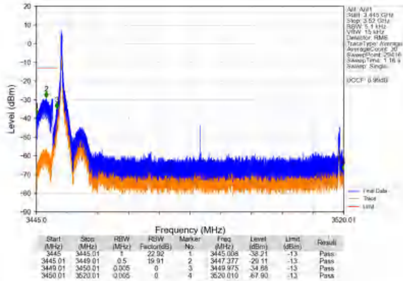
n78e_30kHz_SISO_NTV_70MHz_CP-OFDM QPSK_3485.01MHz_Edge_1RB_Left
