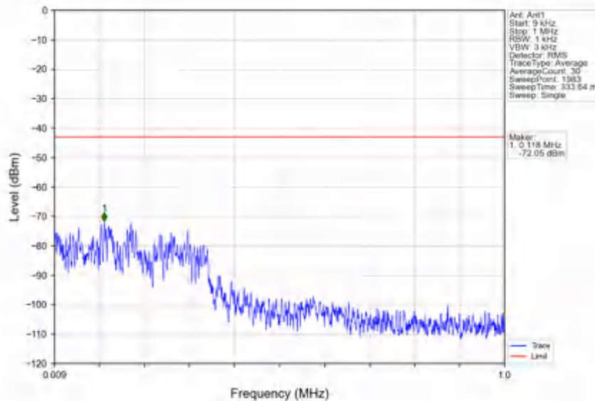
n78e_30kHz_SISO_NTNV_90MHz_DFT-s-OFDM_PI/2_BPSK_3504.99MHz_Edge_1RB_Right
