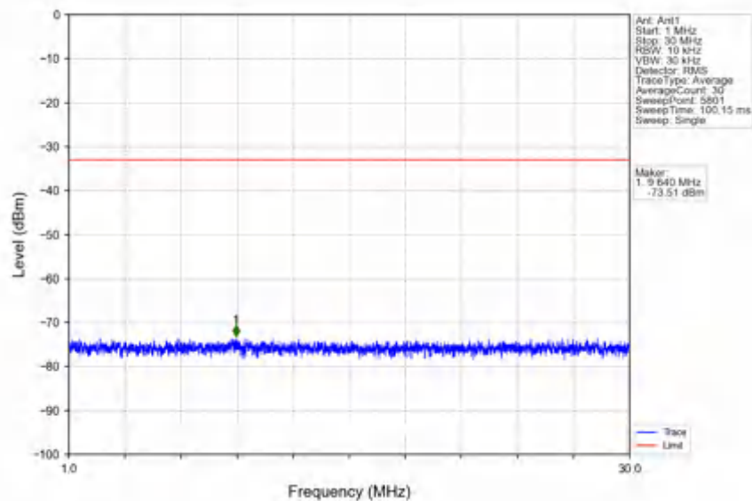
n78e_30kHz_SISO_NTNV_50MHz_CP-OFDM QPSK_3475.02MHz_Outer_Full
