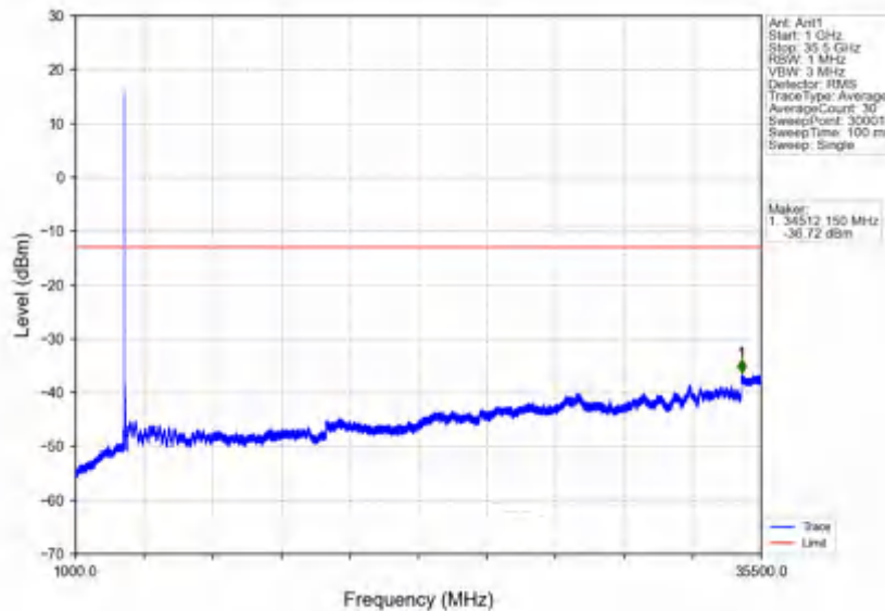
n78e_30kHz_SISO_NTNV_50MHz_DFT-s-OFDM_QPSK_3475.02MHz_Inner_1RB_Left
