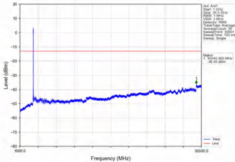
n78e_30kHz_SISO_NTNV_50MHz_DFT-s-OFDM_QPSK_3525MHz_Inner_1RB_Right
