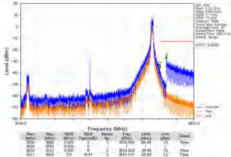
n78e_30kHz_SISO_NTV_20MHz_DFT-s-OFDM PI/2 BPSK_3540MHz_Edge_1RB_Right
