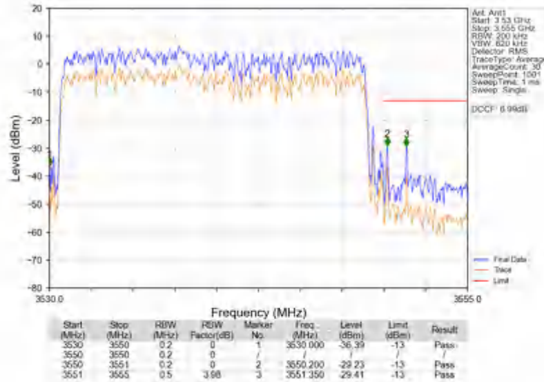
n78e_30kHz_SISO_NTNV_20MHz_DFT-s-OFDM_QPSK_3540MHz_Outer_Full
