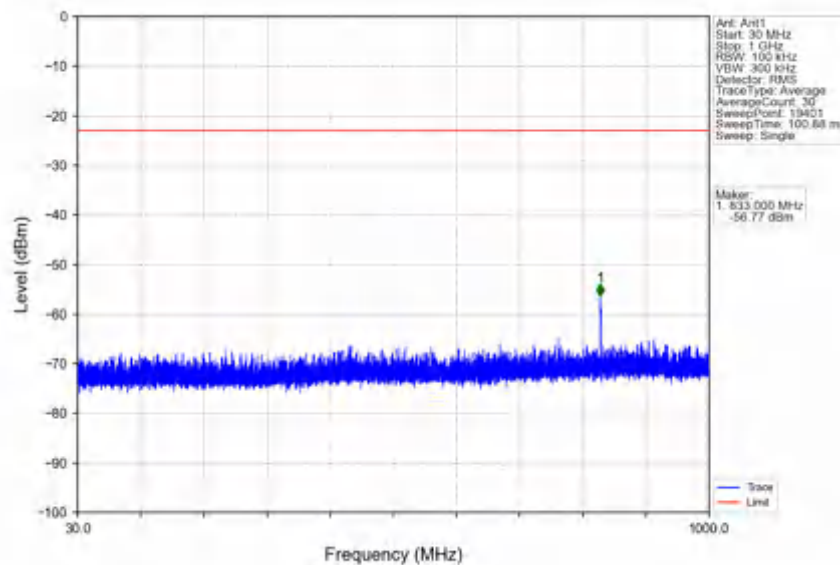
n78e_30kHz_SISO_NTNV_20MHz_DFT-s-OFDM PI/2 BPSK_3460.02MHz_Inner_1RB_Left
