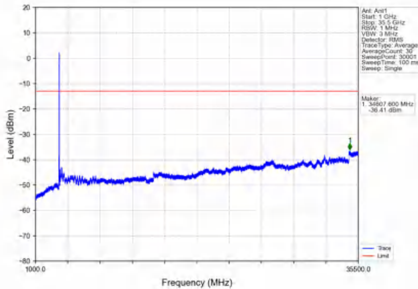
n78e_30kHz_SISO_NTNV_40MHz_DFT-s-OFDM_QPSK_3529.98MHz_Inner_1RB_Right
