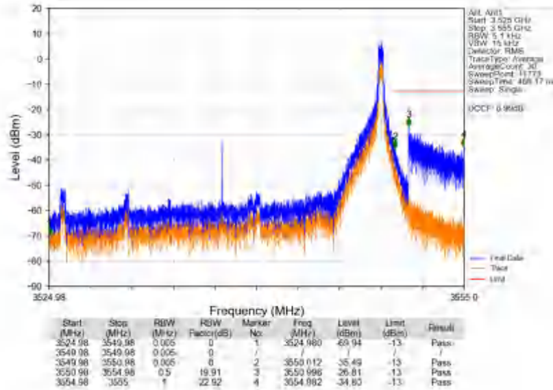
n78e_30kHz_SISO_NTV_25MHz_CP-OFDM QPSK_3537.48MHz_Edge_1RB_Right
