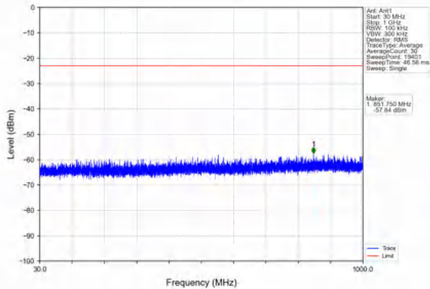
n78e_30kHz_SISO_NTNV_40MHz_DFT-s-OFDM PI/2 BPSK_3470.01MHz_Edge_1RB_Left
