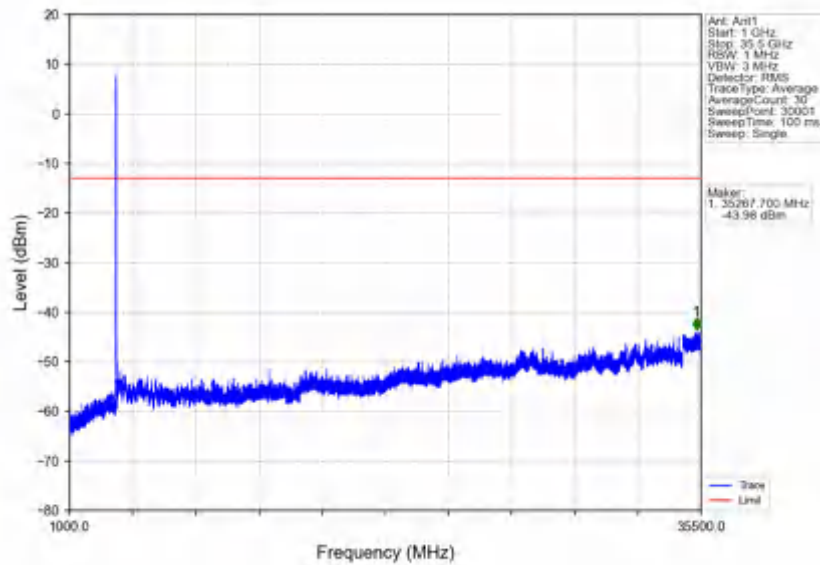
n78e_30kHz_SISO_NTNV_20MHz_DFT-s-OFDM QPSK_3540MHz_Inner_1RB_Right
