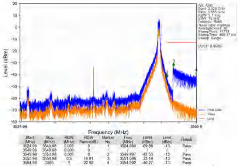
n78e_30kHz_SISO_NTNV_25MHz_DFT-s-OFDM QPSK_3537.48MHz_Inner_1RB_Right
