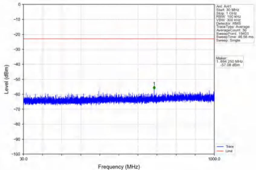
n78e_30kHz_SISO_NTV_25MHz_CP-OFDM QPSK_3462.51MHz_Edge_1RB_Left
