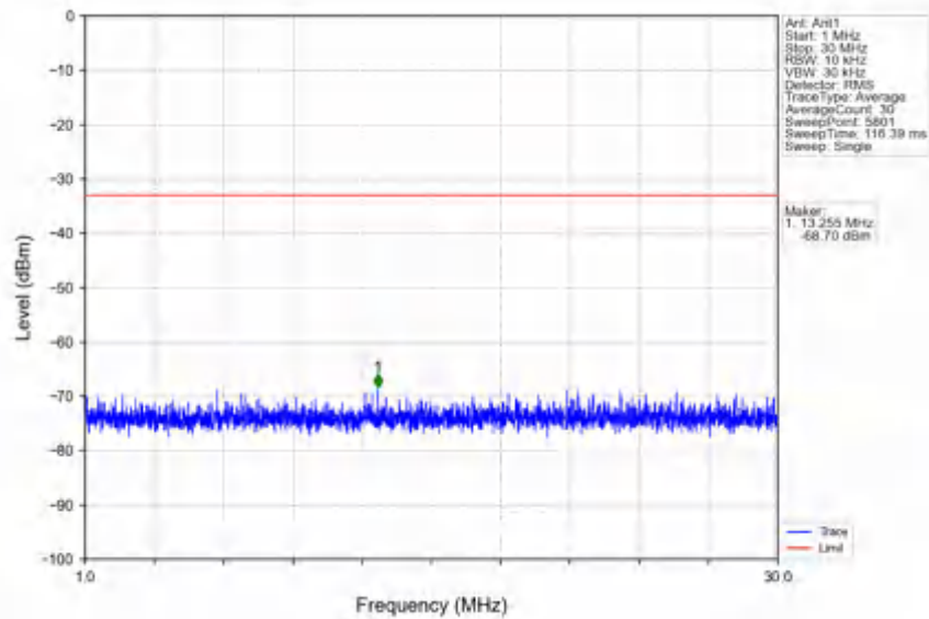
n78e_30kHz_SISO_NTNV_25MHz_DFT-s-OFDM PI/2 BPSK_3537.48MHz_Edge_1RB_Right
