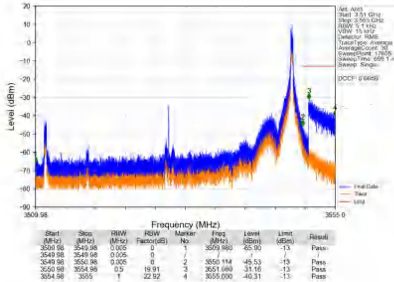
n78e_30kHz_SISO_NTNV_40MHz_DFT-s-OFDM PI/2 BPSK_3529.98MHz_Inner_1RB_Right
