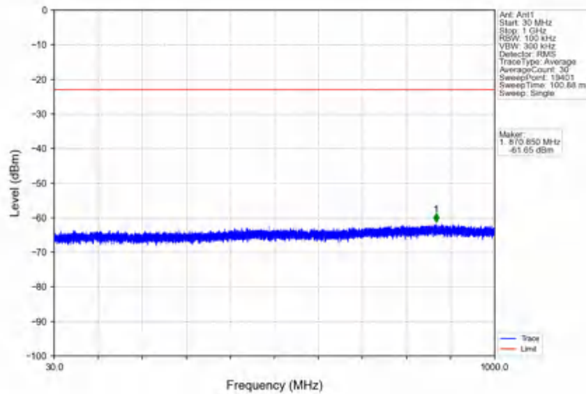
n78e_30kHz_SISO_NTNV_40MHz_DFT-s-OFDM PI/2 BPSK_3529.98MHz_Outer_Full
