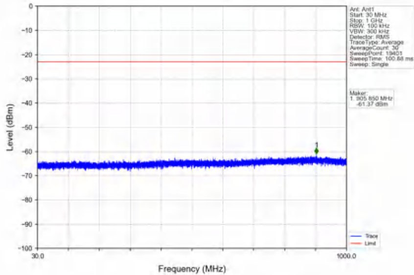
n78e_30kHz_SISO_NTNV_30MHz_DFT-s-OFDM PI/2 BPSK_3534.99MHz_Outer_Full
