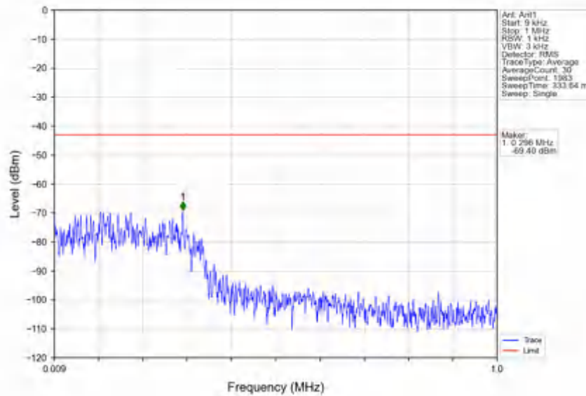
n78e_30kHz_SISO_NTNV_40MHz_DFT-s-OFDM_QPSK_3470.01MHz_Edge_1RB_Left
