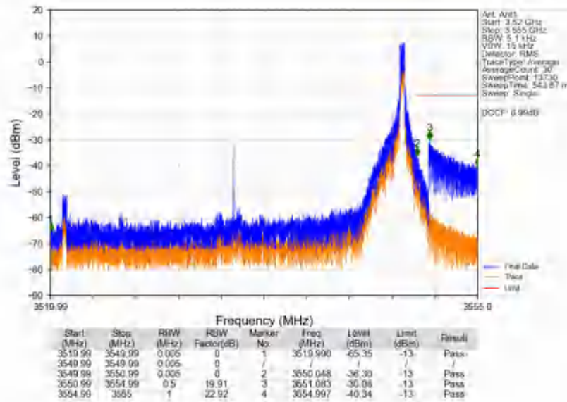
n78e_30kHz_SISO_NTNV_30MHz_DFT-s-OFDM QPSK_3534.99MHz_Edge_1RB_Right
