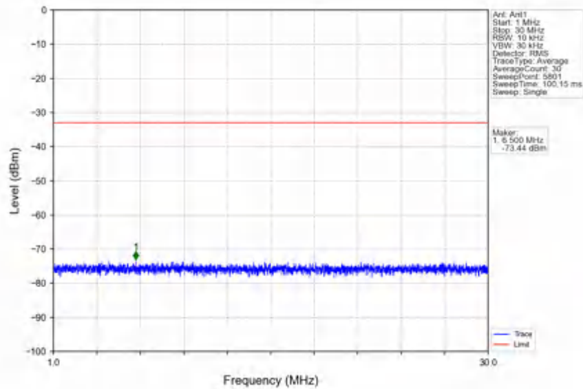
n78e_30kHz_SISO_NTV_50MHz_DFT-s-OFDM PI/2 BPSK_3525MHz_Inner_1RB_Right
