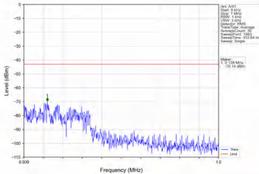
n78e_30kHz_SISO_NTNV_25MHz_DFT-s-OFDM PI/2 BPSK_3500.01MHz_Edge_1RB_Left
