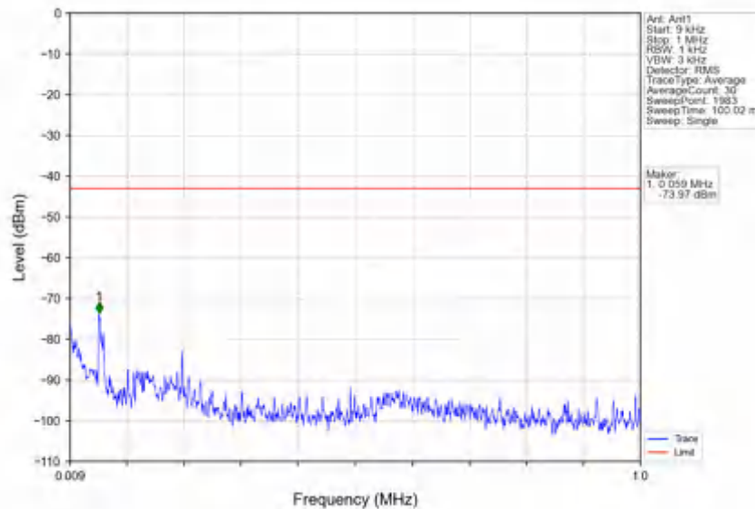
n78e_30kHz_SISO_NTNV_25MHz_DFT-s-OFDM_QPSK_3537.48MHz_Outer_Full
