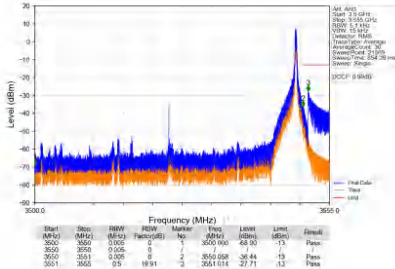
n78e_30kHz_SISO_NTV_50MHz_DFT-s-OFDM PI/2 BPSK_3525MHz_Edge_1RB_Right
