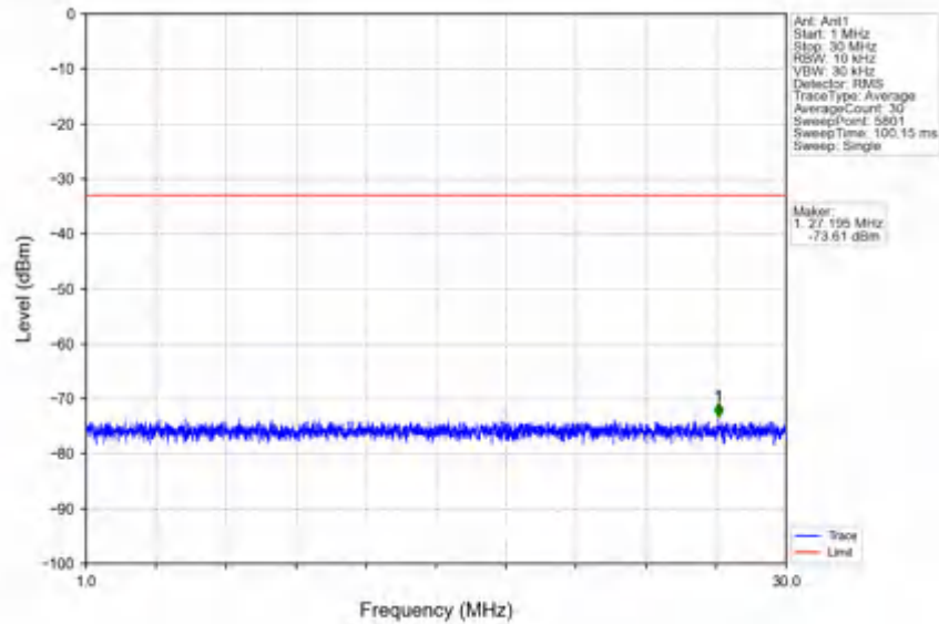
n78e_30kHz_SISO_NTNV_30MHz_DFT-s-OFDM PI/2 BPSK_3534.99MHz_Inner_1RB_Right
