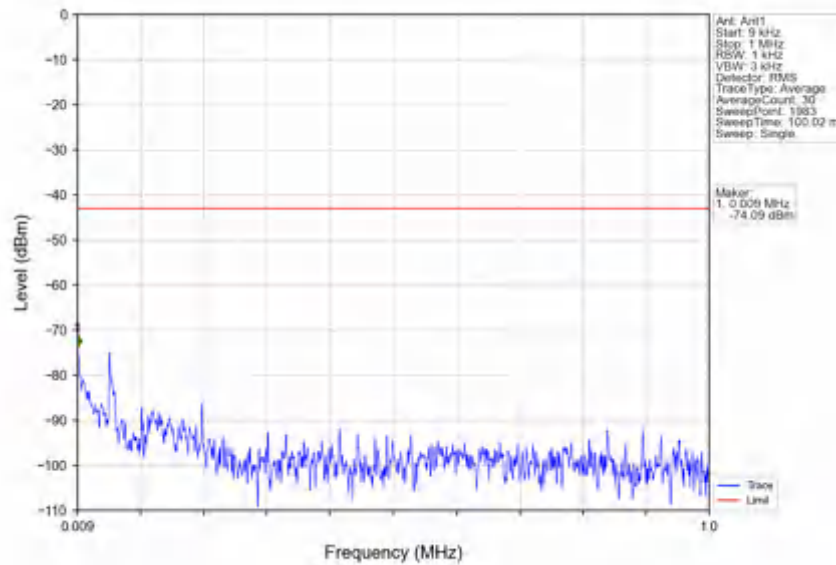
n78e_30kHz_SISO_NTNV_20MHz_DFT-s-OFDM PI/2 BPSK_3460.02MHz_Outer_Full
