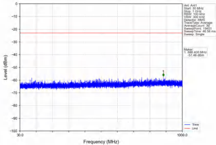
n78e_30kHz_SISO_NTVV_40MHz_CP-OFDM QPSK_3500.01MHz_Edge_1RB_Left
