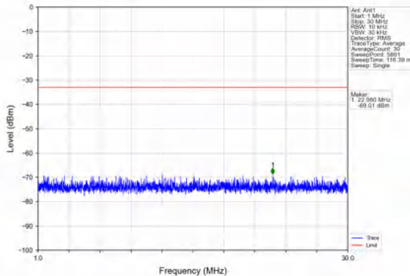
n78e_30kHz_SISO_NTNV_40MHz_DFT-s-OFDM PI/2 BPSK_3500.01MHz_Edge_1RB_Left
