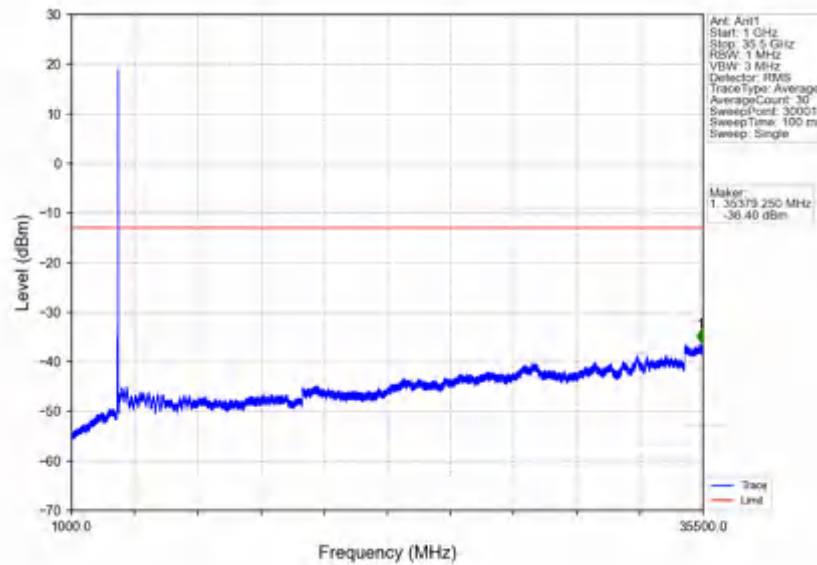
n78e_30kHz_SISO_NTNV_30MHz_DFT-s-OFDM PI/2 BPSK_3534.99MHz_Outer_Full
