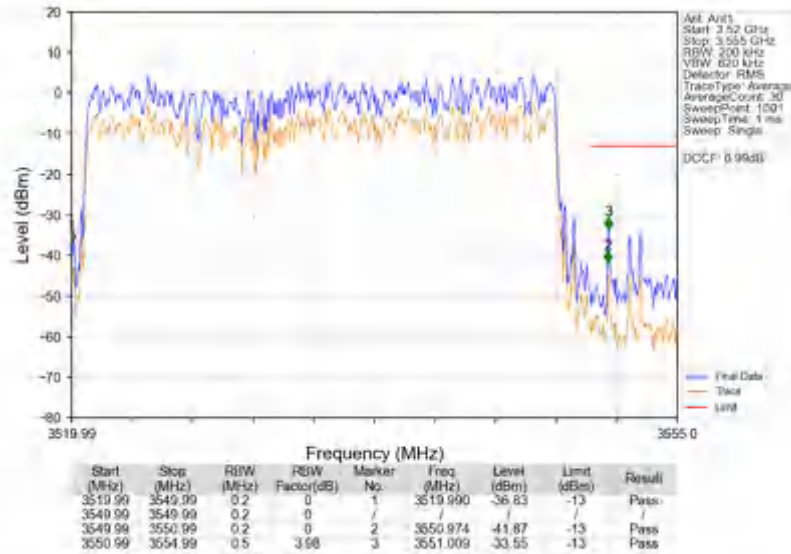
n78e_30kHz_SISO_NTNV_30MHz_DFT-s-OFDM PI/2 BPSK_3534.99MHz_Outer_Full
