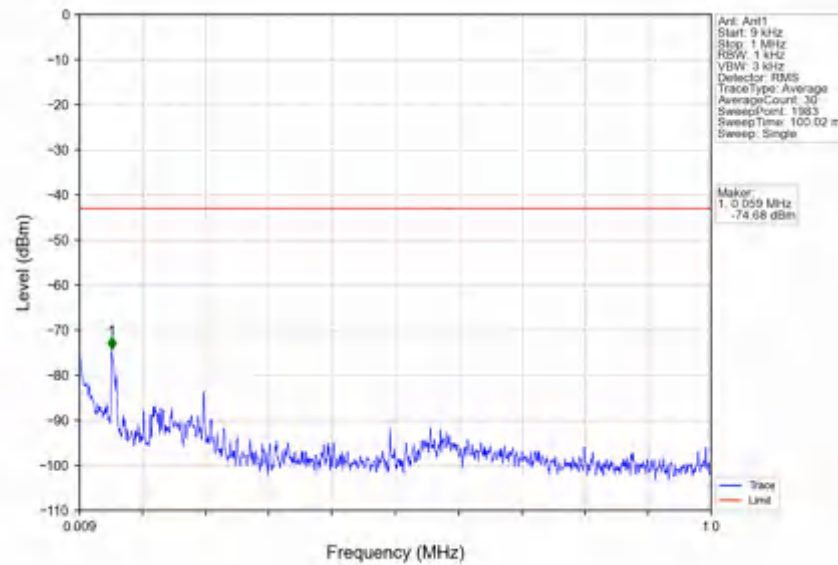
n78e_30kHz_SISO_NTNV_50MHz_DFT-s-OFDM PI/2 BPSK_3475.02MHz_Outer_Full
