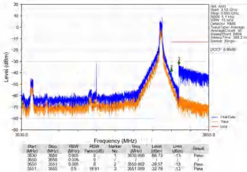
n78e_30kHz_SISO_NTNV_20MHz_DFT-s-OFDM QPSK_3540MHz_Inner_1RB_Right
