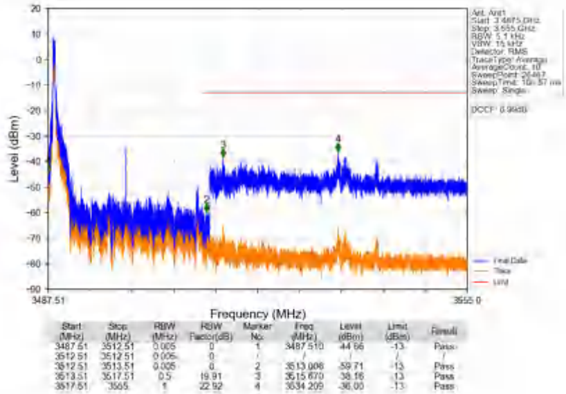
n78e_30kHz_SISO_NTV_25MHz_CP-OFDM QPSK_3500.01MHz_Edge_1RB_Left
