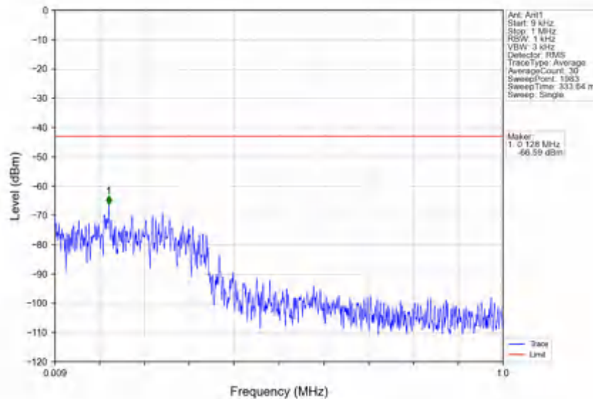
n78e_30kHz_SISO_NTNV_30MHz_DFT-s-OFDM QPSK_3500.01MHz_Edge_1RB_Left
