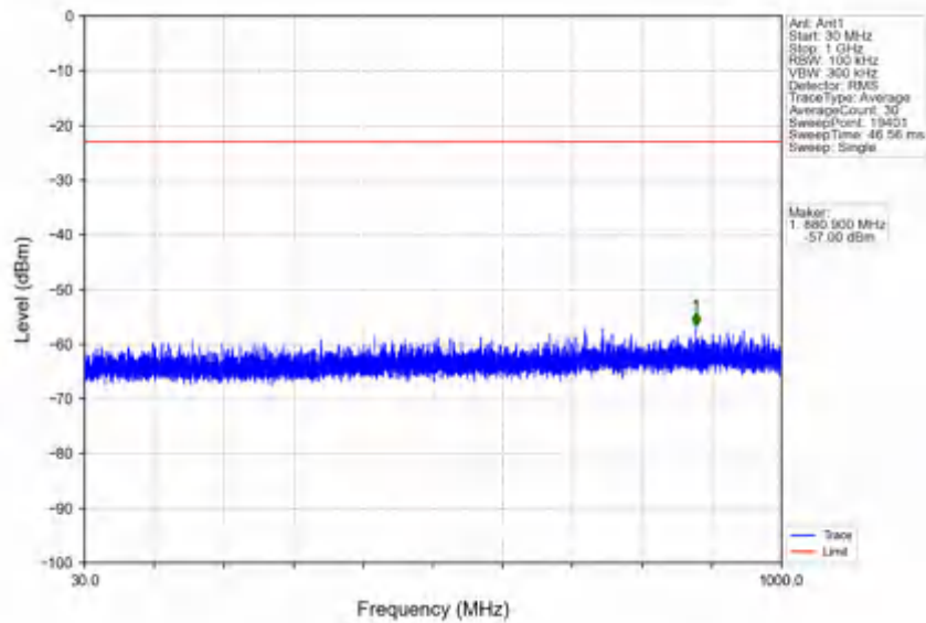
n78e_30kHz_SISO_NTNV_20MHz_DFT-s-OFDM_QPSK_3460.02MHz_Edge_1RB_Left
