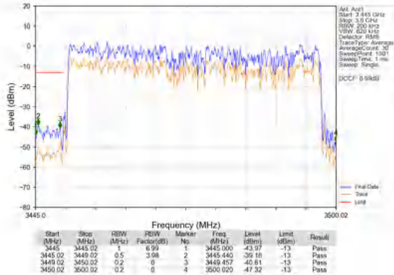
n78e_30kHz_SISO_NTNV_50MHz_DFT-s-OFDM_QPSK_3475.02MHz_Outer_Full
