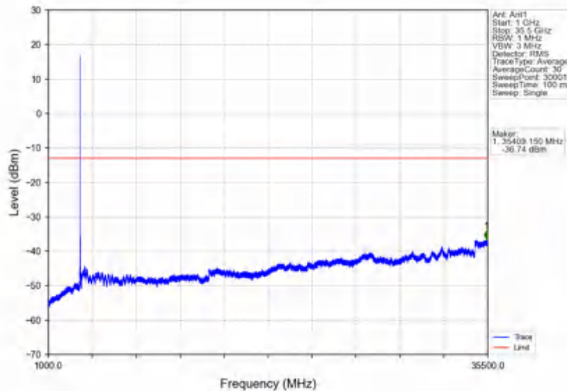
n78e_30kHz_SISO_NTVV_30MHz_CP-OFDM QPSK_3500.01MHz_Edge_1RB_Left
