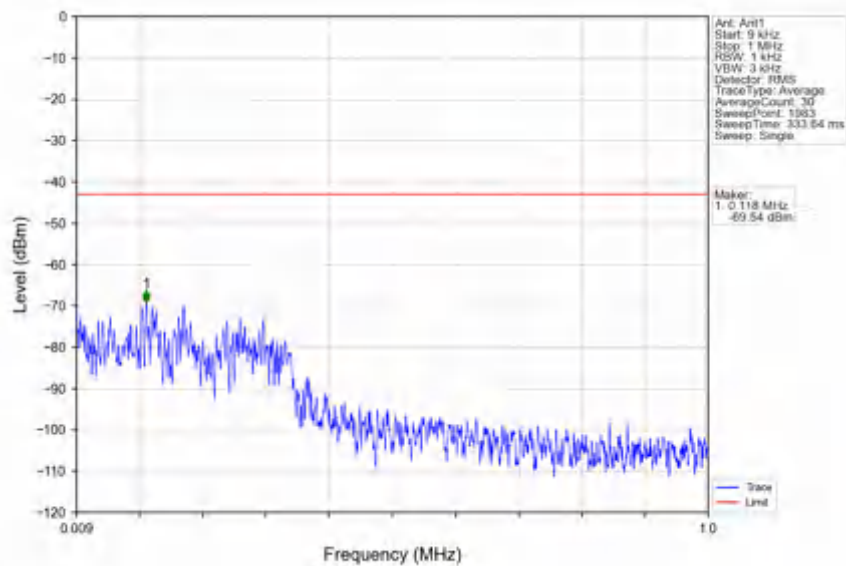
n78e_30kHz_SISO_NTNV_30MHz_DFT-s-OFDM PI/2 BPSK_3465MHz_Edge_1RB_Left
