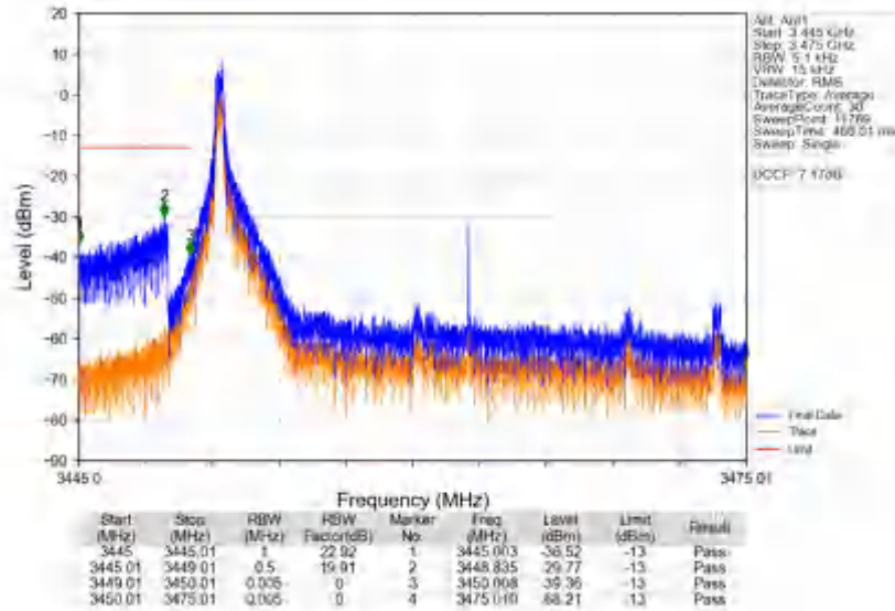
n78e_30kHz_SISO_NTV_25MHz_CP-OFDM_QPSK_3462.51MHz_Inner_1RB_Left
