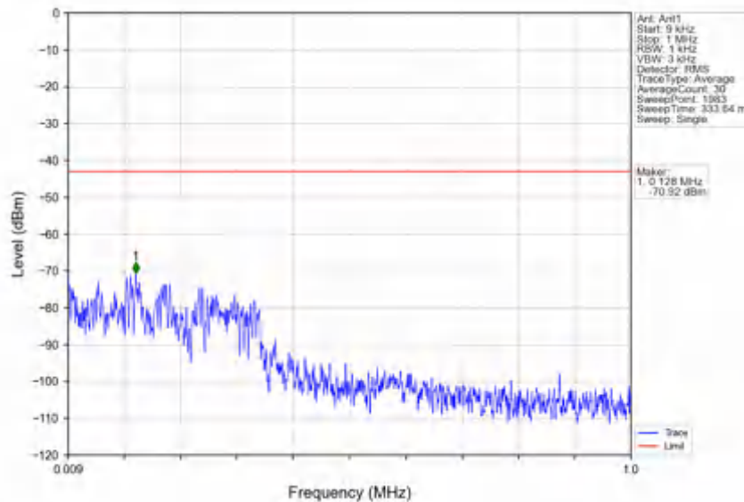
n78e_30kHz_SISO_NTNV_40MHz_DFT-s-OFDM PI/2 BPSK_3529.98MHz_Edge_1RB_Right
