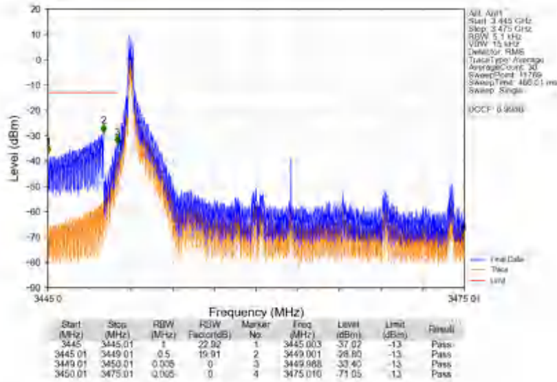
n78e_30kHz_SISO_NTNV_25MHz_DFT-s-OFDM PI/2 BPSK_3462.51MHz_Edge_1RB_Left
