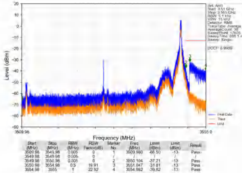
n78e_30kHz_SISO_NTV_40MHz_CP-OFDM QPSK_3529.98MHz_Edge_1RB_Right
