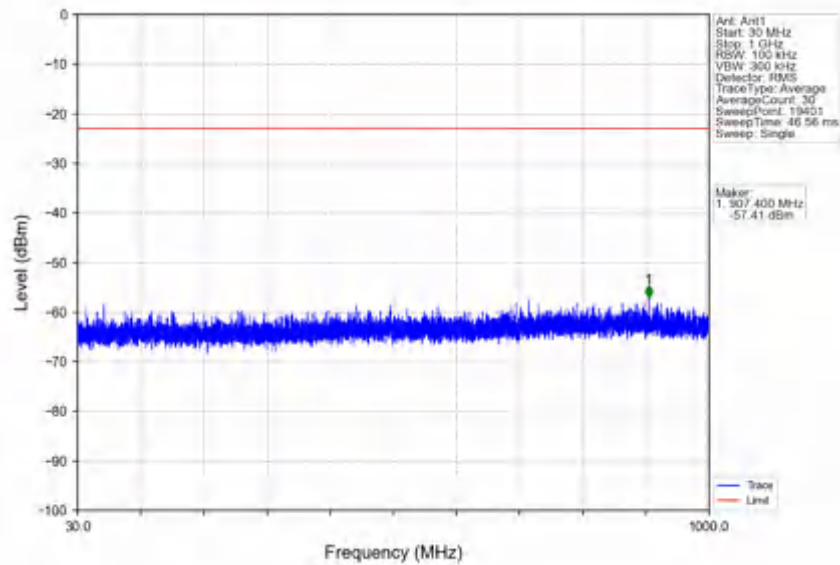
n78e_30kHz_SISO_NTNV_25MHz_DFT-s-OFDM QPSK_3462.51MHz_Edge_1RB_Left
