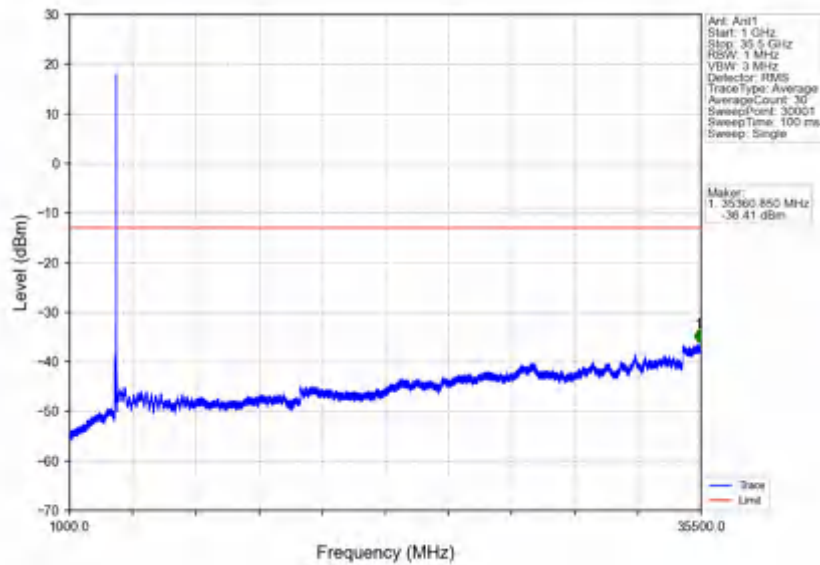
n78e_30kHz_SISO_NTNV_50MHz_DFT-s-OFDM QPSK_3475.02MHz_Edge_1RB_Left
