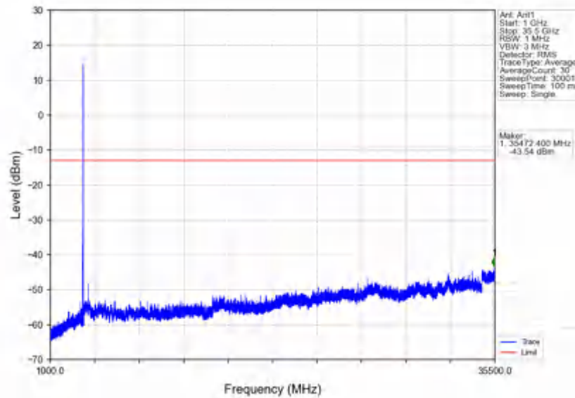
n78e_30kHz_SISO_NTV_20MHz_DFT-s-OFDM QPSK_3540MHz_Edge_1RB_Right
