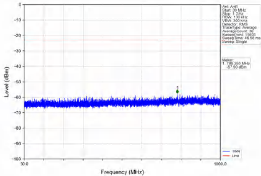
n78e_30kHz_SISO_NTNV_50MHz_DFT-s-OFDM PI/2 BPSK_3500.01MHz_Edge_1RB_Left
