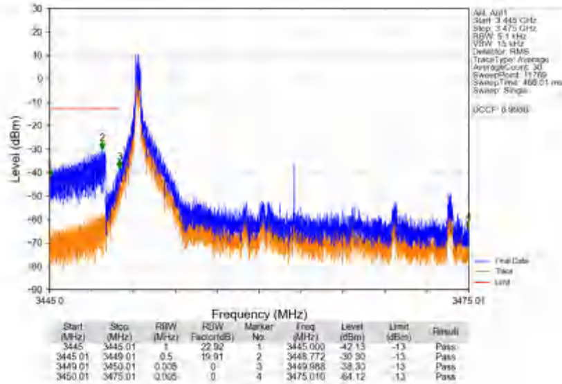
n78e_30kHz_SISO_NTNV_25MHz_DFT-s-OFDM PI/2 BPSK_3462.51MHz_Inner_1RB_Left
