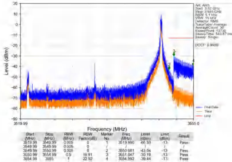
n78e_30kHz_SISO_NTV_30MHz_DFT-s-OFDM PI/2 BPSK_3534.99MHz_Inner_1RB_Right
