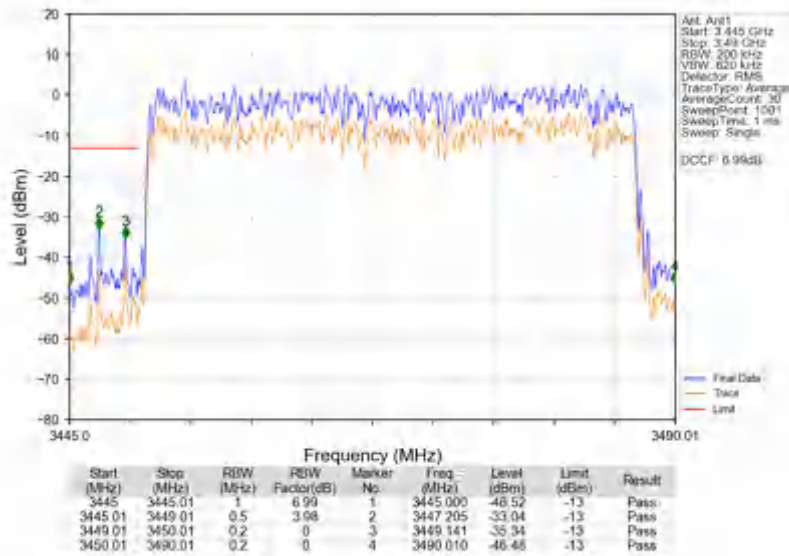
n78e_30kHz_SISO_NTNV_40MHz_DFT-s-OFDM PI/2 BPSK_3470.01MHz_Outer_Full
