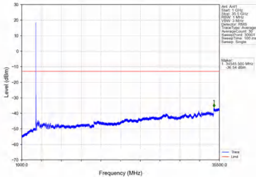
n78e_30kHz_SISO_NTV_40MHz_CP-OFDM QPSK_3470.01MHz_Outer_Full
