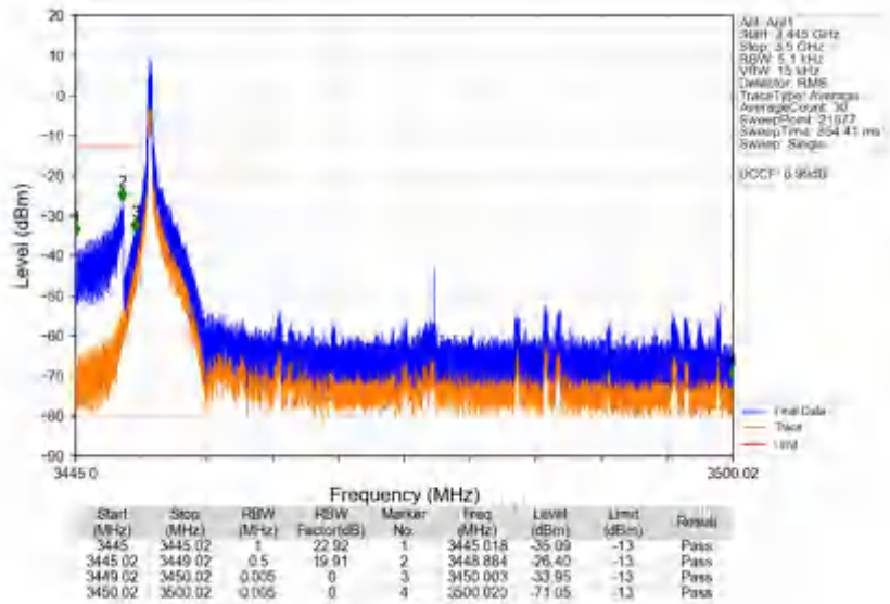
n78e_30kHz_SISO_NTNV_50MHz_DFT-s-OFDM QPSK_3475.02MHz_Edge_1RB_Left
