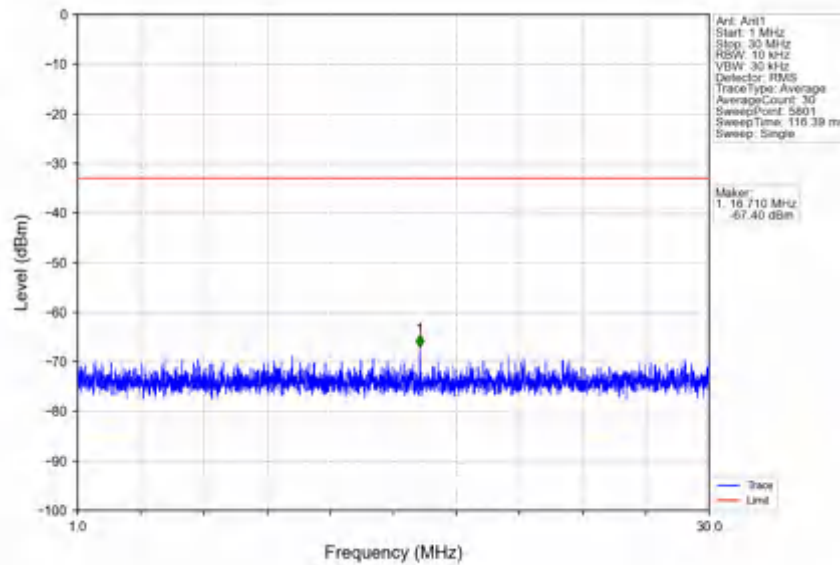
n78e_30kHz_SISO_NTNV_30MHz_DFT-s-OFDM PI/2 BPSK_3534.99MHz_Edge_1RB_Right
