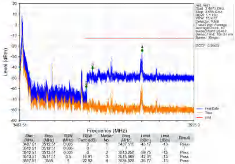
n78e_30kHz_SISO_NTNV_25MHz_DFT-s-OFDM PI/2 BPSK_3500.01MHz_Edge_1RB_Left
