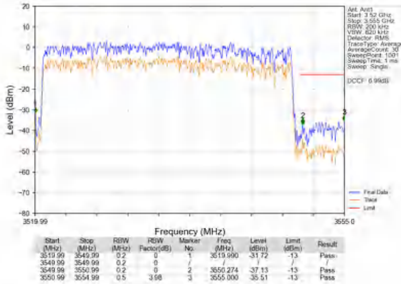
n78e_30kHz_SISO_NTNV_30MHz_CP-OFDM QPSK_3534.99MHz_Outer_Full
