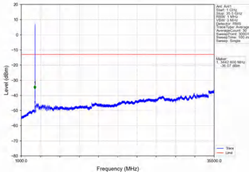
n78e_30kHz_SISO_NTNV_25MHz_CP-OFDM QPSK_3462.51MHz_Outer_Full
