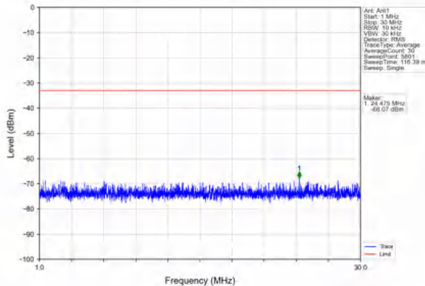
n78e_30kHz_SISO_NTNV_20MHz_DFT-s-OFDM QPSK_3460.02MHz_Edge_1RB_Left
