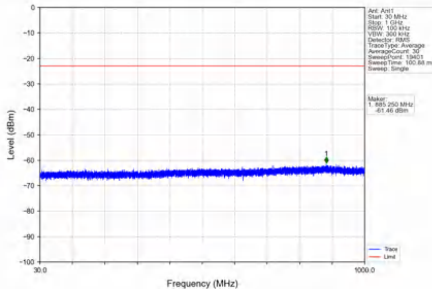
n78e_30kHz_SISO_NTNV_40MHz_DFT-s-OFDM PI/2 BPSK_3470.01MHz_Inner_1RB_Left
