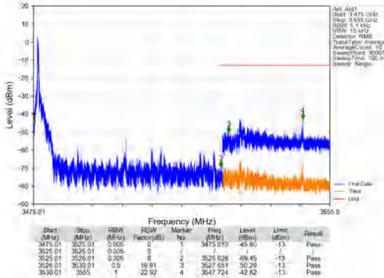
n78e_30kHz_SISO_NTNV_50MHz_DFT-s-OFDM PI/2 BPSK_3500.01MHz_Edge_1RB_Left
