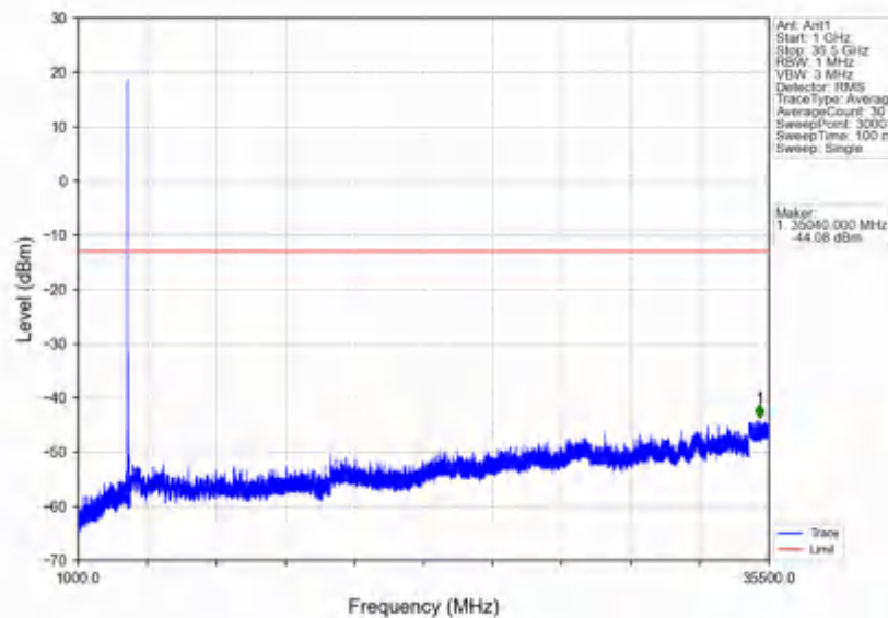
n78e_30kHz_SISO_NTV_20MHz_DFT-s-OFDM_QPSK_3460.02MHz_Inner_1RB_Left
