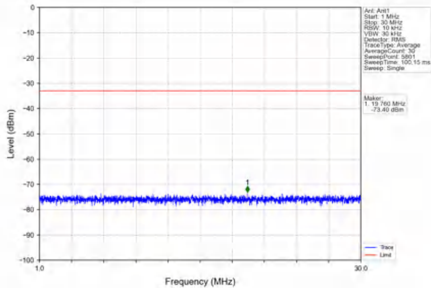
n78e_30kHz_SISO_NTV_40MHz_CP-OFDM QPSK_3529.98MHz_Inner_1RB_Right
