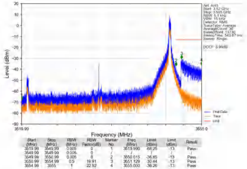
n78e_30kHz_SISO_NTNV_30MHz_DFT-s-OFDM PI/2 BPSK_3534.99MHz_Edge_1RB_Right
