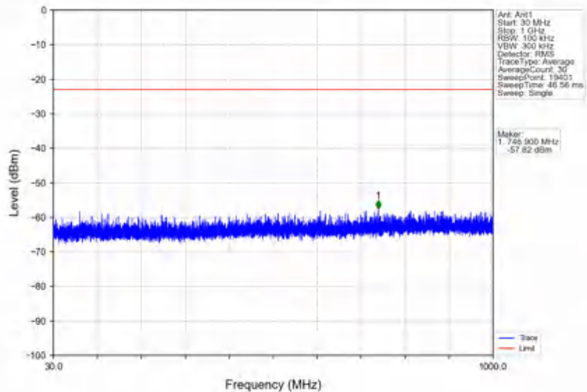
n78e_30kHz_SISO_NTNV_20MHz_DFT-s-OFDM QPSK_3500.01MHz_Edge_1RB_Left
