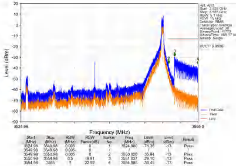
n78e_30kHz_SISO_NTNV_25MHz_DFT-s-OFDM PI/2 BPSK_3537.48MHz_Edge_1RB_Right
