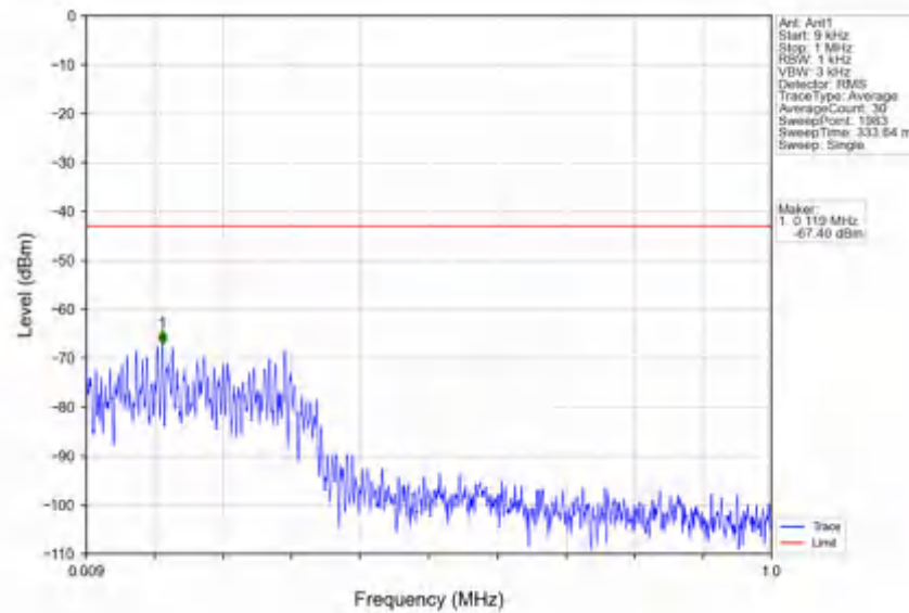
n78e_30kHz_SISO_NTV_25MHz_DFT-s-OFDM QPSK_3462.51MHz_Edge_1RB_Left
