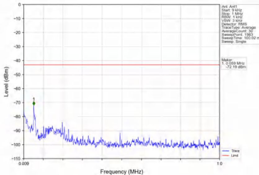
n78e_30kHz_SISO_NTNV_30MHz_DFT-s-OFDM_QPSK_3534.99MHz_Outer_Full
