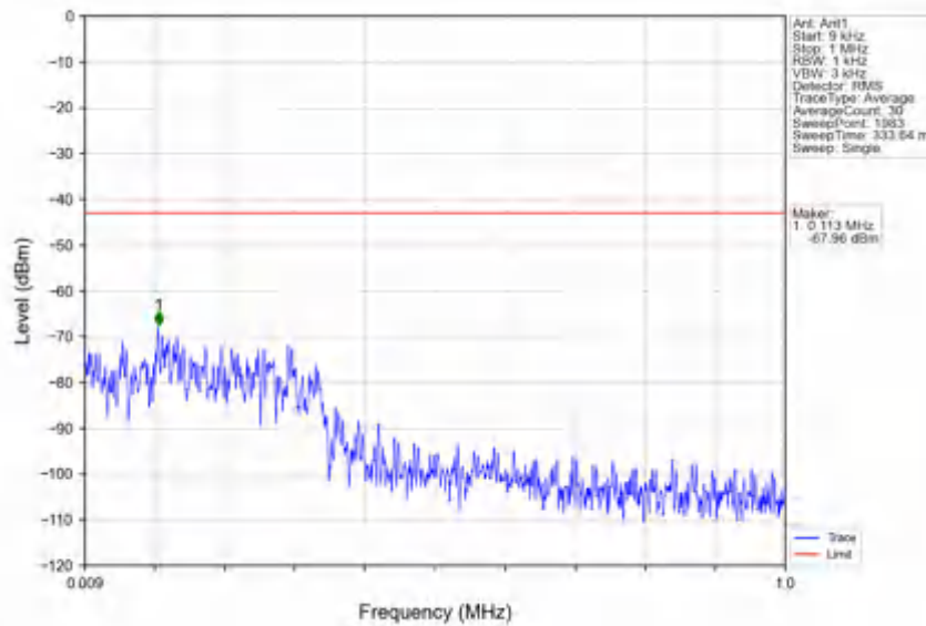
n78e_30kHz_SISO_NTNV_40MHz_DFT-s-OFDM QPSK_3500.01MHz_Edge_1RB_Left
