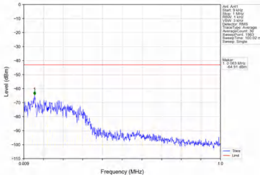
n78e_30kHz_SISO_NTV_25MHz_CP-OFDM_QPSK_3462.51MHz_Inner_1RB_Left
