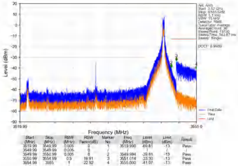
n78e_30kHz_SISO_NTNV_30MHz_DFT-s-OFDM QPSK_3534.99MHz_Inner_1RB_Right
