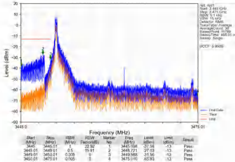
n78e_30kHz_SISO_NTV_25MHz_CP-OFDM_QPSK_3462.51MHz_Edge_1RB_Left
