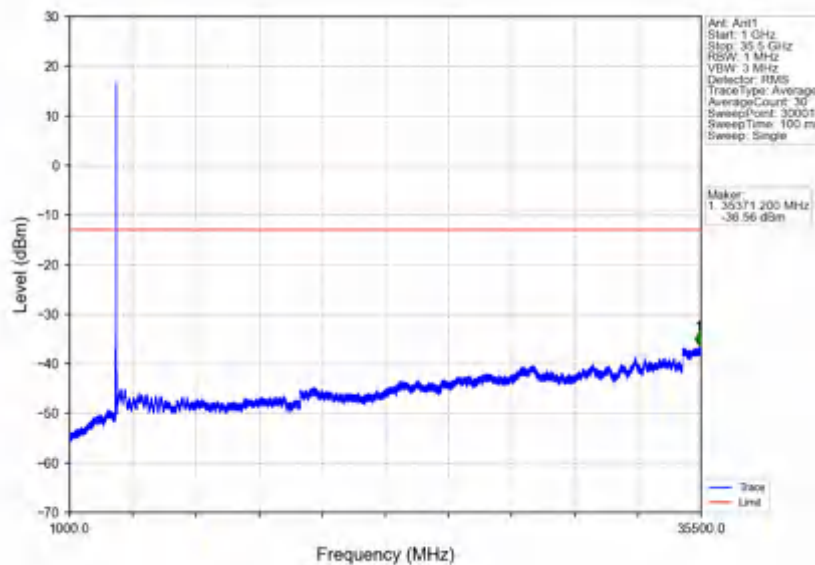
n78e_30kHz_SISO_NTNV_25MHz_DFT-s-OFDM QPSK_3537.48MHz_Edge_1RB_Right
