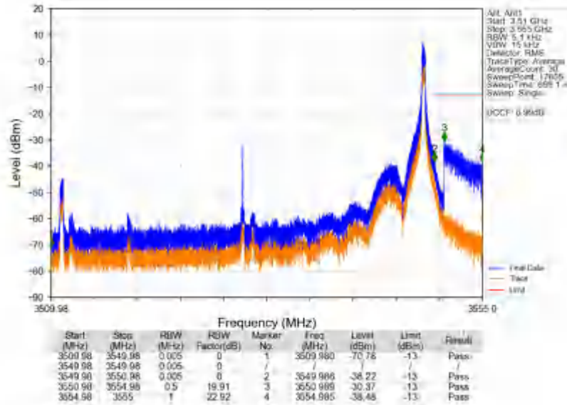
n78e_30kHz_SISO_NTNV_40MHz_DFT-s-OFDM PI/2 BPSK_3529.98MHz_Edge_1RB_Right
