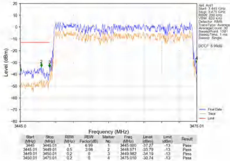
n78e_30kHz_SISO_NTV_25MHz_CP-OFDM QPSK_3462.51MHz_Outer_Full
