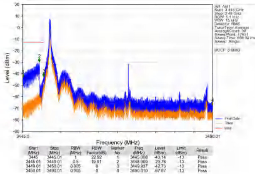
n78e_30kHz_SISO_NTNV_40MHz_DFT-s-OFDM PI/2 BPSK_3470.01MHz_Inner_1RB_Left
