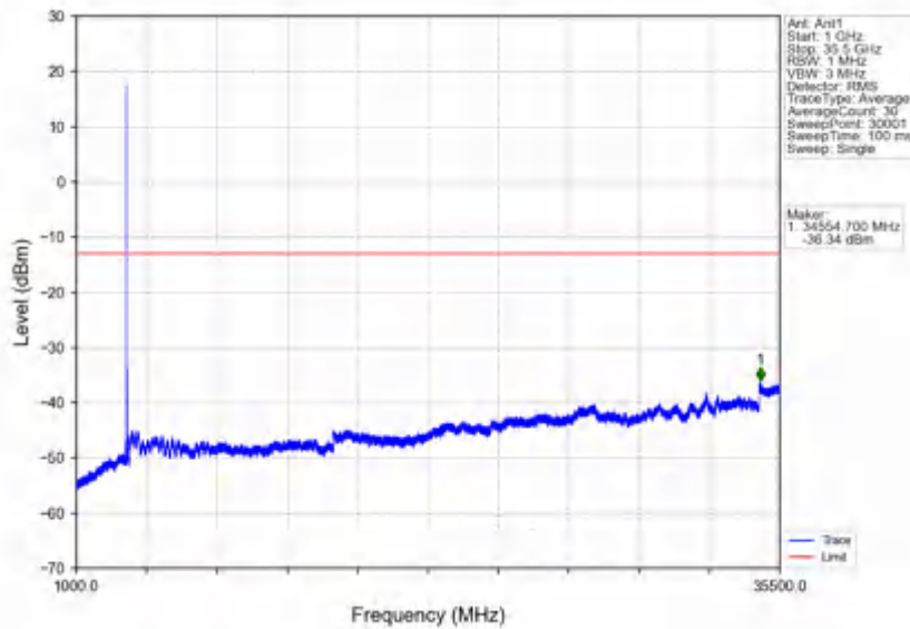
n78e_30kHz_SISO_NTNV_40MHz_DFT-s-OFDM PI/2 BPSK_3500.01MHz_Edge_1RB_Left
