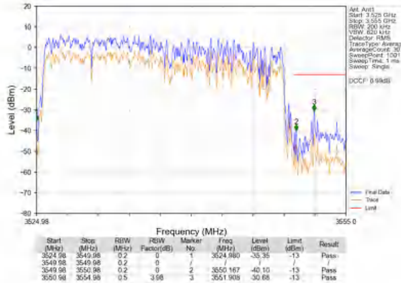
n78e_30kHz_SISO_NTNV_25MHz_DFT-s-OFDM_QPSK_3537.48MHz_Outer_Full
