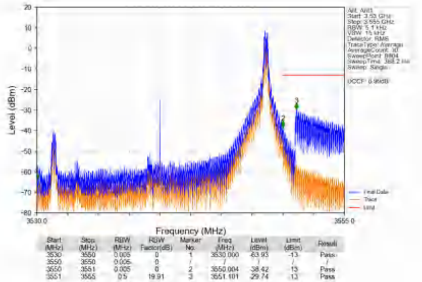
n78e_30kHz_SISO_NTV_20MHz_DFT-s-OFDM PI/2 BPSK_3540MHz_Inner_1RB_Right
