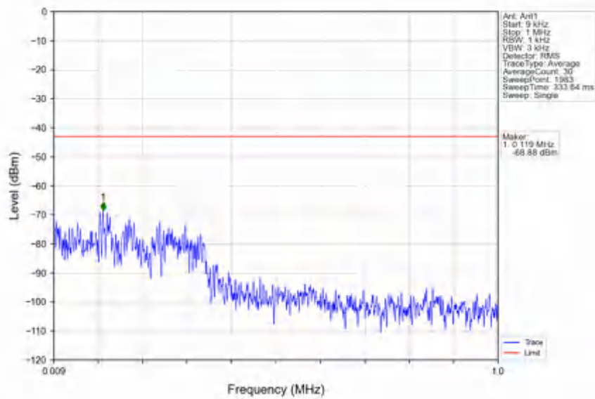
n78e_30kHz_SISO_NTNV_25MHz_DFT-s-OFDM PI/2 BPSK_3462.51MHz_Edge_1RB_Left
