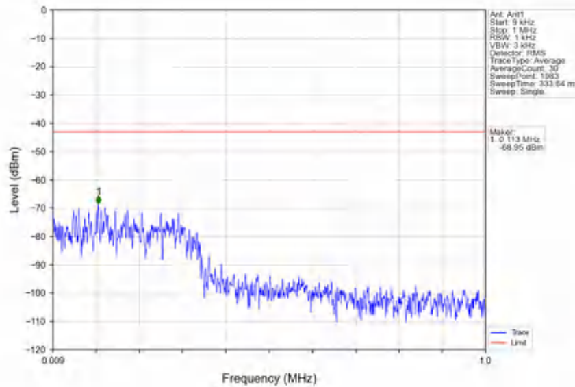
n78e_30kHz_SISO_NTNV_25MHz_DFT-s-OFDM QPSK_3537.48MHz_Edge_1RB_Right
