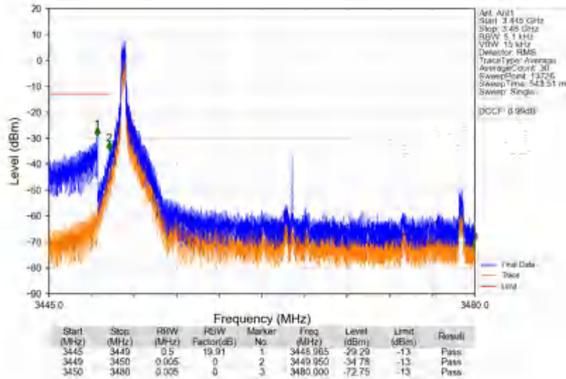
n78e_30kHz_SISO_NTV_30MHz_DFT-s-OFDM QPSK_3465MHz_Edge_1RB_Left
