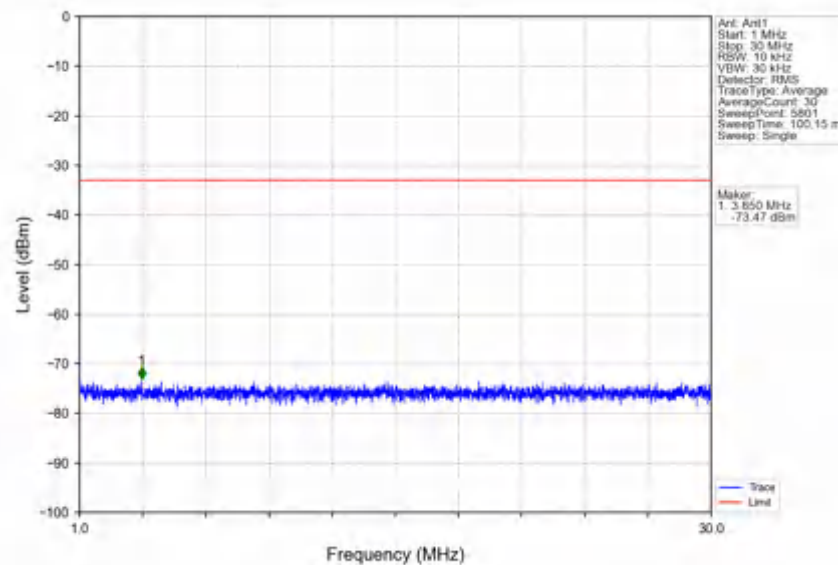
n78e_30kHz_SISO_NTNV_25MHz_DFT-s-OFDM PI/2 BPSK_3462.51MHz_Outer_Full
