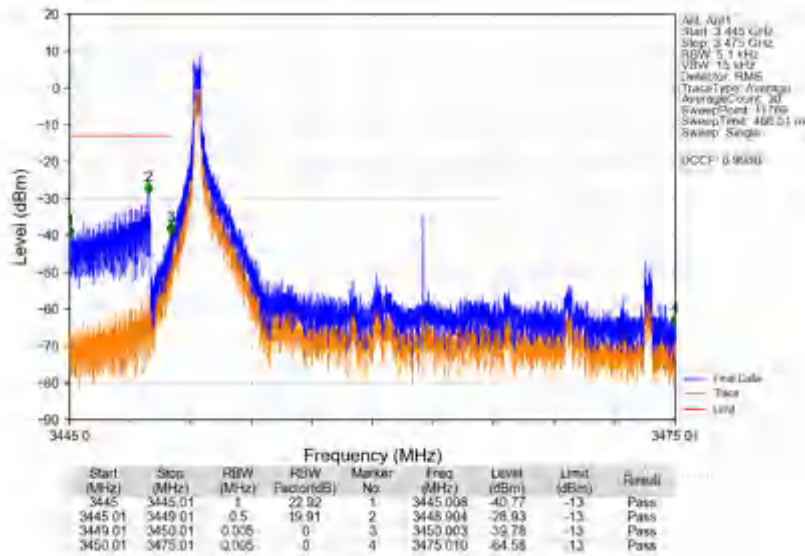
n78e_30kHz_SISO_NTNV_25MHz_DFT-s-OFDM_QPSK_3462.51MHz_Inner_1RB_Left
