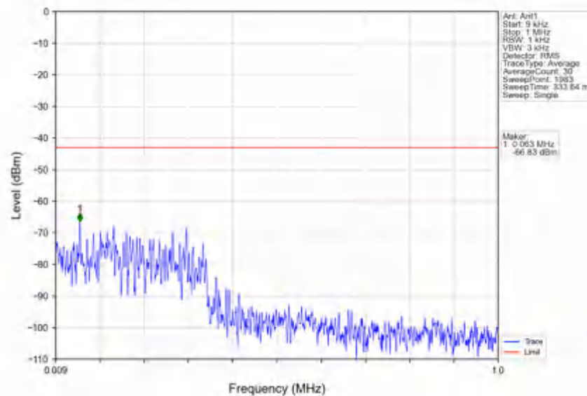
n78e_30kHz_SISO_NTNV_25MHz_DFT-s-OFDM_QPSK_3500.01MHz_Edge_1RB_Left
