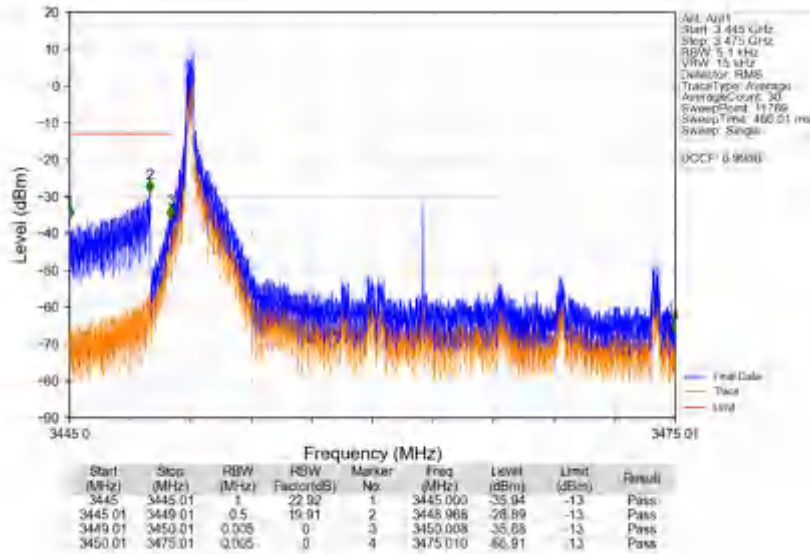
n78e_30kHz_SISO_NTNV_25MHz_DFT-s-OFDM QPSK_3462.51MHz_Edge_1RB_Left
