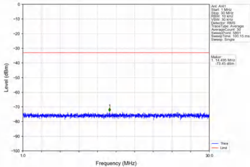
n78e_30kHz_SISO_NTNV_40MHz_DFT-s-OFDM PI/2 BPSK_3529.98MHz_Inner_1RB_Right
