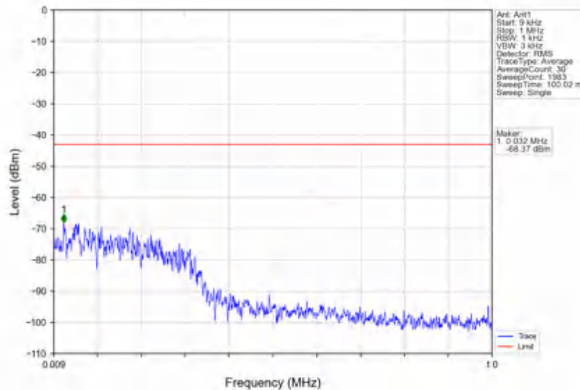
n78e_30kHz_SISO_NTV_30MHz_CP-OFDM QPSK_3534.99MHz_Inner_1RB_Right
