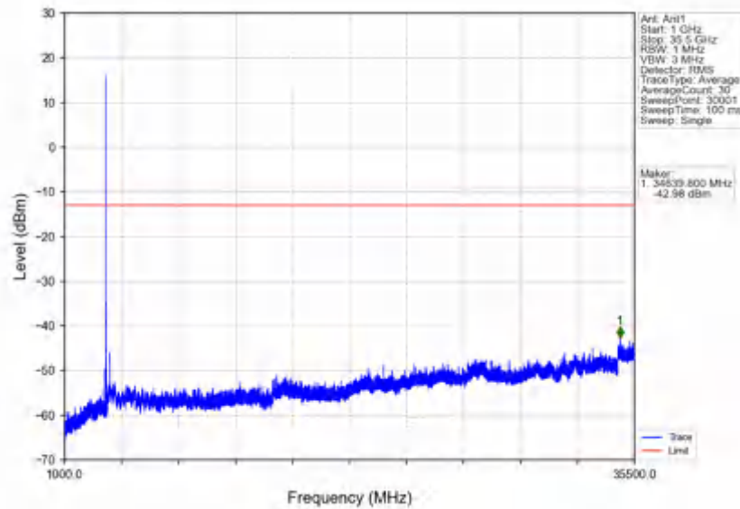
n78e_30kHz_SISO_NTV_20MHz_DFT-s-OFDM QPSK_3540MHz_Edge_1RB_Right
