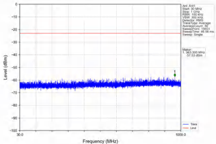
n78e_30kHz_SISO_NTNV_25MHz_DFT-s-OFDM QPSK_3500.01MHz_Edge_1RB_Left
