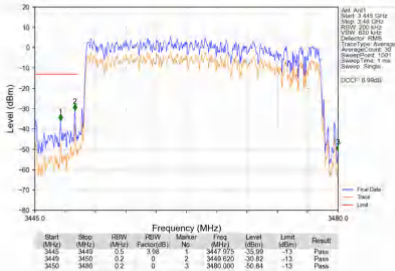
n78e_30kHz_SISO_NTNV_30MHz_DFT-s-OFDM PI/2 BPSK_3465MHz_Outer_Full
