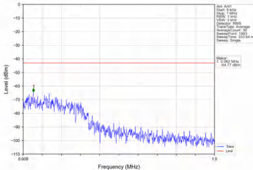
n78e_30kHz_SISO_NTV_25MHz_CP-OFDM_QPSK_3462.51MHz_Edge_1RB_Left
