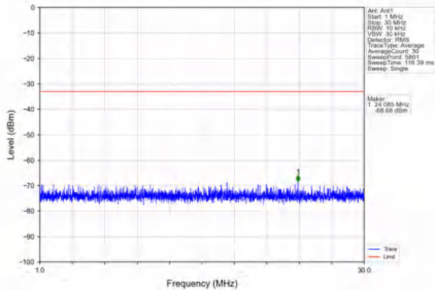
n78e_30kHz_SISO_NTNV_40MHz_DFT-s-OFDM QPSK_3500.01MHz_Edge_1RB_Left
