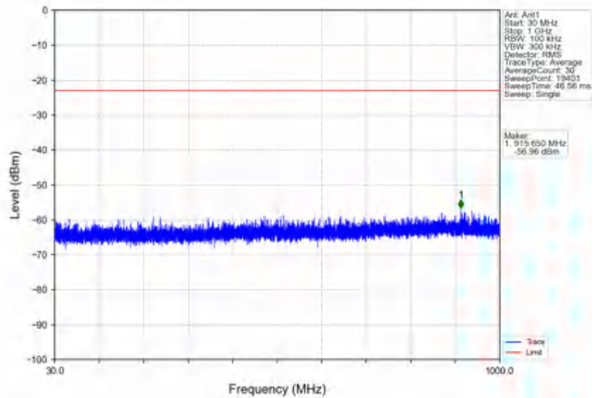
n78e_30kHz_SISO_NTNV_30MHz_DFT-s-OFDM QPSK_3534.99MHz_Edge_1RB_Right
