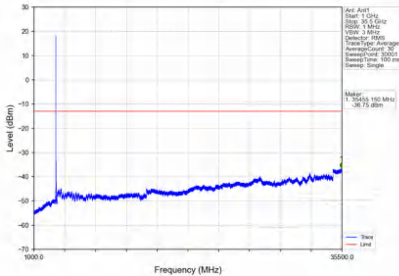
n78e_30kHz_SISO_NTV_25MHz_CP-OFDM QPSK_3500.01MHz_Edge_1RB_Left
