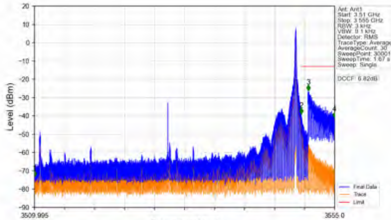
n78e_15kHz_SISO_NTNV_40MHz_DFT-s-OFDM QPSK_3529.995MHz_Inner_1RB_Right
