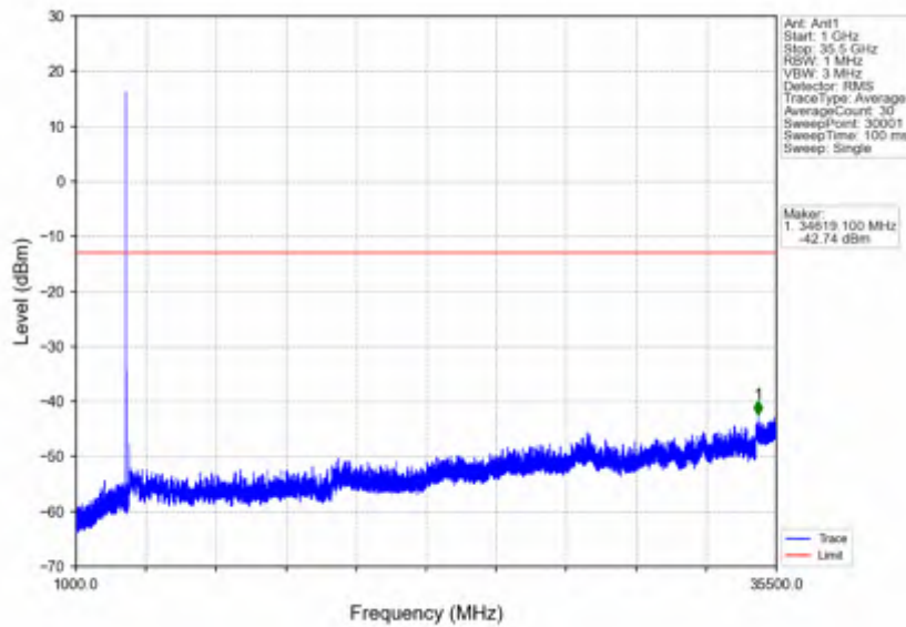
n78e_30kHz_SISO_NTNV_15MHz_DFT-s-OFDM PI/2 BPSK_3457.5MHz_Outer_Full
