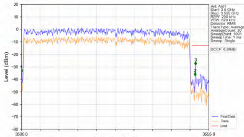
n78e_15kHz_SISO_NTNV_50MHz_CP-OFDM QPSK_3525MHz_Outer_Full
