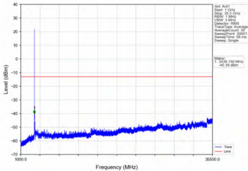
n78e_15kHz_SISO_NTNV_50MHz_DFT-s-OFDM PI/2 BPSK_3475.005MHz_Outer_Full
