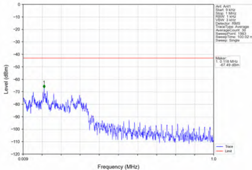
n78e_30kHz_SISO_NTNV_15MHz_DFT-s-OFDM_PI/2_BPSK_3457.5MHz_Inner_1RB_Left
