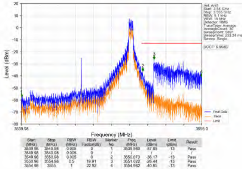
n78e_30kHz_SISO_NTNV_10MHz_DFT-s-OFDM PI/2 BPSK_3544.98MHz_Edge_1RB_Right
