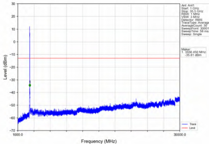
n78e_15kHz_SISO_NTNV_40MHz_CP-OFDM QPSK_3529.995MHz_Outer_Full
