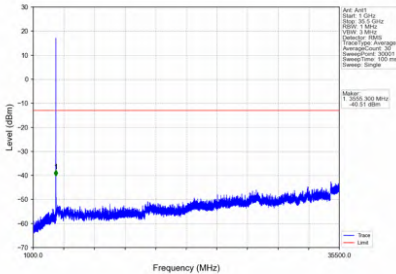
n78e_30kHz_SISO_NTNV_15MHz_DFT-s-OFDM PI/2 BPSK_3542.49MHz_Outer_Full
