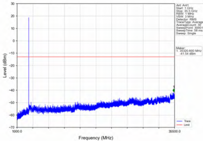
n78e_30kHz_SISO_NTNV_10MHz_DFT-s-OFDM QPSK_3455.01MHz_Edge_1RB_Left
