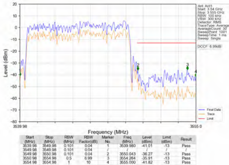
n78e_30kHz_SISO_NTNV_10MHz_DFT-s-OFDM PI/2 BPSK_3544.98MHz_Outer_Full
