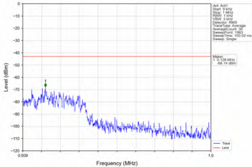
n78e_30kHz_SISO_NTNV_15MHz_DFT-s-OFDM QPSK_3542.49MHz_Inner_1RB_Right
