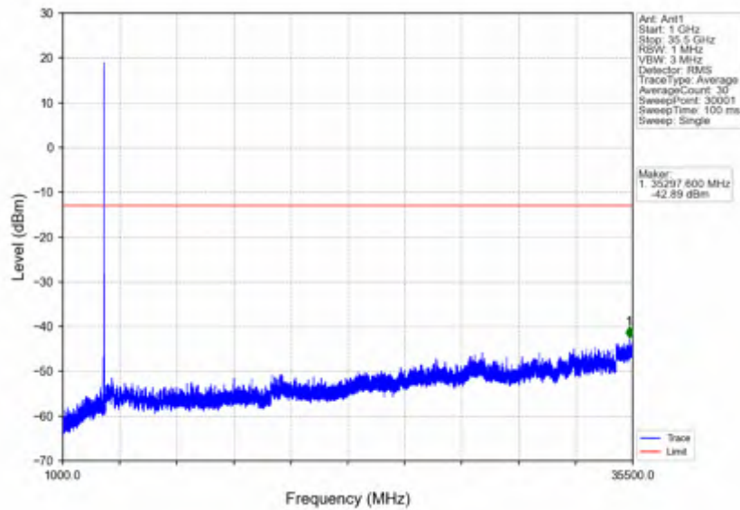
n78e_30kHz_SISO_NTNV_15MHz_DFT-s-OFDM QPSK_3542.49MHz_Edge_1RB_Right
