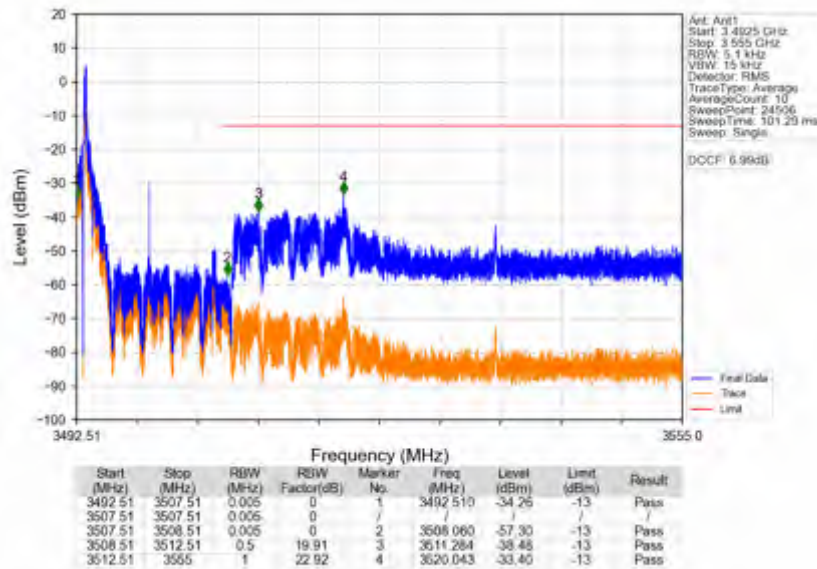
n78e_30kHz_SISO_NTNV_15MHz_CP-OFDM QPSK_3500.01MHz_Edge_1RB_Left
