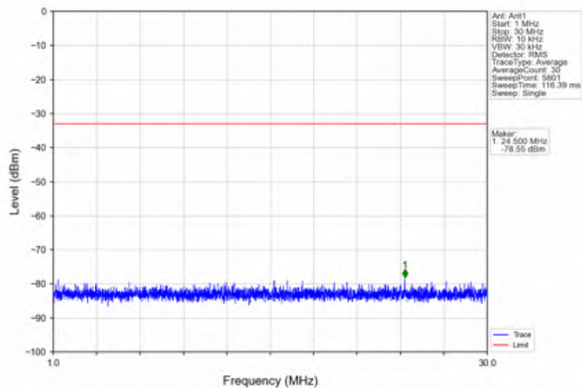
n78e_15kHz_SISO_NTNV_50MHz_CP-OFDM QPSK_3475.005MHz_Outer_Full
