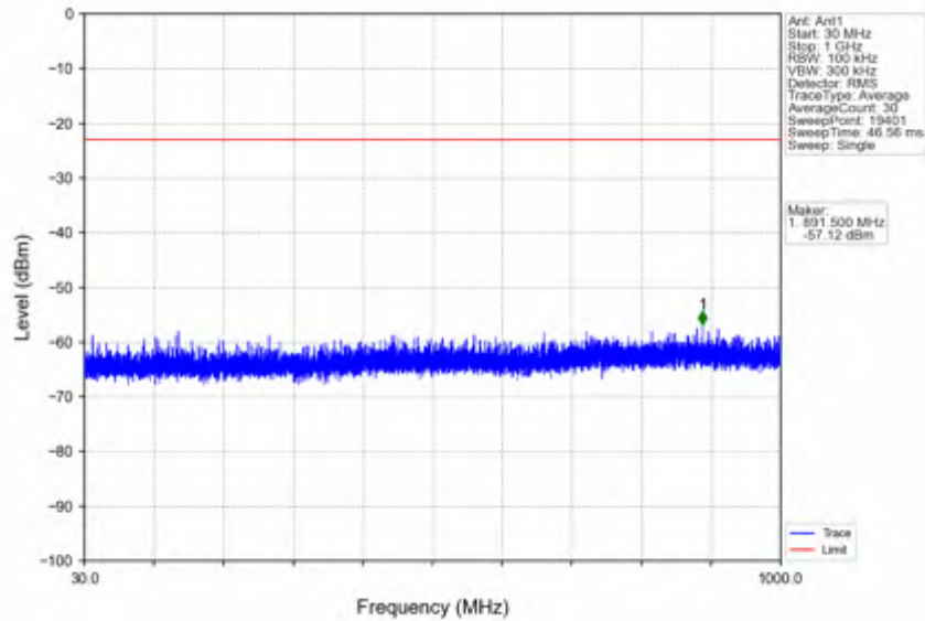
n78e_30kHz_SISO_NTNV_15MHz_DFT-s-OFDM QPSK_3542.49MHz_Edge_1RB_Right
