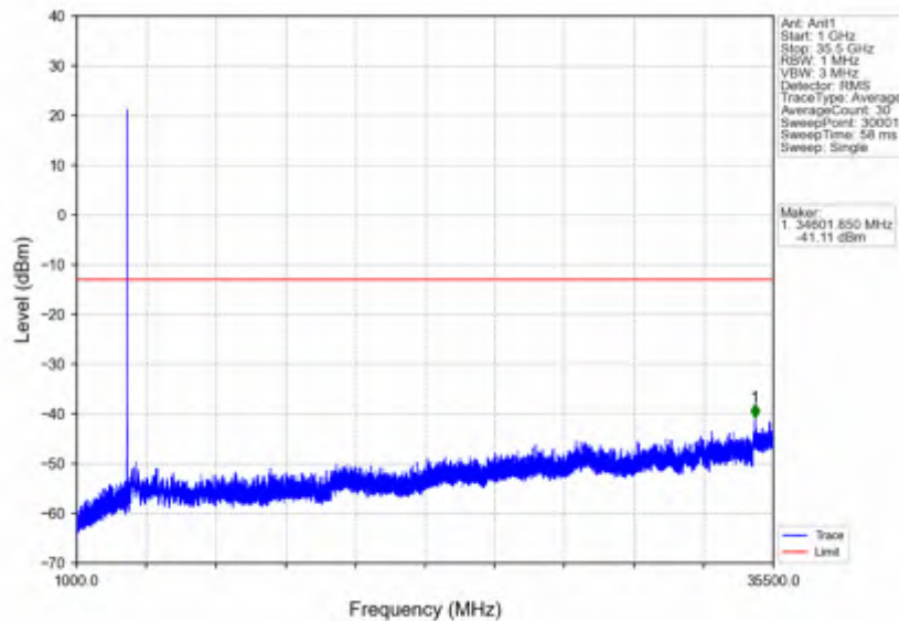
n78e_30kHz_SISO_NTNV_10MHz_DFT-s-OFDM PI/2 BPSK_3500.01MHz_Edge_1RB_Left
