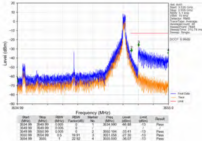
n78e_30kHz_SISO_NTNV_15MHz_DFT-s-OFDM QPSK_3542.49MHz_Edge_1RB_Right
