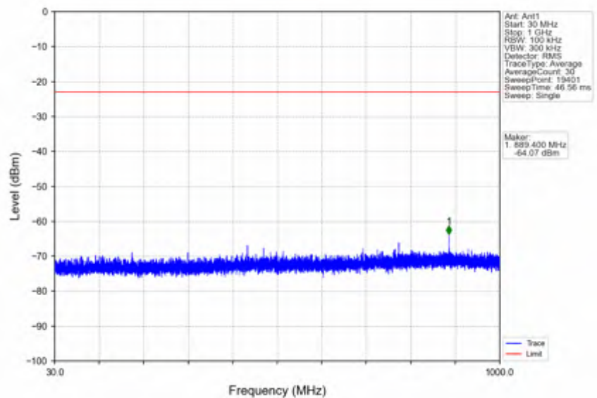
n78e_15kHz_SISO_NTVV_40MHz_CP-OFDM_QPSK_3470.01MHz_Edge_1RB_Left
