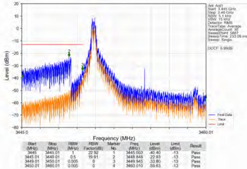
n78e_30kHz_SISO_NTV_10MHz_CP-OFDM QPSK_3455.01MHz_Edge_1RB_Left
