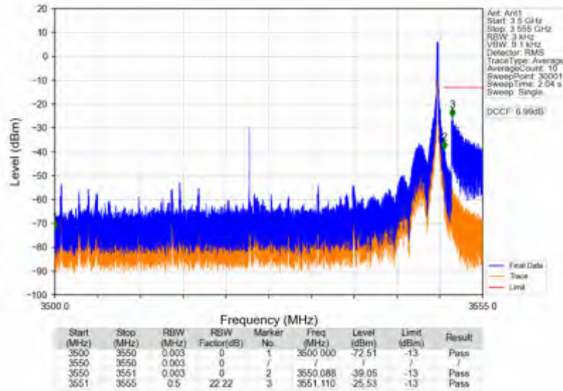
n78e_15kHz_SISO_NTNV_50MHz_DFT-s-OFDM_PI/2_BPSK_3525MHz_Edge_1RB_Right
