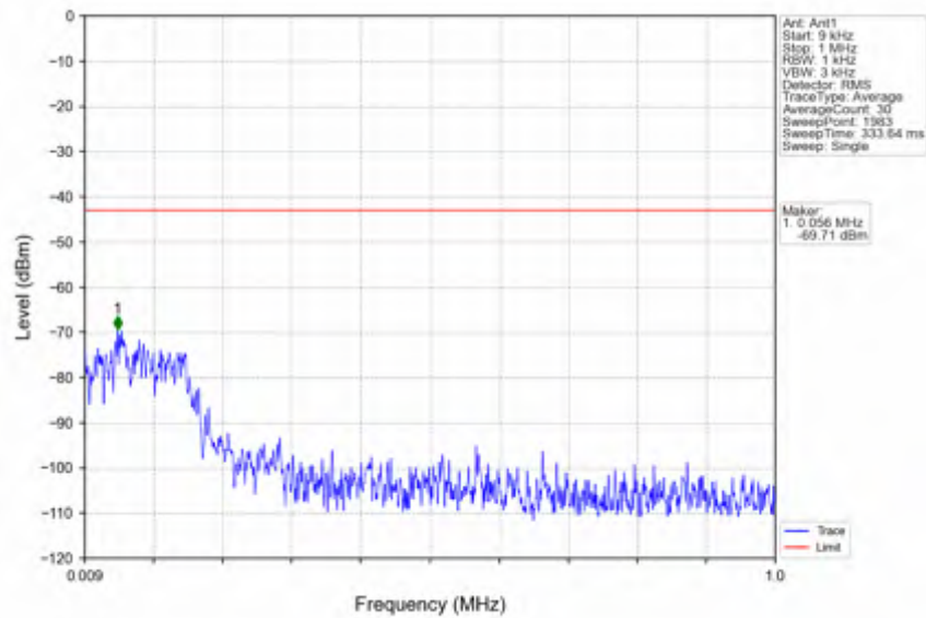
n78e_15kHz_SISO_NTV_40MHz_DFT-s-OFDM_QPSK_3529.995MHz_Inner_1RB_Right
