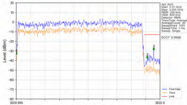
n78e_15kHz_SISO_NTV_40MHz_CP-OFDM QPSK_3529.995MHz_Outer_Full
