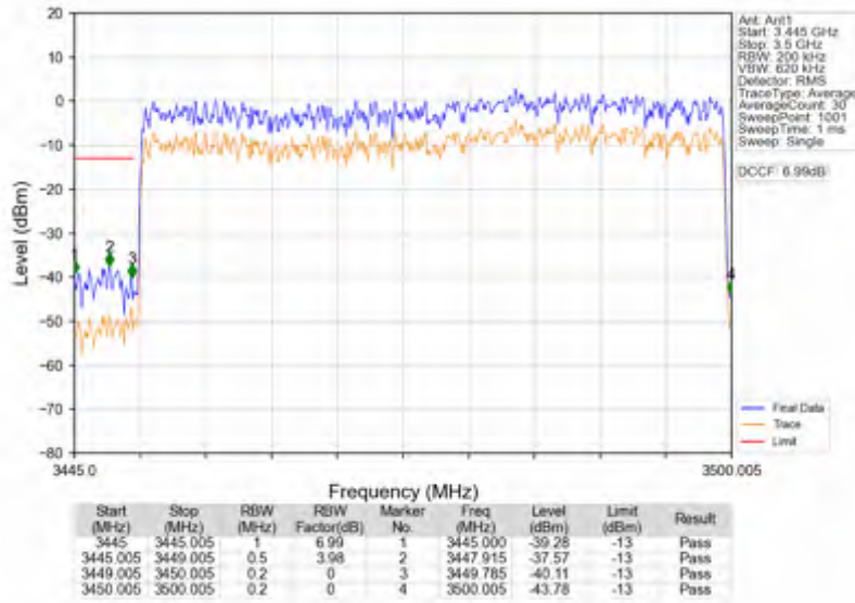
n78e_15kHz_SISO_NTNV_50MHz_CP-OFDM QPSK_3475.005MHz_Outer_Full
