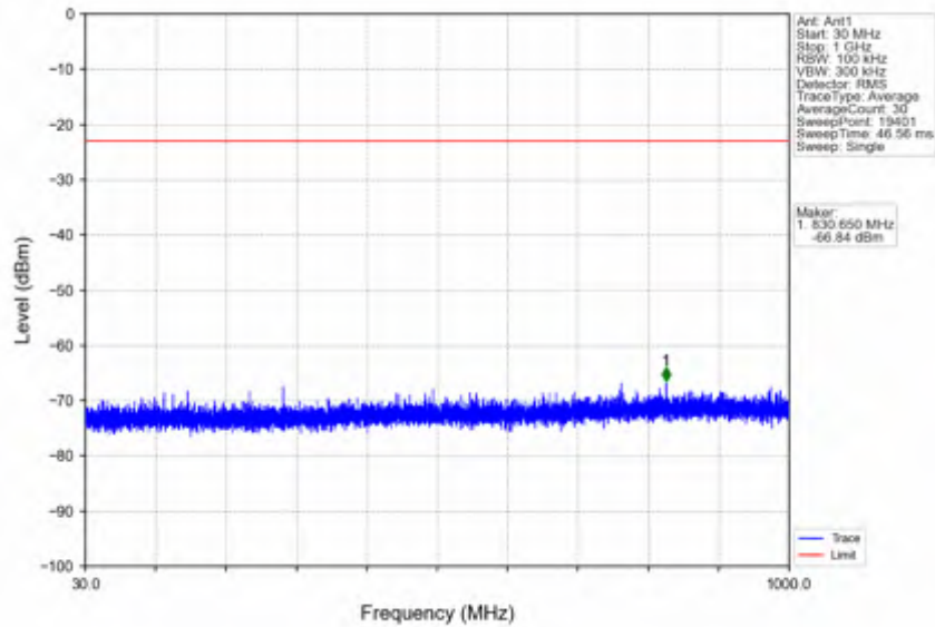
n78e_15kHz_SISO_NTV_40MHz_DFT-s-OFDM_QPSK_3529.995MHz_Inner_1RB_Right
