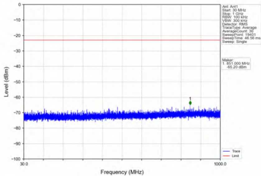
n78e_15kHz_SISO_NTNV_50MHz_CP-OFDM QPSK_3525MHz_Outer_Full
