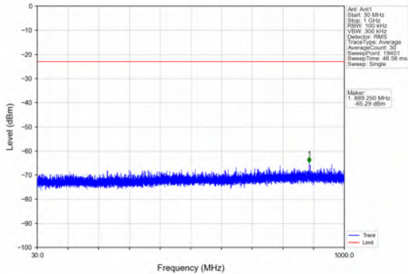
n78e_15kHz_SISO_NTNV_50MHz_DFT-s-OFDM_QPSK_3525MHz_Edge_1RB_Right
