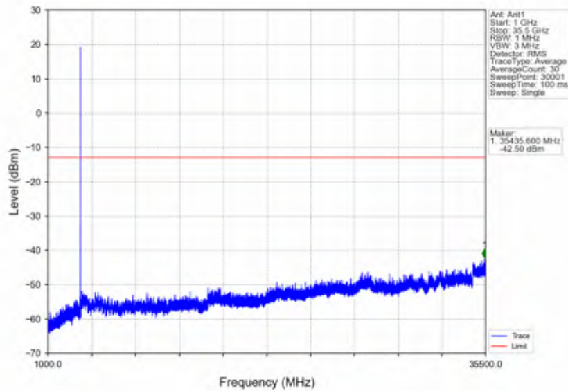
n78e_30kHz_SISO_NTNV_15MHz_CP-OFDM QPSK_3542.49MHz_Outer_Full
