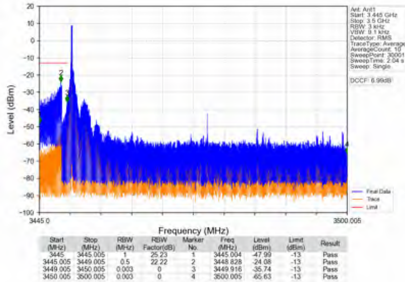
n78e_15kHz_SISO_NTNV_50MHz_CP-OFDM QPSK_3475.005MHz_Edge_1RB_Left
