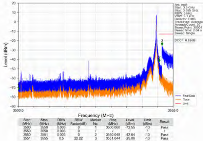
n78e_15kHz_SISO_NTNV_50MHz_CP-OFDM QPSK_3525MHz_Inner_1RB_Right
