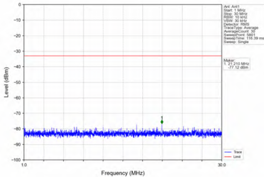
n78e_15kHz_SISO_NTNV_40MHz_DFT-s-OFDM QPSK_3529.995MHz_Outer_Full
