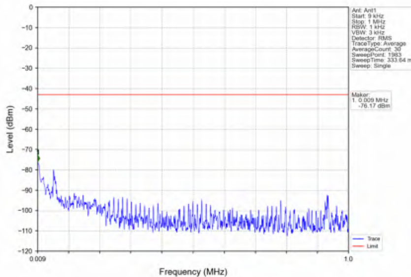
n78e_15kHz_SISO_NTNV_50MHz_DFT-s-OFDM QPSK_3475.005MHz_Outer_Full
