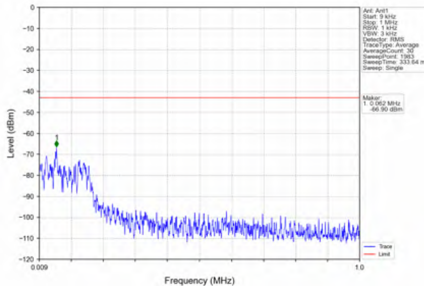
n78e_15kHz_SISO_NTNV_50MHz_DFT-s-OFDM_PI/2_BPSK_3525MHz_Edge_1RB_Right
