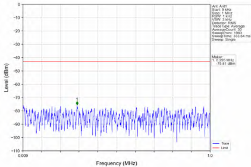
n78e_30kHz_SISO_NTNV_10MHz_CP-OFDM QPSK_3455.01MHz_Outer_Full
