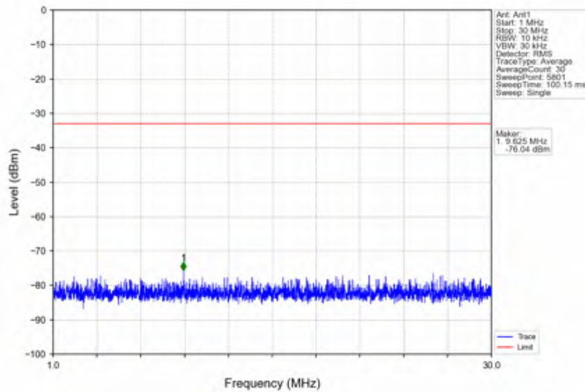
n78e_30kHz_SISO_NTNV_15MHz_DFT-s-OFDM_PI/2_BPSK_3457.5MHz_Inner_1RB_Left
