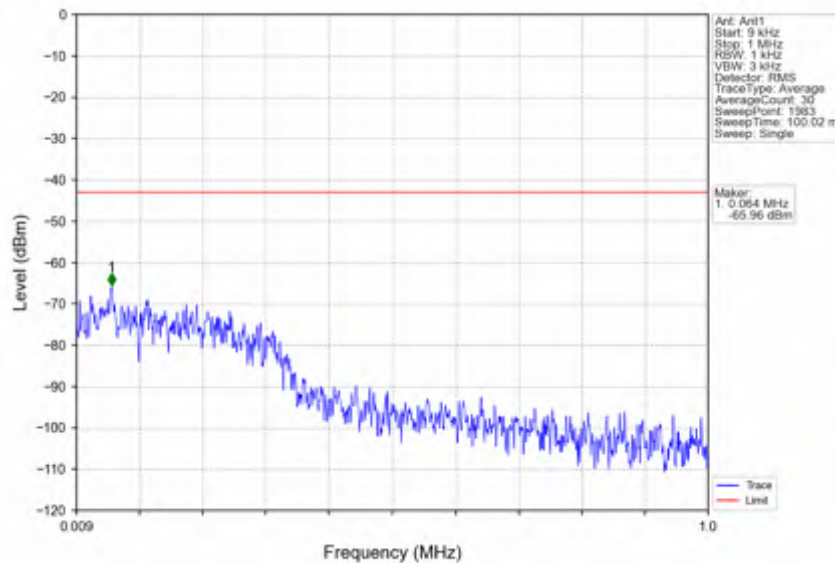
n78e_30kHz_SISO_NTNV_15MHz_CP-OFDM QPSK_3542.49MHz_Inner_1RB_Right
