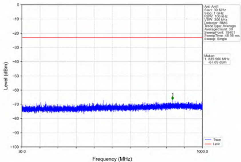
n78e_15kHz_SISO_NTV_50MHz_DFT-s-OFDM PI/2 BPSK_3525MHz_Edge_1RB_Right
