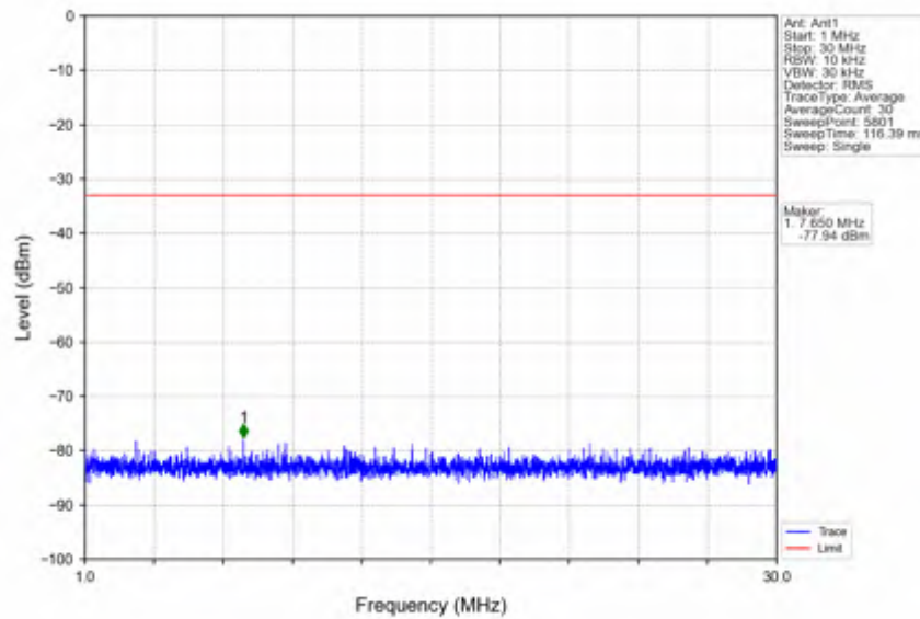
n78e_15kHz_SISO_NTNV_50MHz_DFT-s-OFDM PI/2 BPSK_3475.005MHz_Edge_1RB_Left
