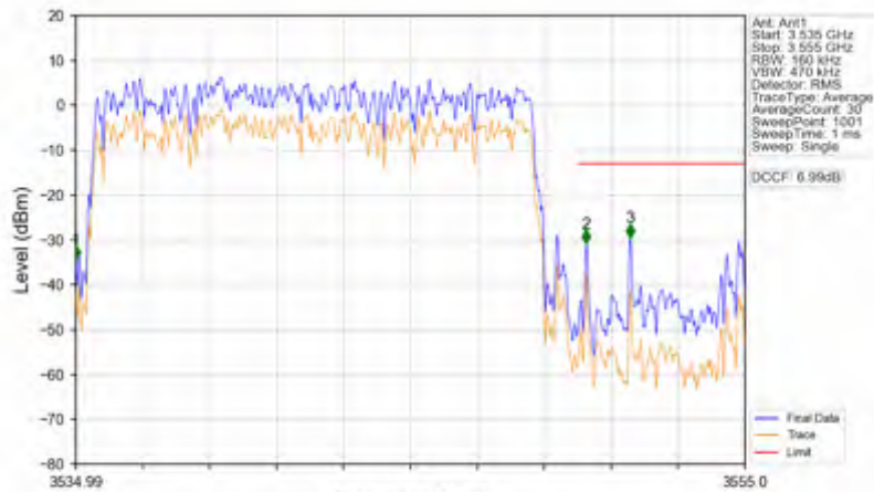
n78e_30kHz_SISO_NTNV_15MHz_DFT-s-OFDM PI/2 BPSK_3542.49MHz_Outer_Full
