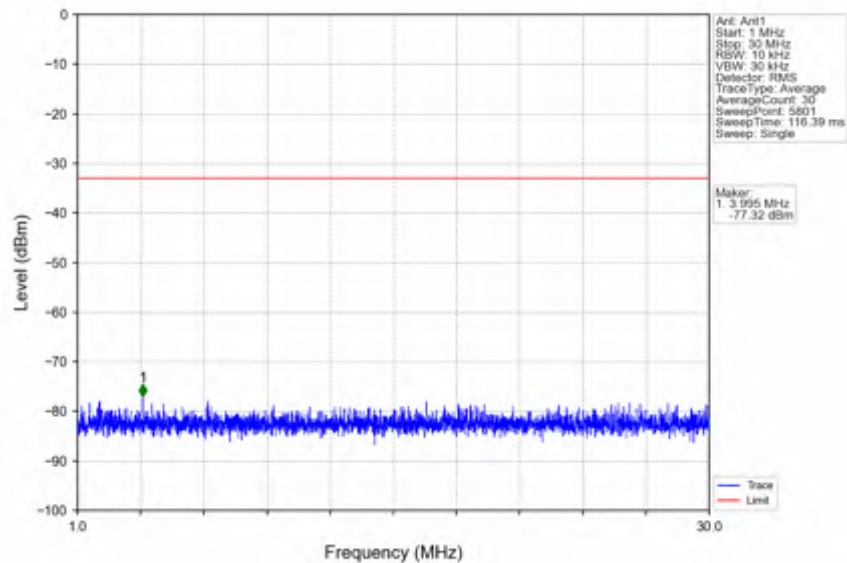
n78e_15kHz_SISO_NTNV_50MHz_CP-OFDM QPSK_3525MHz_Outer_Full
