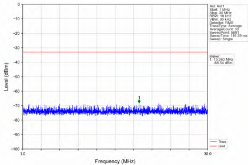
n78e_30kHz_SISO_NTNV_15MHz_CP-OFDM QPSK_3542.49MHz_Edge_1RB_Right
