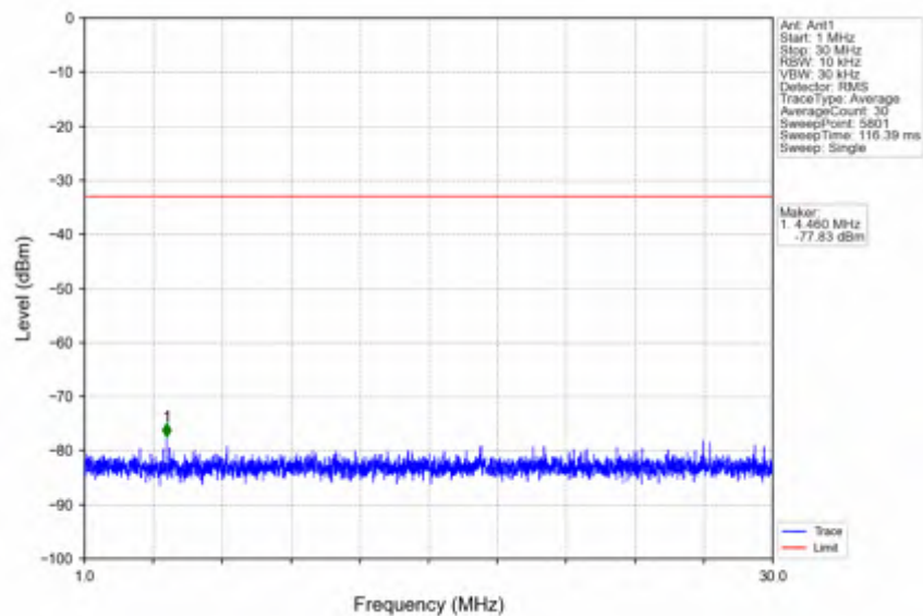
n78e_15kHz_SISO_NTV_40MHz_DFT-s-OFDM QPSK_3529.995MHz_Edge_1RB_Right
