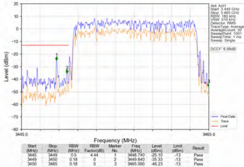
n78e_30kHz_SISO_NTNV_15MHz_DFT-s-OFDM_QPSK_3457.5MHz_Outer_Full
