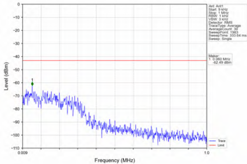
n78e_30kHz_SISO_NTVV_10MHz_CP-OFDM QPSK_3500.01MHz_Edge_1RB_Left
