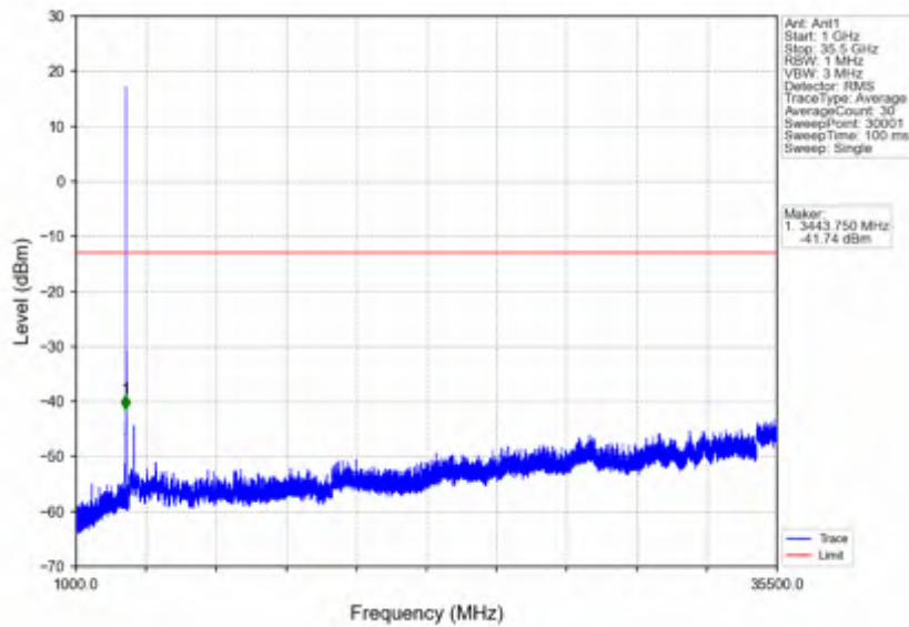
n78e_30kHz_SISO_NTNV_15MHz_CP-OFDM QPSK_3457.5MHz_Outer_Full
