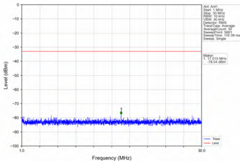
n78e_15kHz_SISO_NTNV_50MHz_DFT-s-OFDM PI/2 BPSK_3525MHz_Outer_Full
