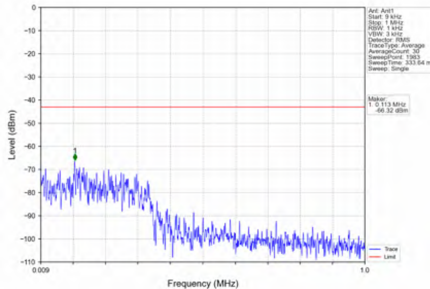
n78e_30kHz_SISO_NTNV_10MHz_DFT-s-OFDM QPSK_3500.01MHz_Edge_1RB_Left
