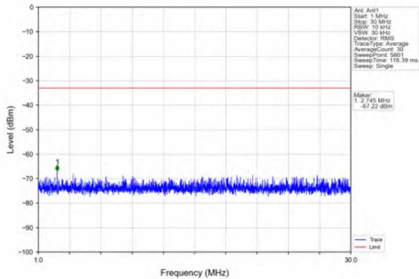
n78e_30kHz_SISO_NTNV_15MHz_CP-OFDM QPSK_3457.5MHz_Edge_1RB_Left
