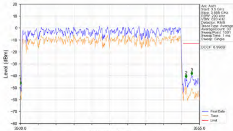
n78e_15kHz_SISO_NTNV_50MHz_DFT-s-OFDM PI/2 BPSK_3525MHz_Outer_Full
