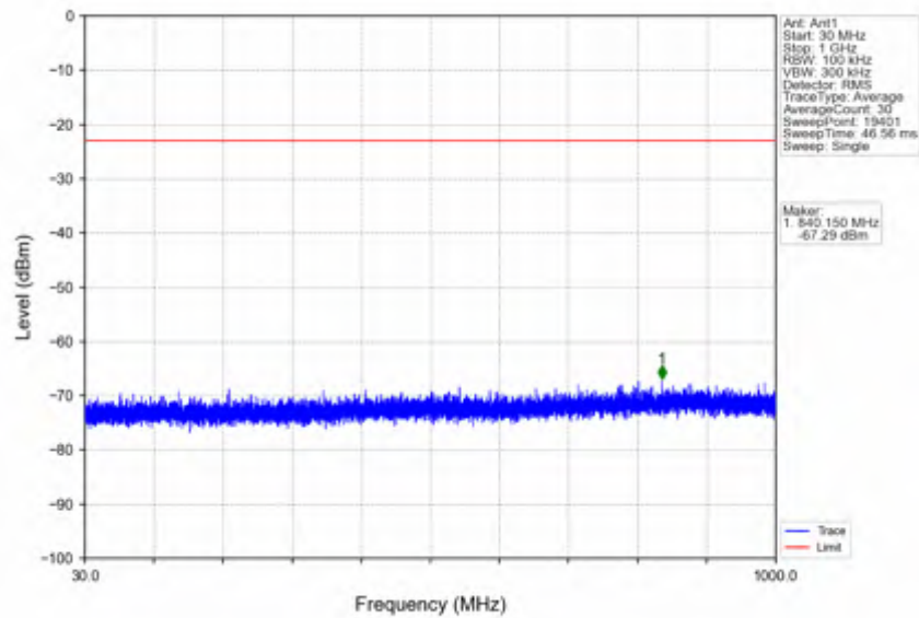
n78e_15kHz_SISO_NTNV_40MHz_CP-OFDM QPSK_3470.01MHz_Outer_Full
