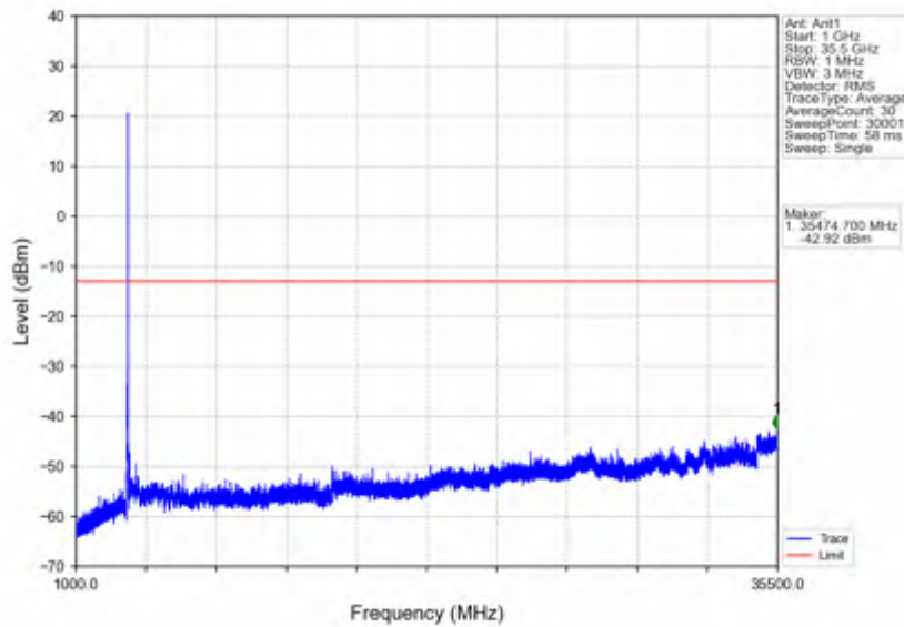
n78e_15kHz_SISO_NTV_40MHz_CP-OFDM QPSK_3529.995MHz_Outer_Full
