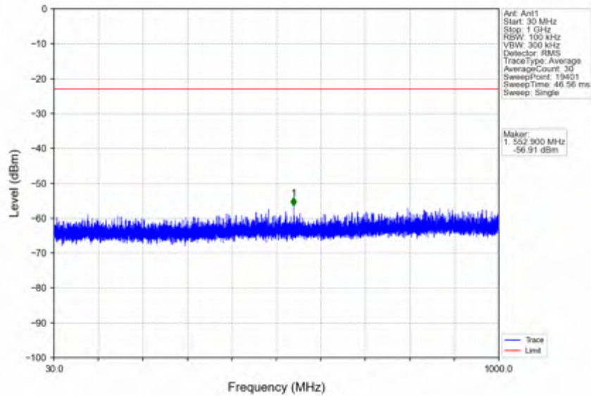
n78e_30kHz_SISO_NTNV_10MHz_DFT-s-OFDM QPSK_3544.98MHz_Edge_1RB_Right
