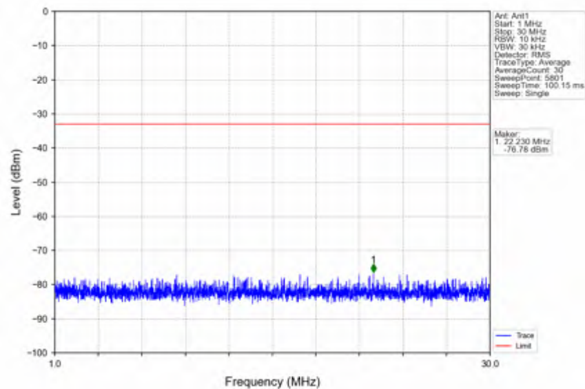
n78e_30kHz_SISO_NTNV_15MHz_CP-OFDM QPSK_3457.5MHz_Outer_Full
