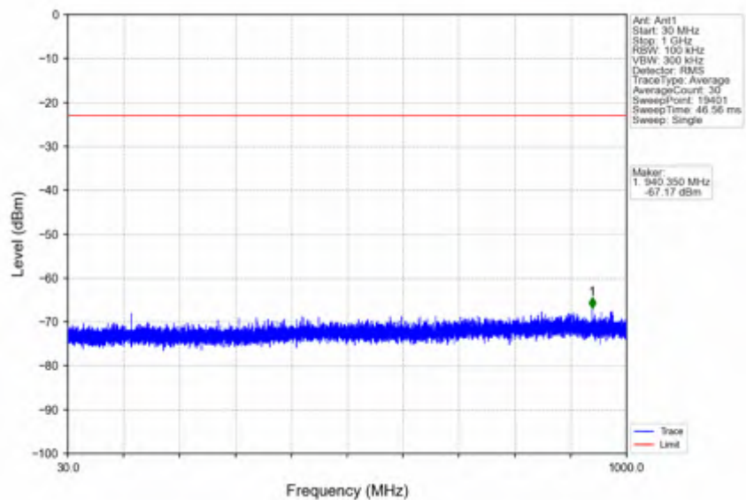
n78e_15kHz_SISO_NTNV_50MHz_DFT-s-OFDM QPSK_3475.005MHz_Outer_Full
