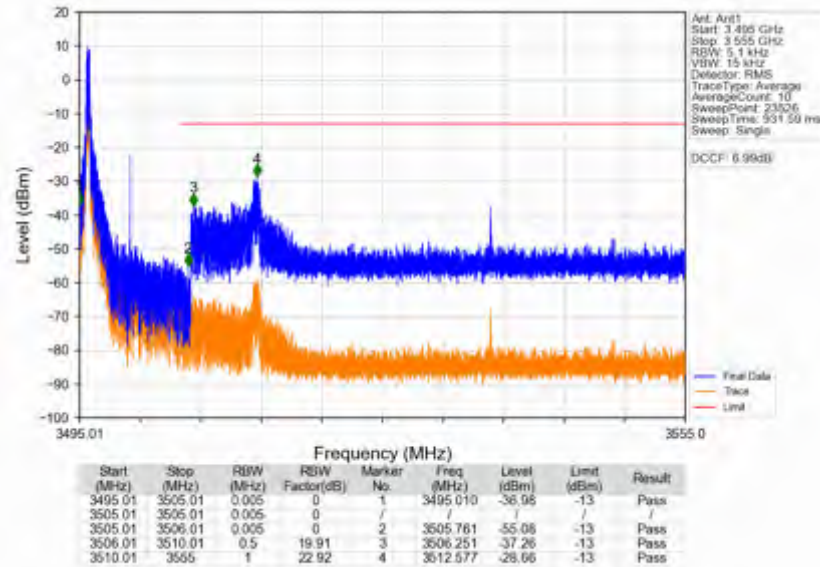
n78e_30kHz_SISO_NTNV_10MHz_DFT-s-OFDM QPSK_3500.01MHz_Edge_1RB_Left
