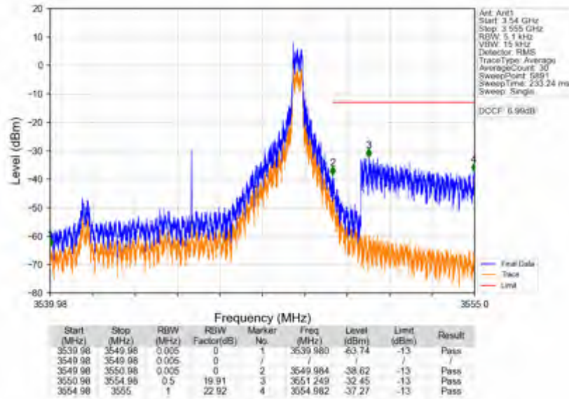
n78e_30kHz_SISO_NTNV_10MHz_CP-OFDM QPSK_3544.98MHz_Inner_1RB_Right
