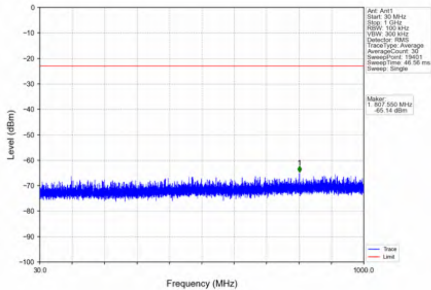
n78e_30kHz_SISO_NTNV_10MHz_CP-OFDM QPSK_3455.01MHz_Outer_Full
