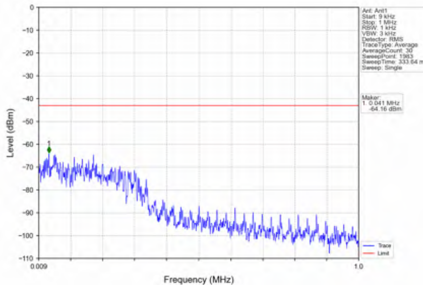
n78e_30kHz_SISO_NTV_10MHz_CP-OFDM QPSK_3455.01MHz_Edge_1RB_Left
