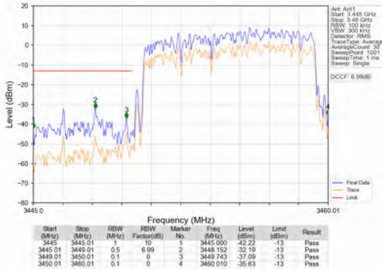
n78e_30kHz_SISO_NTNV_10MHz_DFT-s-OFDM_QPSK_3455.01MHz_Outer_Full
