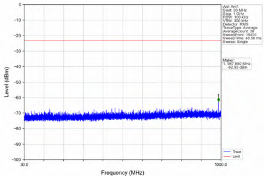
n78e_15kHz_SISO_NTNV_50MHz_CP-OFDM QPSK_3525MHz_Edge_1RB_Right
