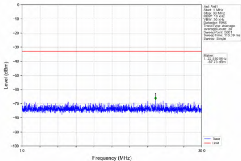
n78e_30kHz_SISO_NTNV_10MHz_DFT-s-OFDM QPSK_3455.01MHz_Edge_1RB_Left
