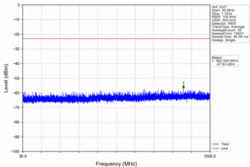
n78e_30kHz_SISO_NTNV_15MHz_DFT-s-OFDM PI/2 BPSK_3542.49MHz_Edge_1RB_Right
