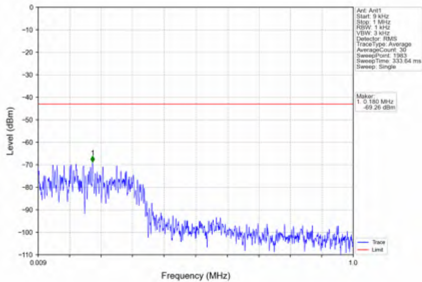
n78e_30kHz_SISO_NTNV_15MHz_DFT-s-OFDM QPSK_3542.49MHz_Edge_1RB_Right
