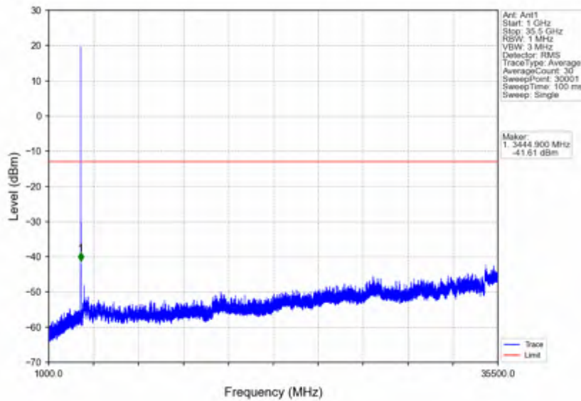
n78e_30kHz_SISO_NTNV_15MHz_CP-OFDM QPSK_3500.01MHz_Edge_1RB_Left
