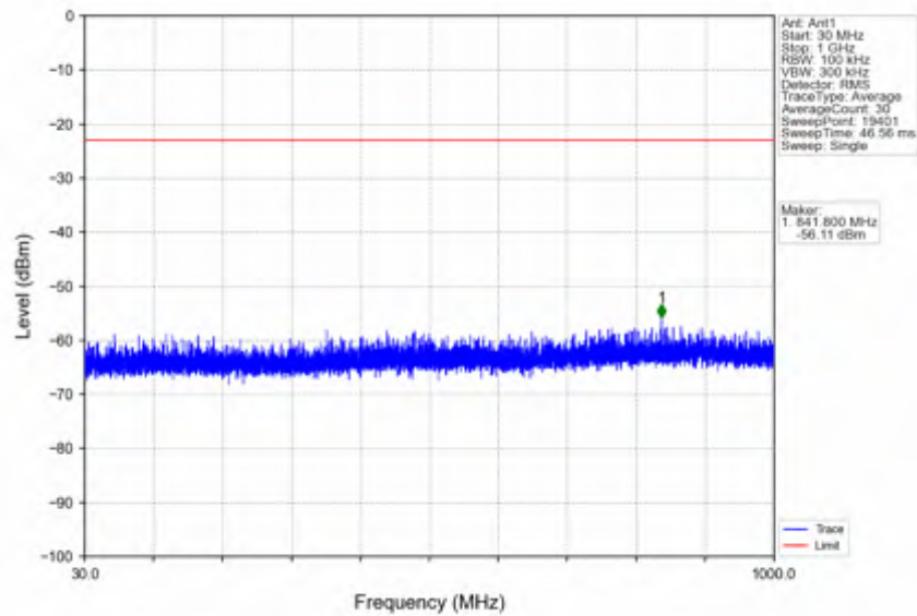
n78e_30kHz_SISO_NTNV_10MHz_DFT-s-OFDM QPSK_3455.01MHz_Edge_1RB_Left
