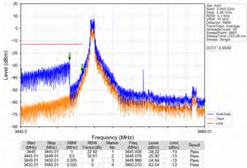
n78e_30kHz_SISO_NTNV_10MHz_DFT-s-OFDM QPSK_3455.01MHz_Edge_1RB_Left
