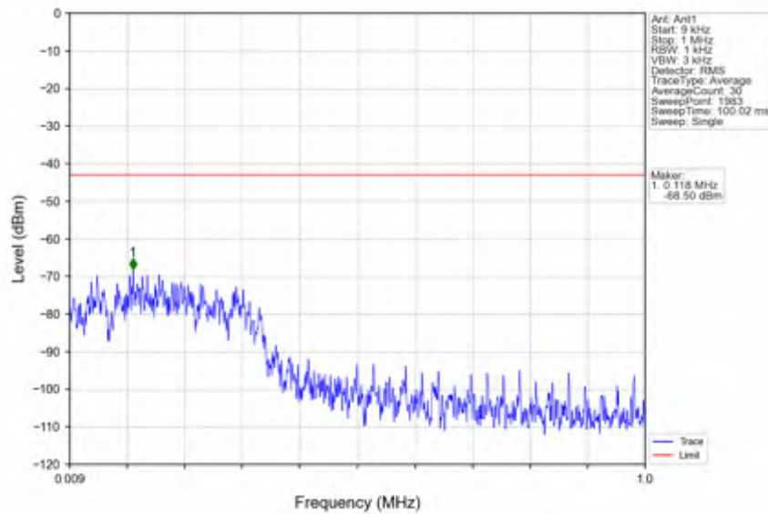
n78e_30kHz_SISO_NTNV_15MHz_DFT-s-OFDM QPSK_3457.5MHz_Inner_1RB_Left
