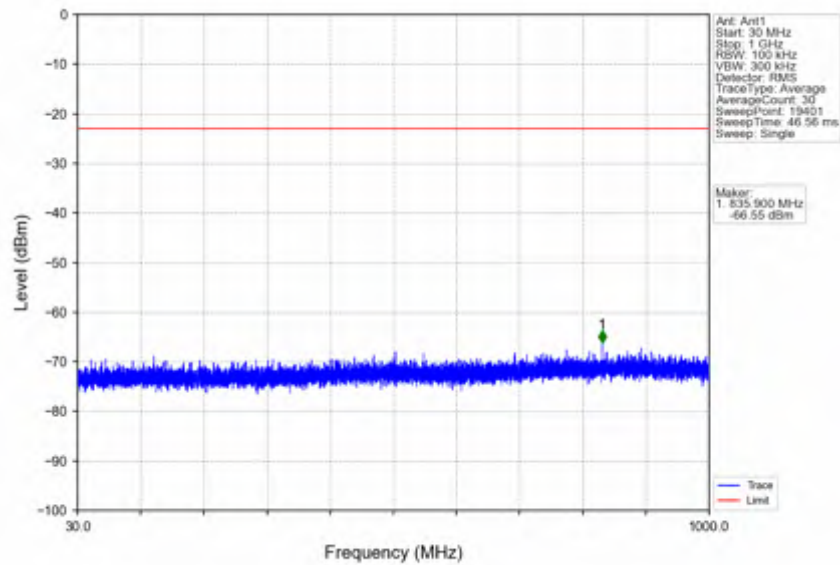
n78e_15kHz_SISO_NTNV_50MHz_DFT-s-OFDM_PI/2_BPSK_3475.005MHz_Outer_Full
