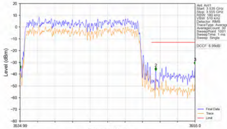
n78e_30kHz_SISO_NTNV_15MHz_DFT-s-OFDM_QPSK_3542.49MHz_Outer_Full
