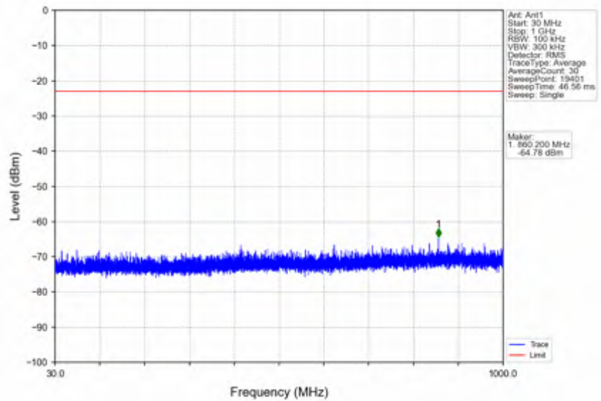
n78e_15kHz_SISO_NTNV_50MHz_CP-OFDM QPSK_3525MHz_Inner_1RB_Right
