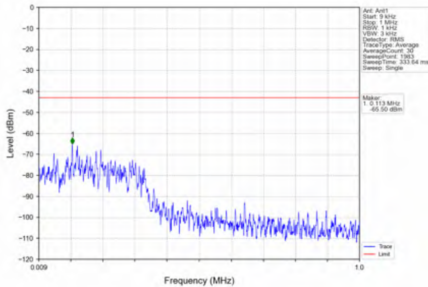
n78e_30kHz_SISO_NTNV_10MHz_DFT-s-OFDM_QPSK_3455.01MHz_Inner_1RB_Left
