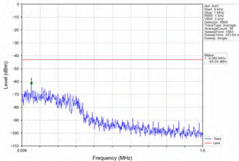
n78e_30kHz_SISO_NTNV_15MHz_CP-OFDM QPSK_3457.5MHz_Edge_1RB_Left
