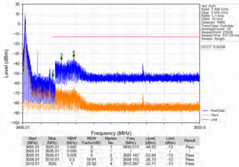
n78e_30kHz_SISO_NTV_10MHz_CP-OFDM QPSK_3500.01MHz_Edge_1RB_Left
