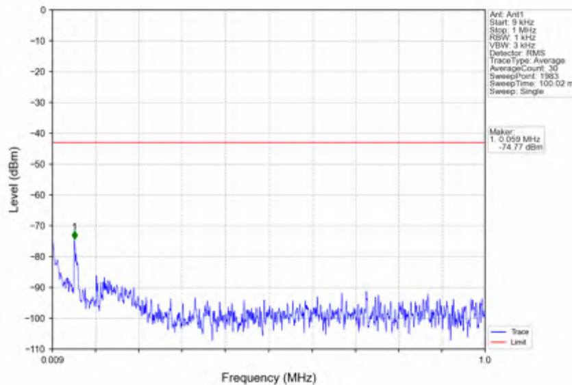
n78e_30kHz_SISO_NTNV_15MHz_DFT-s-OFDM_QPSK_3542.49MHz_Outer_Full
