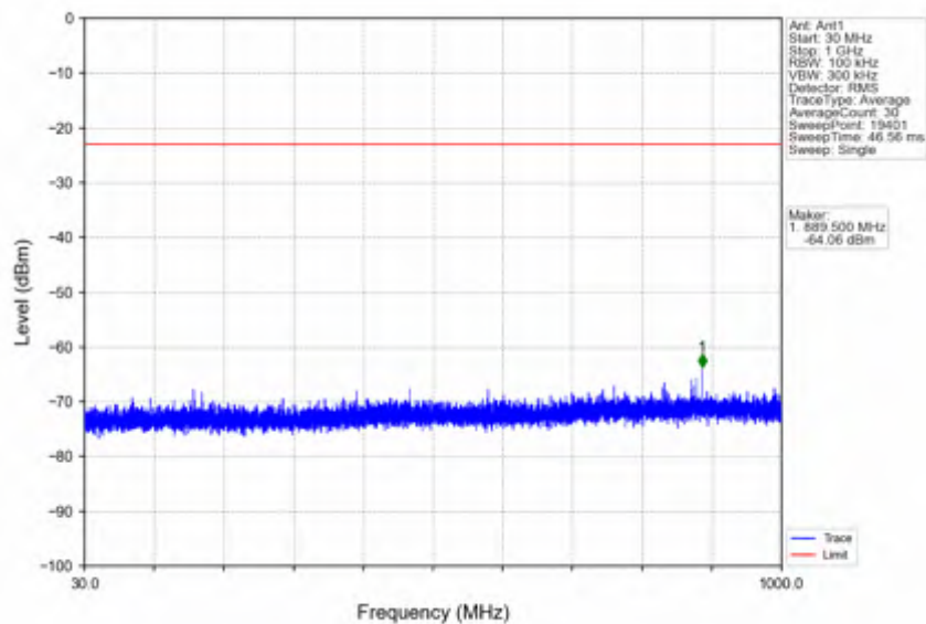
n78e_15kHz_SISO_NTNV_50MHz_CP-OFDM QPSK_3475.005MHz_Edge_1RB_Left
