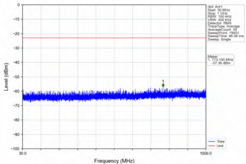
n78e_30kHz_SISO_NTNV_15MHz_DFT-s-OFDM PI/2 BPSK_3457.5MHz_Edge_1RB_Left
