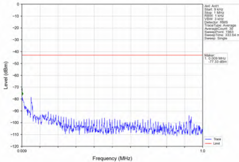
n78e_15kHz_SISO_NTNV_50MHz_DFT-s-OFDM QPSK_3525MHz_Outer_Full
