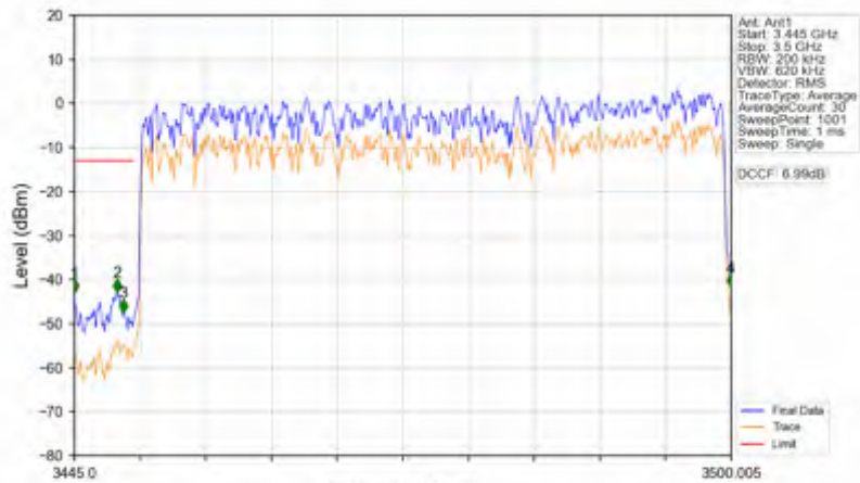
n78e_15kHz_SISO_NTNV_50MHz_DFT-s-OFDM PI/2 BPSK_3475.005MHz_Outer_Full
