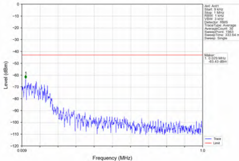
n78e_15kHz_SISO_NTVV_40MHz_CP-OFDM_QPSK_3470.01MHz_Edge_1RB_Left
