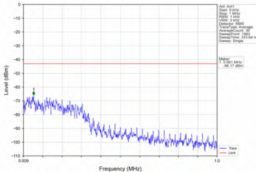
n78e_30kHz_SISO_NTV_10MHz_CP-OFDM QPSK_3544.98MHz_Edge_1RB_Right
