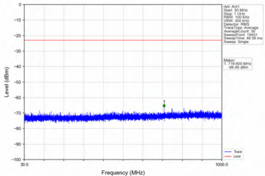
n78e_15kHz_SISO_NTNV_50MHz_DFT-s-OFDM_PI/2_BPSK_3525MHz_Inner_1RB_Right
