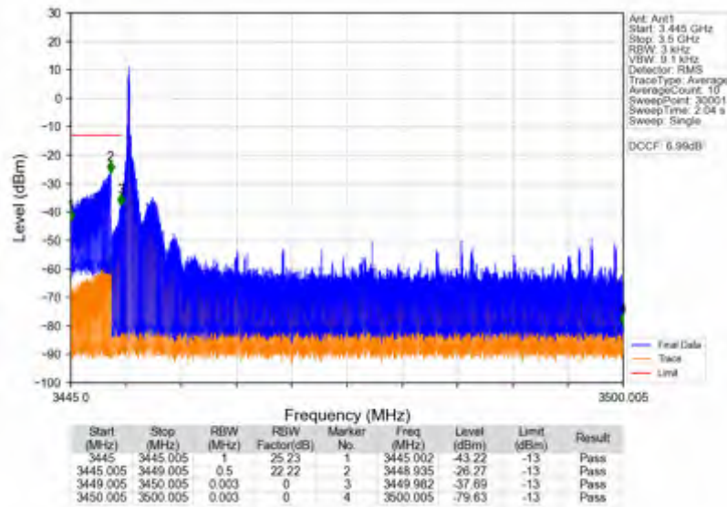
n78e_15kHz_SISO_NTNV_50MHz_DFT-s-OFDM QPSK_3475.005MHz_Edge_1RB_Left
