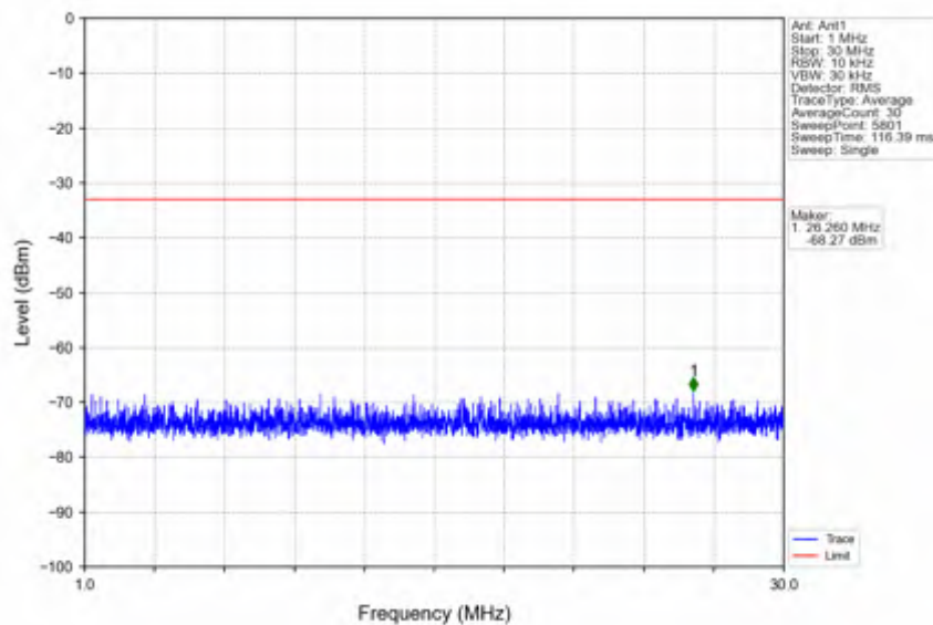
n78e_30kHz_SISO_NTNV_10MHz_DFT-s-OFDM PI/2 BPSK_3500.01MHz_Edge_1RB_Left
