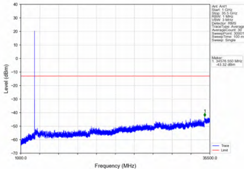
n78e_30kHz_SISO_NTV_15MHz_CP-OFDM QPSK_3500.01MHz_Edge_1RB_Left
