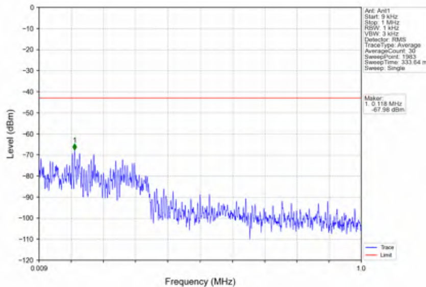
n78e_30kHz_SISO_NTNV_10MHz_DFT-s-OFDM PI/2 BPSK_3544.98MHz_Edge_1RB_Right
