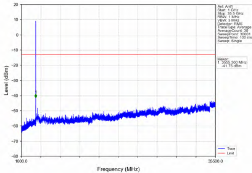
n78e_30kHz_SISO_NTNV_15MHz_DFT-s-OFDM QPSK_3542.49MHz_Inner_1RB_Right
