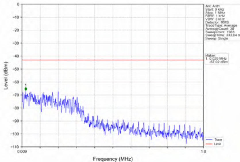
n78e_30kHz_SISO_NTV_15MHz_CP-OFDM QPSK_3542.49MHz_Edge_1RB_Right
