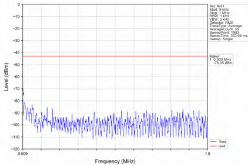
n78e_30kHz_SISO_NTNV_10MHz_DFT-s-OFDM PI/2 BPSK_3544.98MHz_Outer_Full
