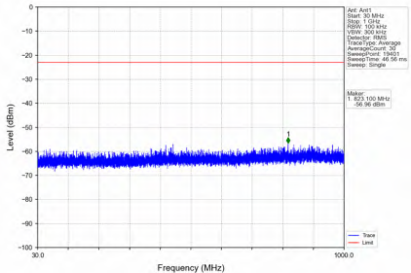
n78e_30kHz_SISO_NTVV_10MHz_CP-OFDM QPSK_3455.01MHz_Edge_1RB_Left
