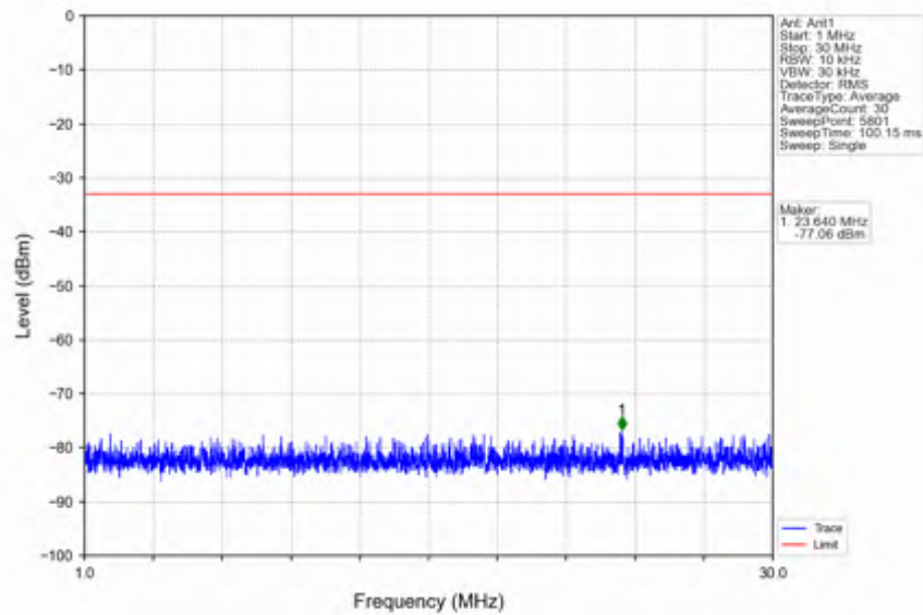
n78e_30kHz_SISO_NTNV_15MHz_CP-OFDM QPSK_3542.49MHz_Inner_1RB_Right
