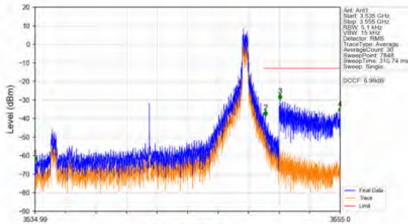
n78e_30kHz_SISO_NTNV_15MHz_DFT-s-OFDM QPSK_3542.49MHz_Inner_1RB_Right
