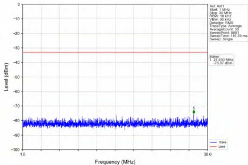
n78e_30kHz_SISO_NTNV_10MHz_DFT-s-OFDM PI/2 BPSK_3455.01MHz_Outer_Full
