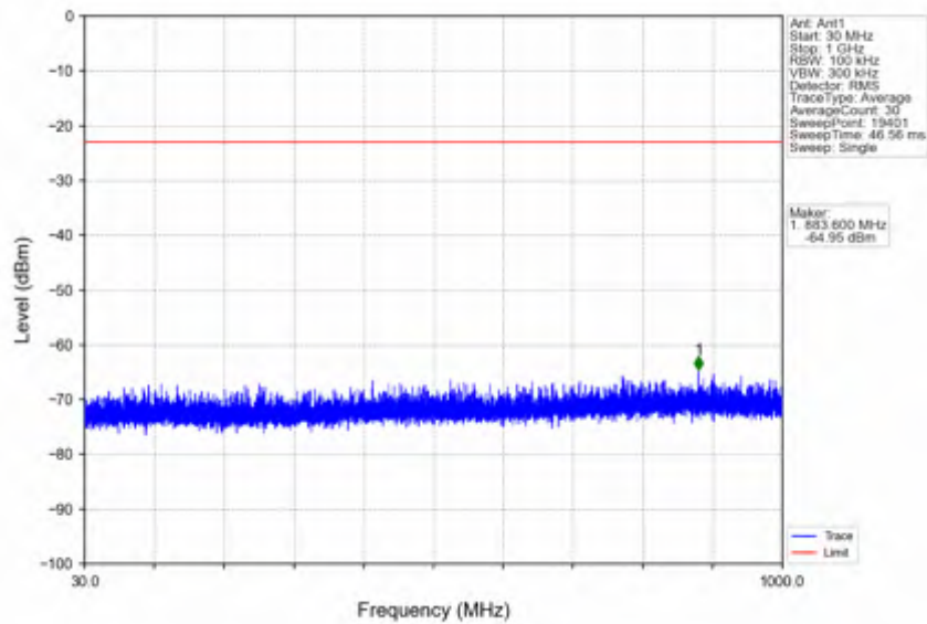
n78e_30kHz_SISO_NTNV_10MHz_DFT-s-OFDM QPSK_3455.01MHz_Inner_1RB_Left
