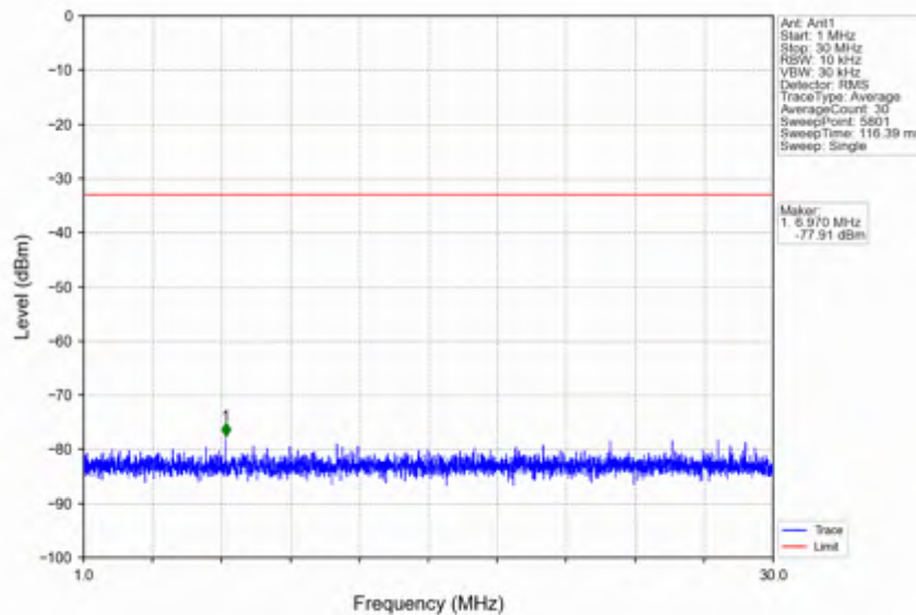
n78e_15kHz_SISO_NTNV_50MHz_DFT-s-OFDM PI/2 BPSK_3475.005MHz_Outer_Full
