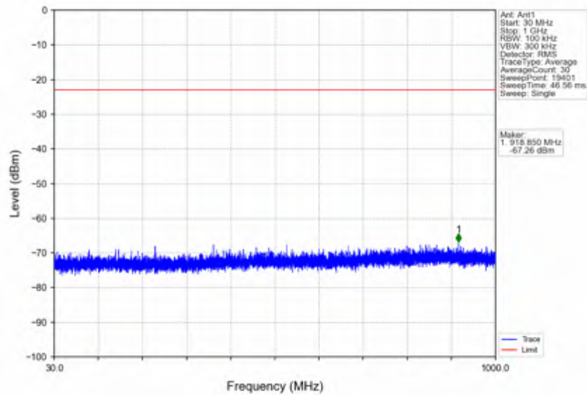
n78e_15kHz_SISO_NTNV_40MHz_CP-OFDM QPSK_3529.995MHz_Outer_Full
