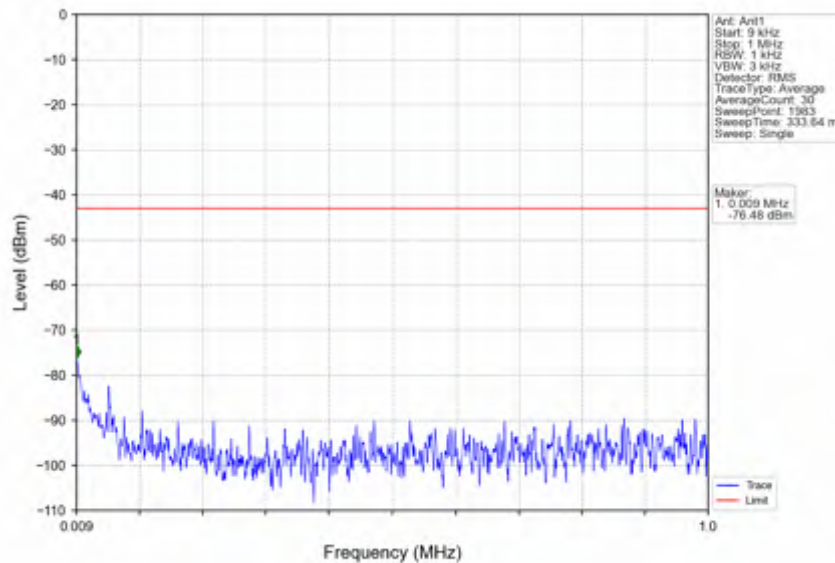
n78e_30kHz_SISO_NTNV_10MHz_DFT-s-OFDM_QPSK_3544.98MHz_Outer_Full
