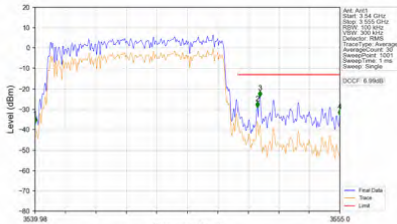
n78e_30kHz_SISO_NTNV_10MHz_CP-OFDM QPSK_3544.98MHz_Outer_Full
