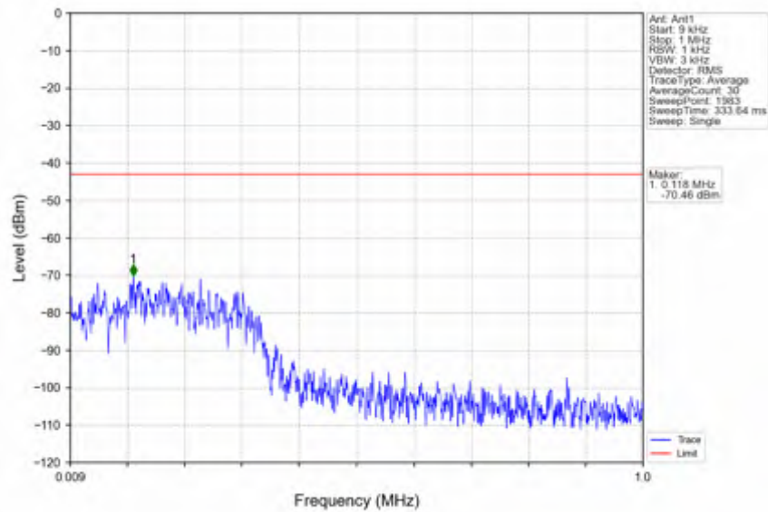
n78e_30kHz_SISO_NTNV_10MHz_DFT-s-OFDM QPSK_3544.98MHz_Inner_1RB_Right
