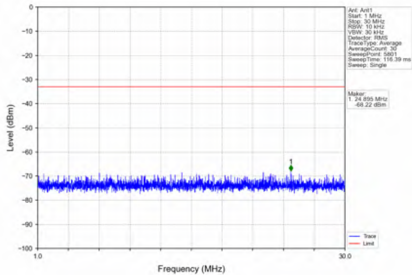
n78e_30kHz_SISO_NTNV_15MHz_DFT-s-OFDM QPSK_3500.01MHz_Edge_1RB_Left
