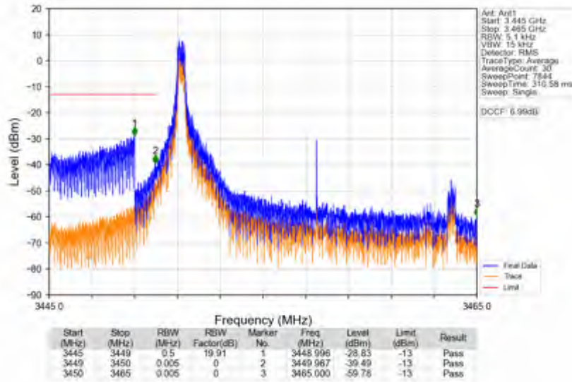
n78e_30kHz_SISO_NTNV_15MHz_DFT-s-OFDM_PI/2_BPSK_3457.5MHz_Inner_1RB_Left
