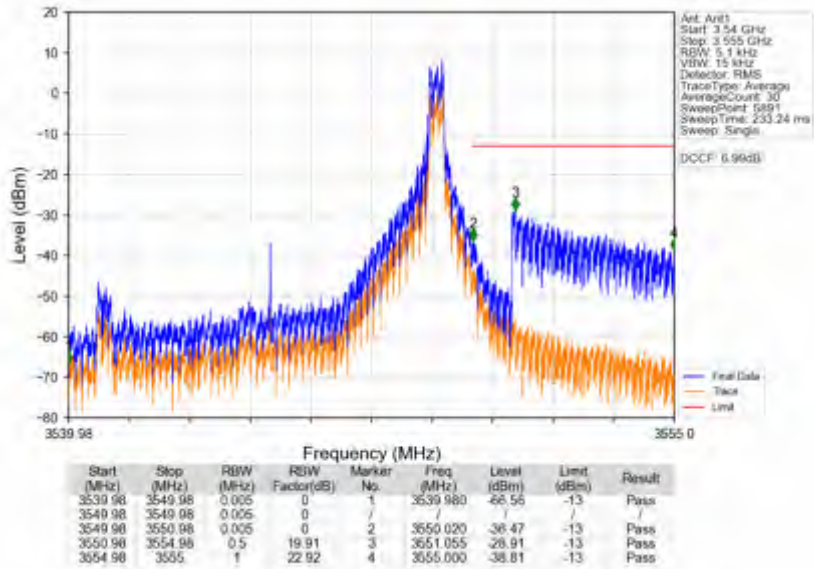
n78e_30kHz_SISO_NTNV_10MHz_DFT-s-OFDM QPSK_3544.98MHz_Edge_1RB_Right
