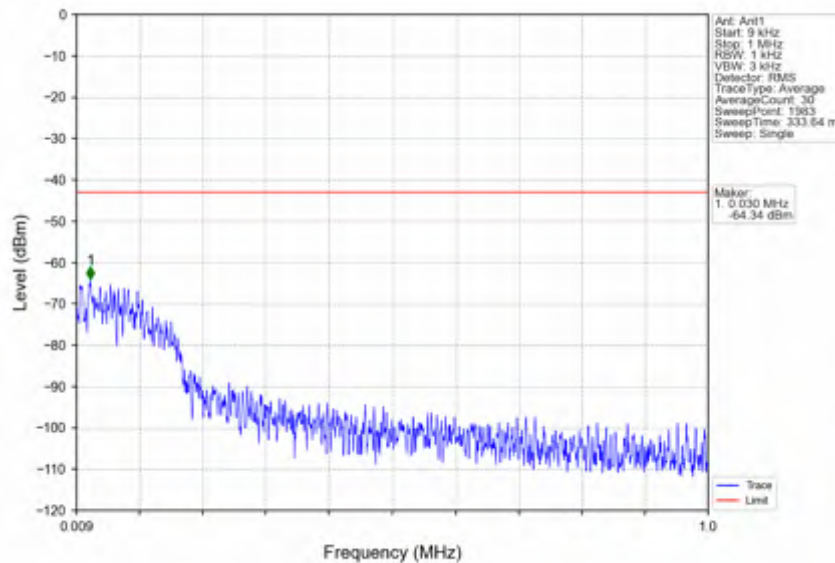
n78e_15kHz_SISO_NTNV_50MHz_CP-OFDM QPSK_3525MHz_Inner_1RB_Right
