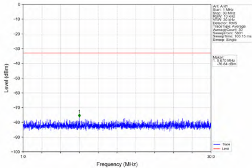
n78e_30kHz_SISO_NTNV_15MHz_DFT-s-OFDM_PI/2_BPSK_3542.49MHz_Inner_1RB_Right
