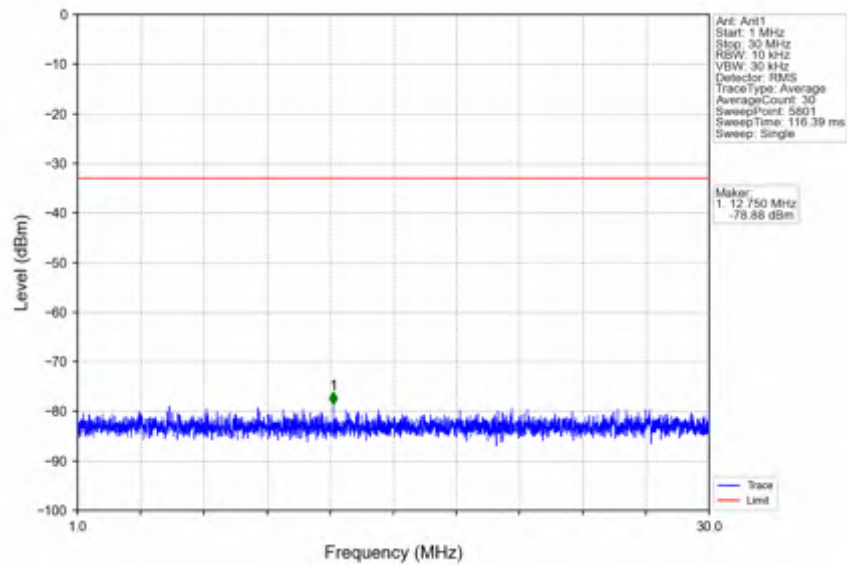
n78e_15kHz_SISO_NTV_40MHz_CP-OFDM QPSK_3529.995MHz_Inner_1RB_Right
