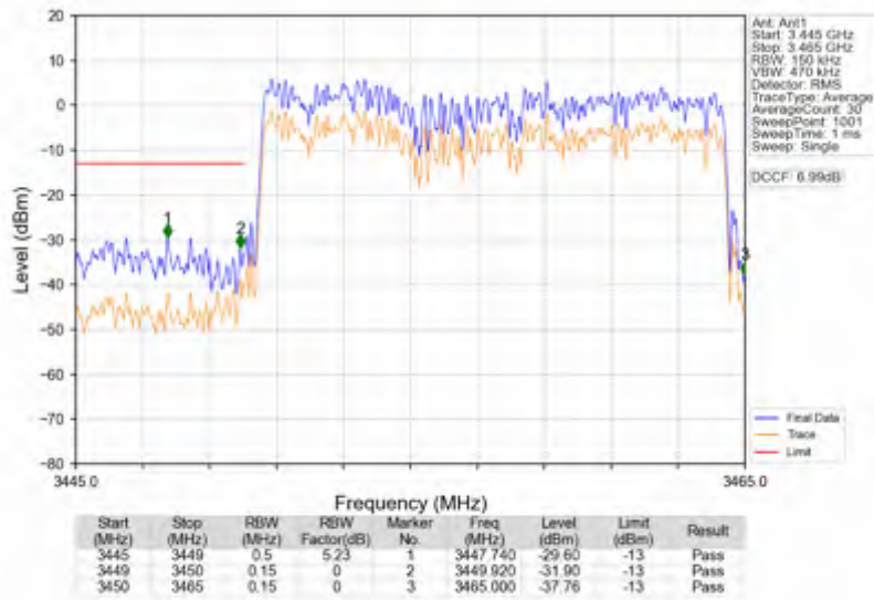
n78e_30kHz_SISO_NTNV_15MHz_CP-OFDM QPSK_3457.5MHz_Outer_Full
