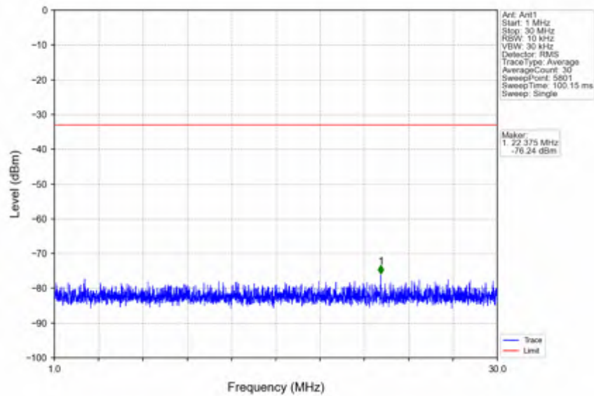
n78e_30kHz_SISO_NTNV_15MHz_CP-OFDM QPSK_3457.5MHz_Inner_1RB_Left
