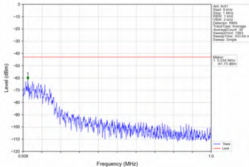
n78e_15kHz_SISO_NTNV_50MHz_CP-OFDM QPSK_3475.005MHz_Edge_1RB_Left
