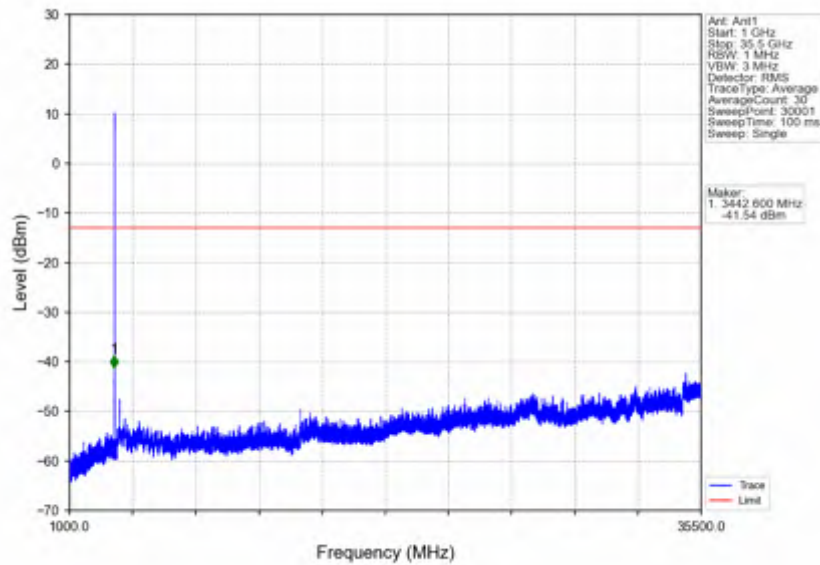
n78e_30kHz_SISO_NTNV_15MHz_DFT-s-OFDM QPSK_3457.5MHz_Inner_1RB_Left
