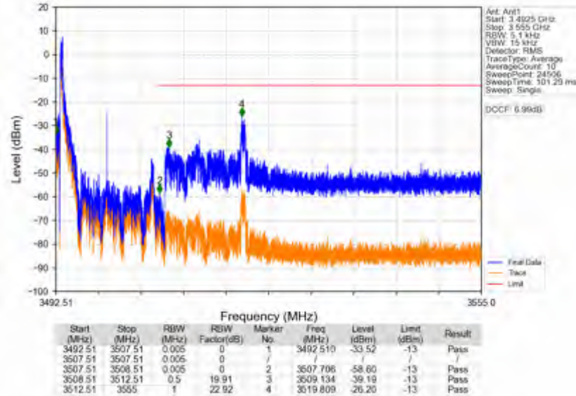
n78e_30kHz_SISO_NTNV_15MHz_DFT-s-OFDM QPSK_3500.01MHz_Edge_1RB_Left
