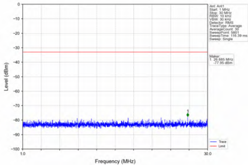
n78e_15kHz_SISO_NTNV_40MHz_CP-OFDM QPSK_3529.995MHz_Edge_1RB_Right
