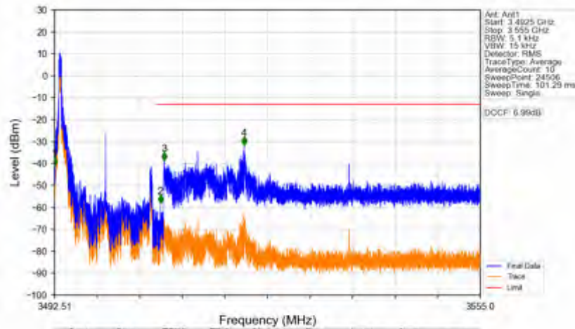
n78e_30kHz_SISO_NTNV_15MHz_DFT-s-OFDM PI/2 BPSK_3500.01MHz_Edge_1RB_Left
