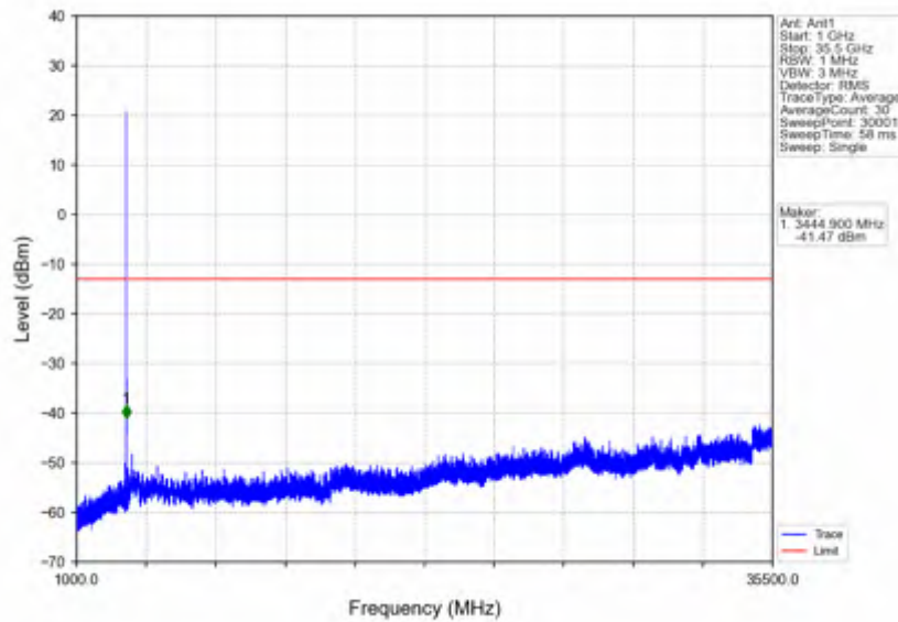
n78e_30kHz_SISO_NTV_10MHz_CP-OFDM QPSK_3500.01MHz_Edge_1RB_Left
