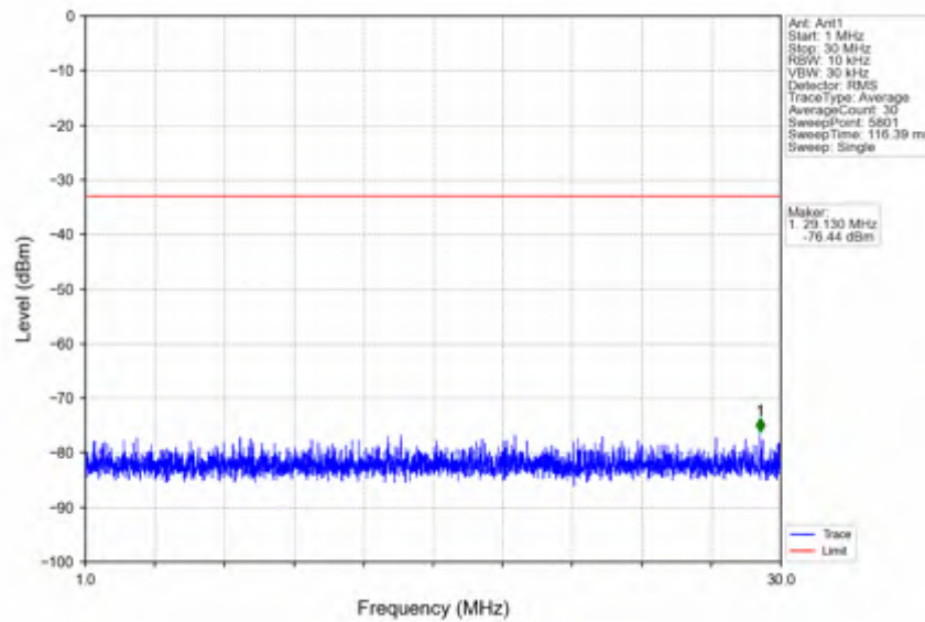
n78e_30kHz_SISO_NTNV_10MHz_DFT-s-OFDM_PI/2_BPSK_3544.98MHz_Inner_1RB_Right
