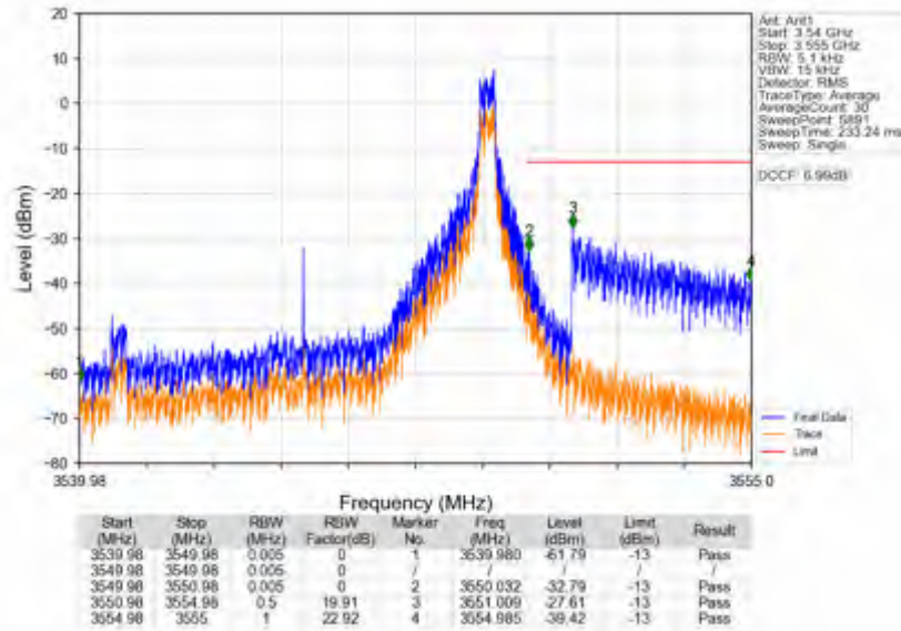
n78e_30kHz_SISO_NTV_10MHz_CP-OFDM QPSK_3544.98MHz_Edge_1RB_Right
