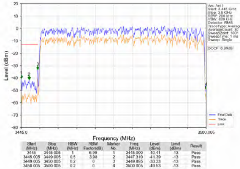
n78e_15kHz_SISO_NTNV_50MHz_DFT-s-OFDM QPSK_3475.005MHz_Outer_Full
