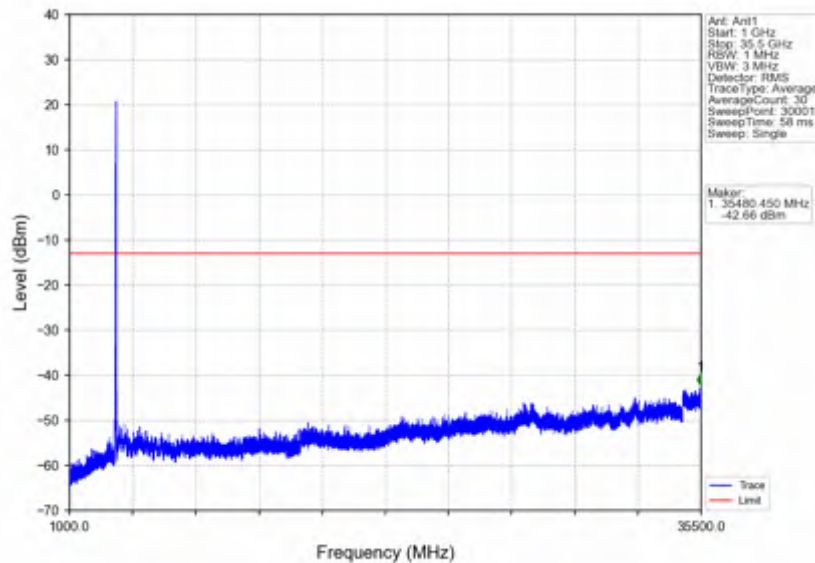
n78e_15kHz_SISO_NTV_40MHz_DFT-s-OFDM_QPSK_3529.995MHz_Inner_1RB_Right
