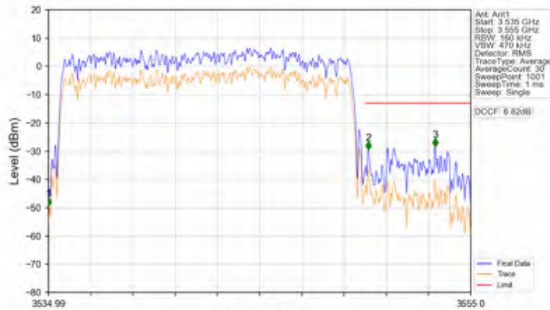
n78e_30kHz_SISO_NTNV_15MHz_CP-OFDM QPSK_3542.49MHz_Outer_Full
