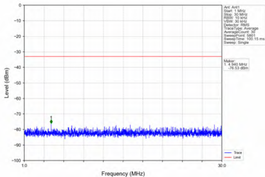
n78e_30kHz_SISO_NTNV_15MHz_CP-OFDM QPSK_3542.49MHz_Outer_Full
