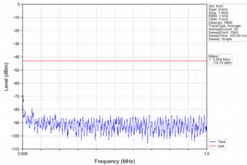
n78e_15kHz_SISO_NTNV_40MHz_CP-OFDM QPSK_3470.01MHz_Outer_Full
