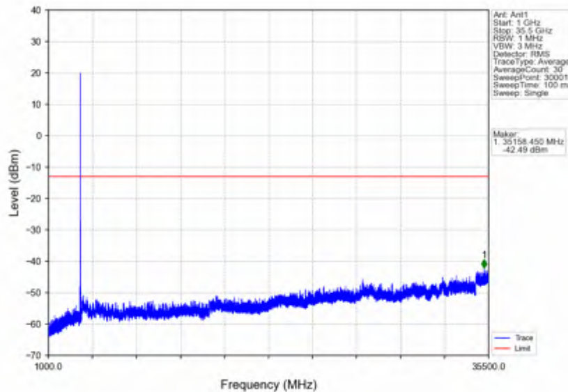
n78e_30kHz_SISO_NTNV_15MHz_DFT-s-OFDM PI/2 BPSK_3500.01MHz_Edge_1RB_Left
