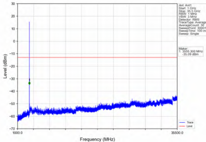
n78e_30kHz_SISO_NTNV_15MHz_DFT-s-OFDM QPSK_3542.49MHz_Edge_1RB_Right
