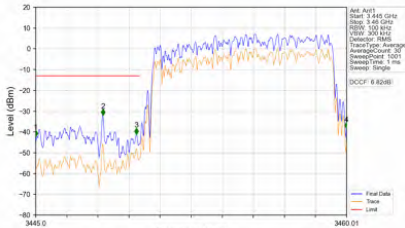
n78e_30kHz_SISO_NTNV_10MHz_DFT-s-OFDM PI/2 BPSK_3455.01MHz_Outer_Full
