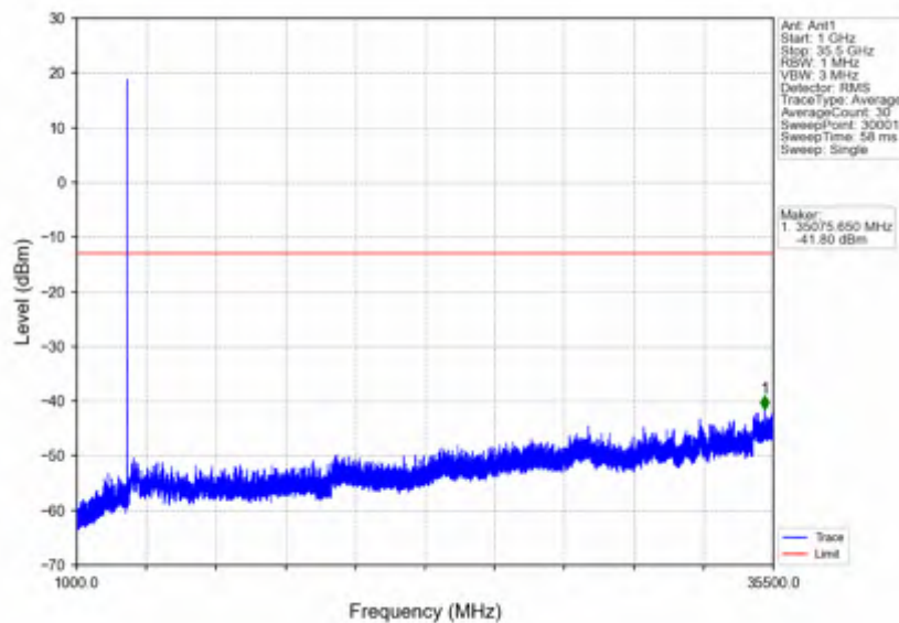
n78e_30kHz_SISO_NTVV_10MHz_CP-OFDM QPSK_3500.01MHz_Edge_1RB_Left
