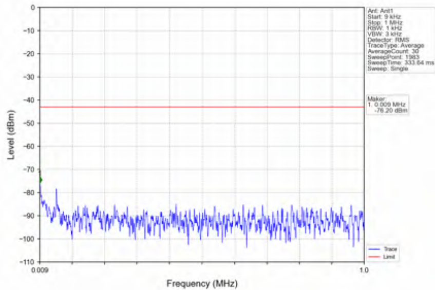
n78e_15kHz_SISO_NTNV_40MHz_CP-OFDM QPSK_3529.995MHz_Outer_Full
