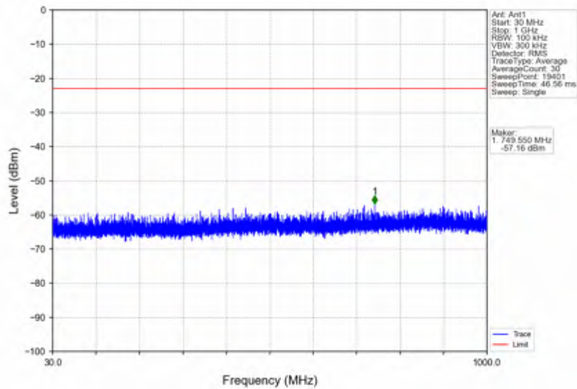
n78e_30kHz_SISO_NTVV_10MHz_CP-OFDM QPSK_3500.01MHz_Edge_1RB_Left
