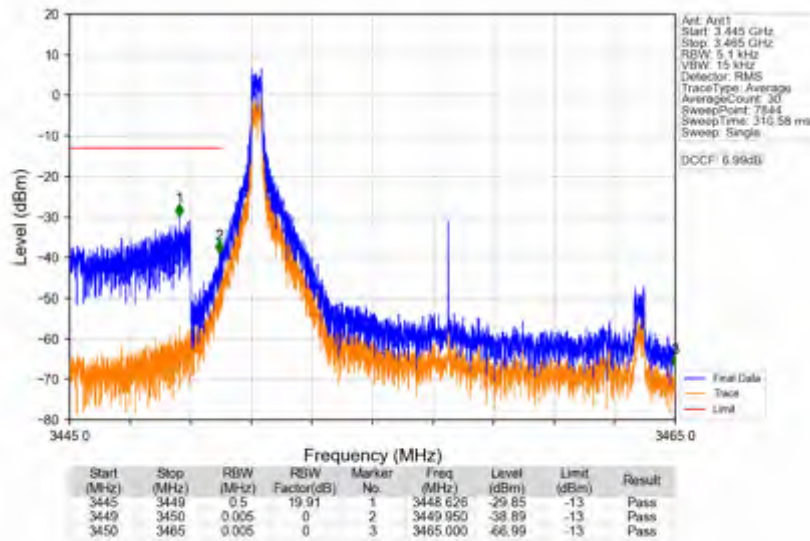
n78e_30kHz_SISO_NTNV_15MHz_DFT-s-OFDM QPSK_3457.5MHz_Inner_1RB_Left
