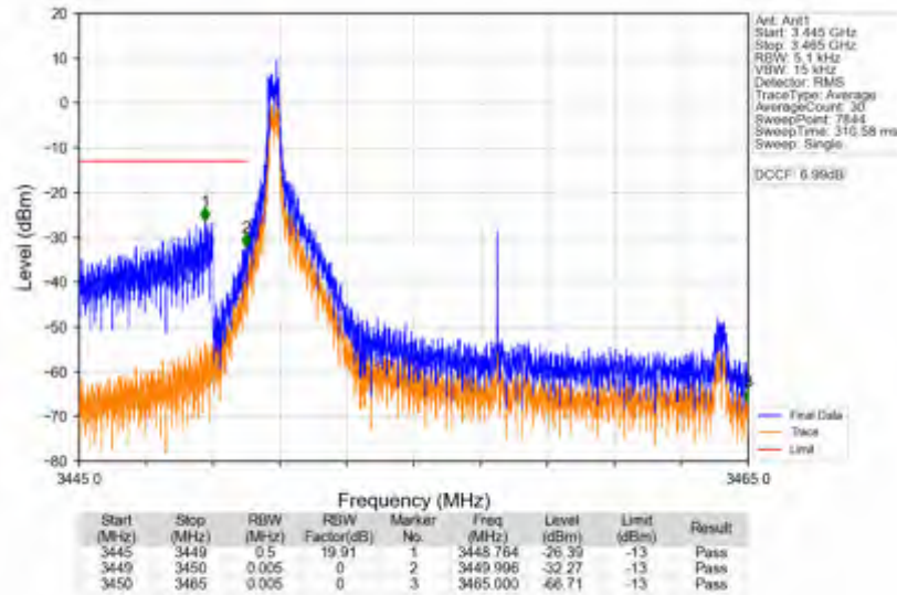
n78e_30kHz_SISO_NTNV_15MHz_CP-OFDM QPSK_3457.5MHz_Edge_1RB_Left
