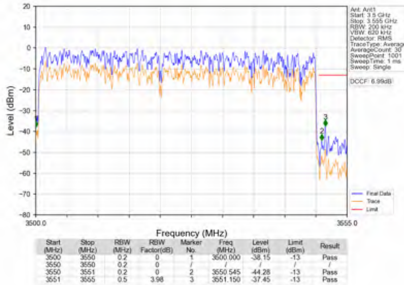
n78e_15kHz_SISO_NTNV_50MHz_DFT-s-OFDM QPSK_3525MHz_Outer_Full
