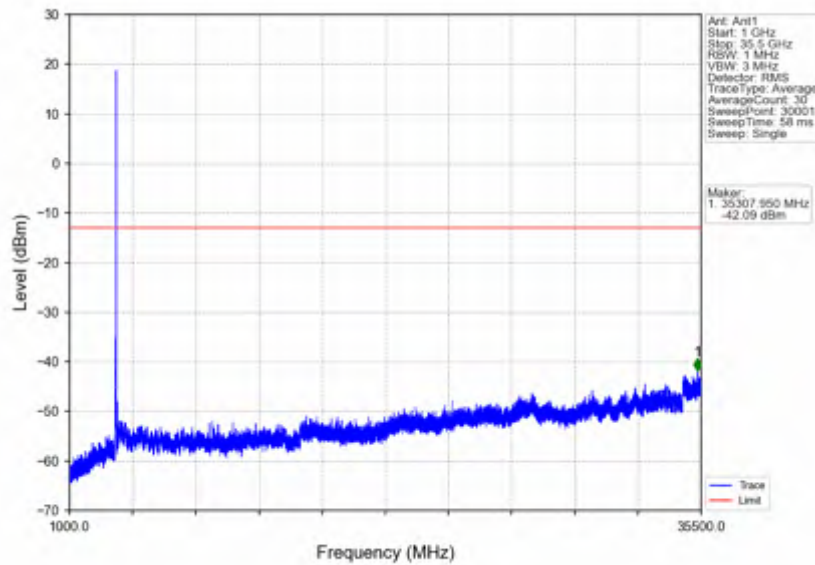
n78e_15kHz_SISO_NTV_40MHz_DFT-s-OFDM_QPSK_3529.995MHz_Edge_1RB_Right
