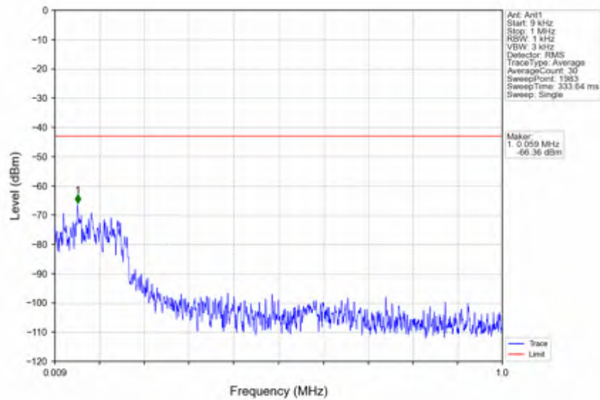
n78e_15kHz_SISO_NTNV_50MHz_DFT-s-OFDM_QPSK_3525MHz_Inner_1RB_Right
