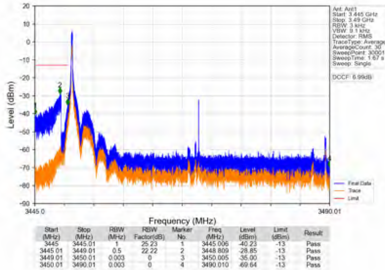
n78e_15kHz_SISO_NTVV_40MHz_CP-OFDM_QPSK_3470.01MHz_Edge_1RB_Left
