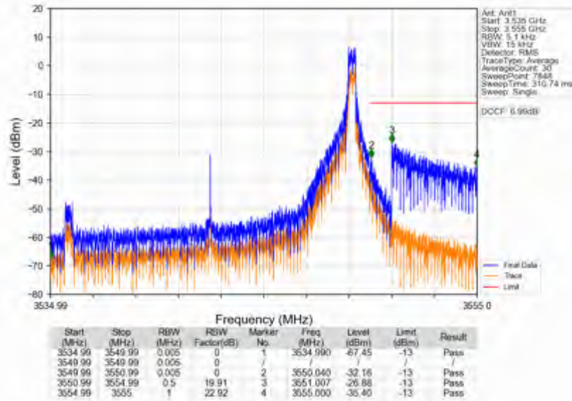
n78e_30kHz_SISO_NTV_15MHz_CP-OFDM QPSK_3542.49MHz_Edge_1RB_Right
