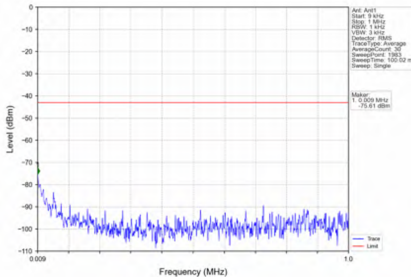
n78e_30kHz_SISO_NTNV_15MHz_DFT-s-OFDM_QPSK_3457.5MHz_Outer_Full
