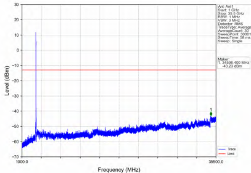
n78e_15kHz_SISO_NTNV_50MHz_DFT-s-OFDM_PI/2_BPSK_3475.005MHz_Outer_Full
