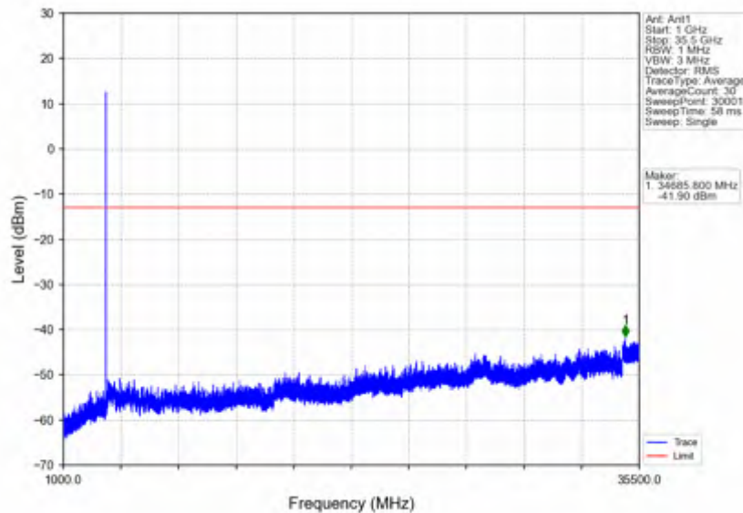
n78e_30kHz_SISO_NTNV_10MHz_DFT-s-OFDM PI/2 BPSK_3544.98MHz_Outer_Full
