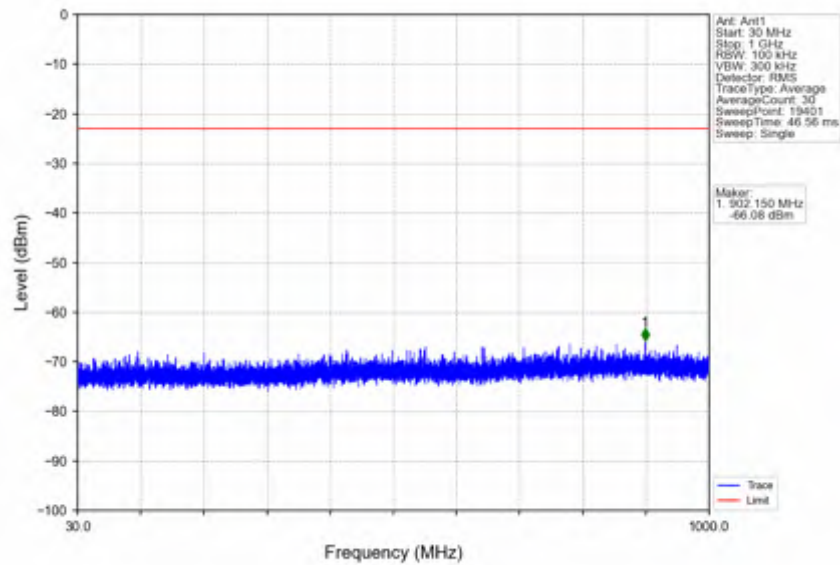
n78e_15kHz_SISO_NTNV_50MHz_DFT-s-OFDM_QPSK_3525MHz_Inner_1RB_Right
