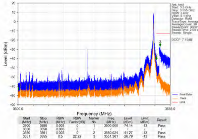
n78e_15kHz_SISO_NTNV_50MHz_DFT-s-OFDM_PI/2_BPSK_3525MHz_Inner_1RB_Right
