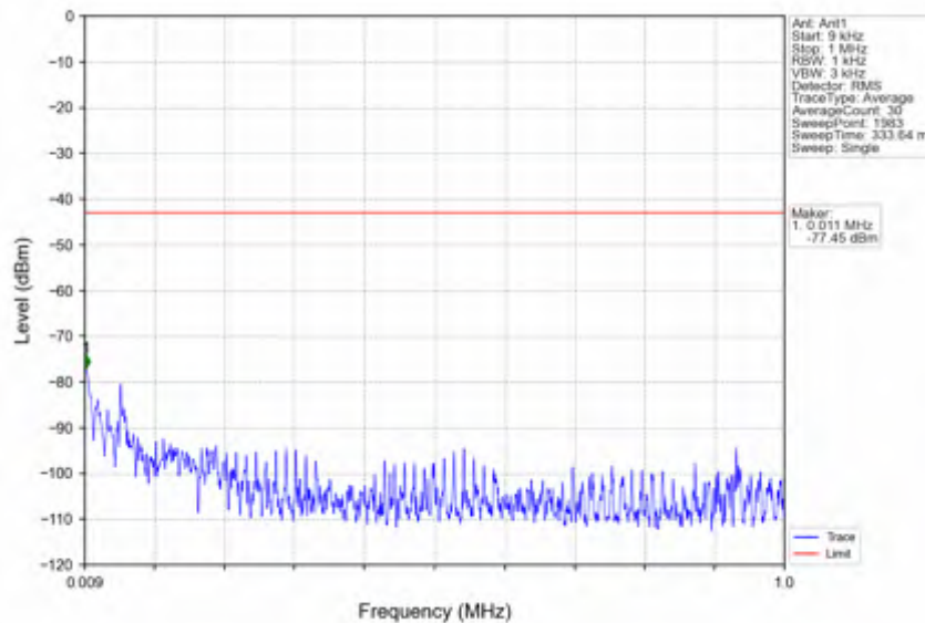
n78e_15kHz_SISO_NTNV_40MHz_DFT-s-OFDM QPSK_3529.995MHz_Outer_Full
