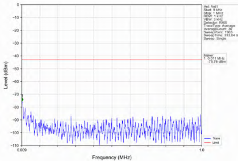
n78e_30kHz_SISO_NTNV_10MHz_DFT-s-OFDM_QPSK_3455.01MHz_Outer_Full
