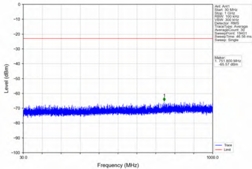
n78e_30kHz_SISO_NTNV_10MHz_CP-OFDM QPSK_3544.98MHz_Outer_Full
