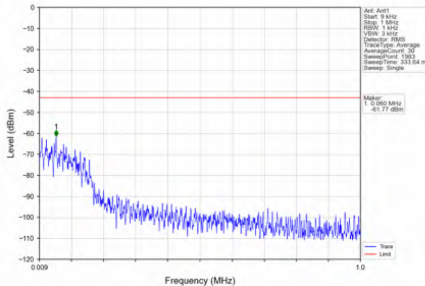
n78e_15kHz_SISO_NTNV_50MHz_CP-OFDM QPSK_3525MHz_Edge_1RB_Right
