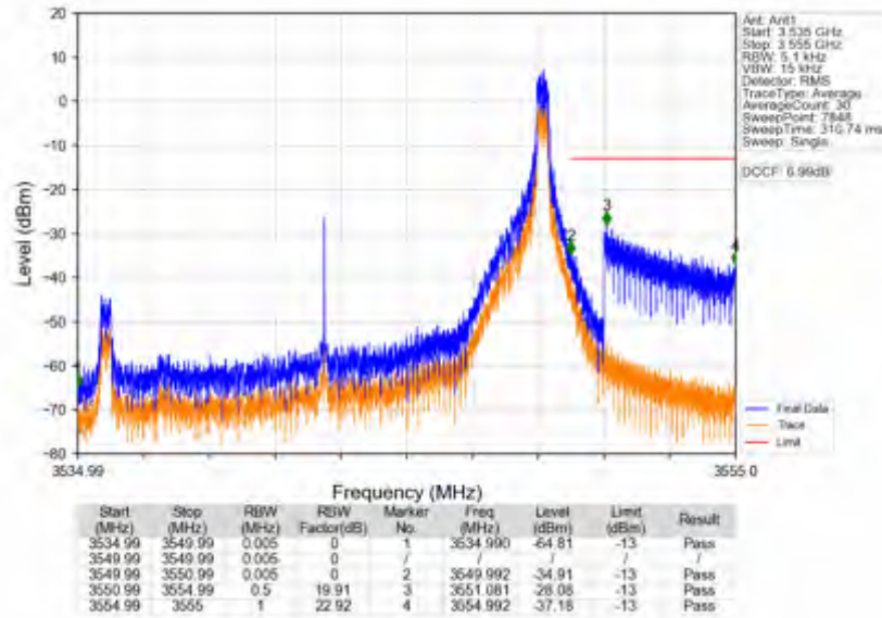
n78e_30kHz_SISO_NTNV_15MHz_DFT-s-OFDM PI/2 BPSK_3542.49MHz_Edge_1RB_Right
