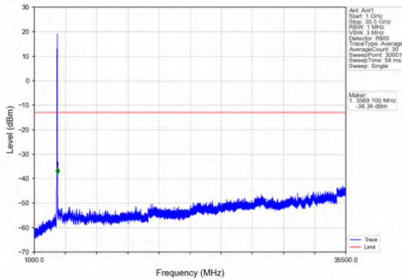
n78e_15kHz_SISO_NTNV_50MHz_CP-OFDM QPSK_3525MHz_Inner_1RB_Right
