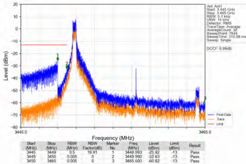
n78e_30kHz_SISO_NTNV_15MHz_DFT-s-OFDM QPSK_3457.5MHz_Edge_1RB_Left
