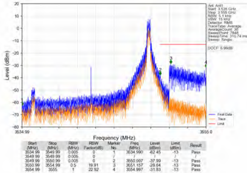
n78e_30kHz_SISO_NTNV_15MHz_CP-OFDM QPSK_3542.49MHz_Inner_1RB_Right
