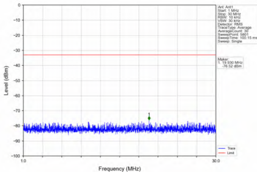
n78e_30kHz_SISO_NTNV_15MHz_DFT-s-OFDM PI/2 BPSK_3457.5MHz_Outer_Full
