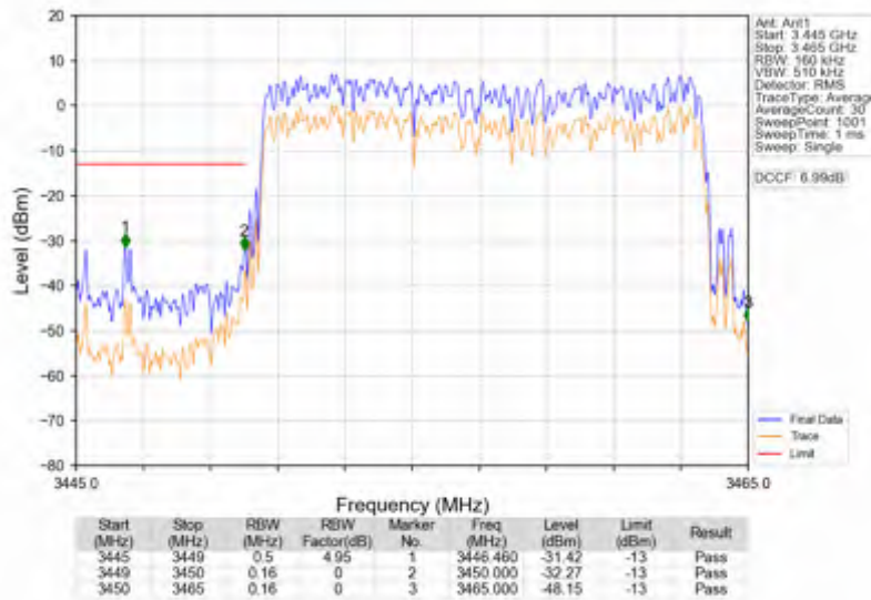
n78e_30kHz_SISO_NTNV_15MHz_DFT-s-OFDM PI/2 BPSK_3457.5MHz_Outer_Full
