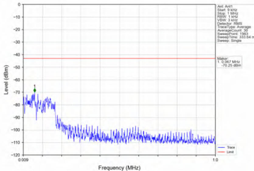
n78e_15kHz_SISO_NTNV_50MHz_DFT-s-OFDM_PI/2_BPSK_3525MHz_Inner_1RB_Right
