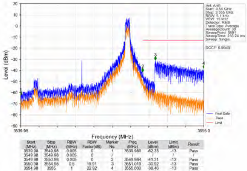
n78e_30kHz_SISO_NTNV_10MHz_DFT-s-OFDM QPSK_3544.98MHz_Inner_1RB_Right
