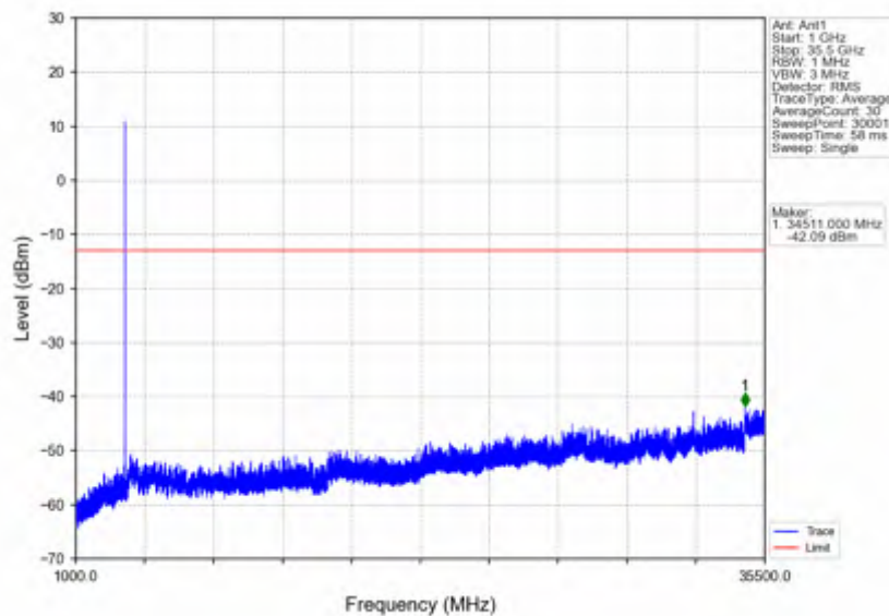
n78e_30kHz_SISO_NTNV_10MHz_DFT-s-OFDM PI/2 BPSK_3455.01MHz_Outer_Full
