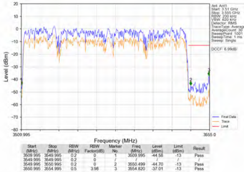
n78e_15kHz_SISO_NTNV_40MHz_DFT-s-OFDM QPSK_3529.995MHz_Outer_Full
