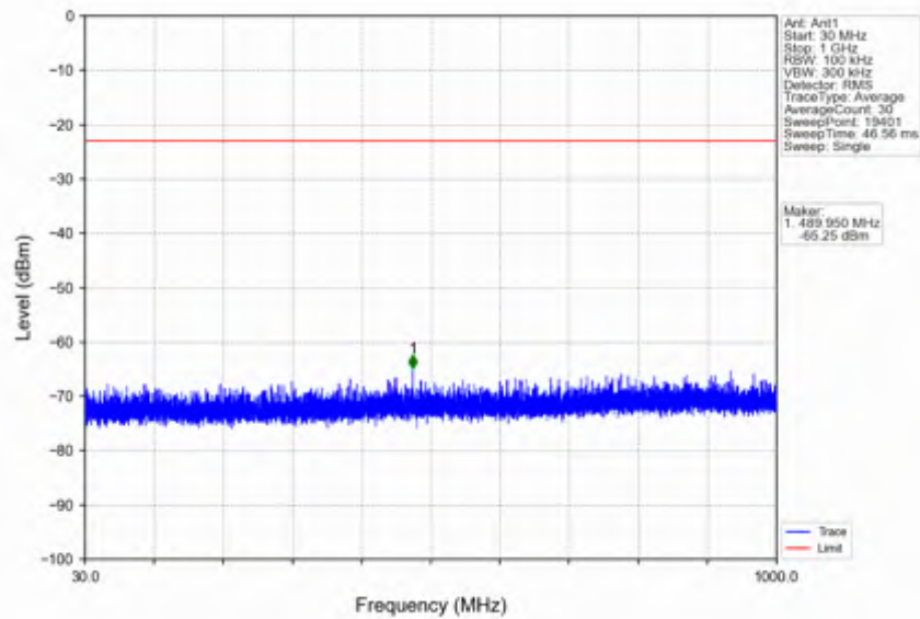
n78e_30kHz_SISO_NTNV_10MHz_DFT-s-OFDM QPSK_3544.98MHz_Inner_1RB_Right
