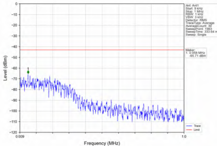
n78e_30kHz_SISO_NTNV_10MHz_CP-OFDM QPSK_3544.98MHz_Inner_1RB_Right
