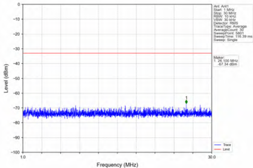
n78e_30kHz_SISO_NTNV_10MHz_DFT-s-OFDM QPSK_3544.98MHz_Edge_1RB_Right
