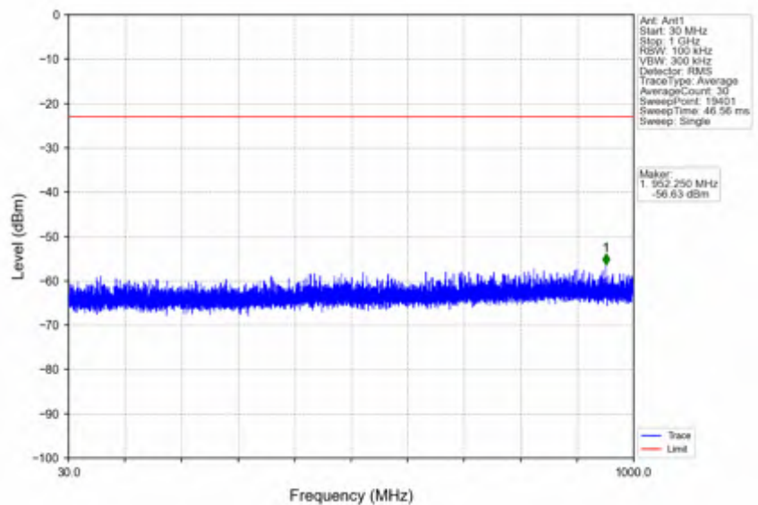
n78e_15kHz_SISO_NTNV_30MHz_CP-OFDM QPSK_3534.99MHz_Edge_1RB_Right
