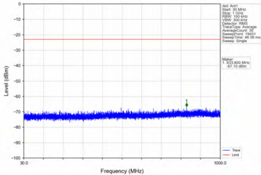
n78e_15kHz_SISO_NTNV_30MHz_DFT-s-OFDM PI/2 BPSK_3534.99MHz_Outer_Full
