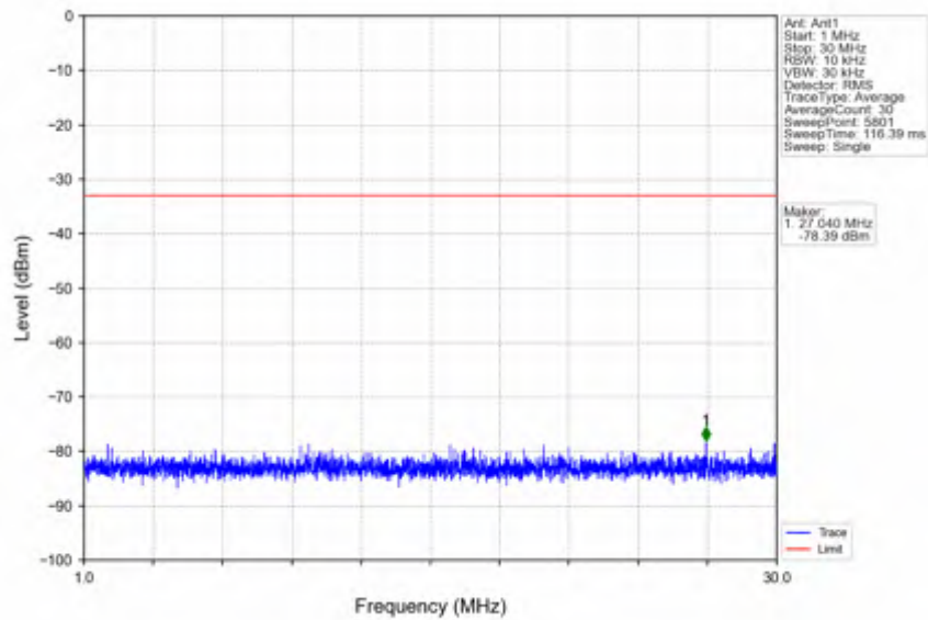
n78e_15kHz_SISO_NTNV_30MHz_CP-OFDM QPSK_3534.99MHz_Inner_1RB_Right
