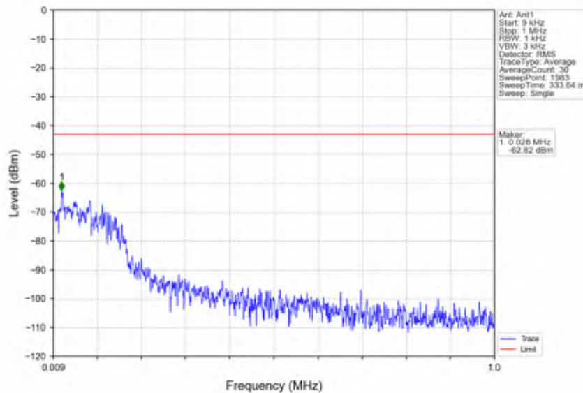
n78e_15kHz_SISO_NTV_25MHz_CP-OFDM_QPSK_3462.51MHz_Inner_1RB_Left
