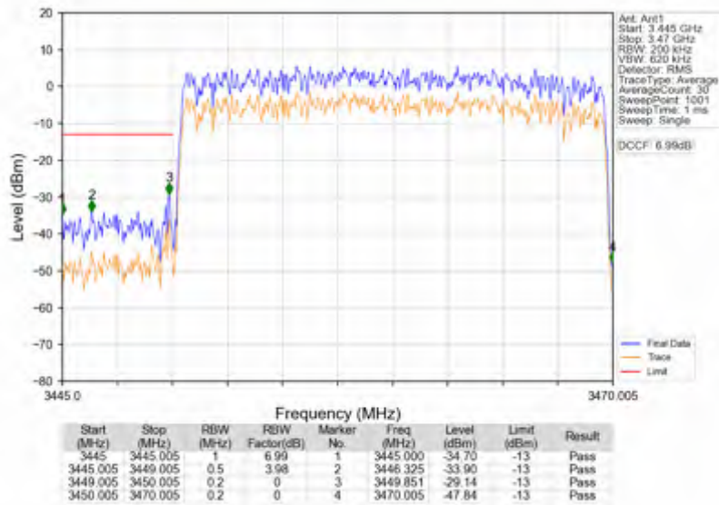
n78e_15kHz_SISO_NTNV_20MHz_CP-OFDM QPSK_3460.005MHz_Outer_Full
