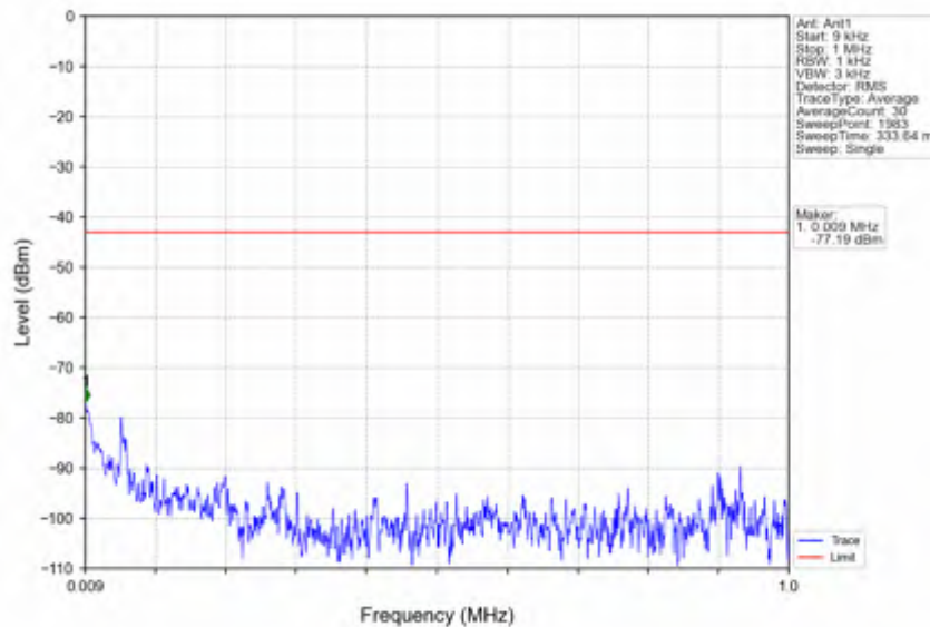
n78e_15kHz_SISO_NTNV_25MHz_DFT-s-OFDM_QPSK_3462.51MHz_Outer_Full
