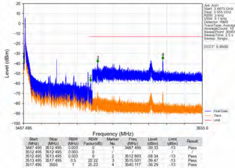
n78e_15kHz_SISO_NTNV_25MHz_DFT-s-OFDM QPSK_3499.995MHz_Edge_1RB_Left
