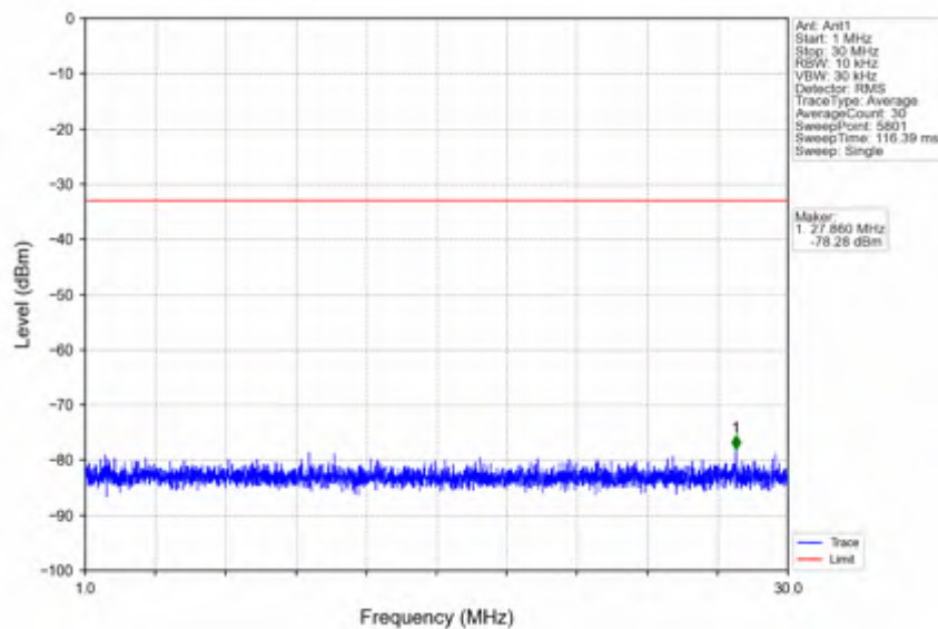
n78e_15kHz_SISO_NTNV_40MHz_DFT-s-OFDM_QPSK_3470.01MHz_Edge_1RB_Left
