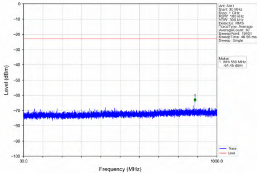
n78e_15kHz_SISO_NTNV_25MHz_DFT-s-OFDM QPSK_3462.51MHz_Inner_1RB_Left
