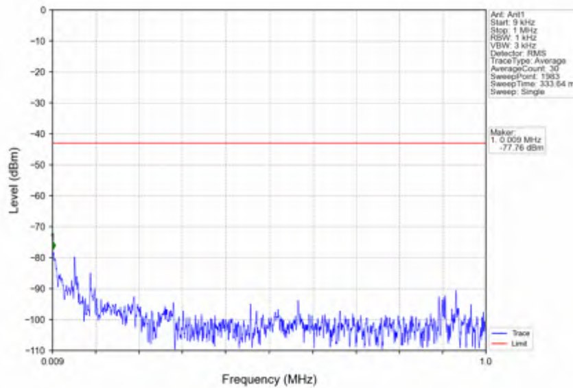
n78e_15kHz_SISO_NTNV_25MHz_DFT-s-OFDM QPSK_3537.495MHz_Outer_Full
