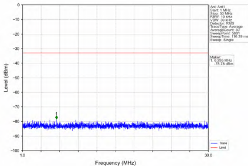
n78e_15kHz_SISO_NTV_25MHz_DFT-s-OFDM_QPSK_3537.495MHz_Inner_1RB_Right
