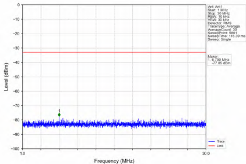
n78e_15kHz_SISO_NTNV_30MHz_DFT-s-OFDM PI/2 BPSK_3465MHz_Outer_Full
