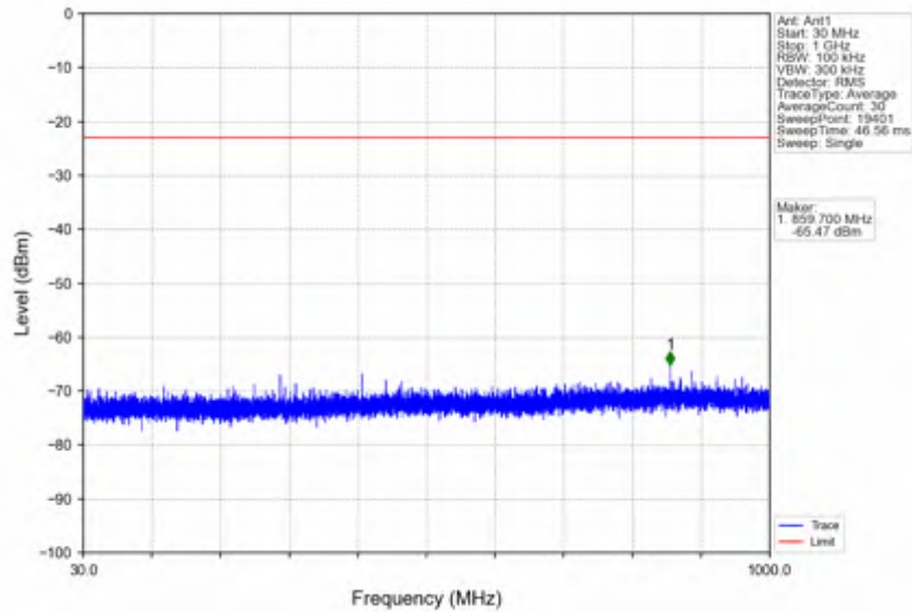
n78e_15kHz_SISO_NTNV_40MHz_DFT-s-OFDM_QPSK_3470.01MHz_Inner_1RB_Left
