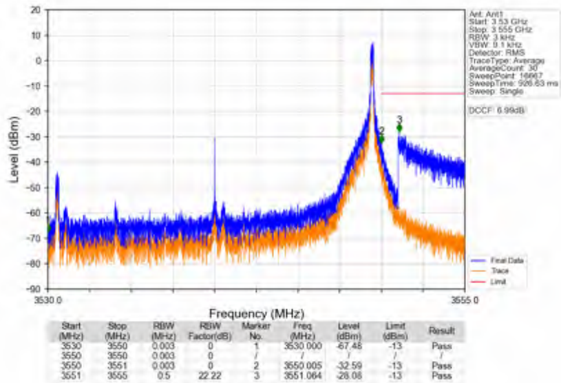
n78e_15kHz_SISO_NTNV_20MHz_DFT-s-OFDM QPSK_3540MHz_Edge_1RB_Right
