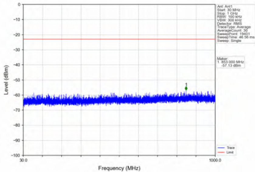
n78e_15kHz_SISO_NTNV_25MHz_DFT-s-OFDM QPSK_3462.51MHz_Edge_1RB_Left
