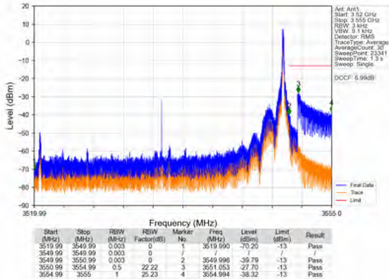
n78e_15kHz_SISO_NTNV_30MHz_DFT-s-OFDM QPSK_3534.99MHz_Edge_1RB_Right
