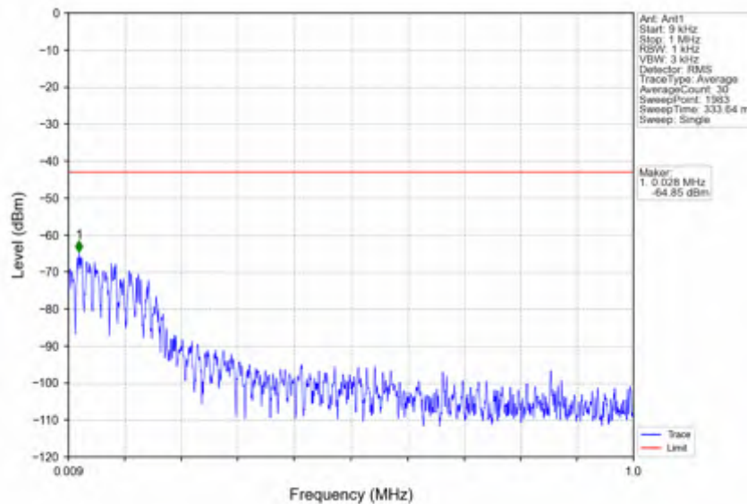
n78e_15kHz_SISO_NTV_30MHz_CP-OFDM QPSK_3534.99MHz_Inner_1RB_Right
