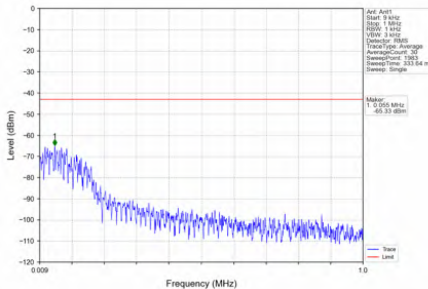
n78e_15kHz_SISO_NTNV_20MHz_CP-OFDM QPSK_3540MHz_Inner_1RB_Right
