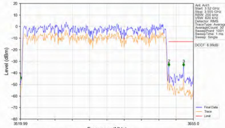
n78e_15kHz_SISO_NTNV_30MHz_DFT-s-OFDM_QPSK_3534.99MHz_Outer_Full
