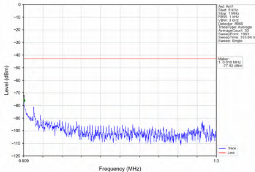
n78e_15kHz_SISO_NTNV_30MHz_DFT-s-OFDM_QPSK_3534.99MHz_Outer_Full
