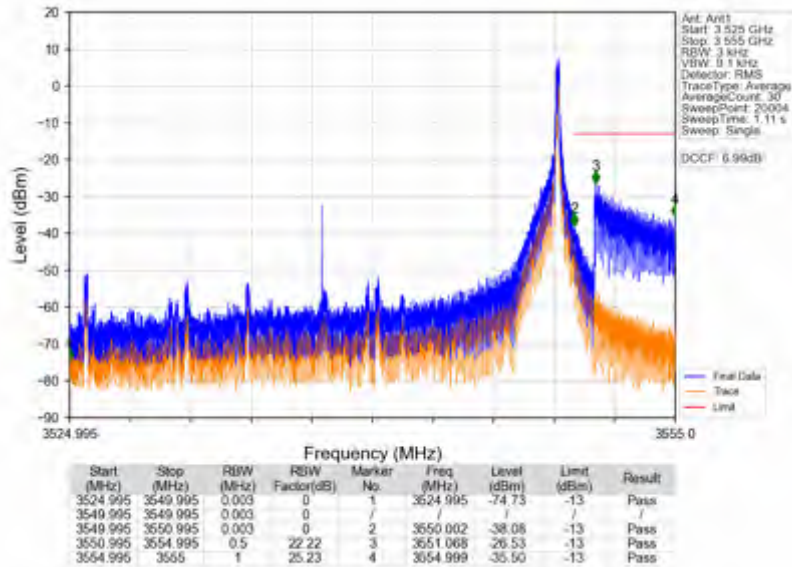
n78e_15kHz_SISO_NTNV_25MHz_DFT-s-OFDM QPSK_3537.495MHz_Inner_1RB_Right
