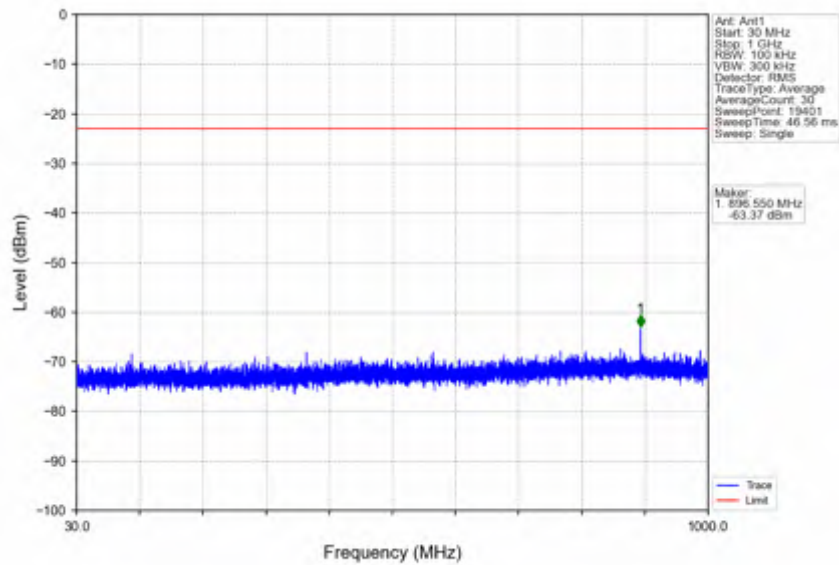
n78e_15kHz_SISO_NTV_25MHz_DFT-s-OFDM_QPSK_3537.495MHz_Inner_1RB_Right
