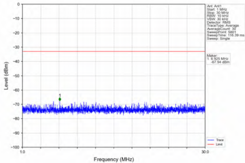
n78e_15kHz_SISO_NTV_25MHz_CP-OFDM QPSK_3537.495MHz_Edge_1RB_Right
