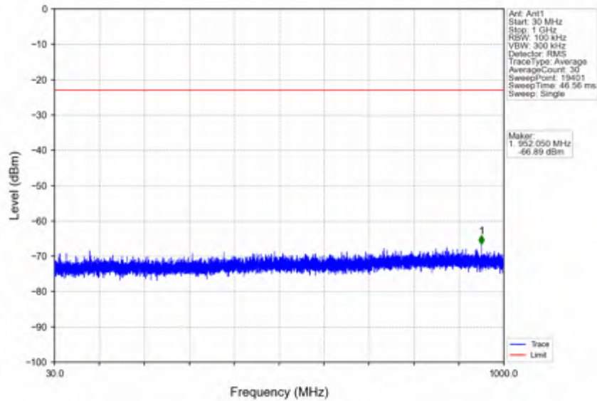
n78e_15kHz_SISO_NTNV_30MHz_DFT-s-OFDM QPSK_3534.99MHz_Inner_1RB_Right
