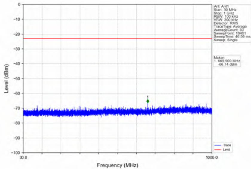
n78e_15kHz_SISO_NTNV_30MHz_CP-OFDM QPSK_3465MHz_Outer_Full
