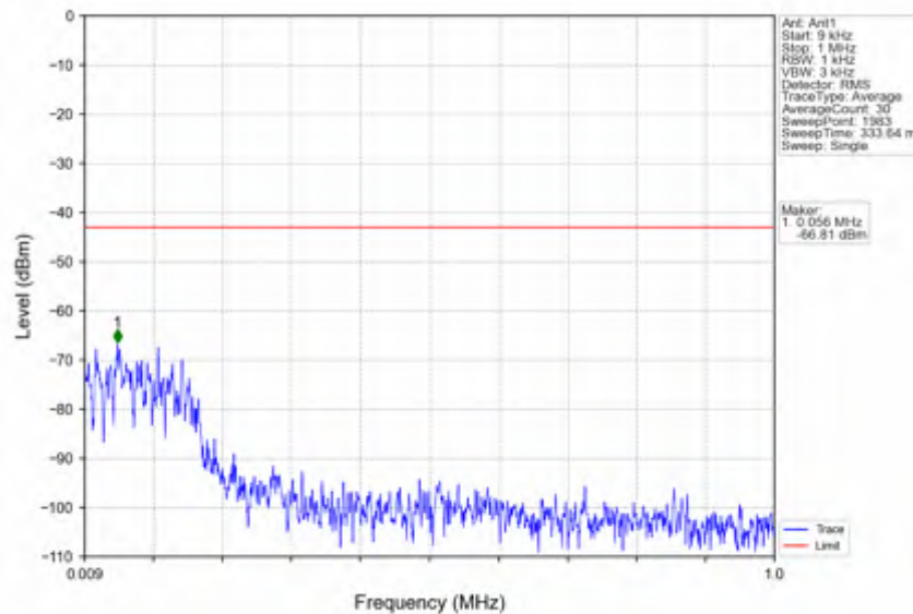
n78e_15kHz_SISO_NTNV_30MHz_DFT-s-OFDM QPSK_3499.995MHz_Edge_1RB_Left
