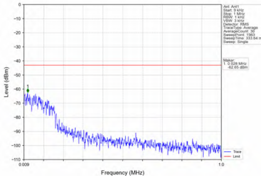
n78e_15kHz_SISO_NTV_25MHz_CP-OFDM QPSK_3462.51MHz_Edge_1RB_Left
