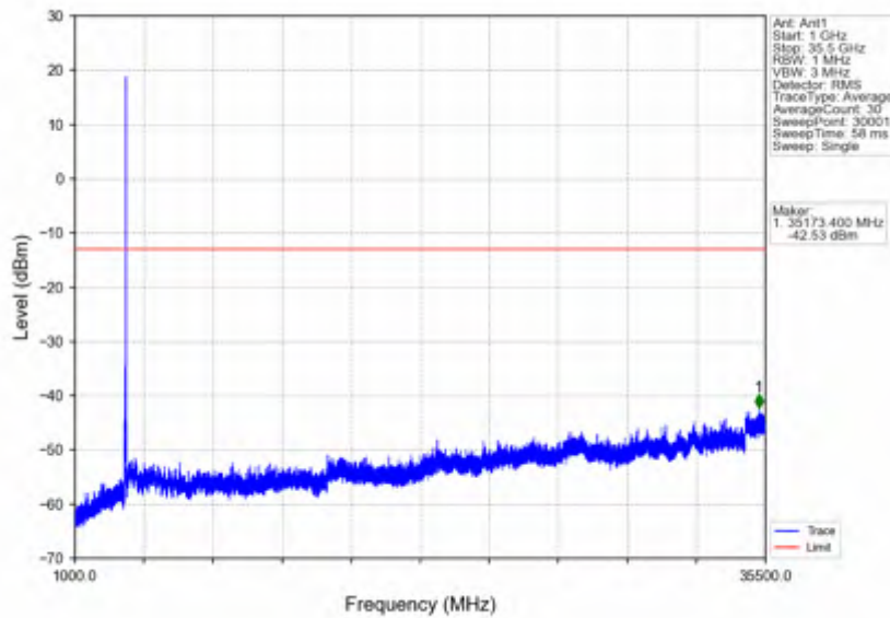
n78e_15kHz_SISO_NTNV_40MHz_DFT-s-OFDM PI/2 BPSK_3529.995MHz_Outer_Full
