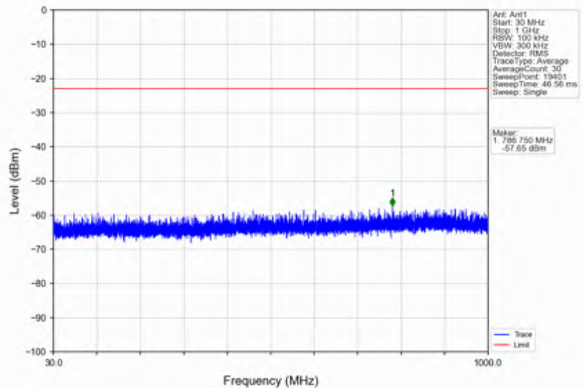
n78e_15kHz_SISO_NTV_20MHz_DFT-s-OFDM_PI/2_BPSK_3540MHz_Edge_1RB_Right
