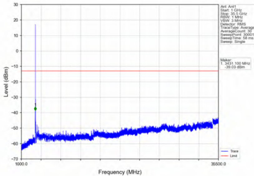
n78e_15kHz_SISO_NTV_25MHz_CP-OFDM QPSK_3462.51MHz_Outer_Full
