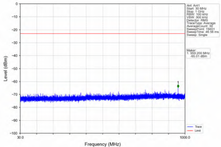
n78e_15kHz_SISO_NTV_25MHz_CP-OFDM QPSK_3537.495MHz_Inner_1RB_Right
