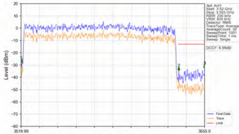
n78e_15kHz_SISO_NTNV_30MHz_CP-OFDM QPSK_3534.99MHz_Outer_Full
