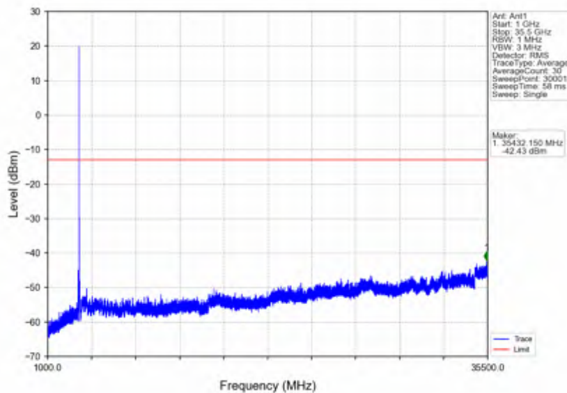
n78e_15kHz_SISO_NTNV_25MHz_DFT-s-OFDM QPSK_3462.51MHz_Edge_1RB_Left
