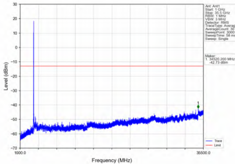
n78e_15kHz_SISO_NTNV_40MHz_DFT-s-OFDM QPSK_3470.01MHz_Edge_1RB_Left
