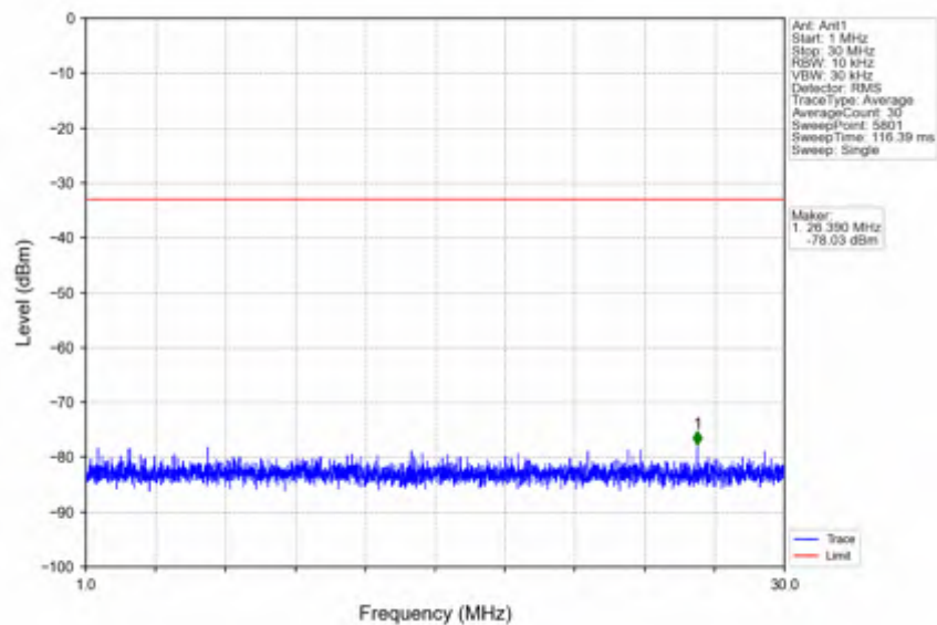
n78e_15kHz_SISO_NTNV_25MHz_CP-OFDM QPSK_3537.495MHz_Outer_Full
