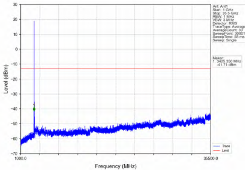
n78e_15kHz_SISO_NTNV_40MHz_DFT-s-OFDM PI/2 BPSK_3470.01MHz_Outer_Full
