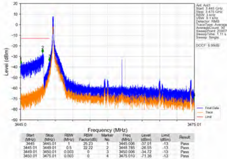
n78e_15kHz_SISO_NTV_25MHz_CP-OFDM QPSK_3462.51MHz_Edge_1RB_Left
