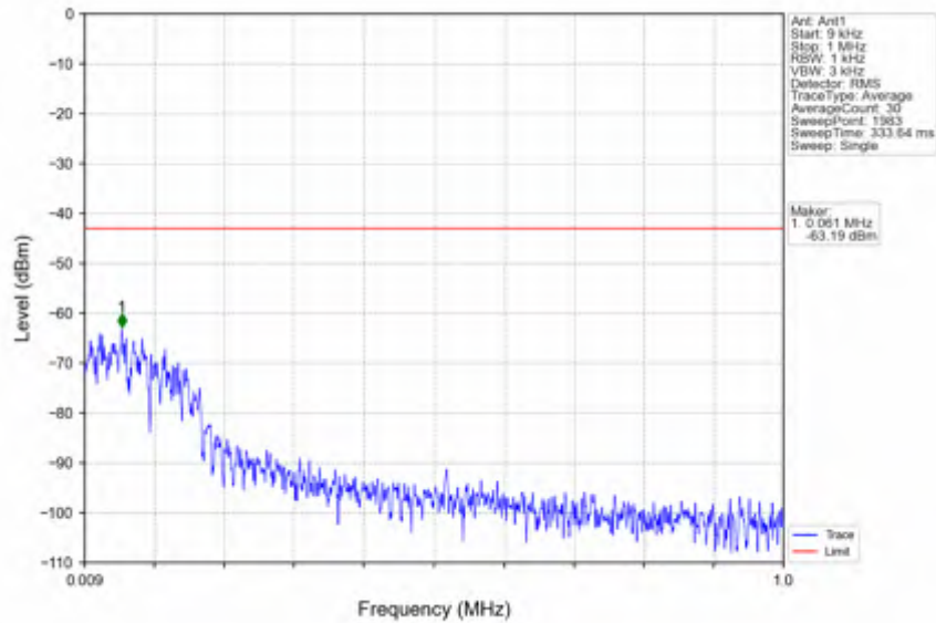
n78e_15kHz_SISO_NTNV_25MHz_CP-OFDM QPSK_3499.995MHz_Edge_1RB_Left
