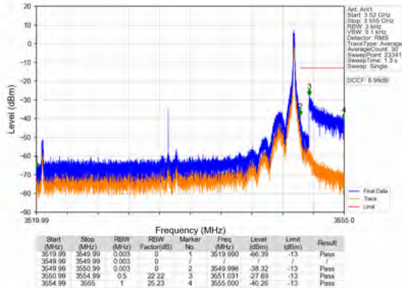
n78e_15kHz_SISO_NTV_30MHz_CP-OFDM QPSK_3534.99MHz_Edge_1RB_Right
