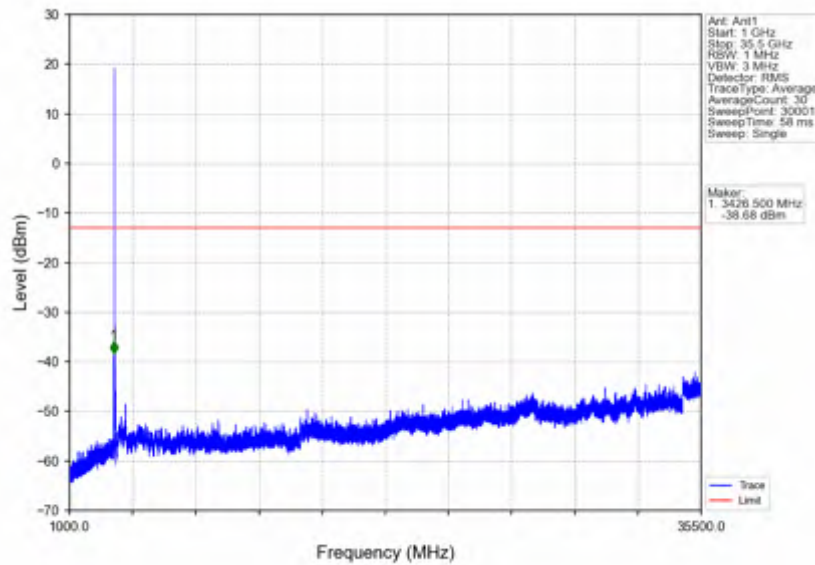
n78e_15kHz_SISO_NTNV_25MHz_DFT-s-OFDM PI/2 BPSK_3499.995MHz_Edge_1RB_Left
