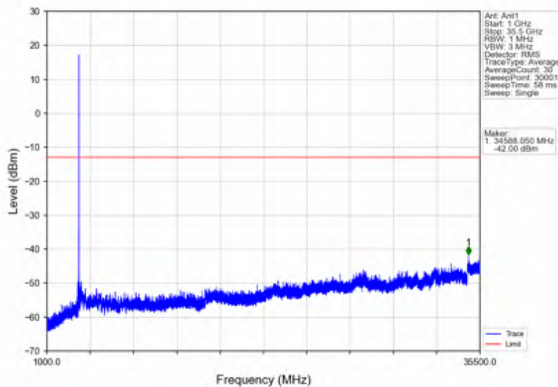
n78e_15kHz_SISO_NTV_25MHz_DFT-s-OFDM_QPSK_3537.495MHz_Edge_1RB_Right
