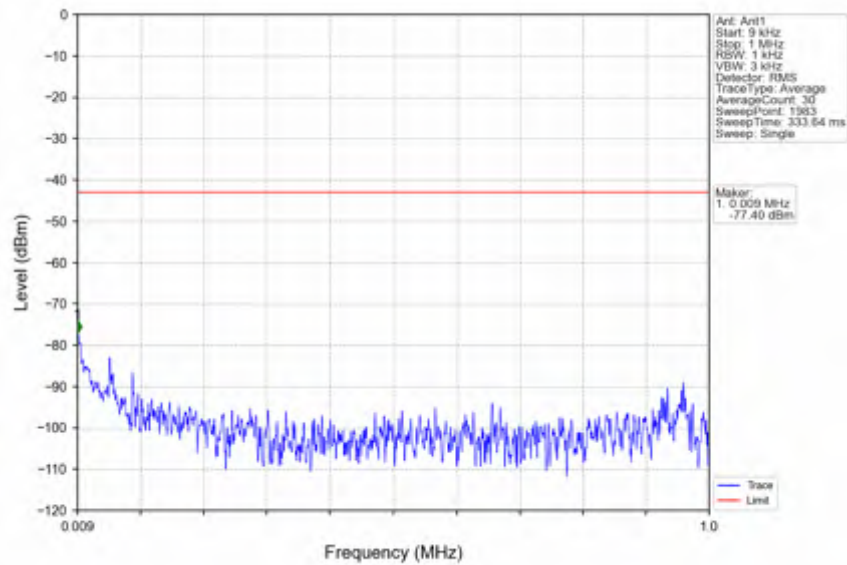
n78e_15kHz_SISO_NTNV_20MHz_DFT-s-OFDM PI/2 BPSK_3540MHz_Outer_Full
