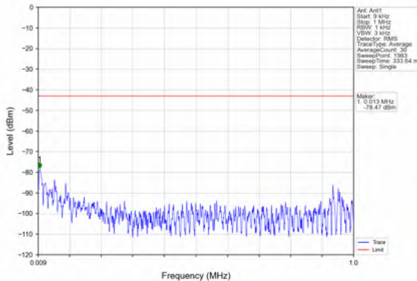
n78e_15kHz_SISO_NTNV_20MHz_DFT-s-OFDM QPSK_3460.005MHz_Outer_Full
