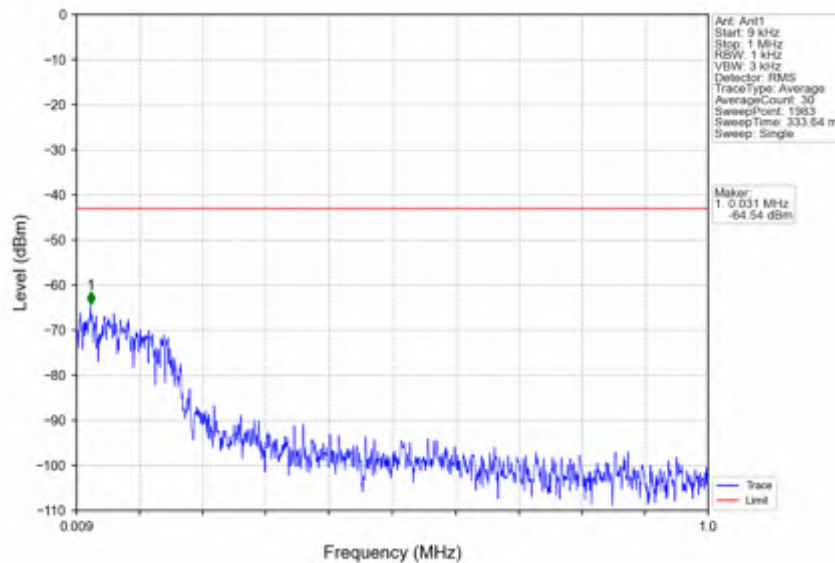
n78e_15kHz_SISO_NTV_30MHz_CP-OFDM QPSK_3534.99MHz_Edge_1RB_Right
