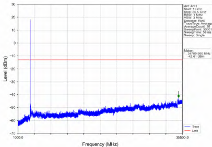
n78e_15kHz_SISO_NTV_25MHz_DFT-s-OFDM_QPSK_3537.495MHz_Inner_1RB_Right
