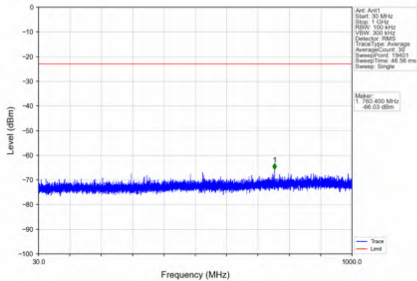
n78e_15kHz_SISO_NTNV_20MHz_DFT-s-OFDM QPSK_3540MHz_Inner_1RB_Right
