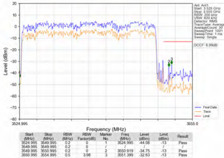
n78e_15kHz_SISO_NTNV_25MHz_DFT-s-OFDM QPSK_3537.495MHz_Outer_Full
