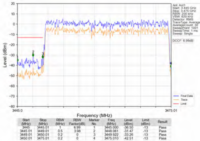
n78e_15kHz_SISO_NTV_25MHz_CP-OFDM QPSK_3462.51MHz_Outer_Full
