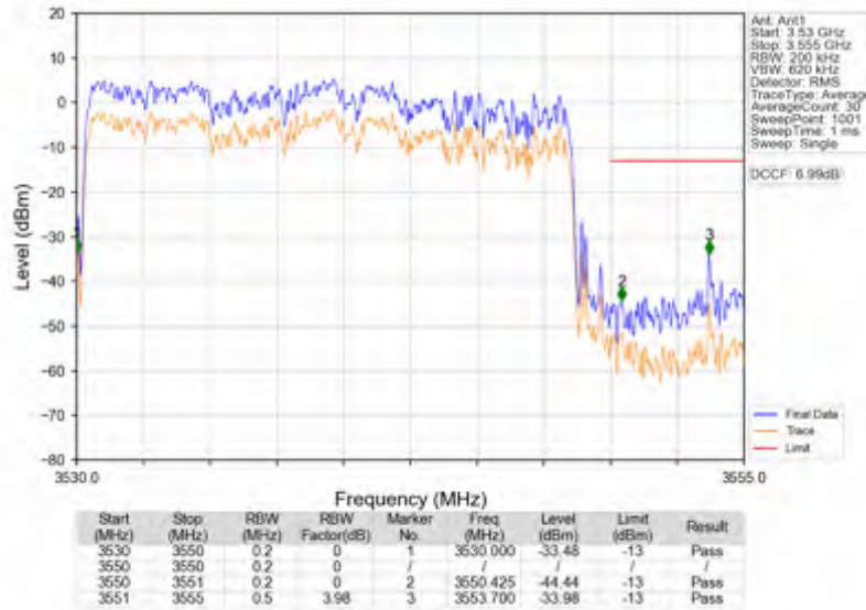
n78e_15kHz_SISO_NTNV_20MHz_DFT-s-OFDM_QPSK_3540MHz_Outer_Full
