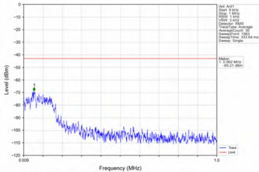
n78e_15kHz_SISO_NTNV_20MHz_DFT-s-OFDM_QPSK_3540MHz_Inner_1RB_Right
