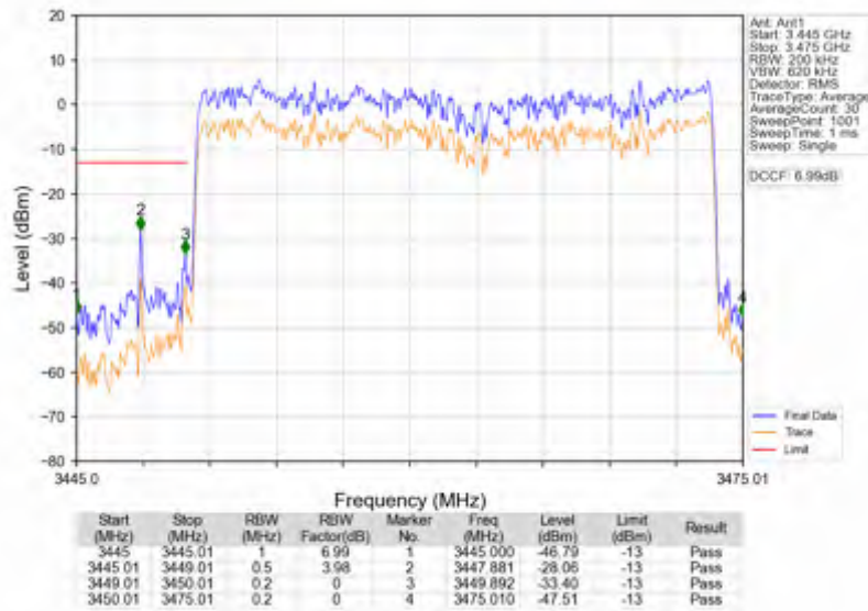
n78e_15kHz_SISO_NTNV_25MHz_DFT-s-OFDM PI/2 BPSK_3462.51MHz_Outer_Full
