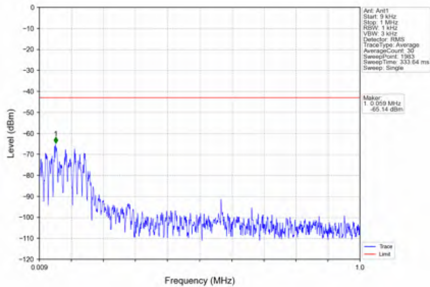
n78e_15kHz_SISO_NTNV_25MHz_DFT-s-OFDM_QPSK_3462.51MHz_Inner_1RB_Left
