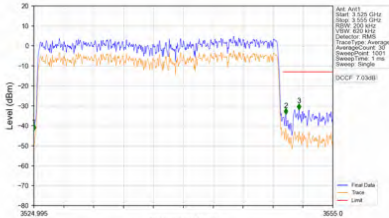
n78e_15kHz_SISO_NTV_25MHz_CP-OFDM QPSK_3537.495MHz_Outer_Full
