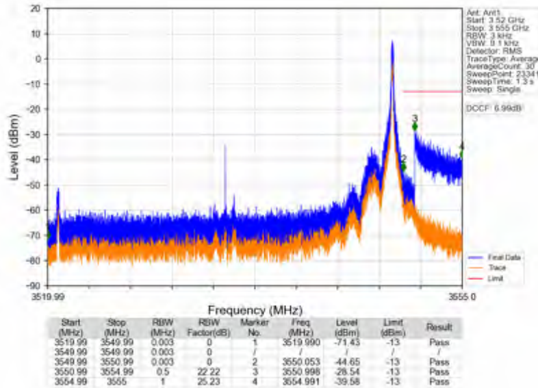
n78e_15kHz_SISO_NTV_30MHz_CP-OFDM QPSK_3534.99MHz_Inner_1RB_Right
