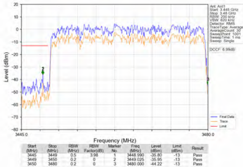
n78e_15kHz_SISO_NTNV_30MHz_DFT-s-OFDM PI/2 BPSK_3465MHz_Outer_Full
