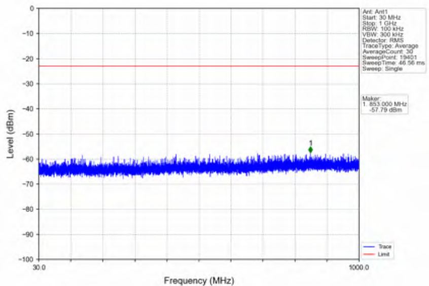
n78e_15kHz_SISO_NTV_25MHz_CP-OFDM QPSK_3462.51MHz_Edge_1RB_Left
