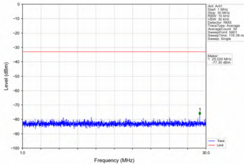
n78e_15kHz_SISO_NTNV_20MHz_DFT-s-OFDM QPSK_3460.005MHz_Outer_Full
