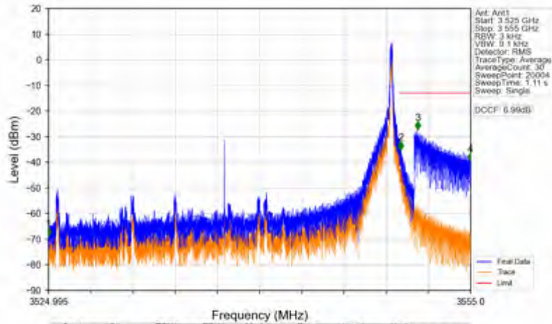
n78e_15kHz_SISO_NTNV_25MHz_DFT-s-OFDM QPSK_3537.495MHz_Edge_1RB_Right
