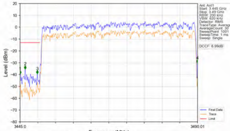
n78e_15kHz_SISO_NTNV_40MHz_DFT-s-OFDM_QPSK_3470.01MHz_Outer_Full
