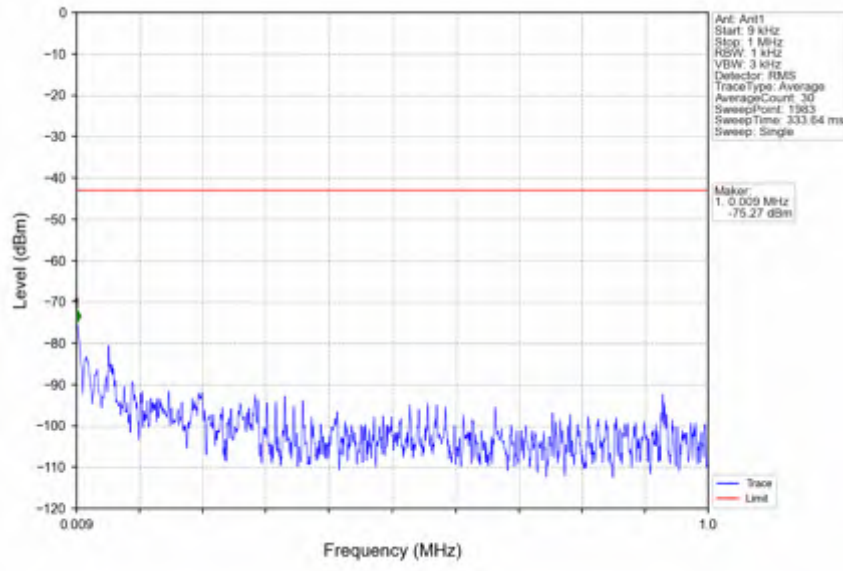
n78e_15kHz_SISO_NTNV_40MHz_DFT-s-OFDM_QPSK_3470.01MHz_Outer_Full
