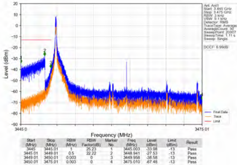
n78e_15kHz_SISO_NTV_25MHz_CP-OFDM_QPSK_3462.51MHz_Inner_1RB_Left
