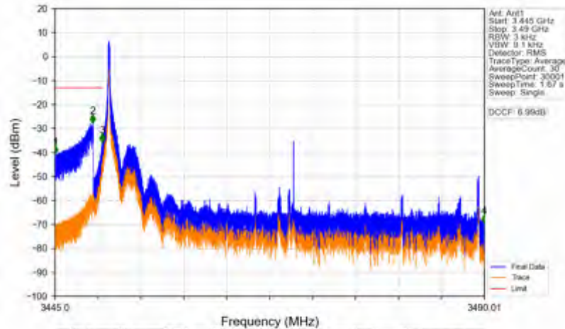
n78e_15kHz_SISO_NTNV_40MHz_DFT-s-OFDM QPSK_3470.01MHz_Edge_1RB_Left
