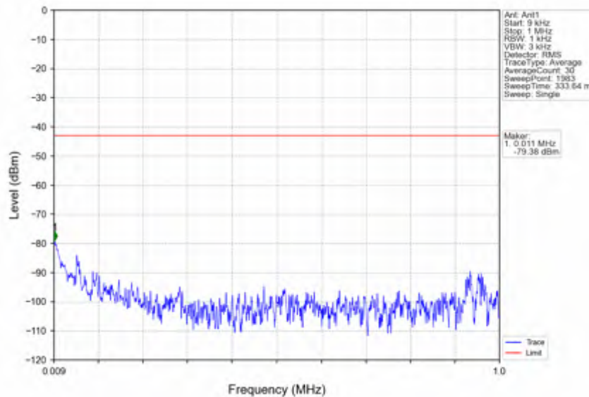
n78e_15kHz_SISO_NTNV_20MHz_DFT-s-OFDM_QPSK_3540MHz_Outer_Full
