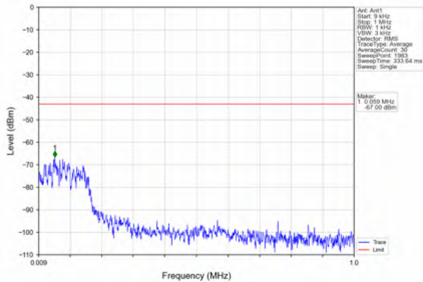
n78e_15kHz_SISO_NTNV_25MHz_DFT-s-OFDM QPSK_3462.51MHz_Edge_1RB_Left
