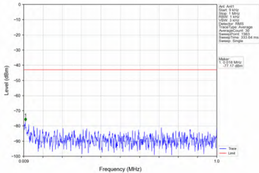
n78e_15kHz_SISO_NTNV_25MHz_CP-OFDM QPSK_3462.51MHz_Outer_Full
