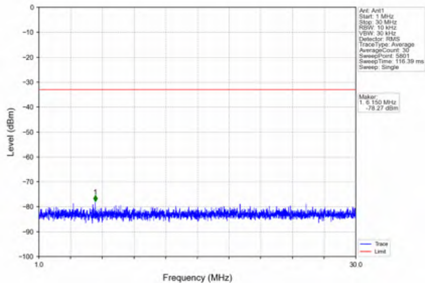
n78e_15kHz_SISO_NTNV_20MHz_CP-OFDM_QPSK_3540MHz_Outer_Full
