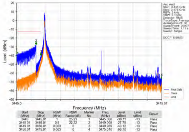
n78e_15kHz_SISO_NTNV_25MHz_DFT-s-OFDM PI/2 BPSK_3462.51MHz_Inner_1RB_Left
