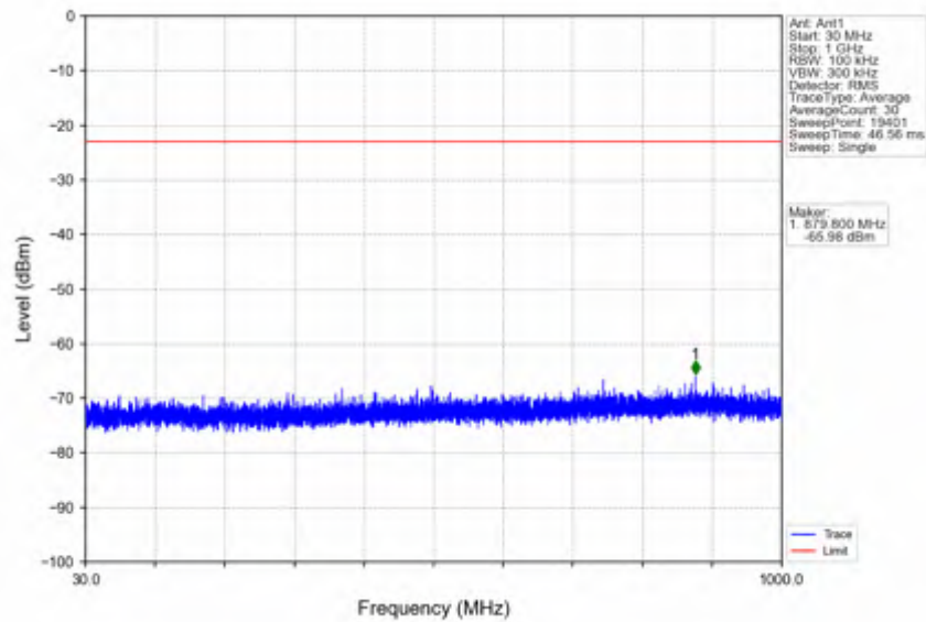
n78e_15kHz_SISO_NTNV_30MHz_CP-OFDM QPSK_3534.99MHz_Outer_Full
