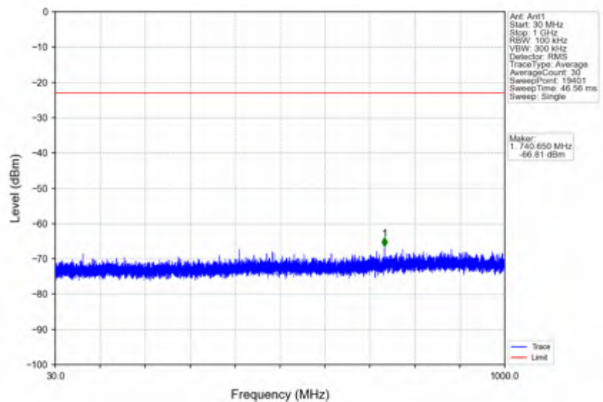
n78e_15kHz_SISO_NTNV_20MHz_DFT-s-OFDM_QPSK_3540MHz_Outer_Full
