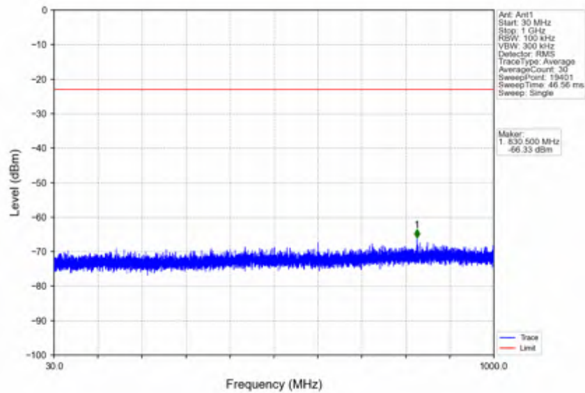
n78e_15kHz_SISO_NTNV_20MHz_CP-OFDM QPSK_3460.005MHz_Outer_Full
