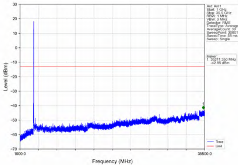
n78e_15kHz_SISO_NTV_25MHz_CP-OFDM QPSK_3537.495MHz_Outer_Full
