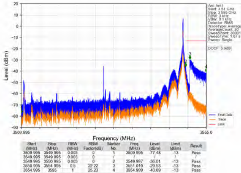
n78e_15kHz_SISO_NTNV_40MHz_DFT-s-OFDM QPSK_3529.995MHz_Edge_1RB_Right
