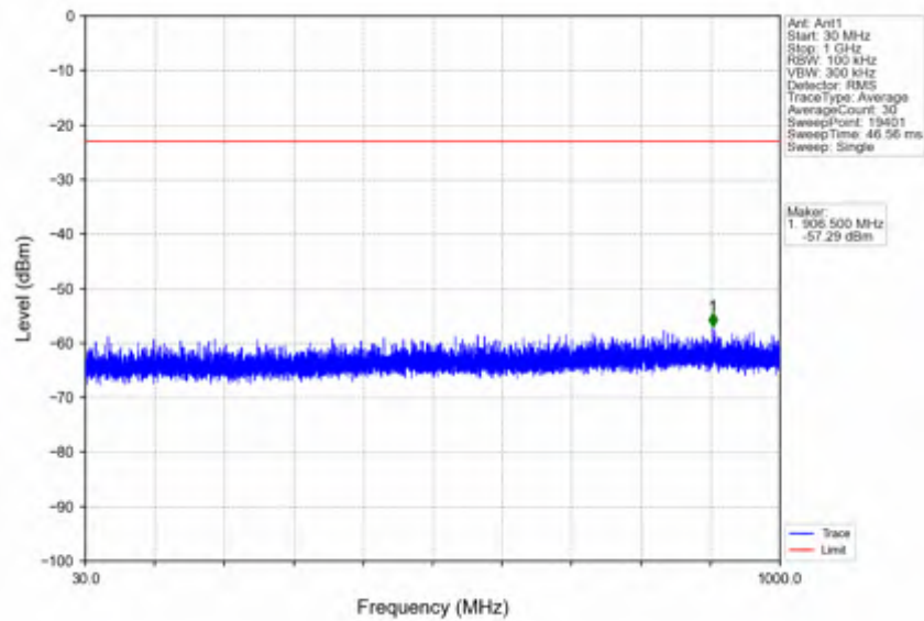
n78e_15kHz_SISO_NTNV_25MHz_CP-OFDM QPSK_3499.995MHz_Edge_1RB_Left
