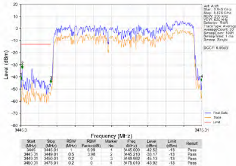
n78e_15kHz_SISO_NTNV_25MHz_DFT-s-OFDM_QPSK_3462.51MHz_Outer_Full
