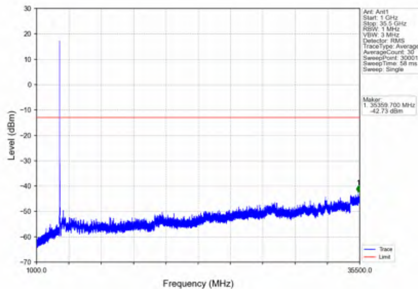
n78e_15kHz_SISO_NTNV_40MHz_DFT-s-OFDM QPSK_3470.01MHz_Edge_1RB_Left
