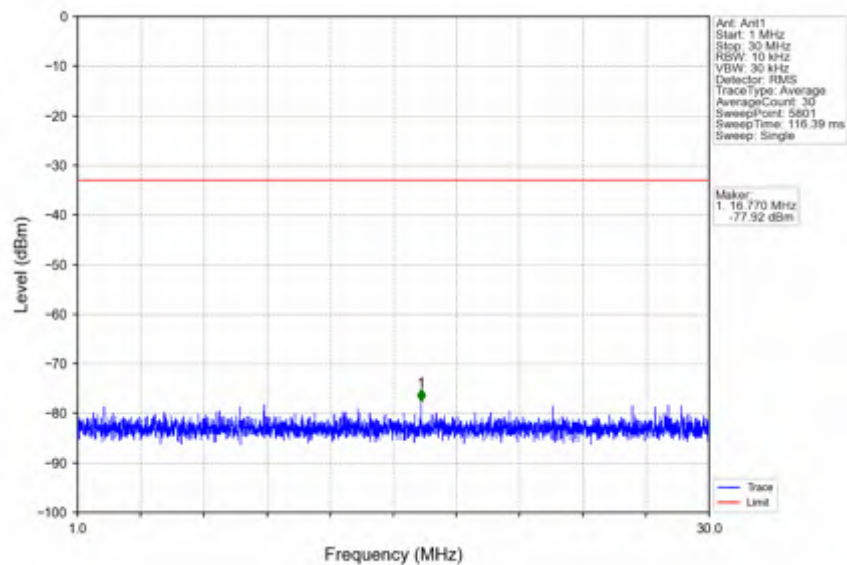
n78e_15kHz_SISO_NTNV_20MHz_CP-OFDM QPSK_3460.005MHz_Outer_Full
