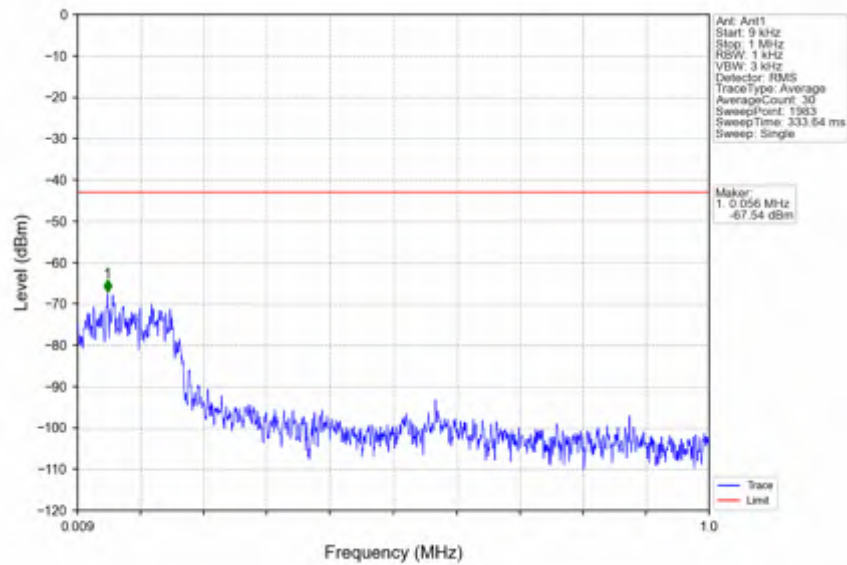
n78e_15kHz_SISO_NTV_20MHz_DFT-s-OFDM_QPSK_3540MHz_Edge_1RB_Right
