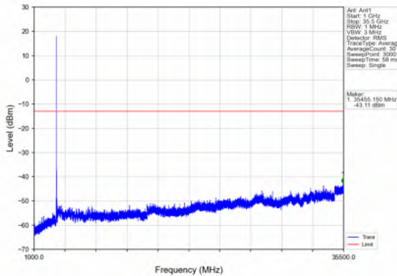
n78e_15kHz_SISO_NTNV_40MHz_DFT-s-OFDM QPSK_3529.995MHz_Edge_1RB_Right
