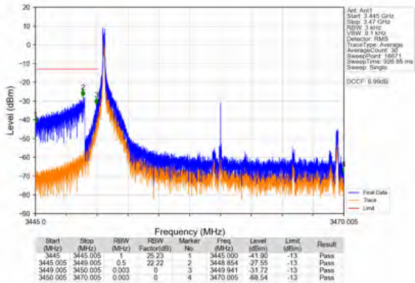
n78e_15kHz_SISO_NTNV_20MHz_DFT-s-OFDM QPSK_3460.005MHz_Edge_1RB_Left
