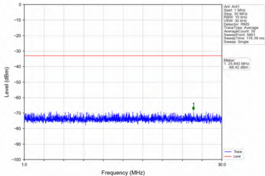
n78e_15kHz_SISO_NTV_30MHz_DFT-s-OFDM_QPSK_3465MHz_Edge_1RB_Left
