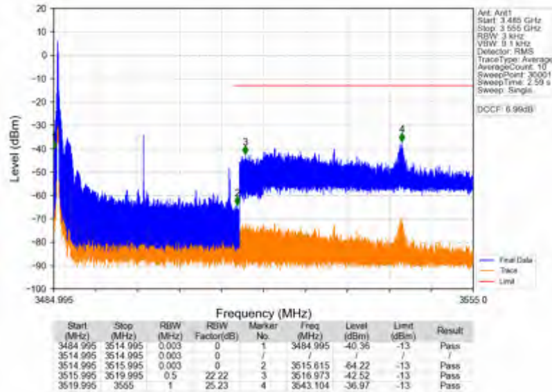
n78e_15kHz_SISO_NTNV_30MHz_DFT-s-OFDM QPSK_3499.995MHz_Edge_1RB_Left
