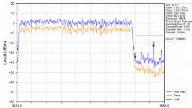
n78e_15kHz_SISO_NTNV_20MHz_CP-OFDM QPSK_3540MHz_Outer_Full
