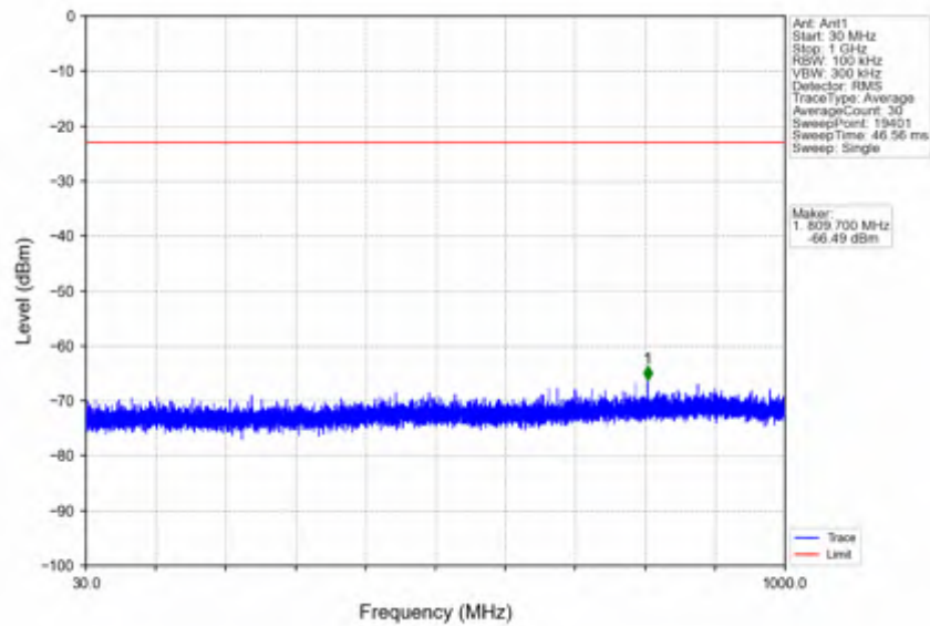
n78e_15kHz_SISO_NTNV_25MHz_CP-OFDM QPSK_3462.51MHz_Outer_Full
