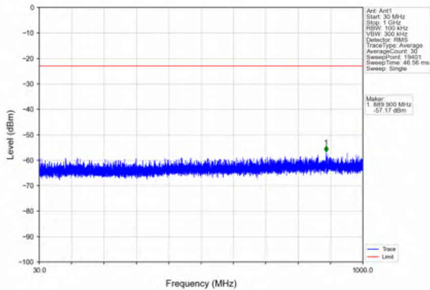
n78e_15kHz_SISO_NTV_25MHz_DFT-s-OFDM_QPSK_3537.495MHz_Edge_1RB_Right
