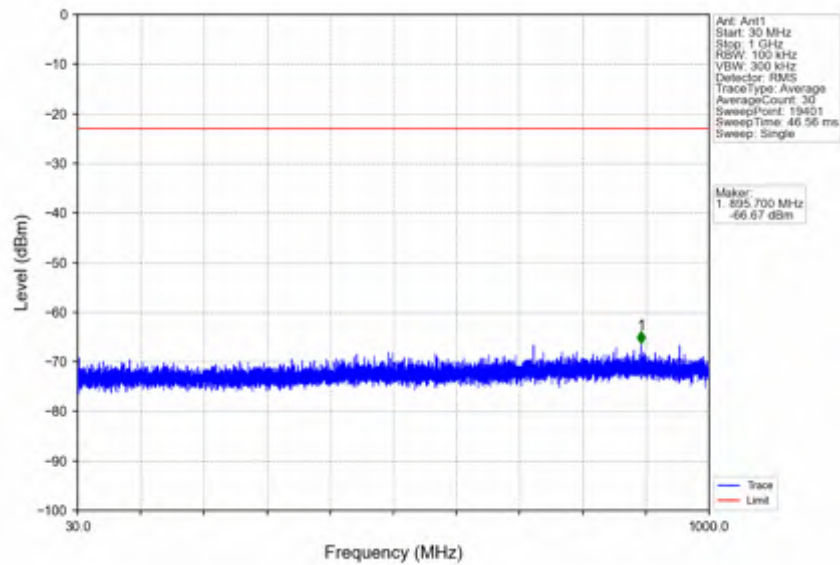
n78e_15kHz_SISO_NTNV_25MHz_CP-OFDM QPSK_3537.495MHz_Outer_Full
