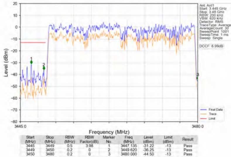
n78e_15kHz_SISO_NTNV_30MHz_DFT-s-OFDM_QPSK_3465MHz_Outer_Full
