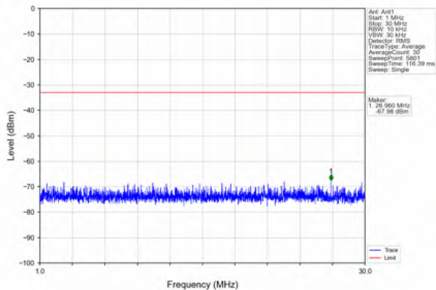
n78e_15kHz_SISO_NTV_25MHz_DFT-s-OFDM QPSK_3537.495MHz_Edge_1RB_Right
