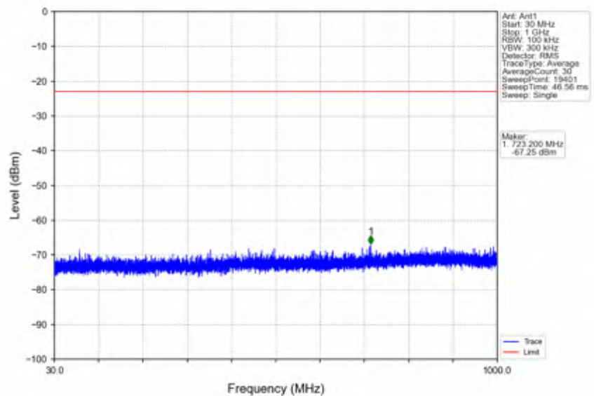
n78e_15kHz_SISO_NTNV_40MHz_DFT-s-OFDM_QPSK_3470.01MHz_Outer_Full
