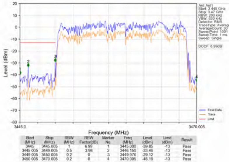
n78e_15kHz_SISO_NTNV_20MHz_DFT-s-OFDM QPSK_3460.005MHz_Outer_Full
