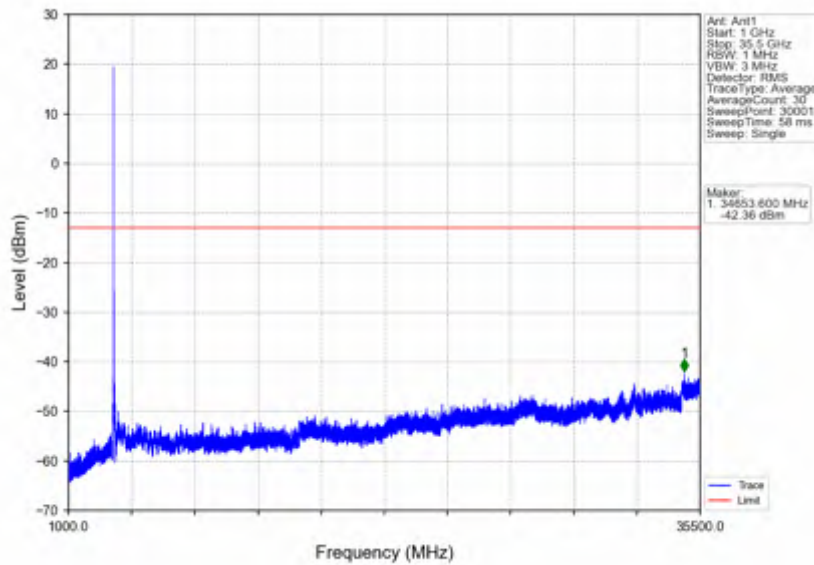
n78e_15kHz_SISO_NTV_25MHz_CP-OFDM_QPSK_3499.995MHz_Edge_1RB_Left
