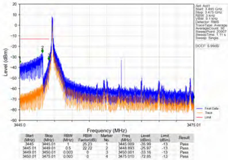
n78e_15kHz_SISO_NTNV_25MHz_DFT-s-OFDM QPSK_3462.51MHz_Edge_1RB_Left
