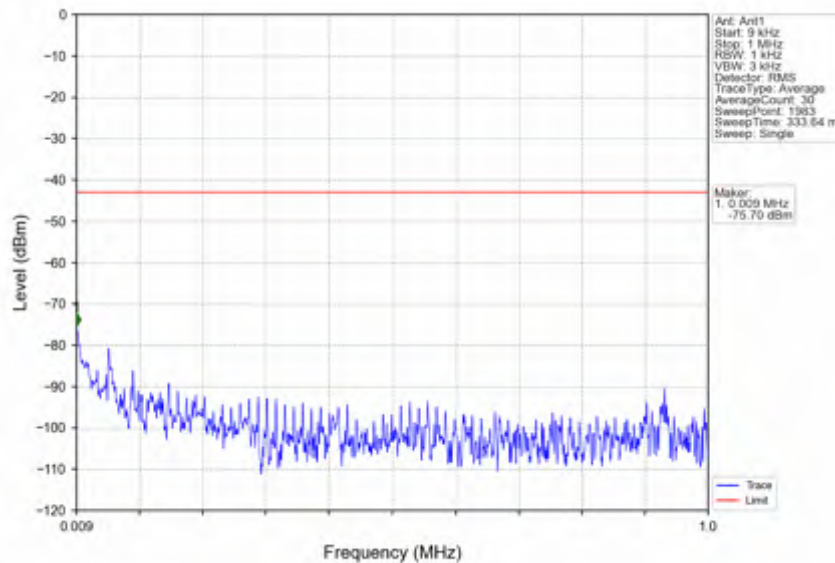
n78e_15kHz_SISO_NTNV_30MHz_DFT-s-OFDM_QPSK_3465MHz_Outer_Full
