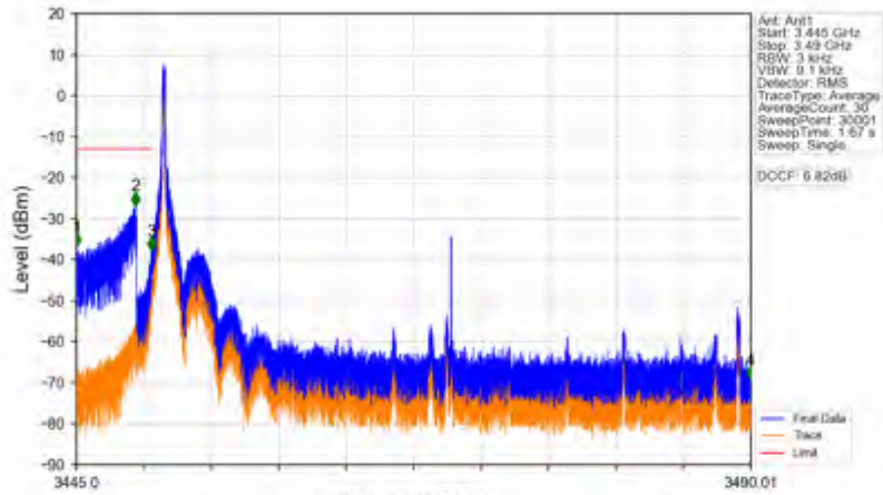
n78e_15kHz_SISO_NTNV_40MHz_DFT-s-OFDM_QPSK_3470.01MHz_Inner_1RB_Left
