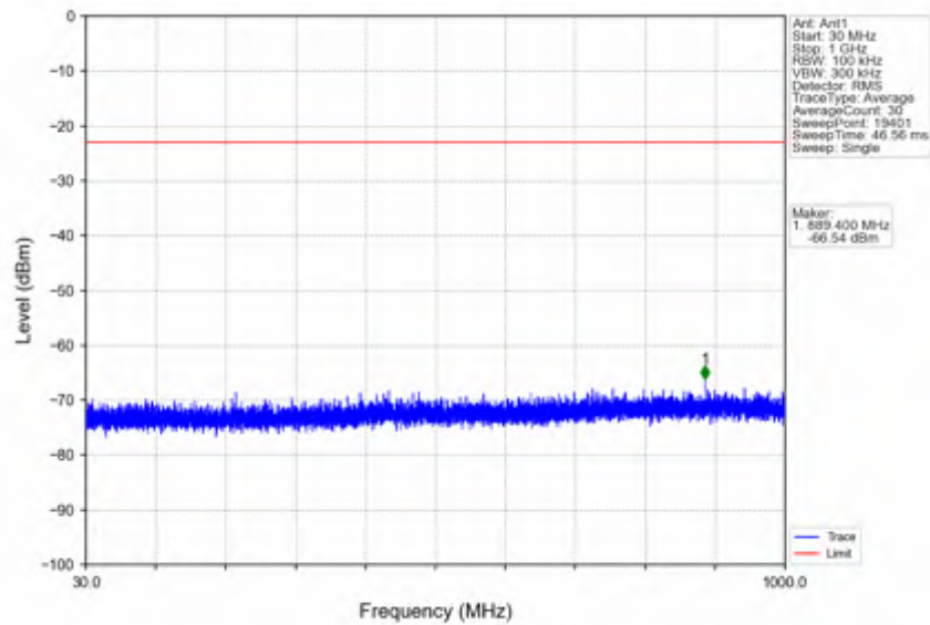
n78e_15kHz_SISO_NTNV_40MHz_DFT-s-OFDM QPSK_3470.01MHz_Edge_1RB_Left
