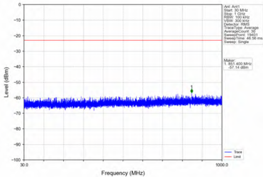
n78e_15kHz_SISO_NTNV_25MHz_DFT-s-OFDM PI/2 BPSK_3499.995MHz_Edge_1RB_Left
