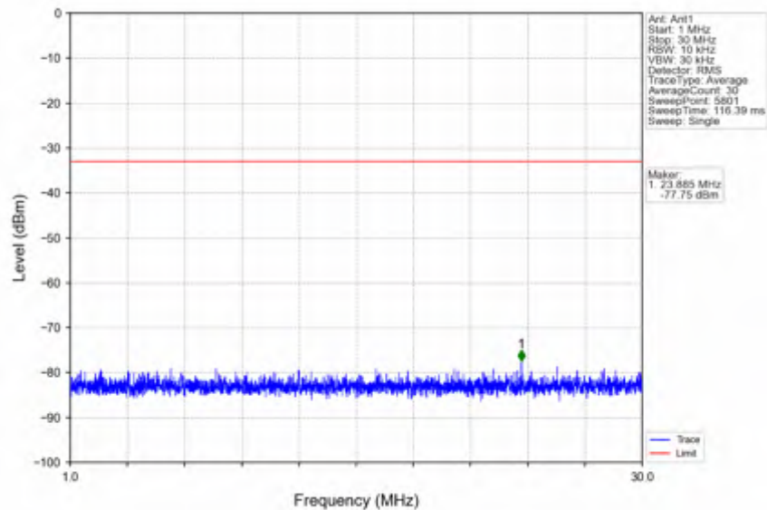
n78e_15kHz_SISO_NTNV_40MHz_DFT-s-OFDM_QPSK_3470.01MHz_Inner_1RB_Left
