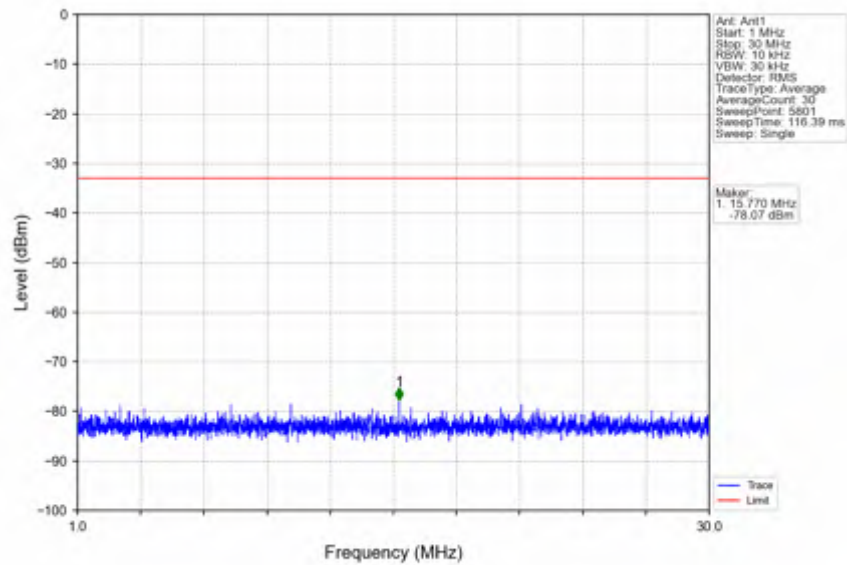
n78e_15kHz_SISO_NTNV_25MHz_CP-OFDM QPSK_3462.51MHz_Inner_1RB_Left
