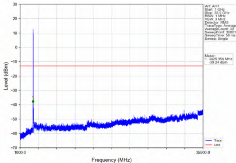
n78e_15kHz_SISO_NTNV_25MHz_DFT-s-OFDM PI/2 BPSK_3462.51MHz_Outer_Full
