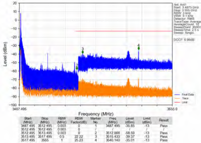
n78e_15kHz_SISO_NTV_25MHz_CP-OFDM_QPSK_3499.995MHz_Edge_1RB_Left
