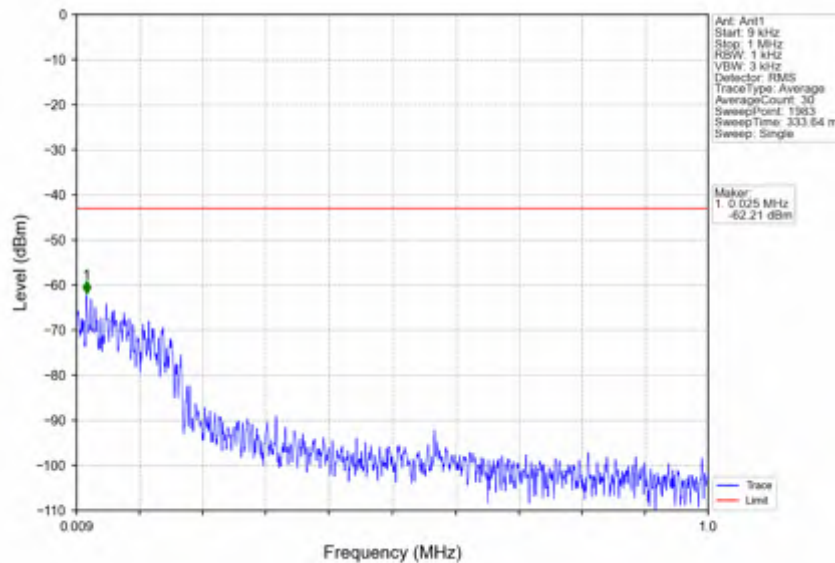
n78e_15kHz_SISO_NTNV_20MHz_CP-OFDM QPSK_3540MHz_Edge_1RB_Right
