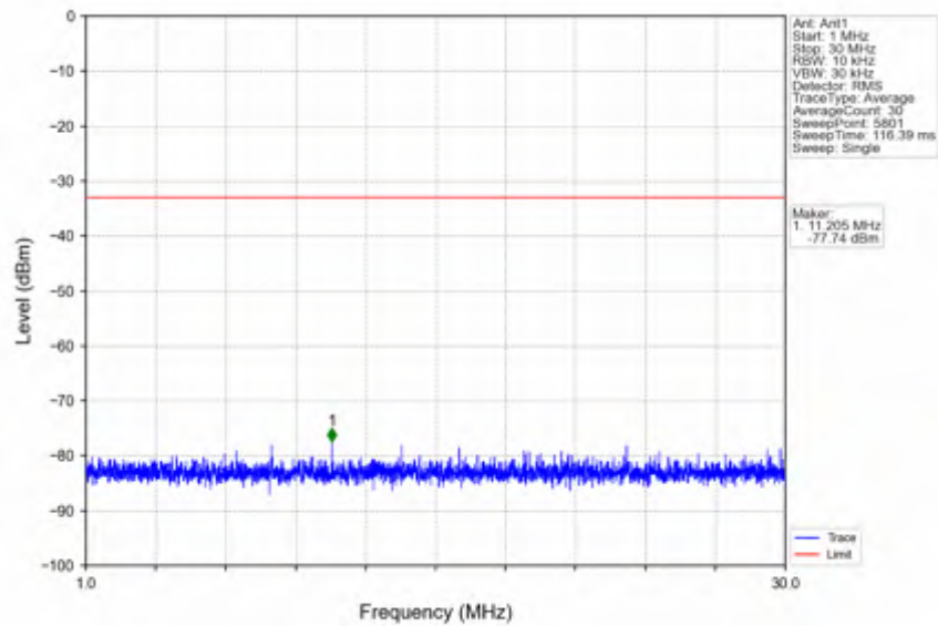
n78e_15kHz_SISO_NTNV_20MHz_CP-OFDM QPSK_3540MHz_Inner_1RB_Right
