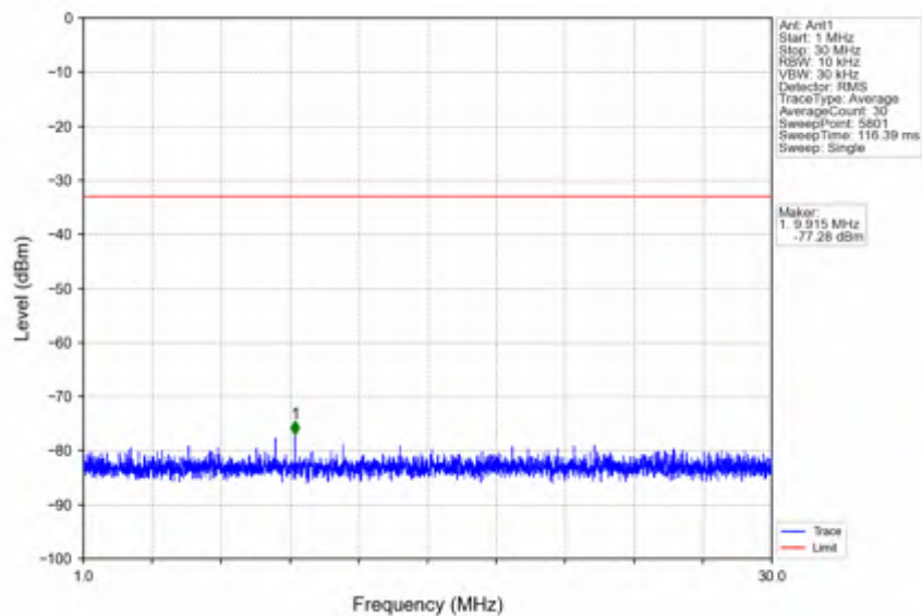
n78e_15kHz_SISO_NTNV_30MHz_DFT-s-OFDM QPSK_3534.99MHz_Inner_1RB_Right
