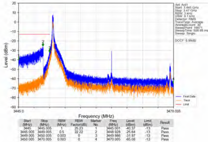
n78e_15kHz_SISO_NTNV_20MHz_CP-OFDM QPSK_3460.005MHz_Edge_1RB_Left
