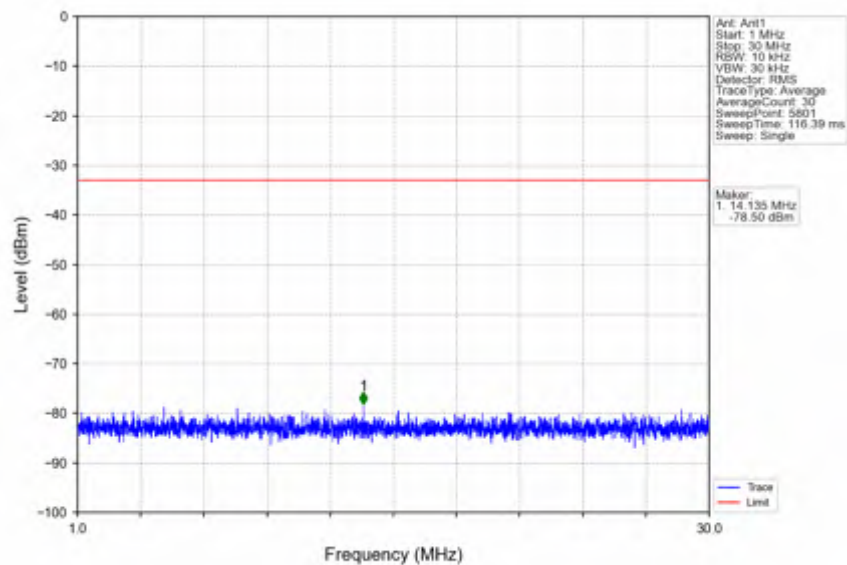
n78e_15kHz_SISO_NTNV_30MHz_CP-OFDM QPSK_3534.99MHz_Outer_Full
