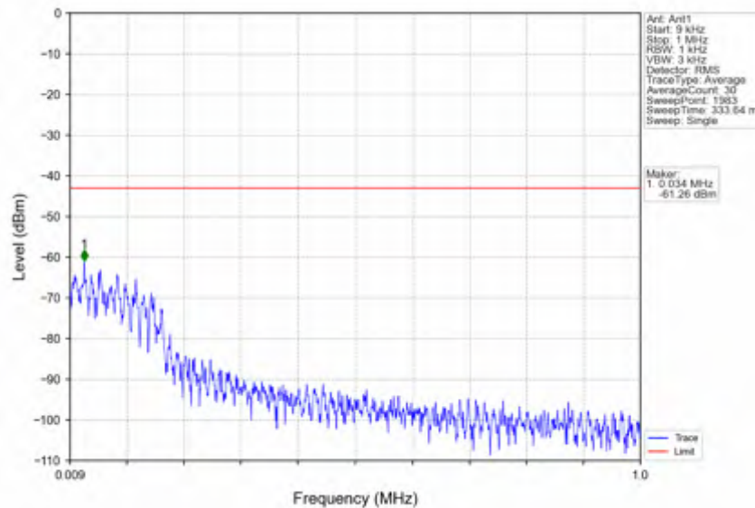
n78e_15kHz_SISO_NTNV_20MHz_CP-OFDM QPSK_3460.005MHz_Edge_1RB_Left
