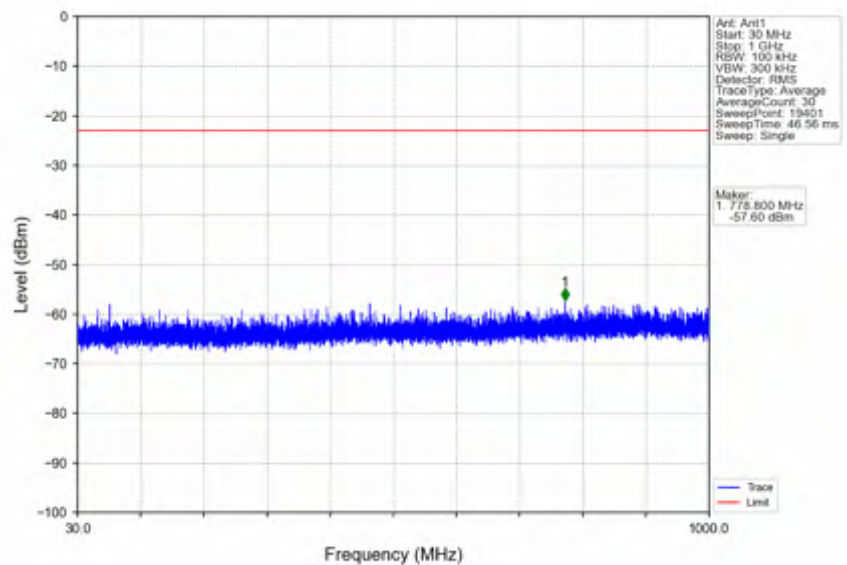
n78e_15kHz_SISO_NTNV_25MHz_DFT-s-OFDM QPSK_3499.995MHz_Edge_1RB_Left
